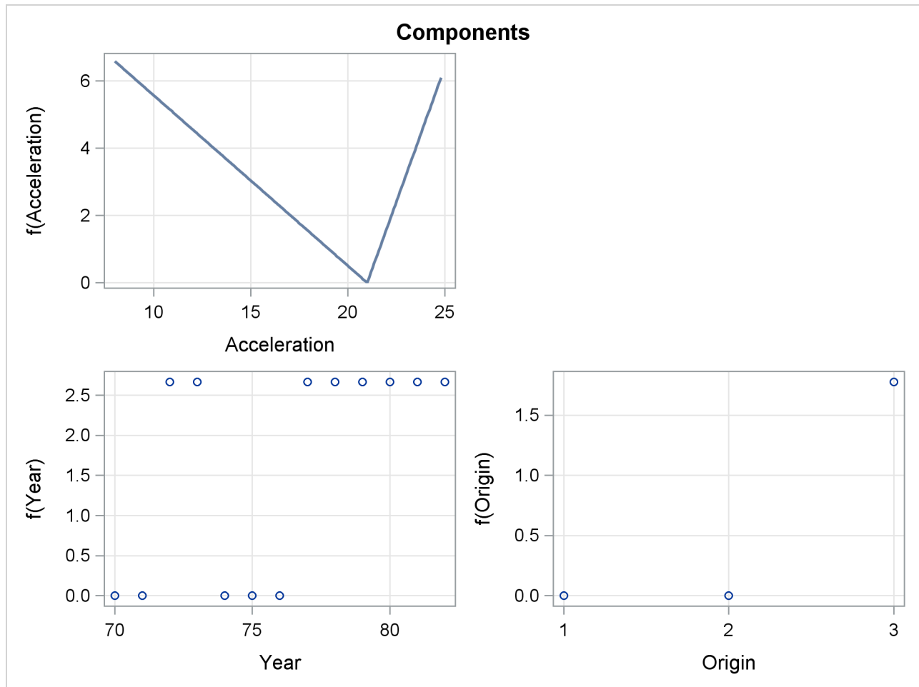
Figure 25.9 Component Panel 2
