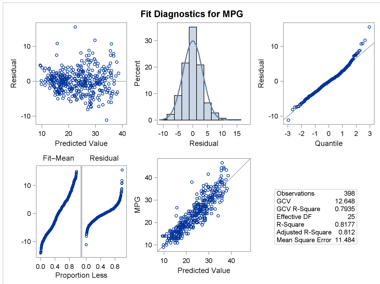
Figure 25.10 Diagnostics Panel
