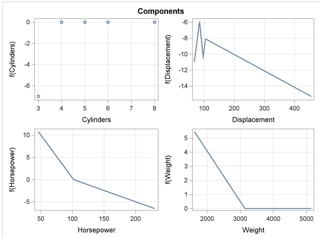
Figure 25.8 Component Panel 1
