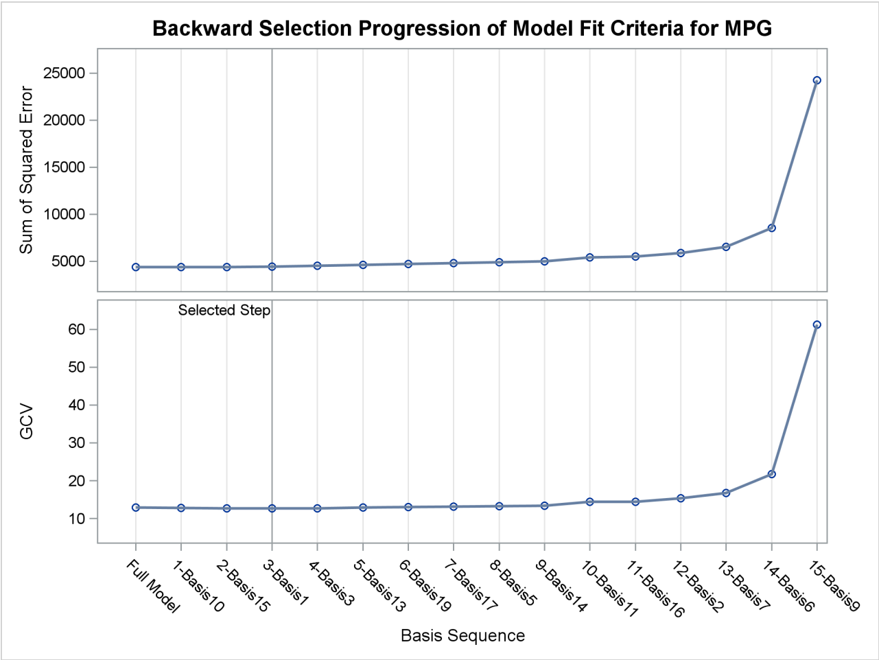
Figure 25.5 Selection Plot
