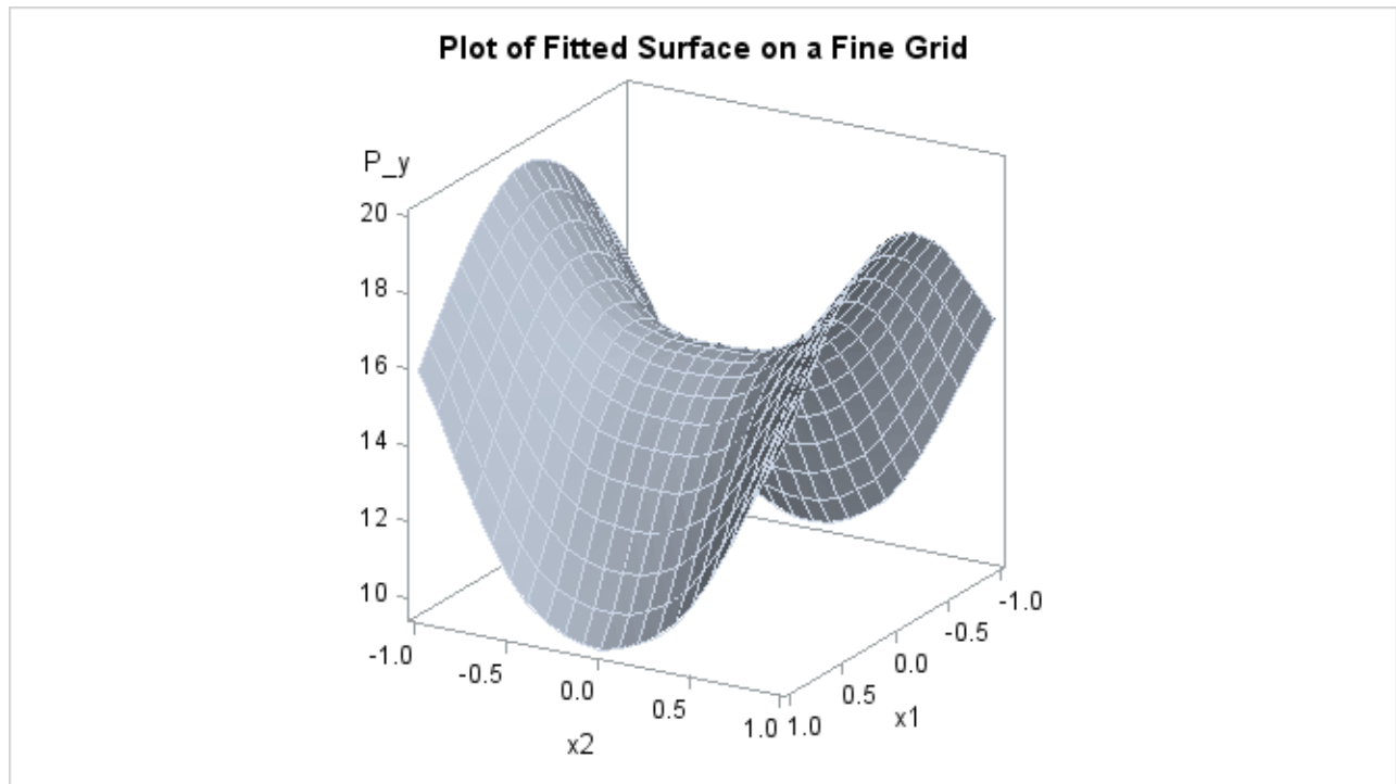
Figure 103.6 Plot of TPSPLINE Fit
