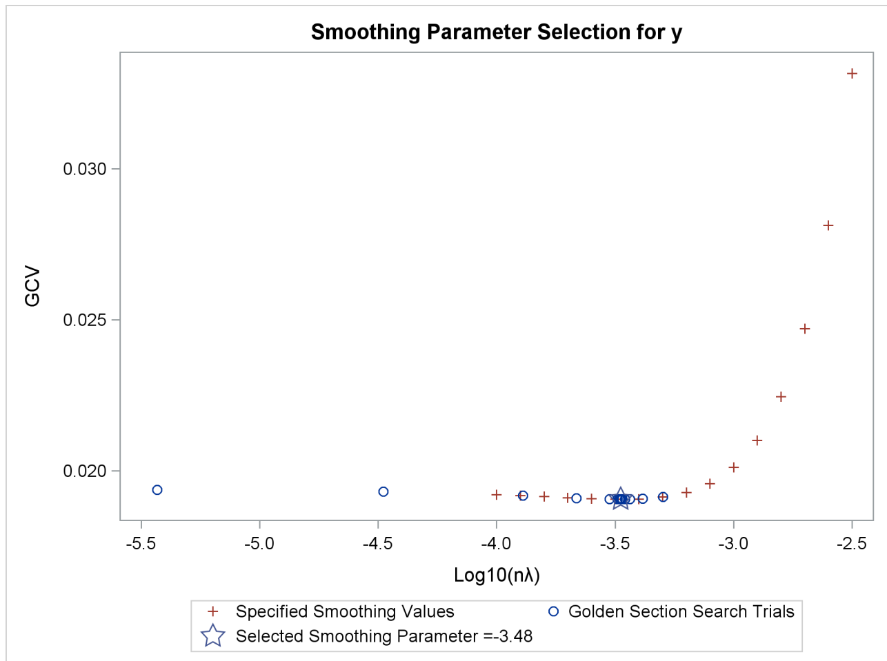
Figure 103.3 The GCV Criterion by \log_{10}(n\lambda)
