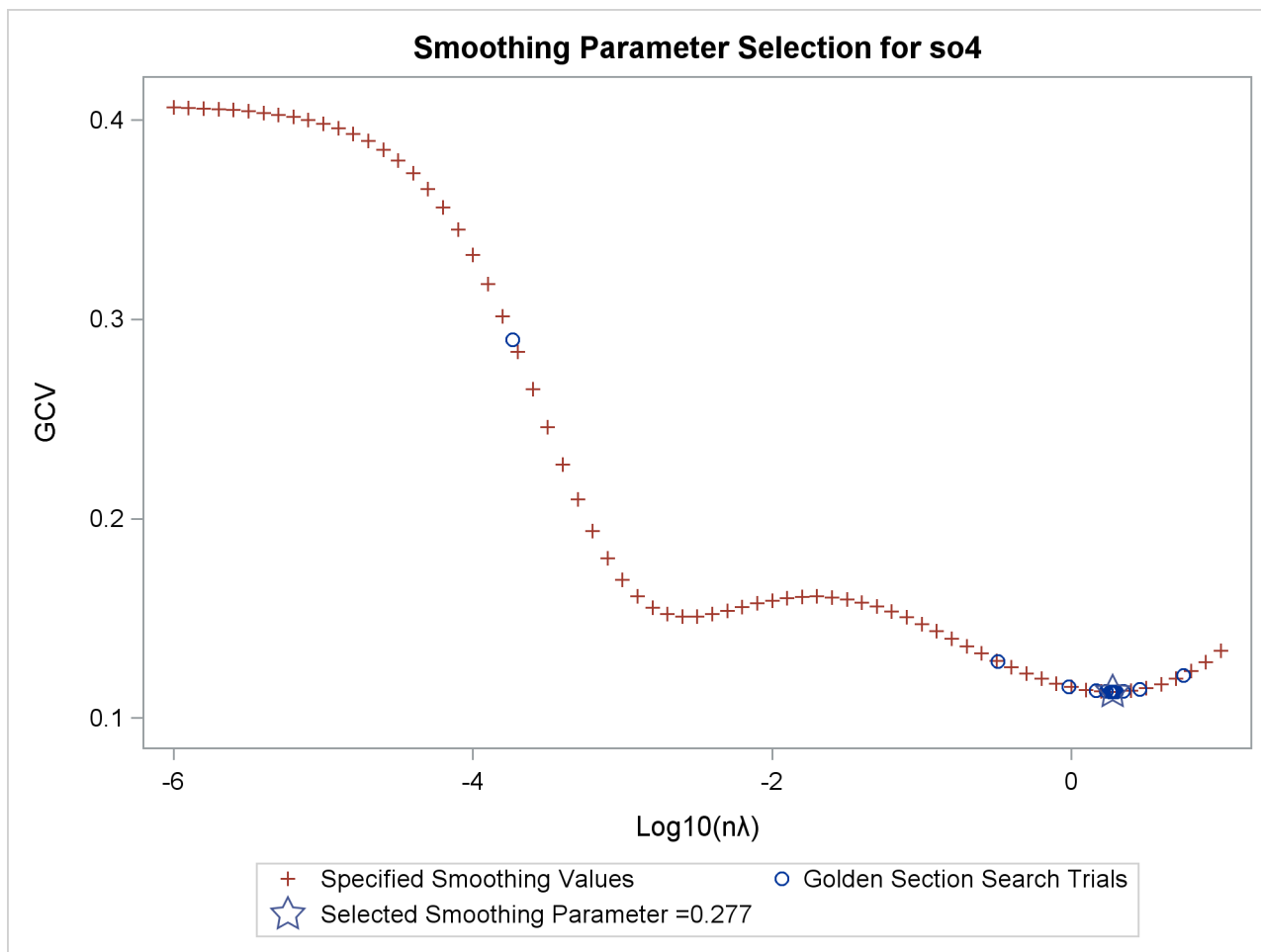
Output 103.3.3 GCV Function of SO 4 Data Set
