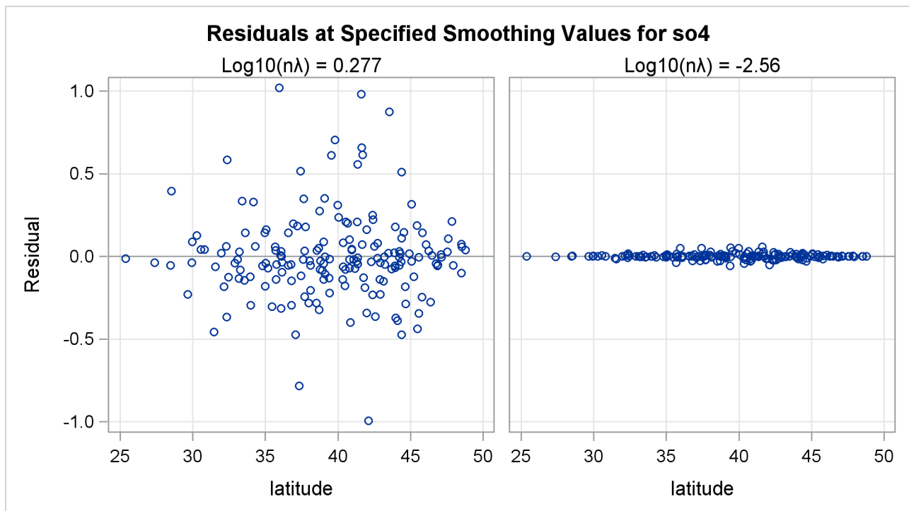
Output 103.3.6 Panel of Residuals by Latitude Plots
