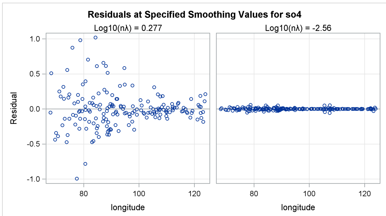
Output 103.3.7 Panel of Residuals by Longitude Plots
