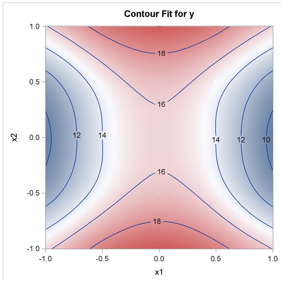
Figure 103.2 Fitted Surface from PROC TPSPLINE
