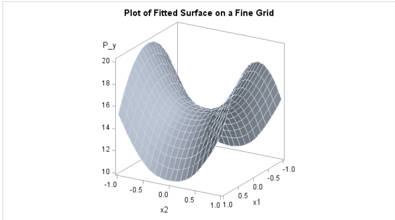
Output 103.1.2 Plot of PROC TPSPLINE Fit from the Partial Spline Model
