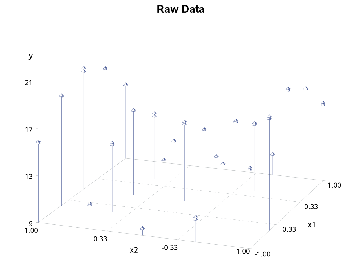
Figure 103.1 Plot of Data Set MEASURE
