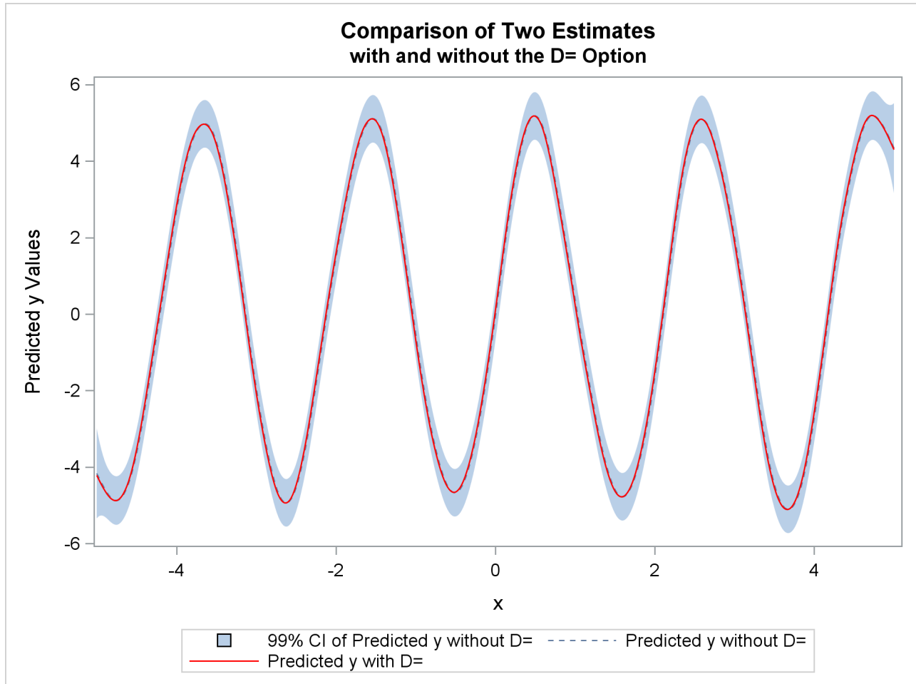
Output 103.4.3 Comparison of Two PROC TPSPLINE Fits with and without the D= Option
