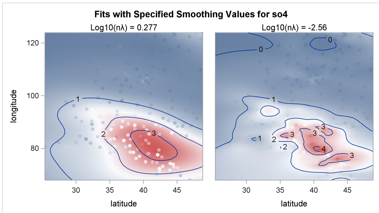
Output 103.3.5 Panel of Contour Fit Plots by 0.277 and -2.56
