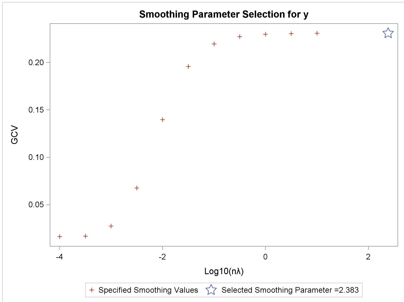
Output 103.2.4 Criterion Plot
