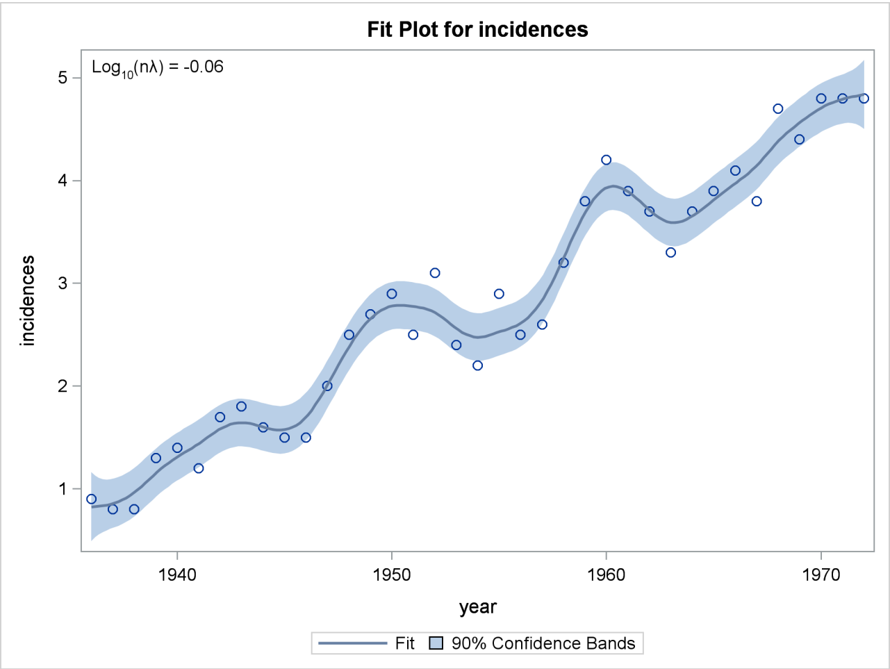
Output 103.5.2 PROC TPSPLINE Estimate and 90% Confidence Interval of Data Set MELANOMA
