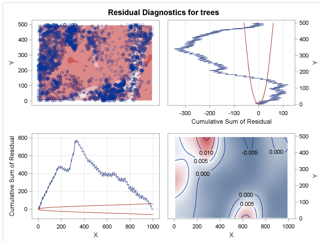
Figure 93.10 Residual Diagnostics for Fitted Log-Intensity Model
