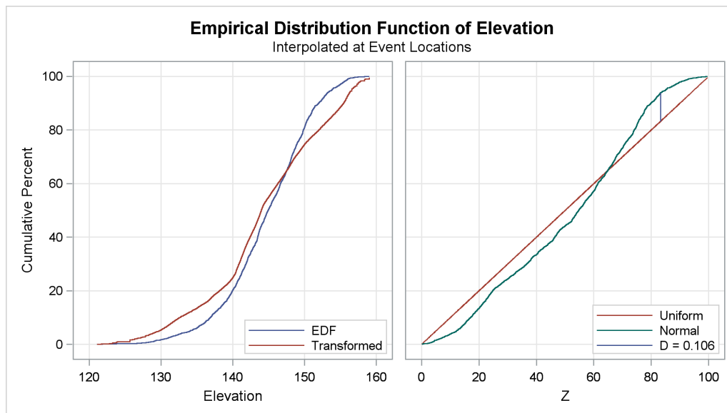
Output 93.2.3 Kolmogorov-Smirnov CSR Test Plot for Elevation
