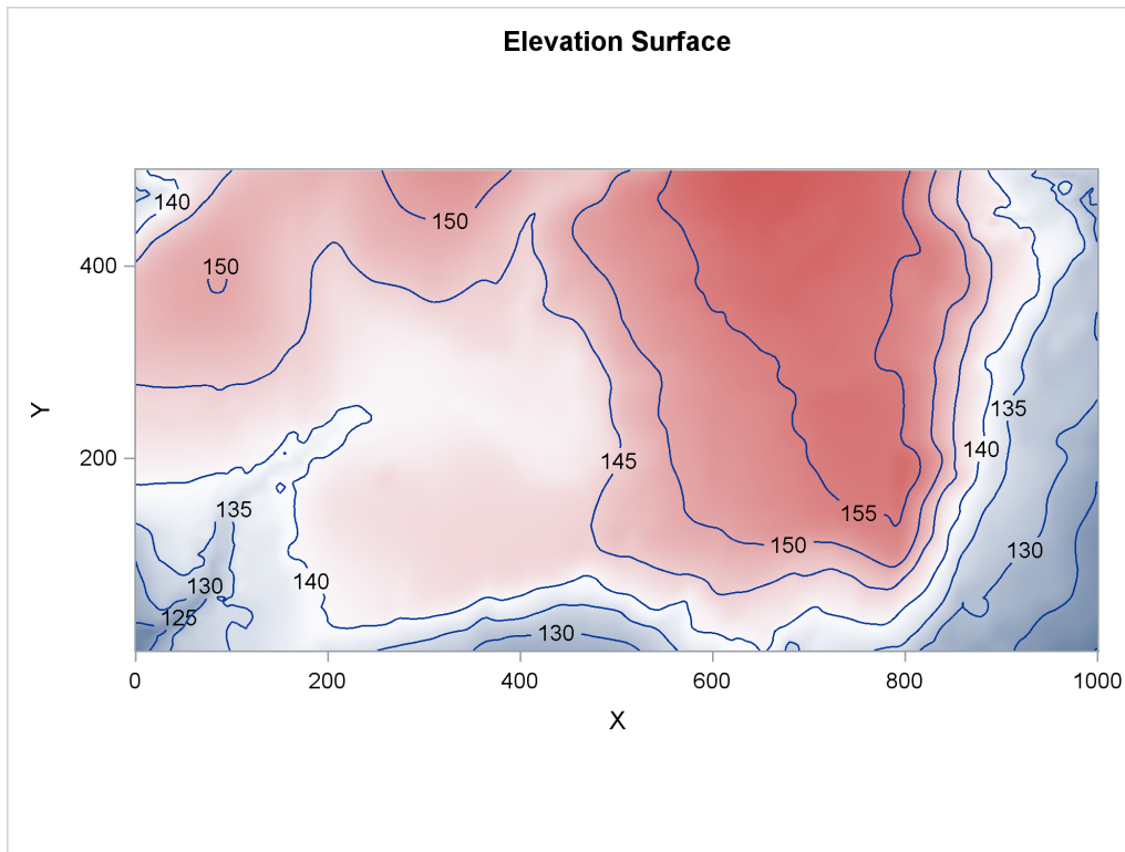
Figure 93.6 Spatial Covariate Elevation
