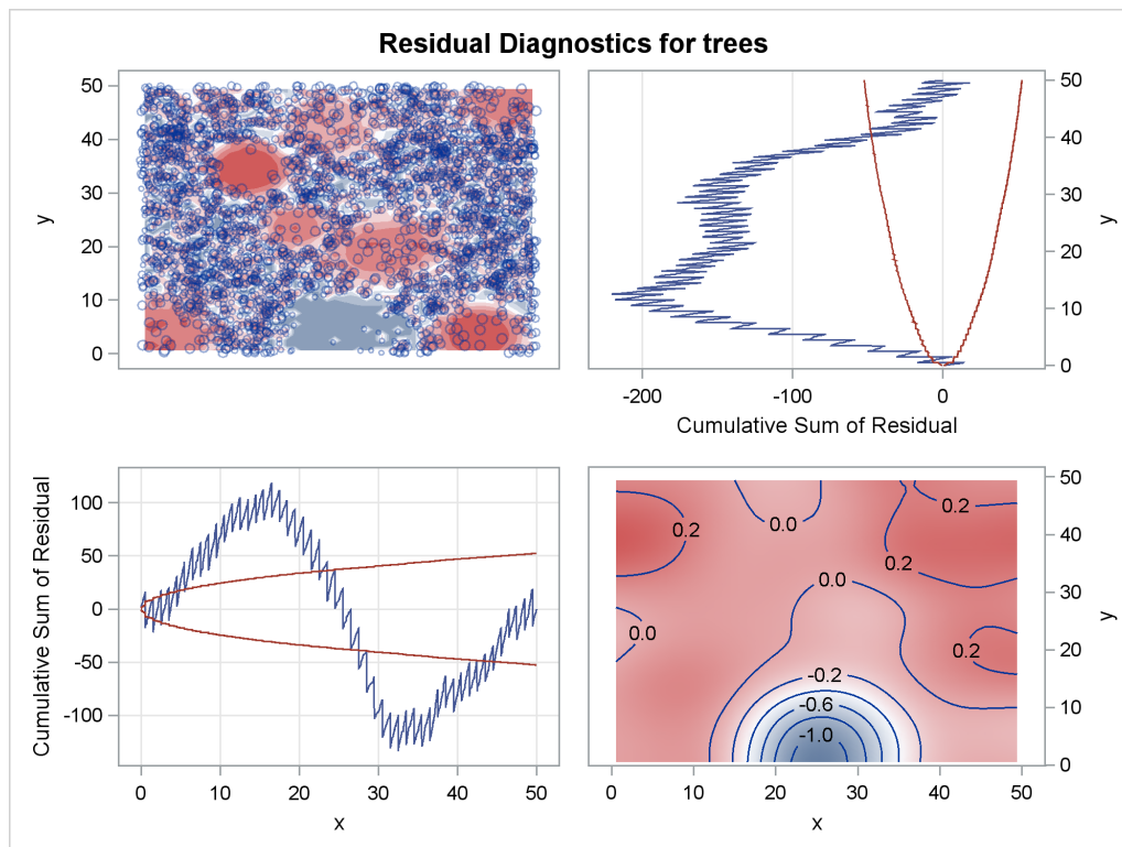
Output 93.3.5 Residual Diagnostics for the Fitted Model
