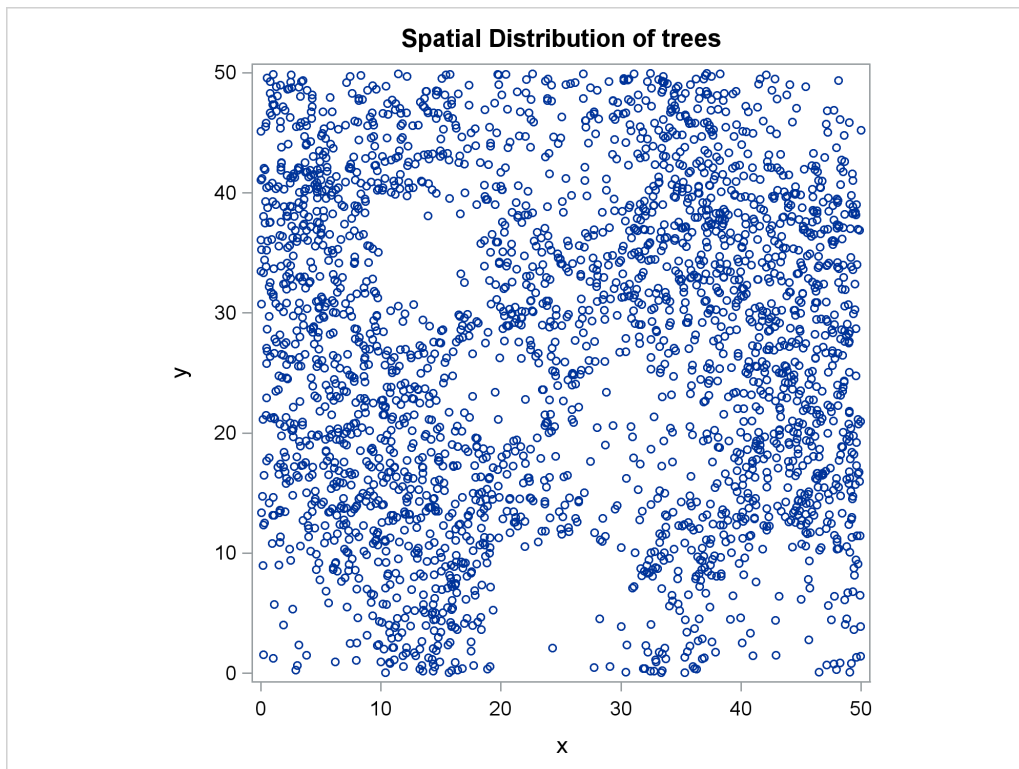
Output 93.3.1 Spatial Point Pattern of Simulated Flowers
