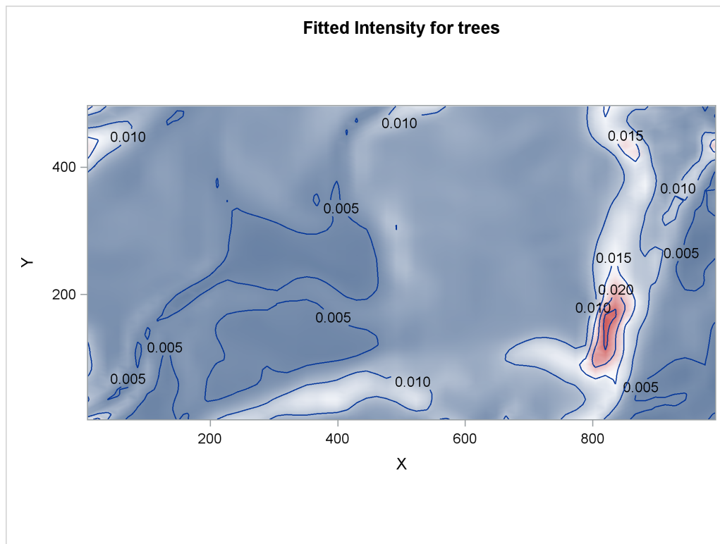
Figure 93.9 Intensity Estimates of Tree presence in Study Area
