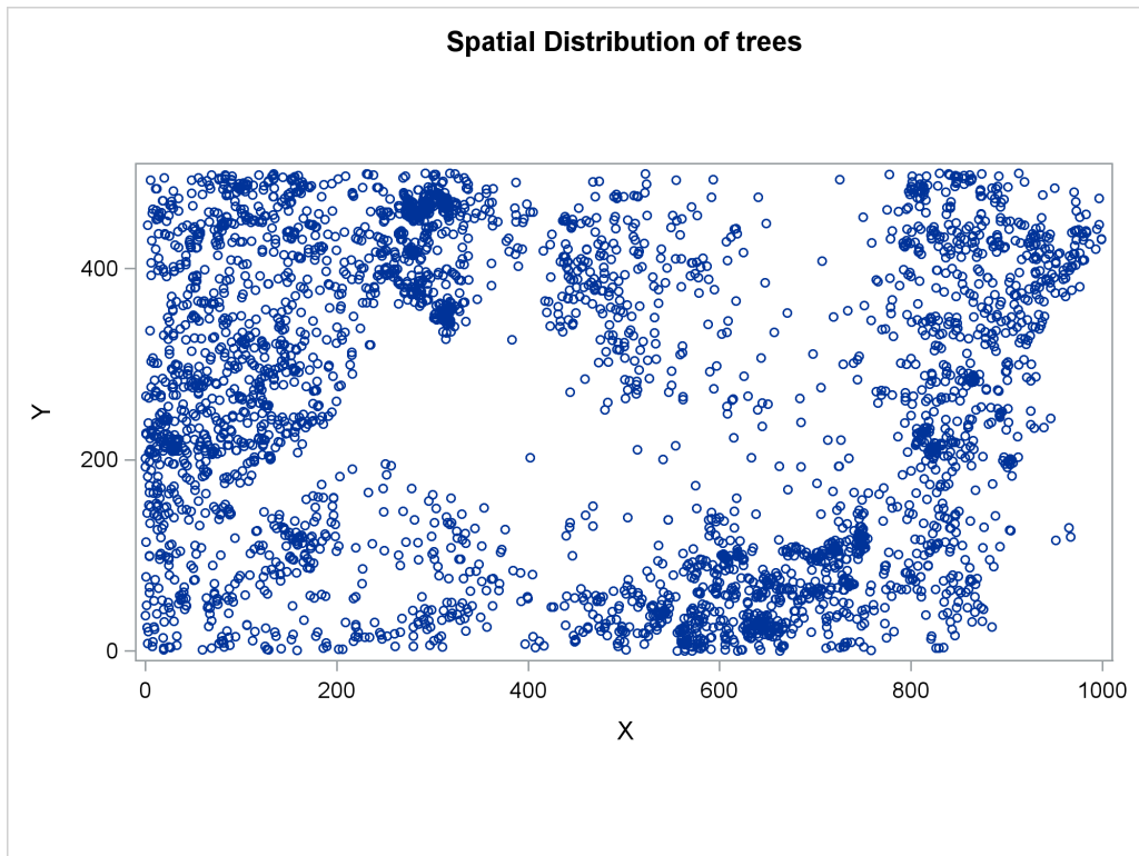
Figure 93.4 Spatial Point Pattern of Tropical Rain forest Trees
