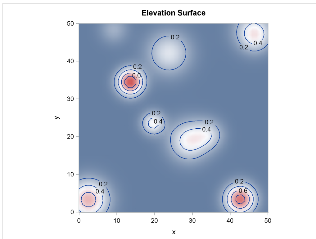
Output 93.3.2 Spatial Covariate Elevation
