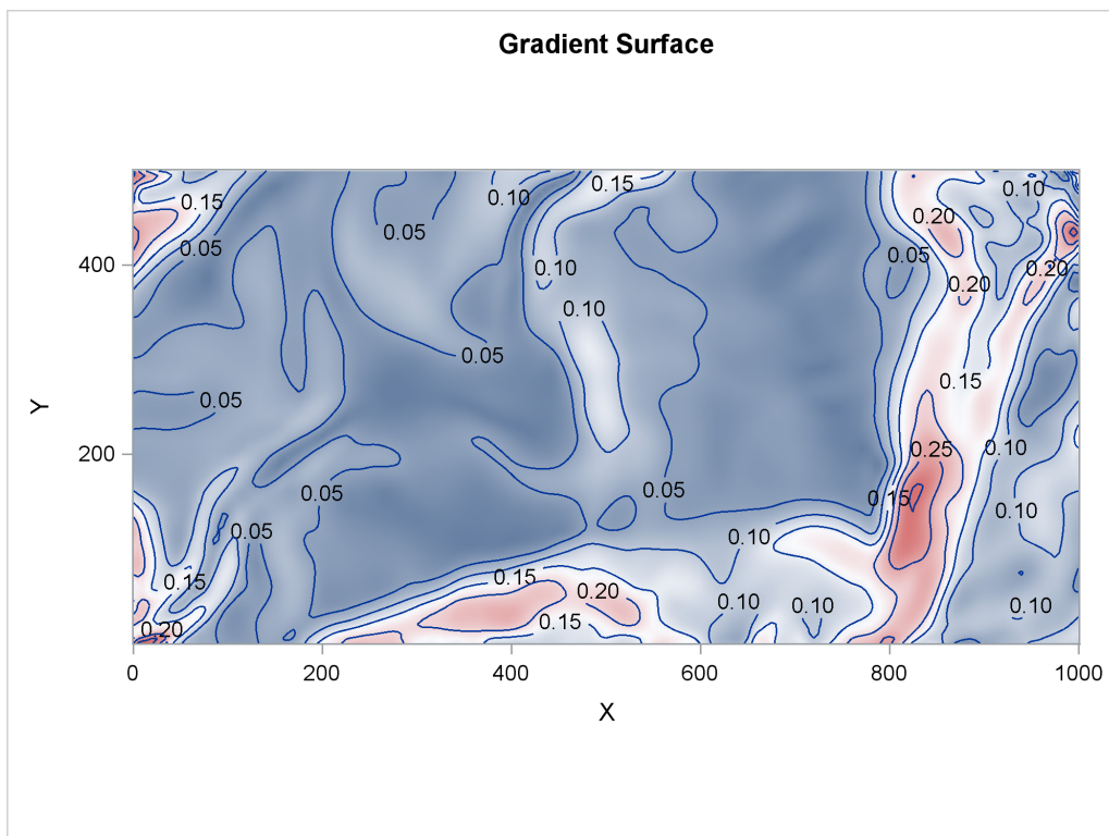
Figure 93.5 Spatial Covariate Gradient
