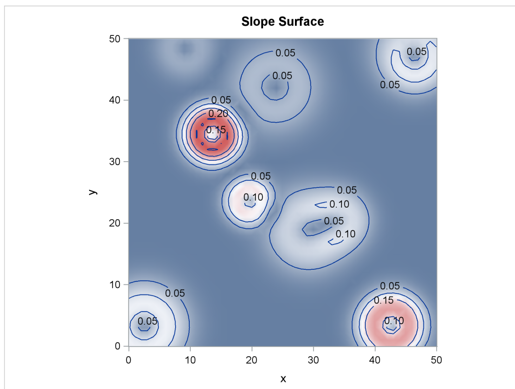
Output 93.3.3 Spatial Covariate Slope
