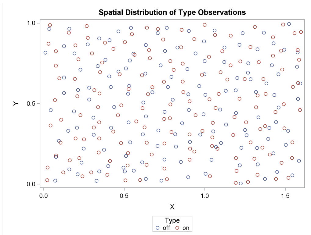
Output 93.1.1 Amacrine Cell Types
