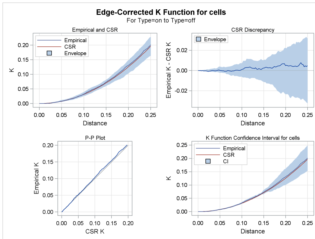
Output 93.1.4 Cross-K Function Panel
