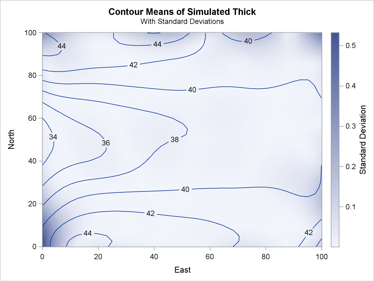
Figure 91.5 Contour Plot of Conditionally Simulated Coal Seam Thickness
