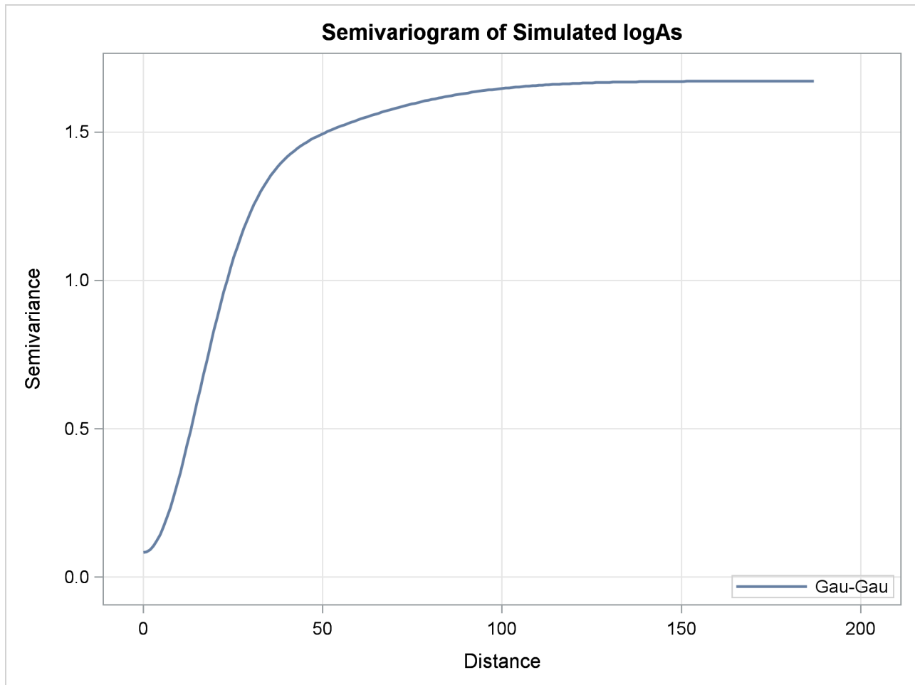
Output 91.3.6 Gaussian-Gaussian Semivariogram Model Used in Simulation
