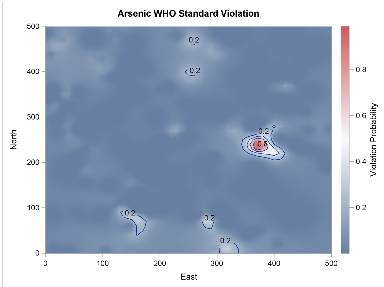
Output 91.3.9 Map of Violation of the Arsenic WHO Standard Probability
