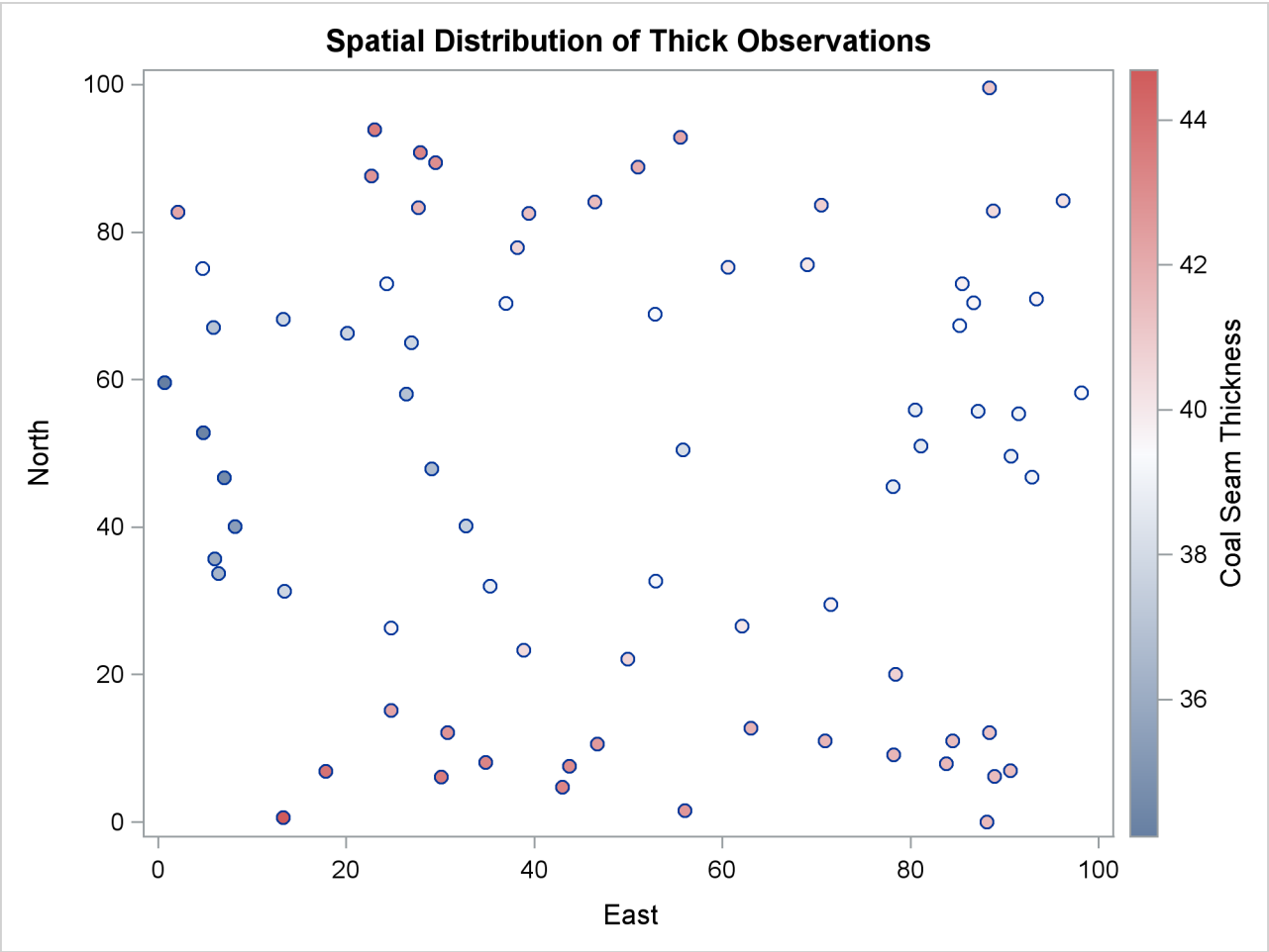
Figure 91.2 Scatter Plot of the Observations Spatial Distribution
