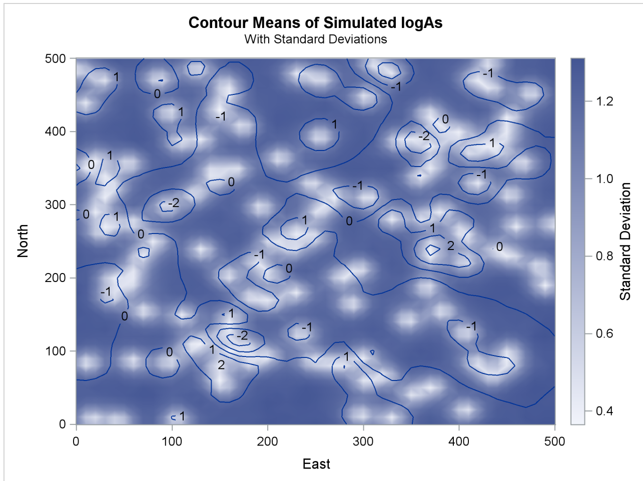
Output 91.3.7 Simulated Arsenic Logarithm Values with Gaussian-Gaussian Covariance
