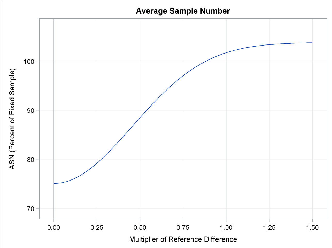
Output 90.3.15 ASN Plot
