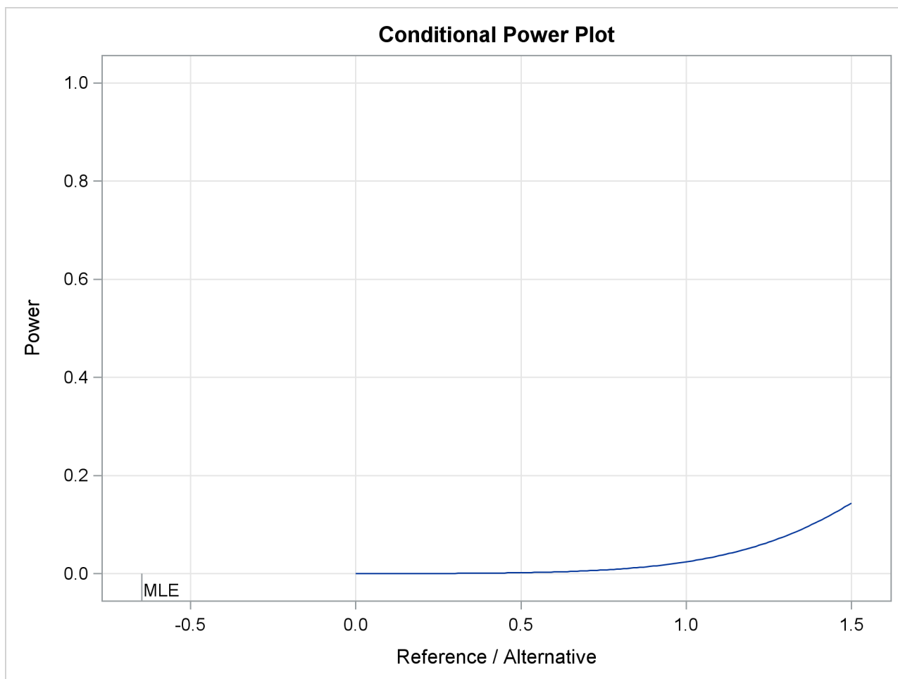
Output 90.4.16 Conditional Power Plot
