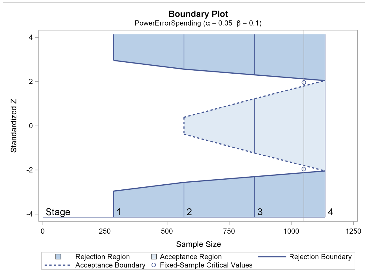
Figure 90.20 Boundary Plot for Two-Sided Test
