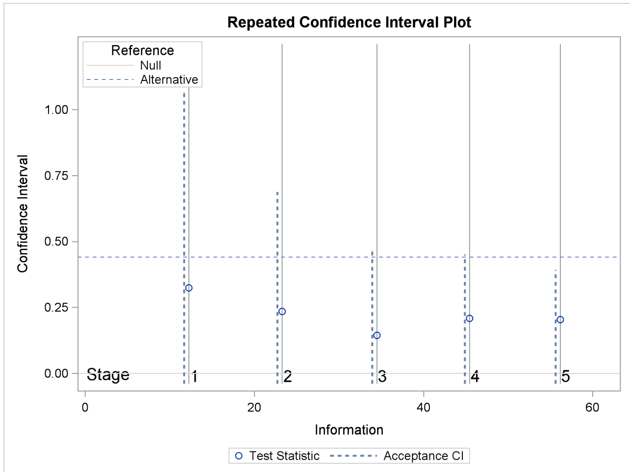
Output 90.5.18 Repeated Confidence Intervals Plot
