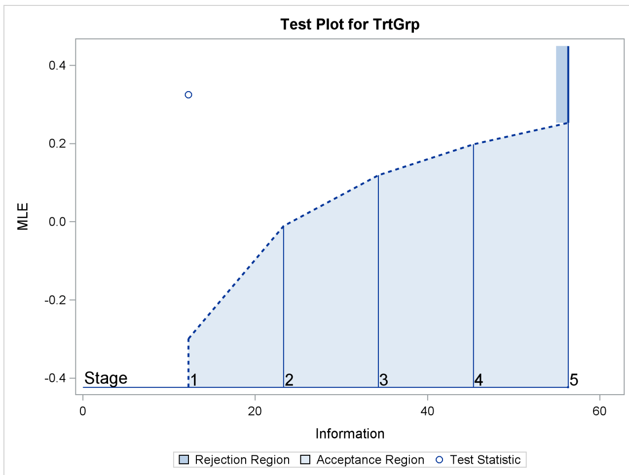
Output 90.5.10 Sequential Test Plot
