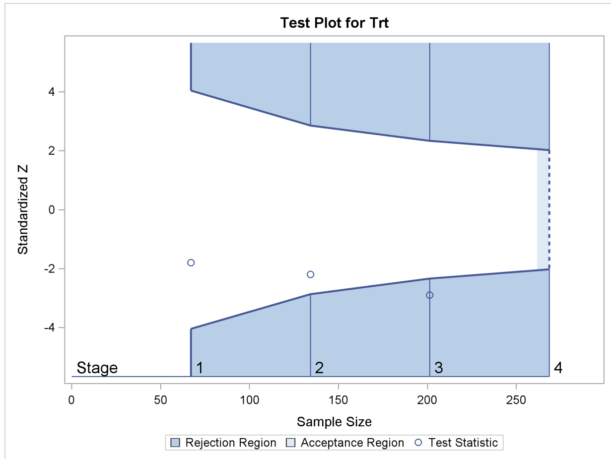
Figure 90.1 Sequential Plot for Two-Sided Test
