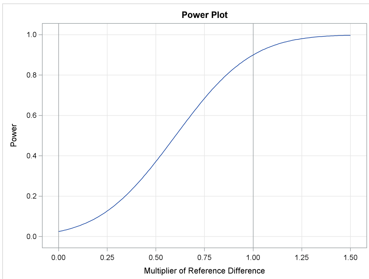
Output 90.3.16 Power Plot
