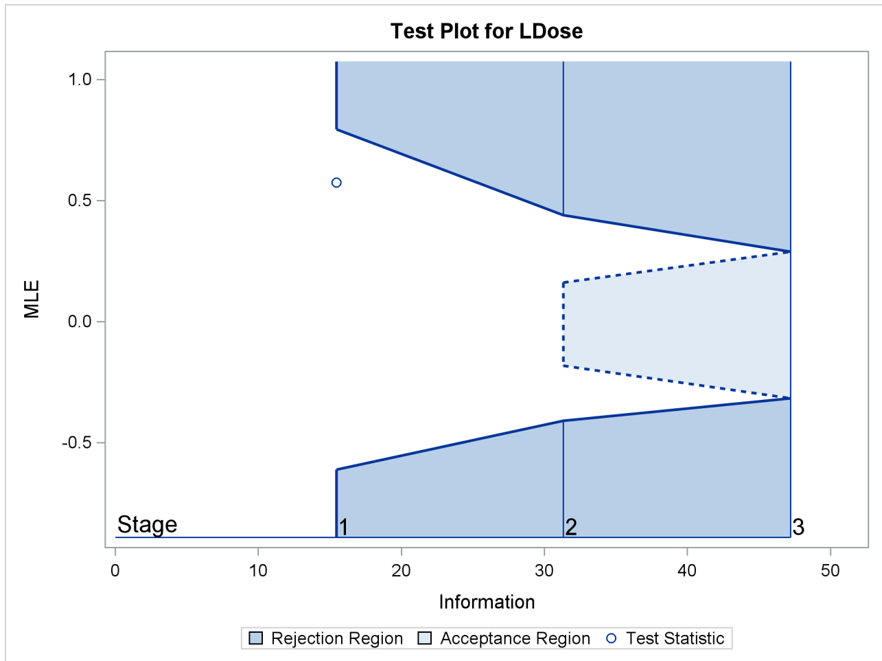
Output 90.8.10 Sequential Test Plot
