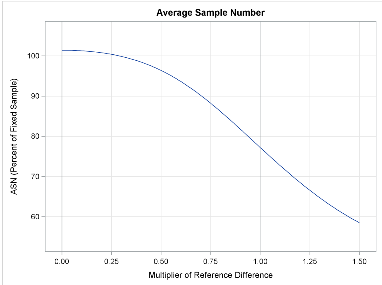
Output 90.2.16 ASN Plot
