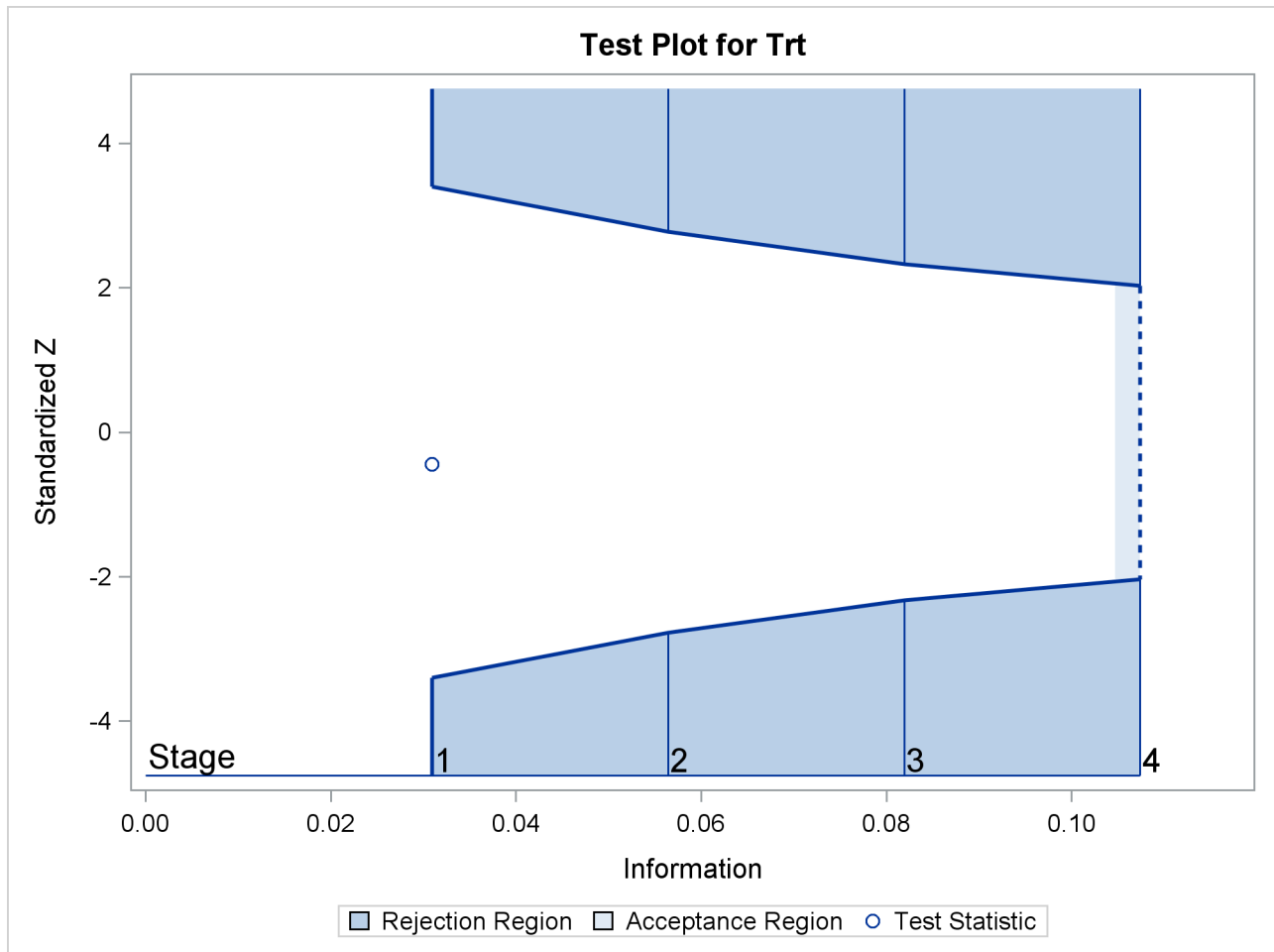
Figure 90.12 Sequential Test Plot
