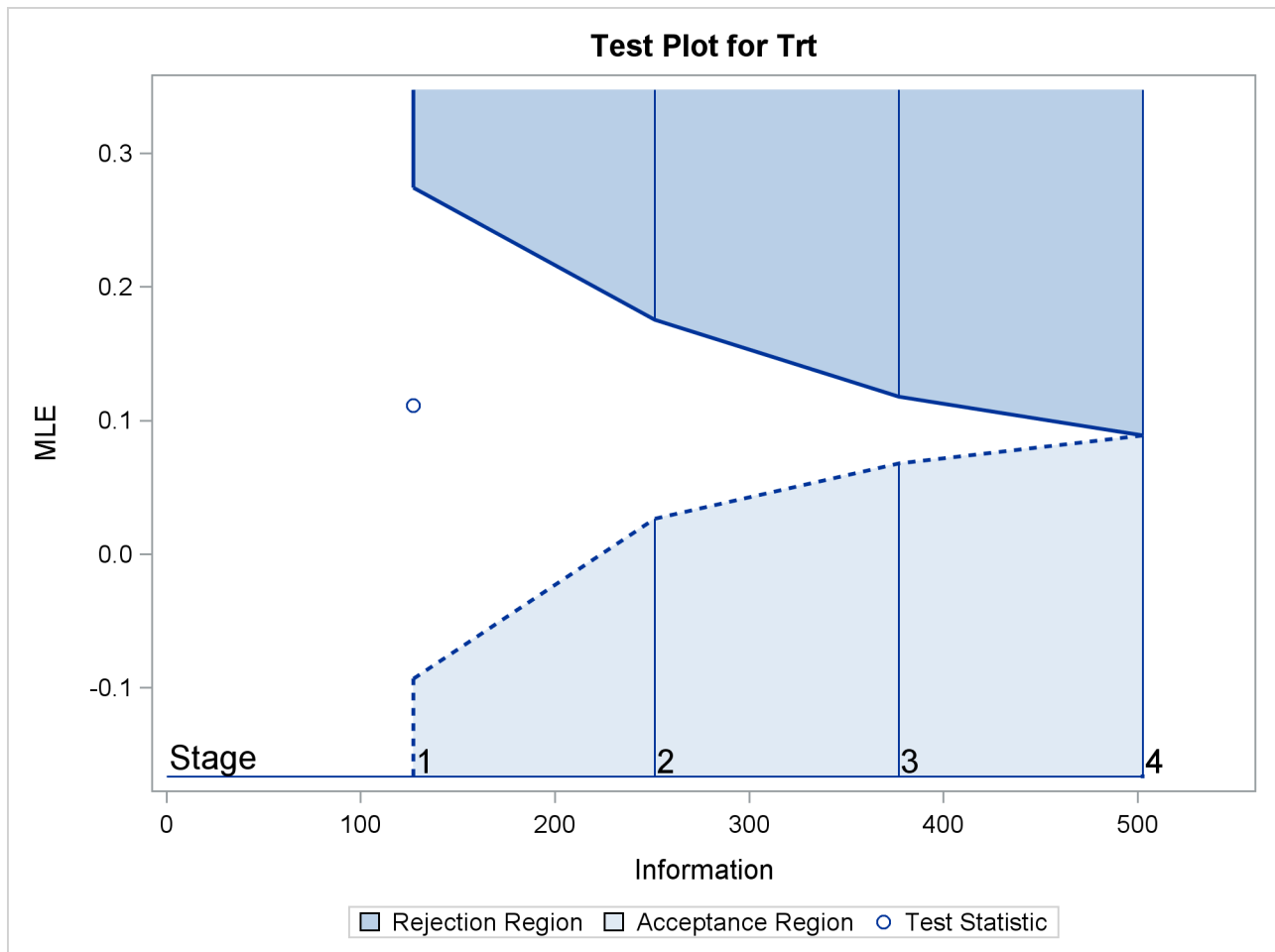
Output 90.1.13 Sequential Test Plot
