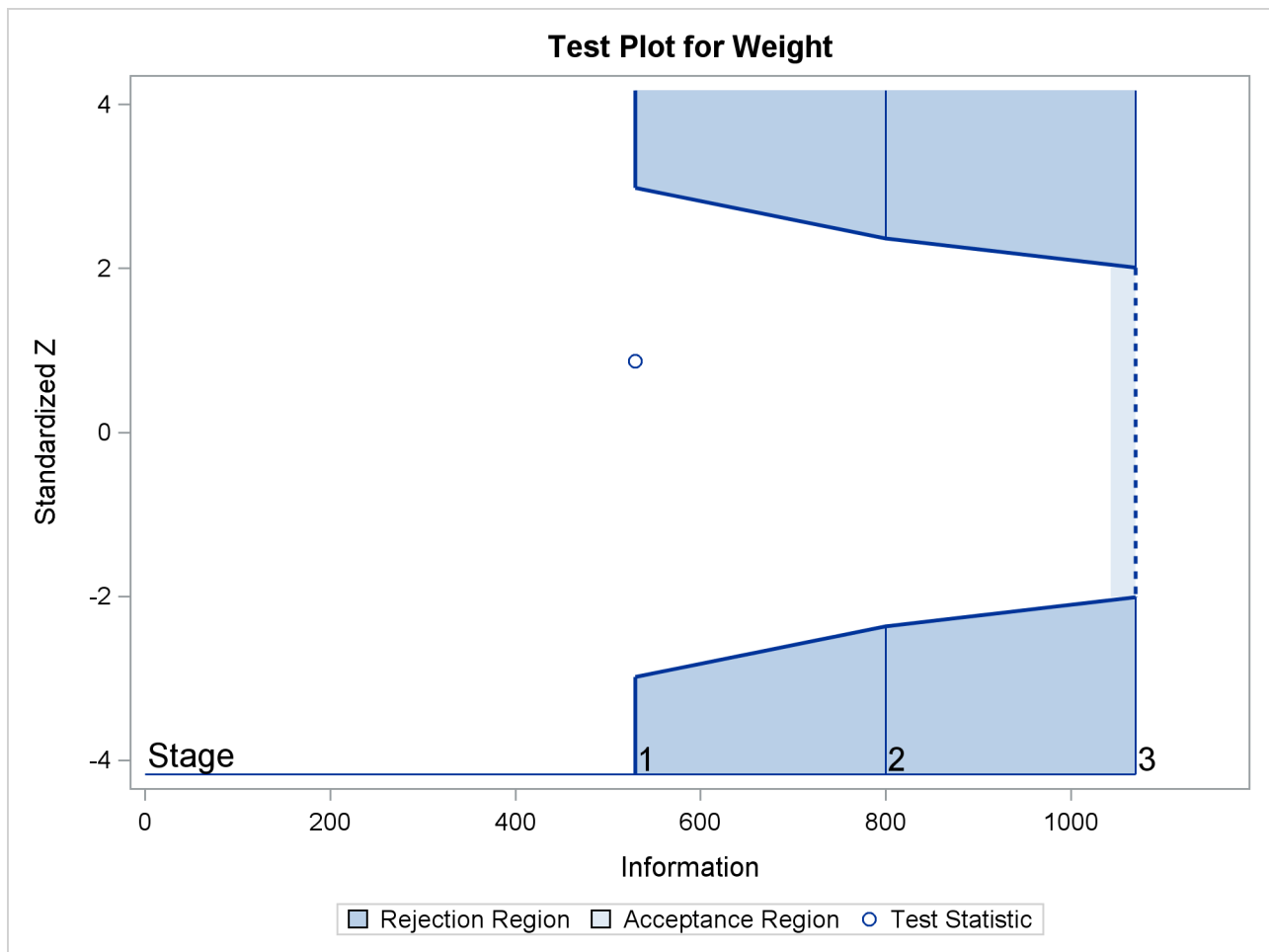
Output 90.2.11 Sequential Test Plot
