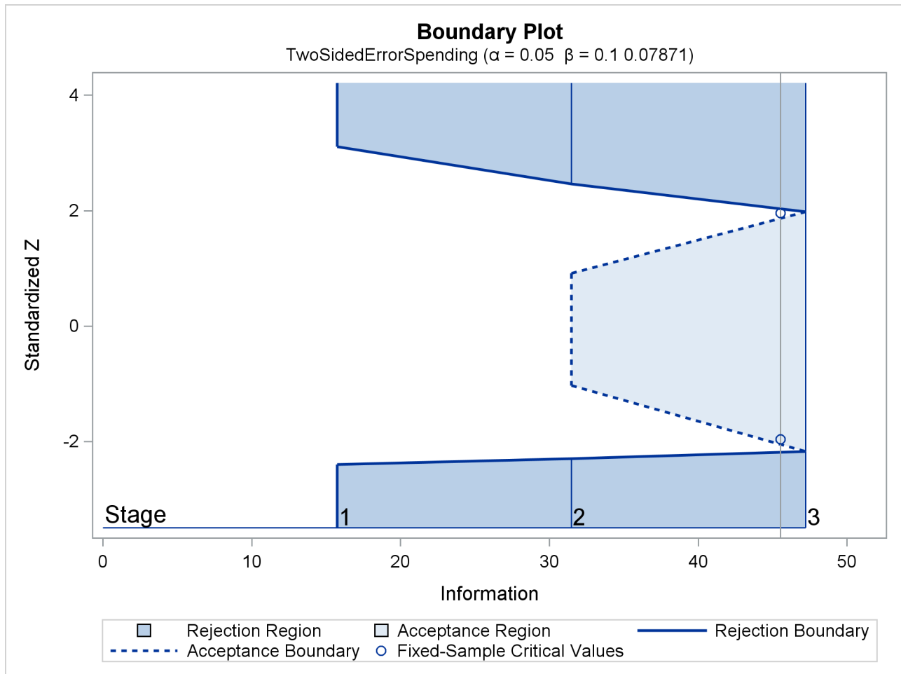
Output 90.8.3 Boundary Plot
