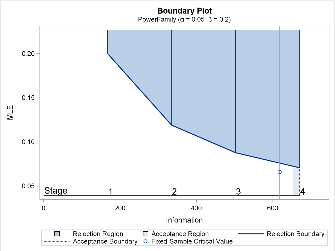
Output 90.4.3 Boundary Plot
