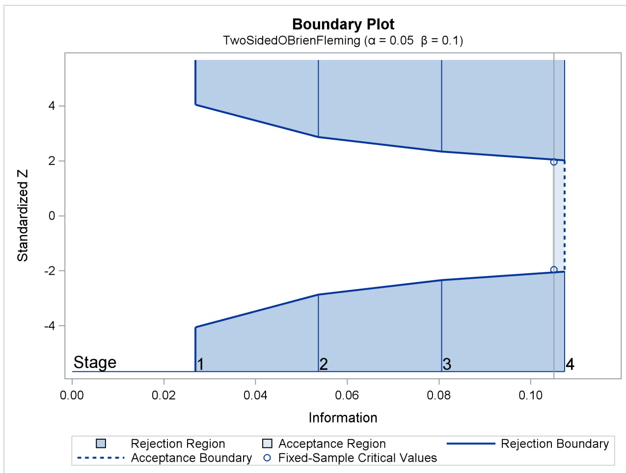
Figure 90.5 O'Brien-Fleming Boundary Plot
