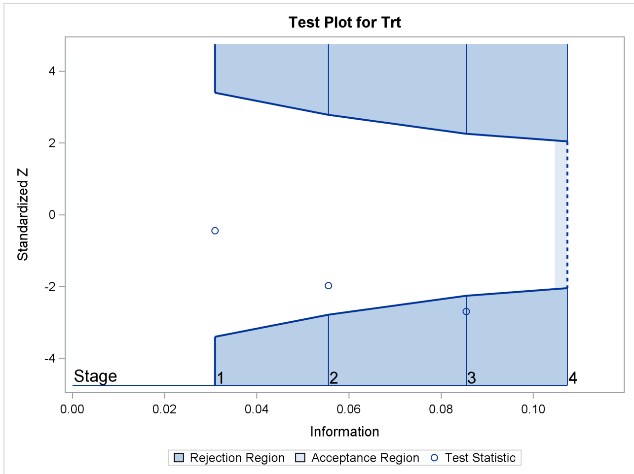
Figure 90.17 Sequential Test Plot
