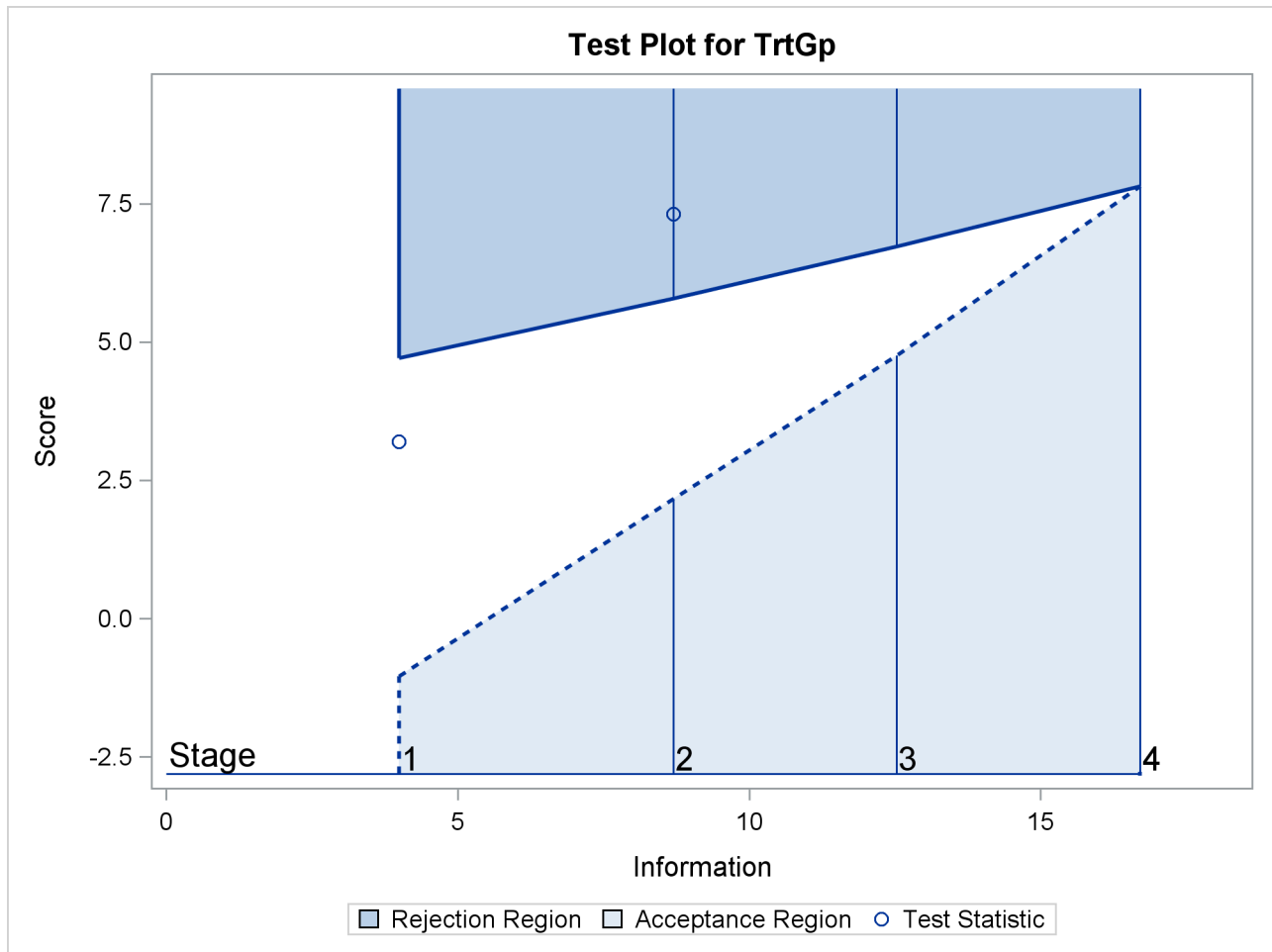
Output 90.6.16 Sequential Test Plot
