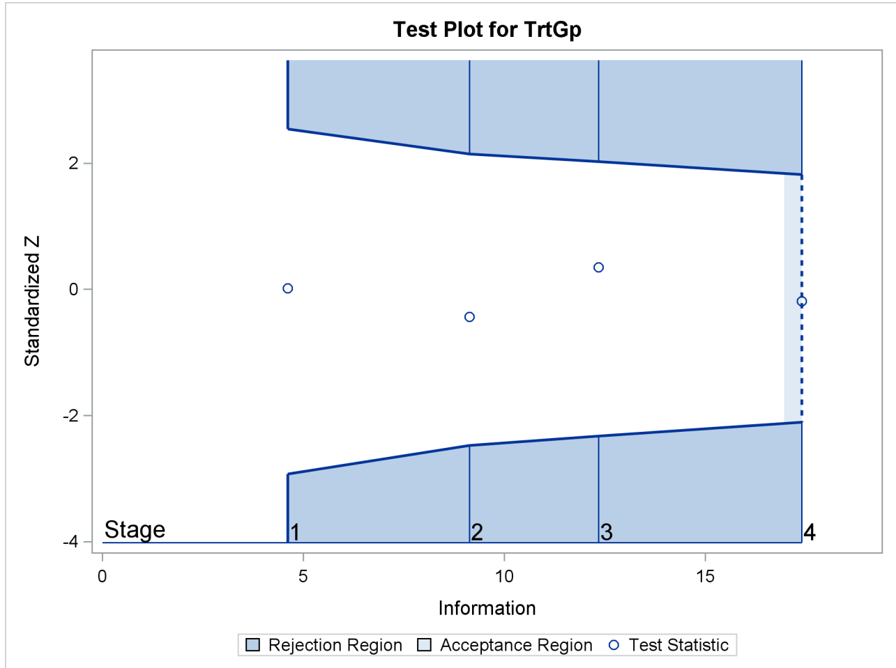
Output 90.7.16 Sequential Test Plot
