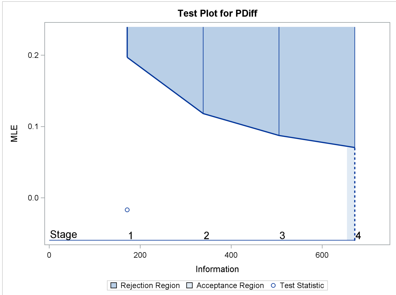
Output 90.4.11 Sequential Test Plot
