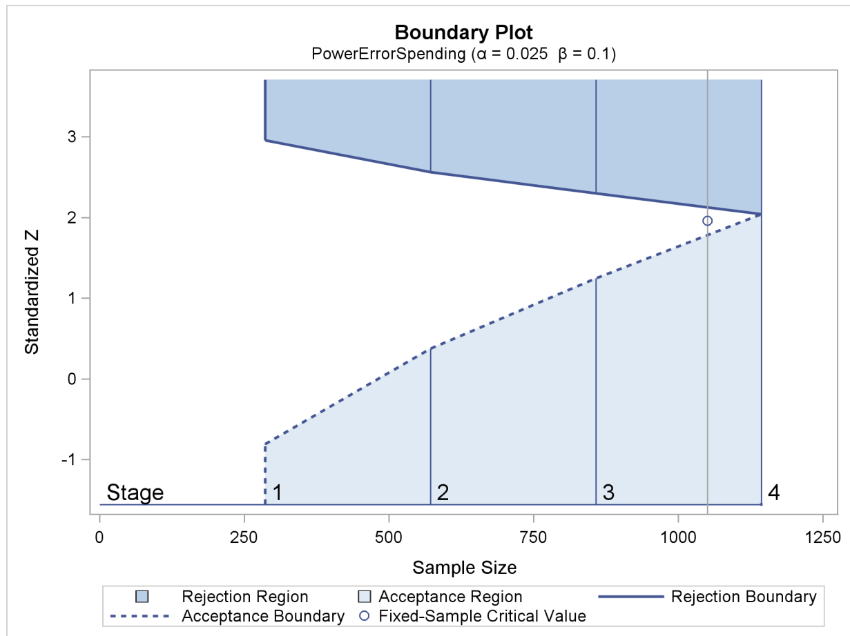
Figure 90.19 Boundary Plot for One-Sided Test
