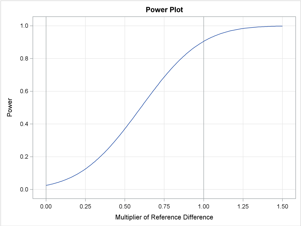
Output 90.2.17 Power Plot
