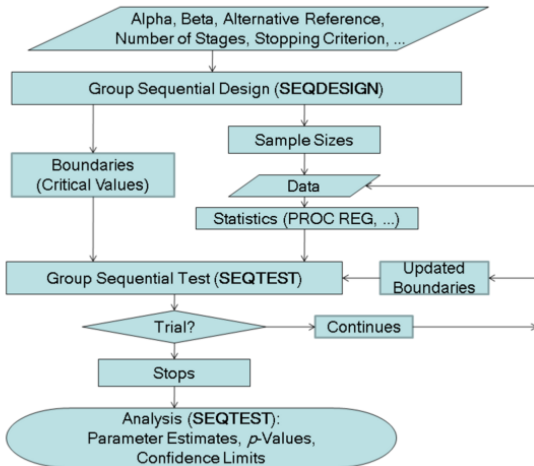
Figure 90.2 Group Sequential Trial
