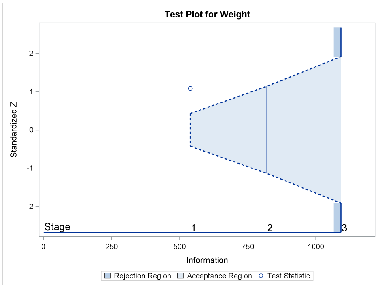
Output 90.3.11 Sequential Test Plot
