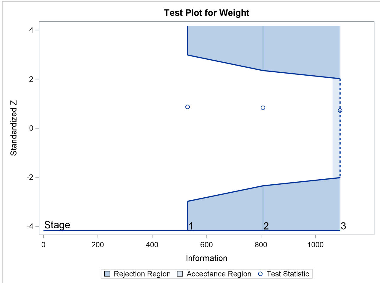
Output 90.2.19 Sequential Test Plot
