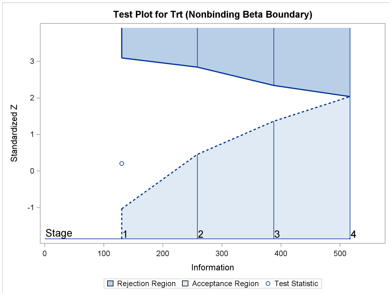
Output 90.9.13 Sequential Test Plot
