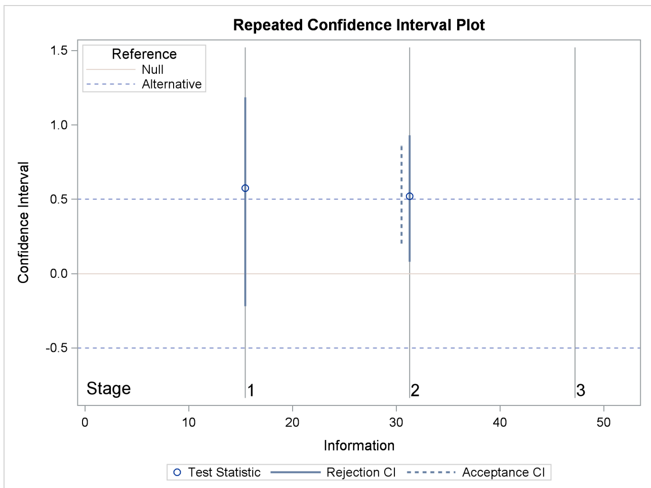
Output 90.8.17 Repeated Confidence Intervals Plot
