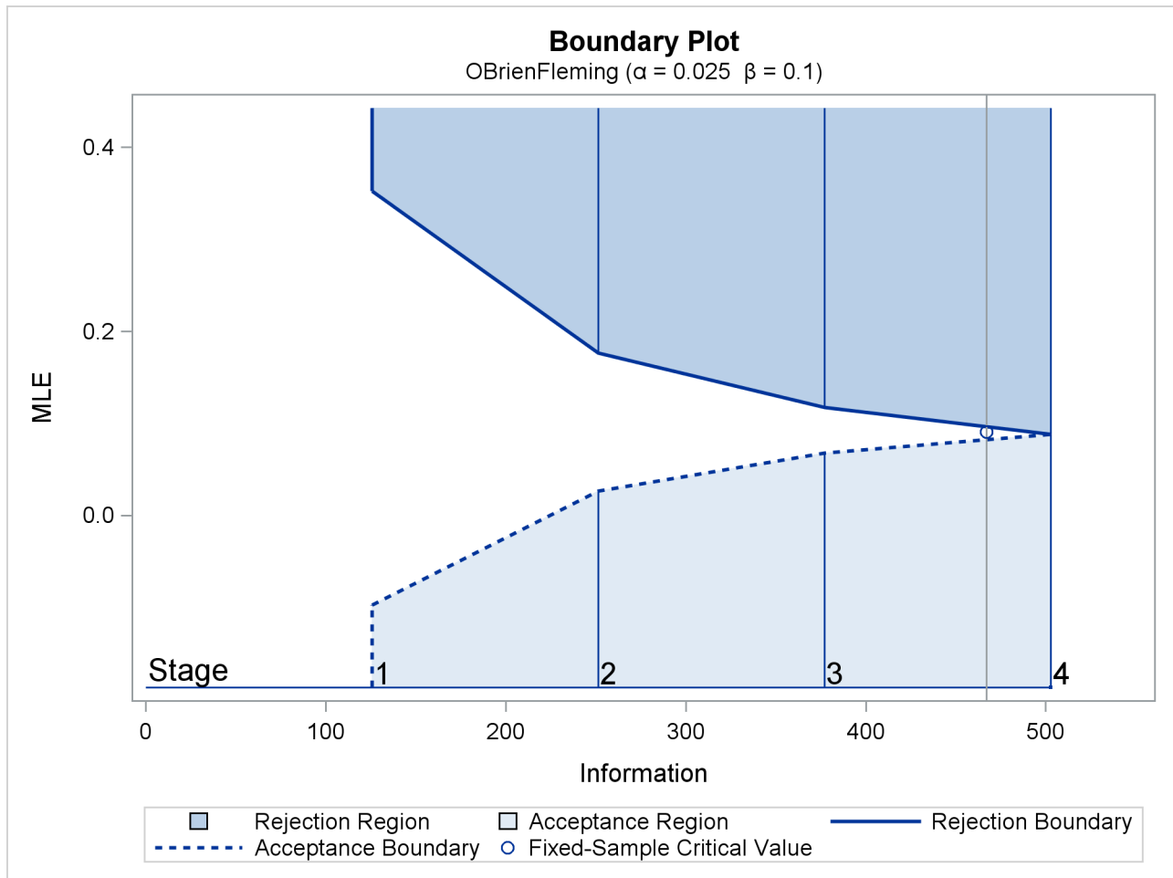
Output 90.1.3 O'Brien-Fleming Boundary Plot
