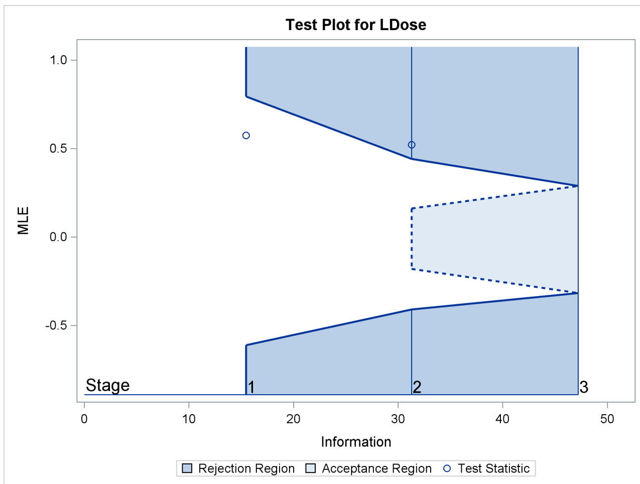
Output 90.8.14 Sequential Test Plot
