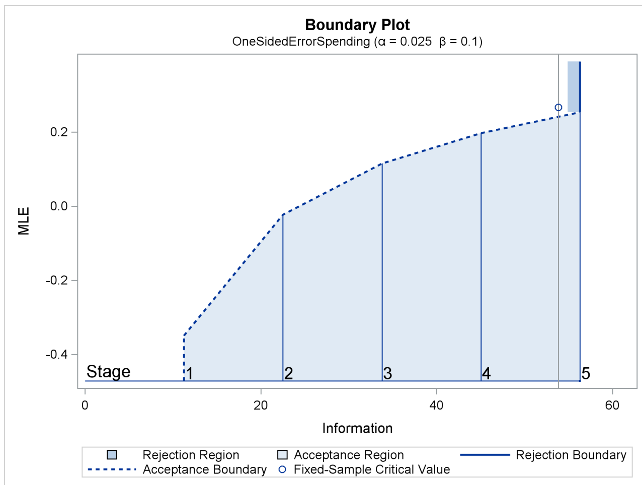
Output 90.5.3 Boundary Plot
