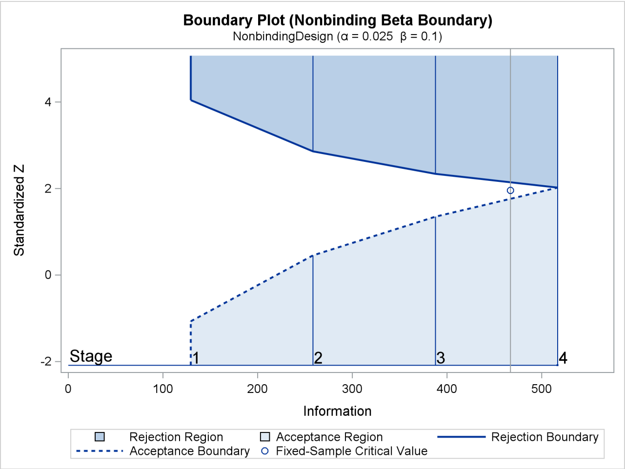
Output 90.9.3 O'Brien-Fleming Boundary Plot
