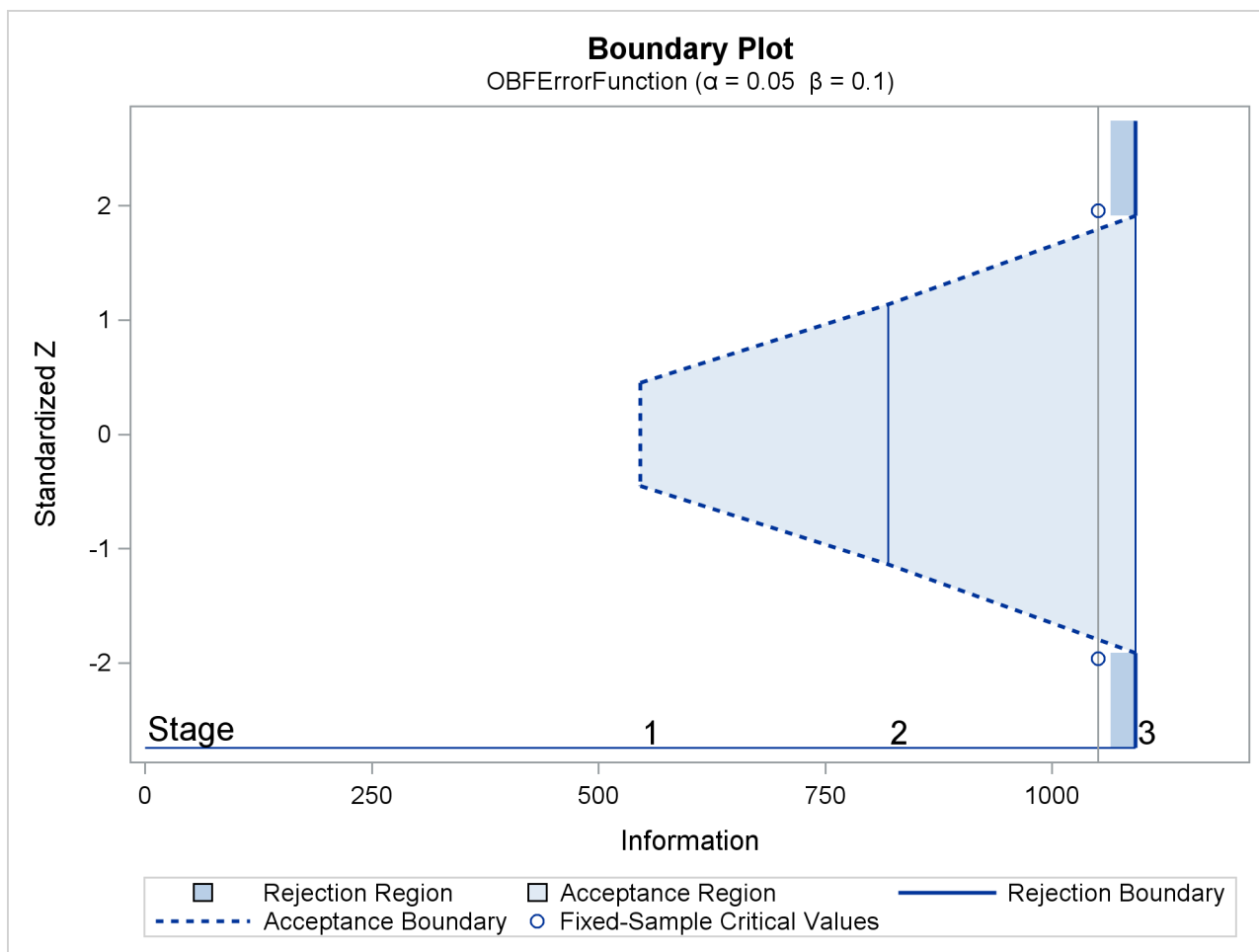
Output 90.3.3 Boundary Plot
