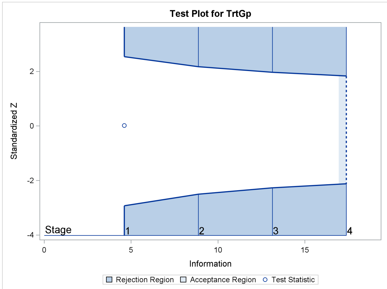
Output 90.7.12 Sequential Test Plot
