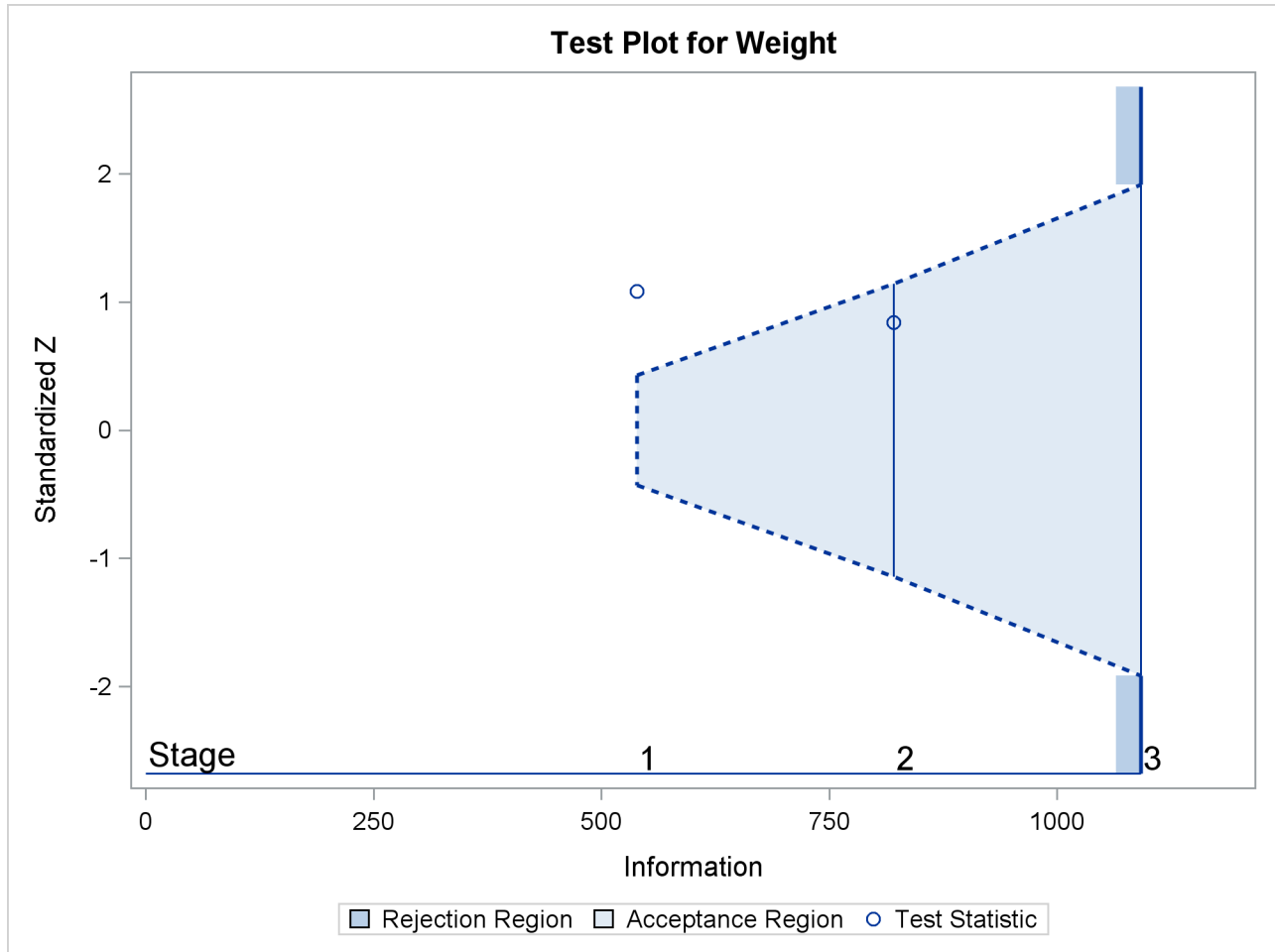
Output 90.3.18 Sequential Test Plot
