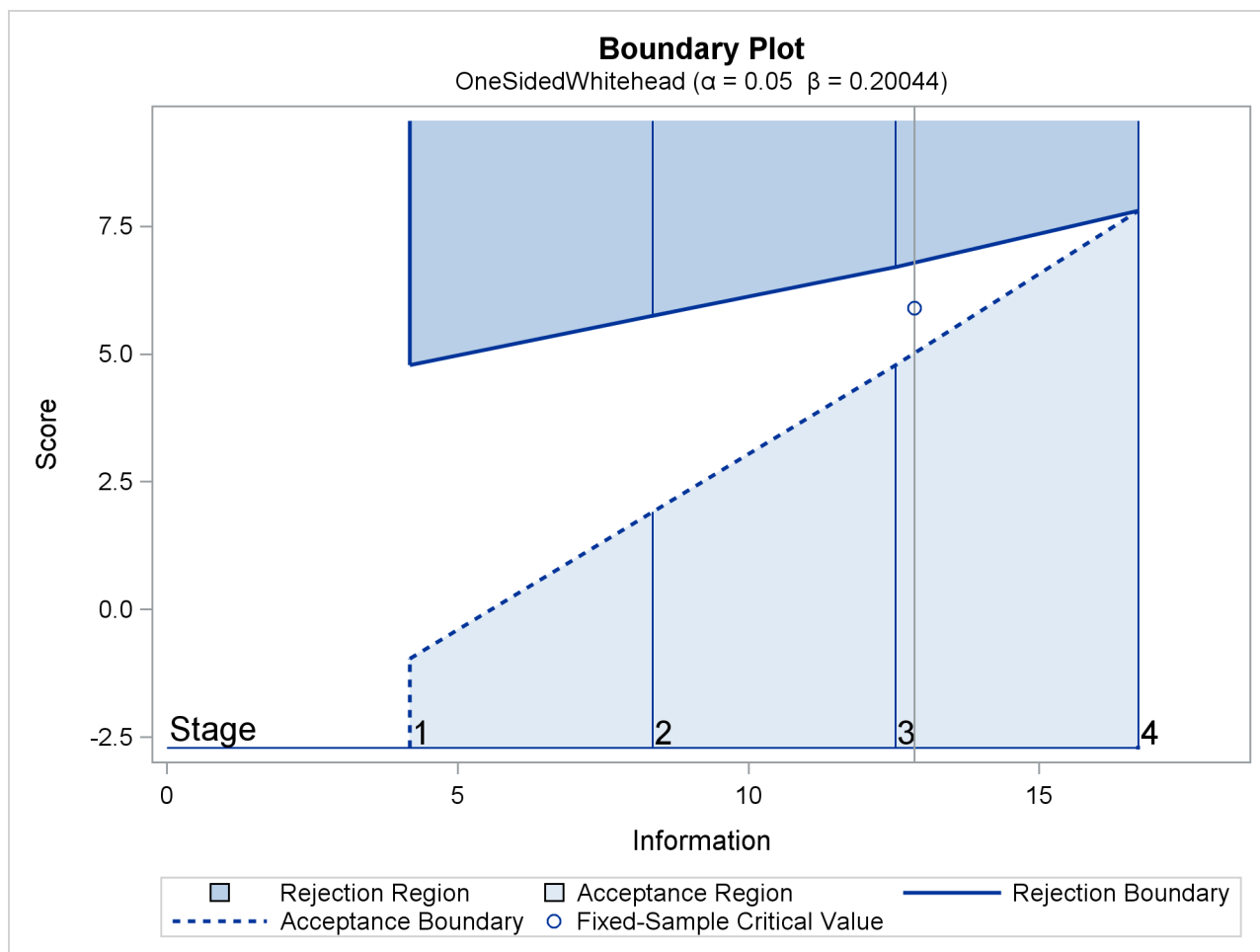
Output 90.6.3 Boundary Plot
