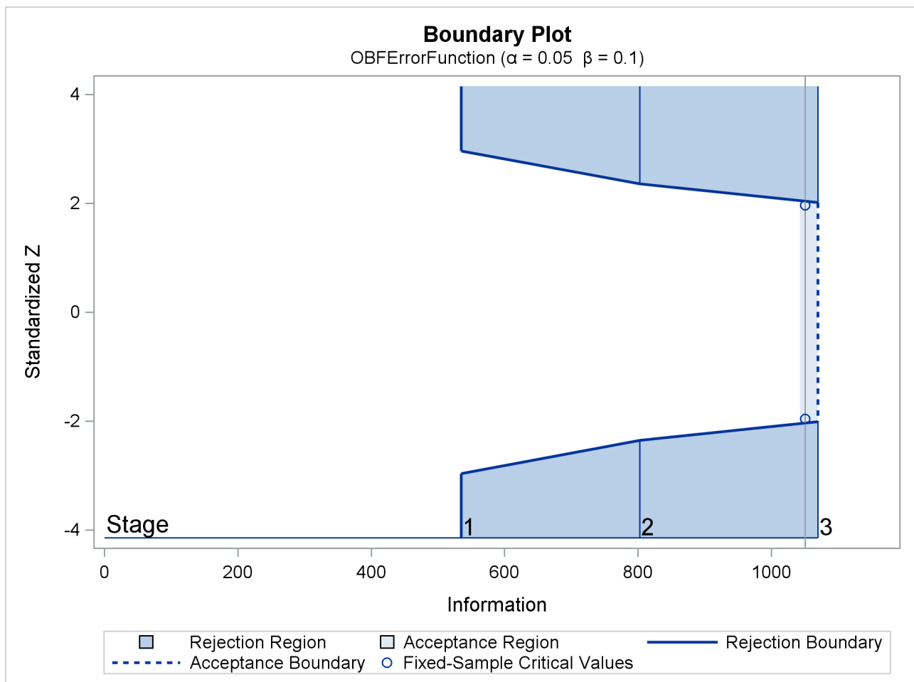
Output 90.2.3 Boundary Plot
