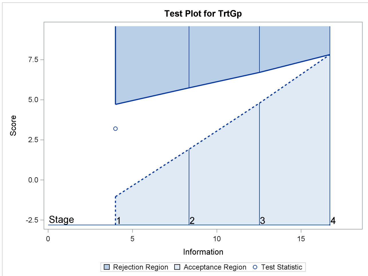
Output 90.6.12 Sequential Test Plot
