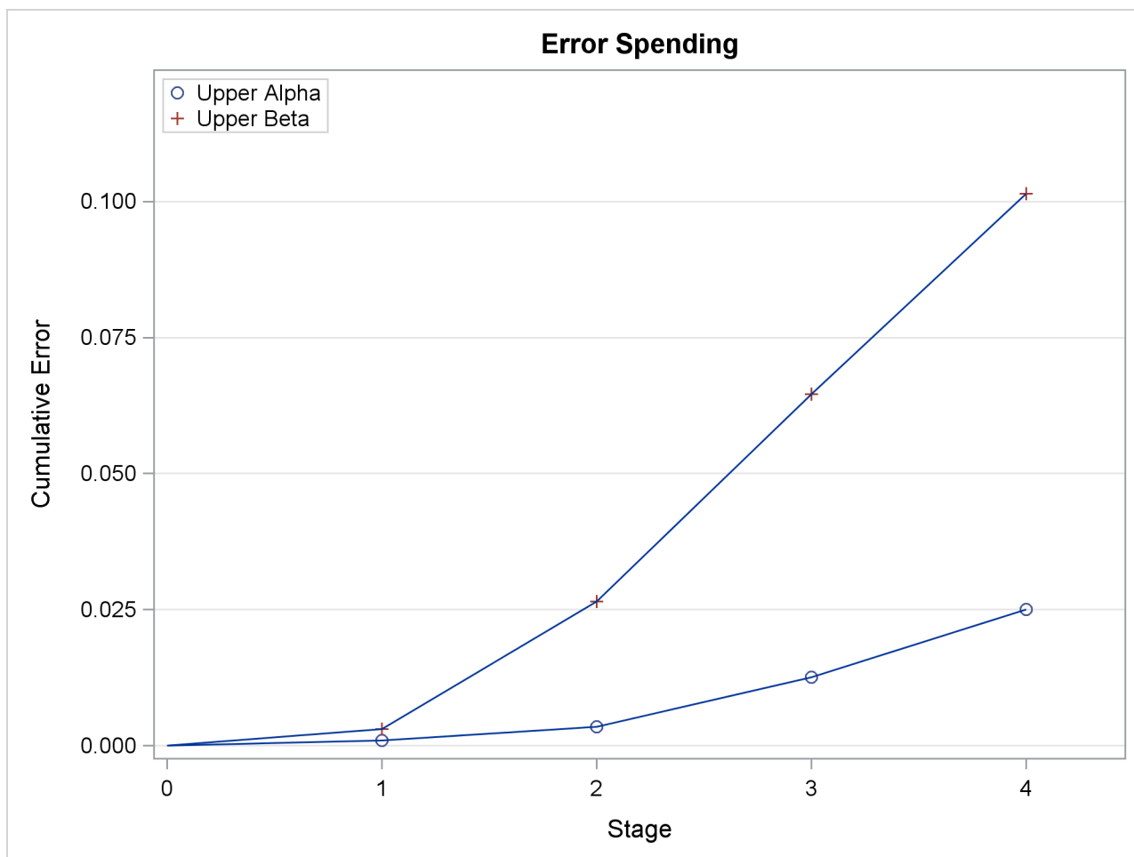
Output 90.1.11 Error Spending Plot
