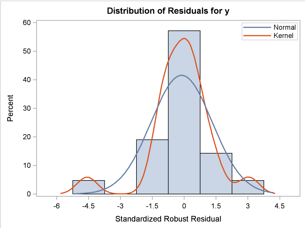
Figure 86.6 Histogram
