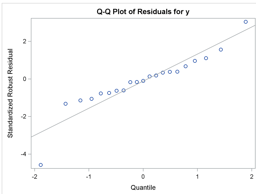
Figure 86.7 Q-Q Plot
