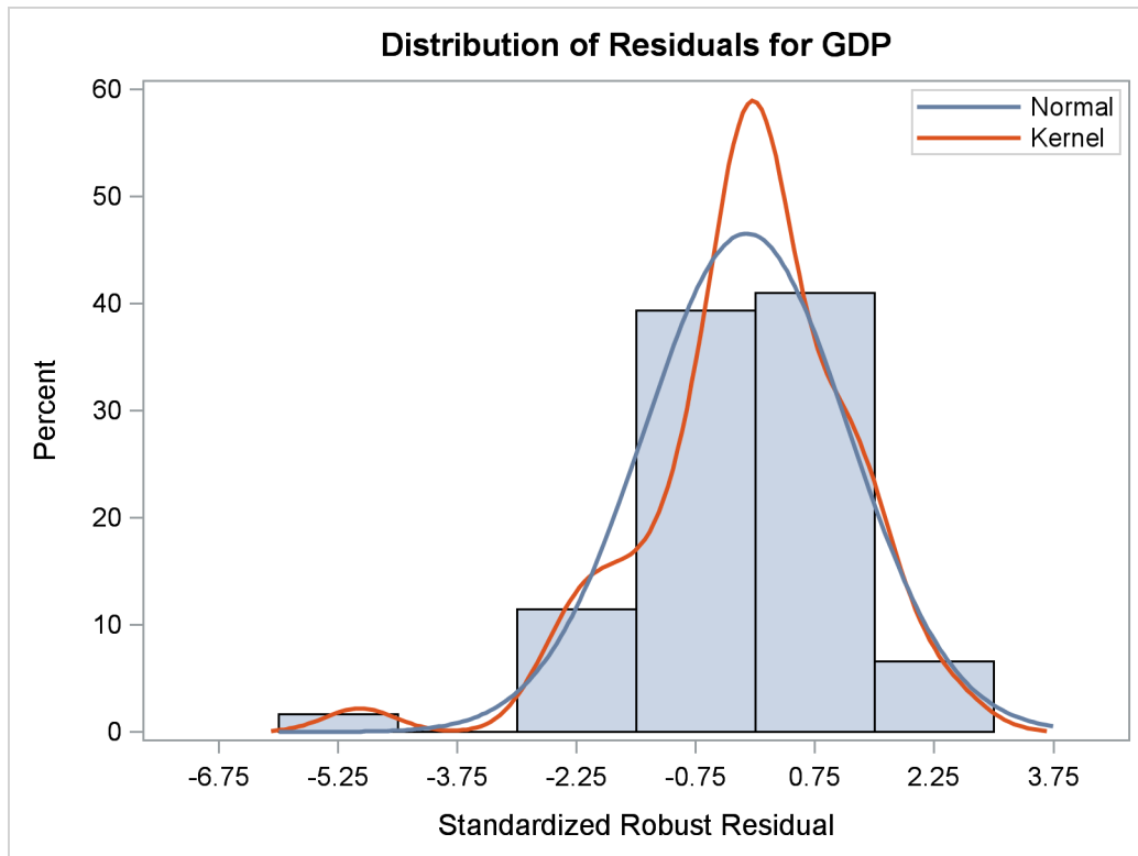
Output 86.3.8 Histogram
