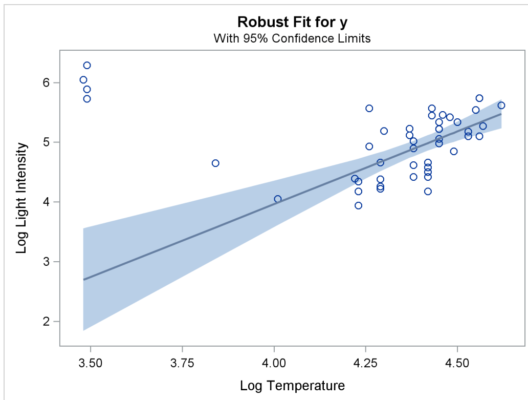
Figure 86.22 Robust Fit
