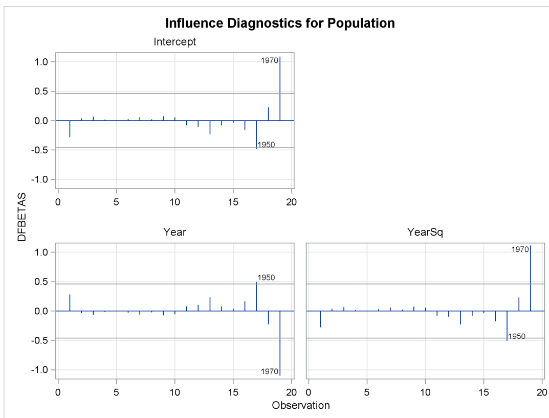
Figure 85.40 continued
