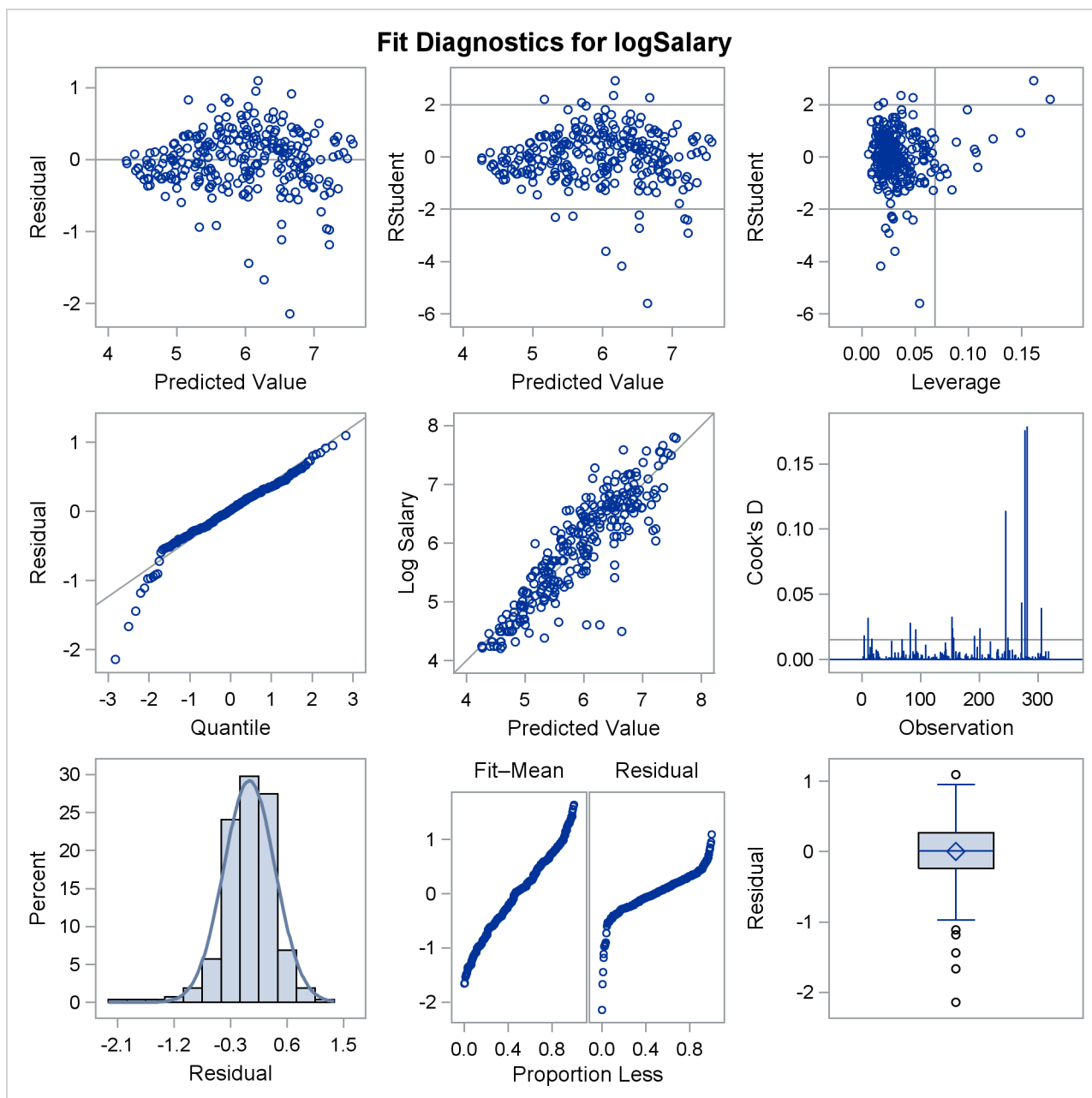
Output 85.1.11 Fit Diagnostics
