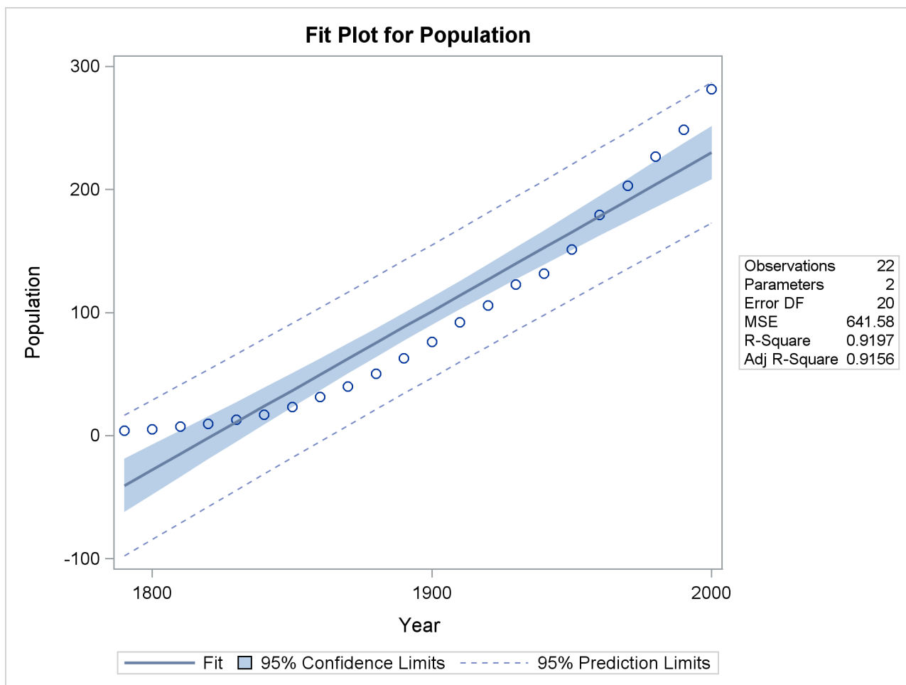
Figure 85.11 Fit Plot
