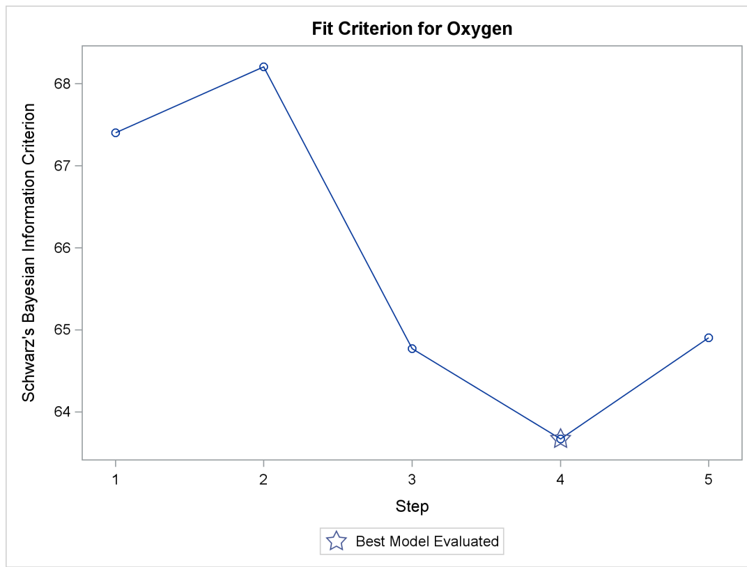
Output 85.2.6 SBC Criterion
