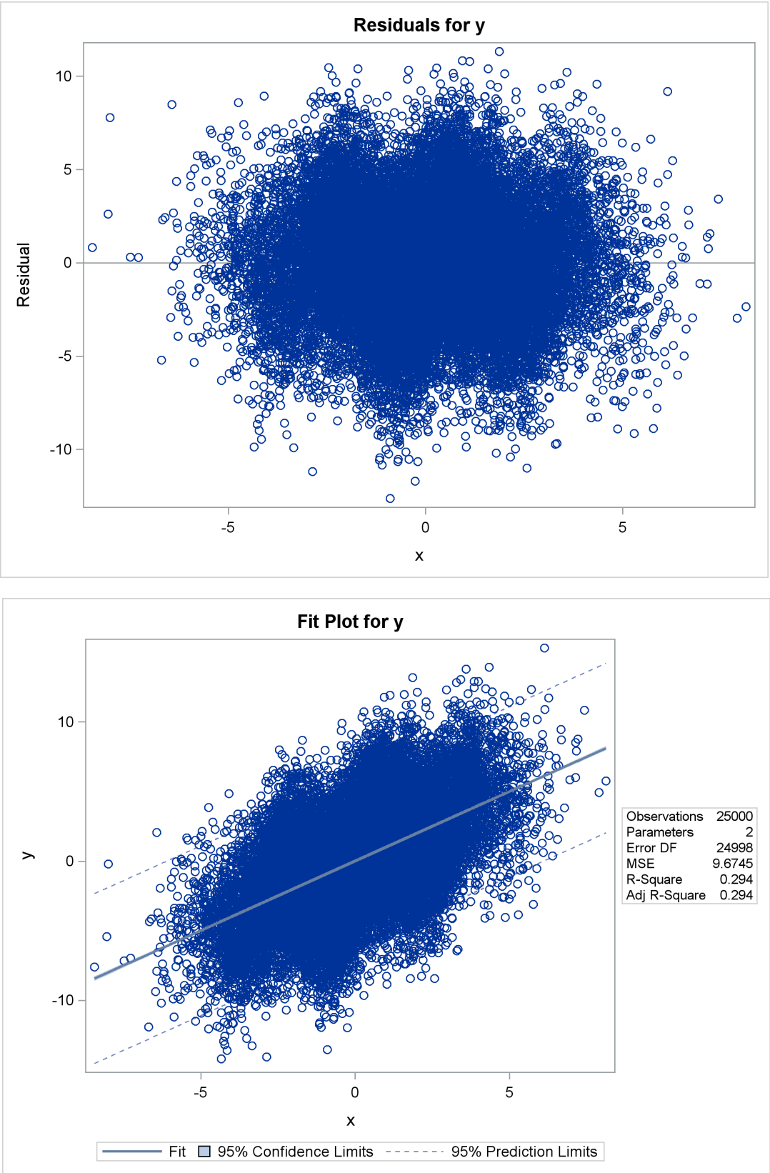
Figure 85.54 Scatter Plot
