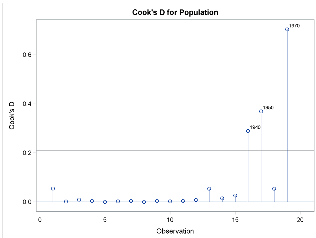
Figure 85.40 Influence Diagnostics
