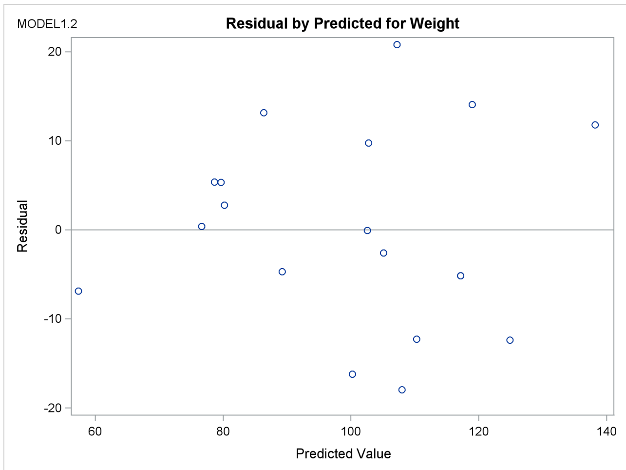
Figure 85.28 Interactive Analysis: Scatter Plot
