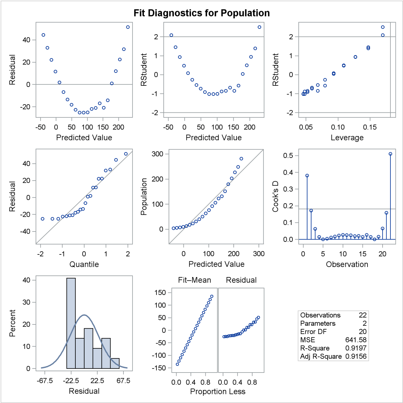
Figure 85.9 Diagnostics Panel
