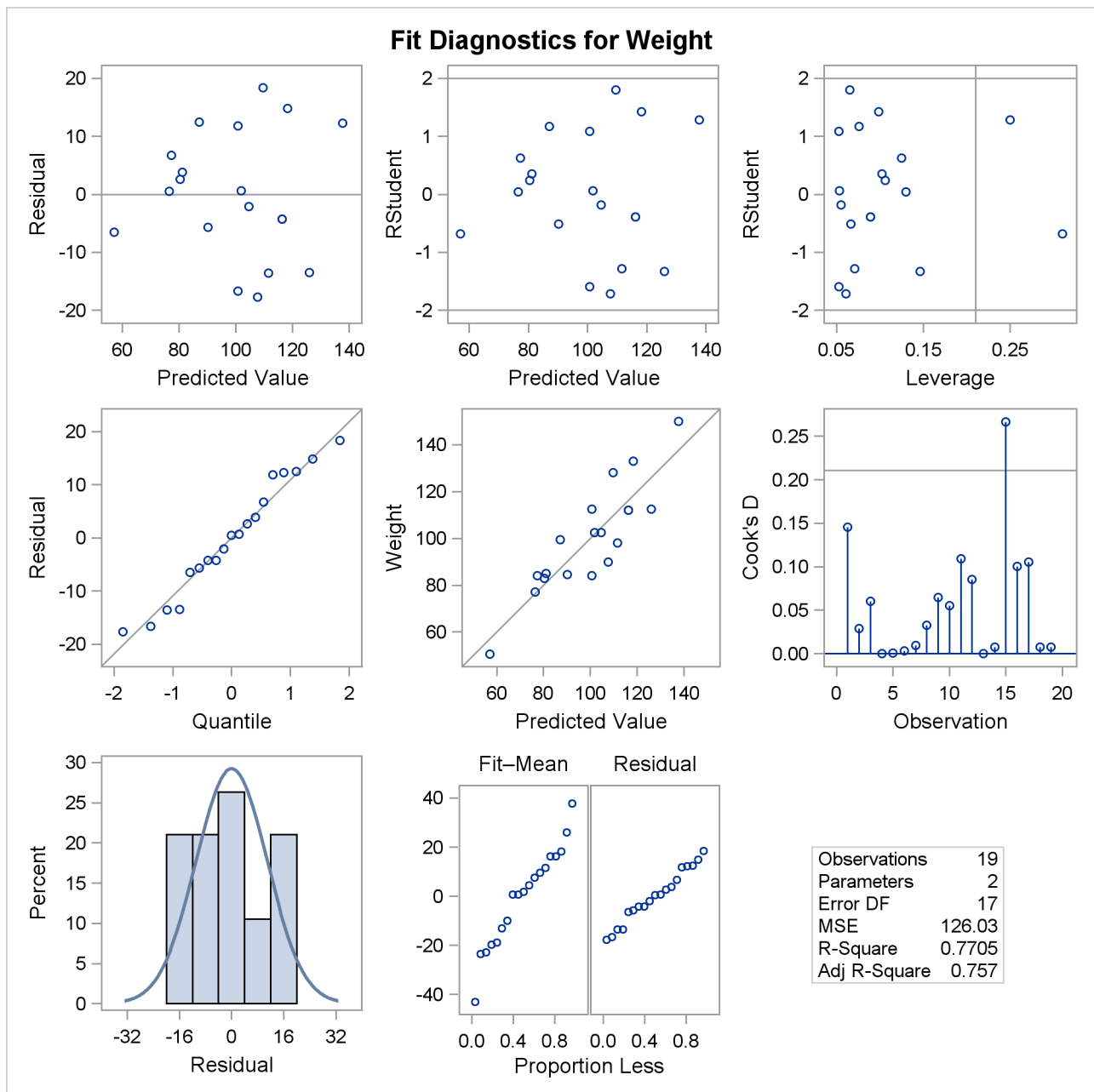
Figure 85.4 Fit Diagnostics
