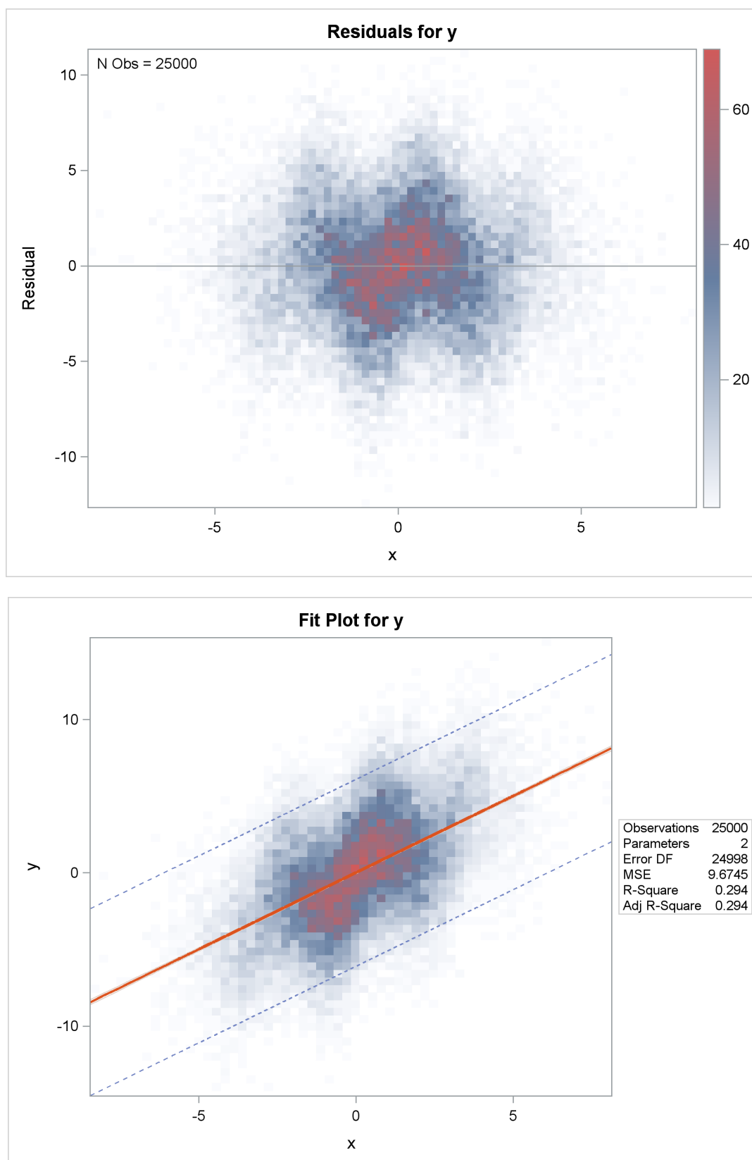
Figure 85.55 Heat Map
