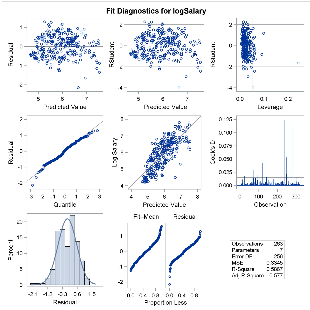
Output 85.1.3 Fit Diagnostics
