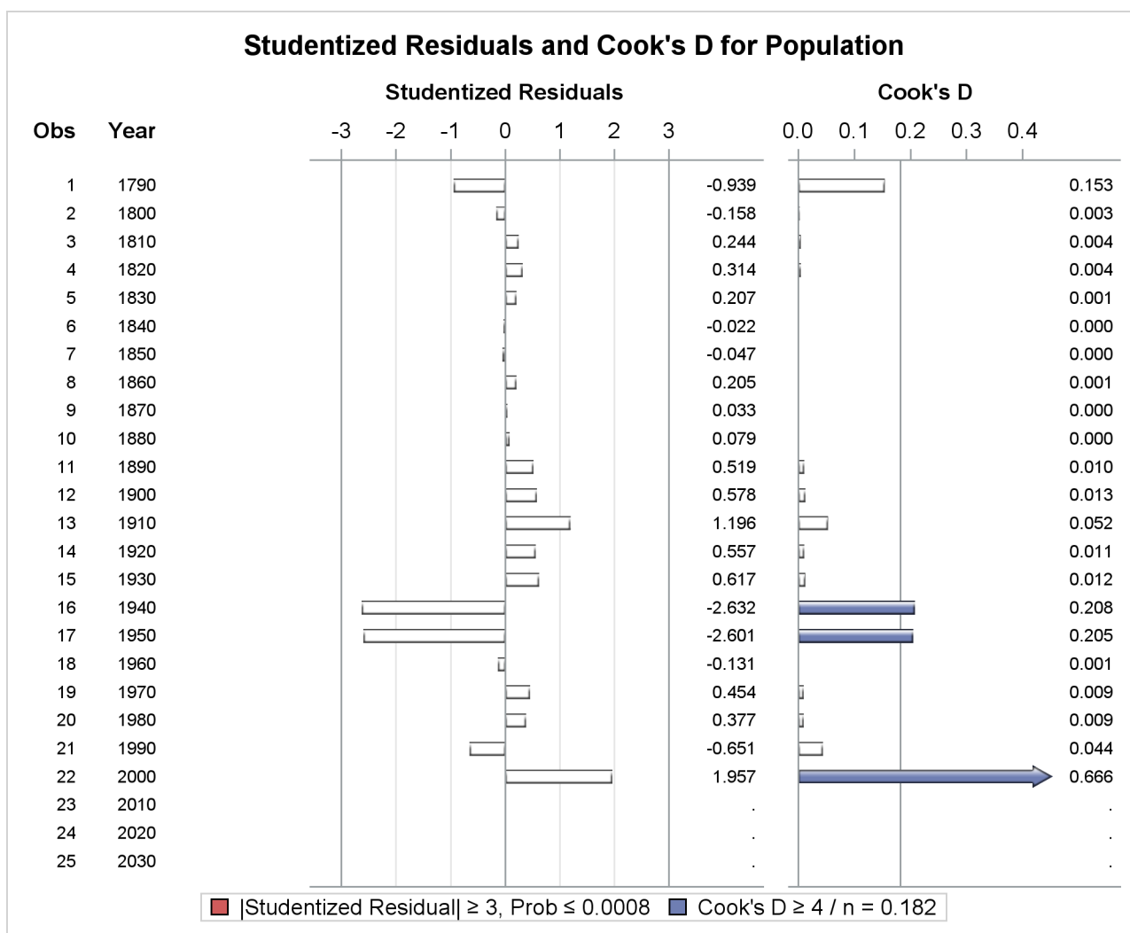
Figure 85.35 Studentized Residuals and Cook's D
