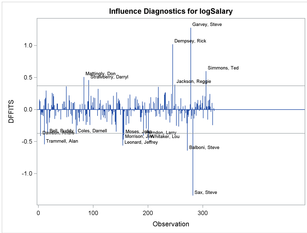
Output 85.1.15 DFFITS
