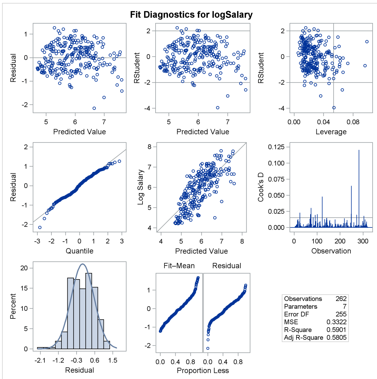
Output 85.1.6 Fit Diagnostics
