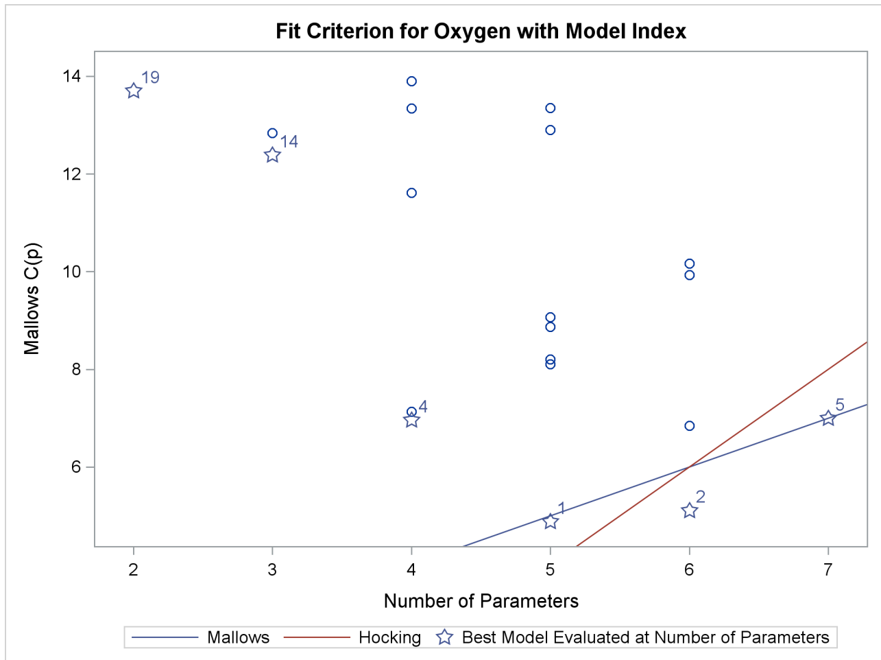
Output 85.2.11 C_p Criterion
