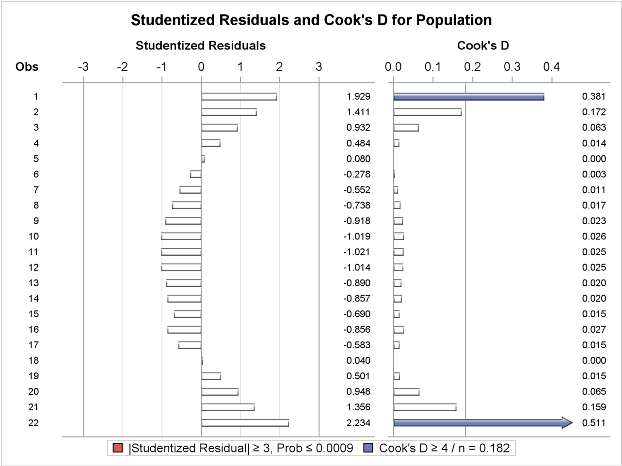
Figure 85.7 Studentized Residuals
