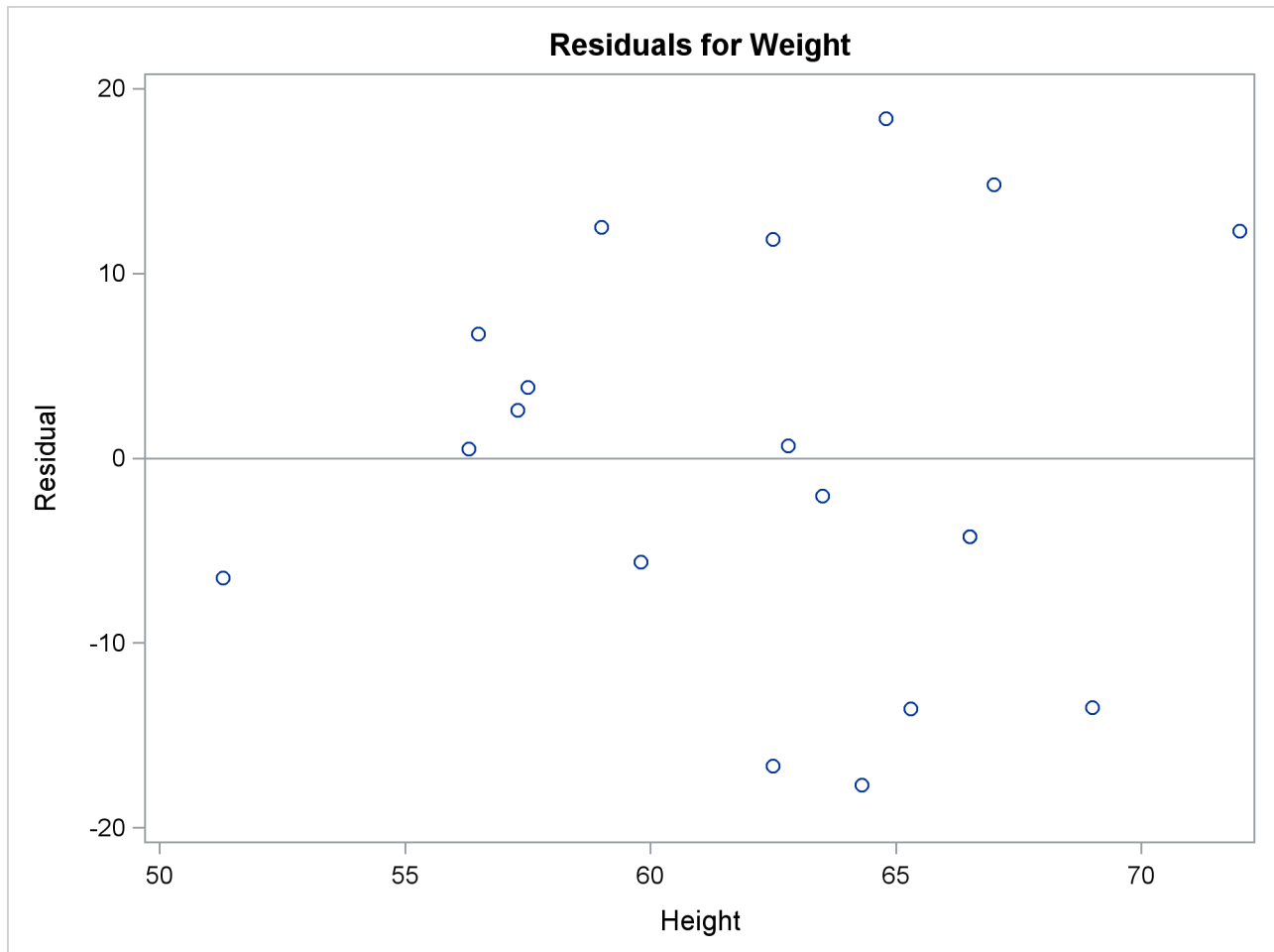
Figure 85.3 Residuals vs. Regressor
