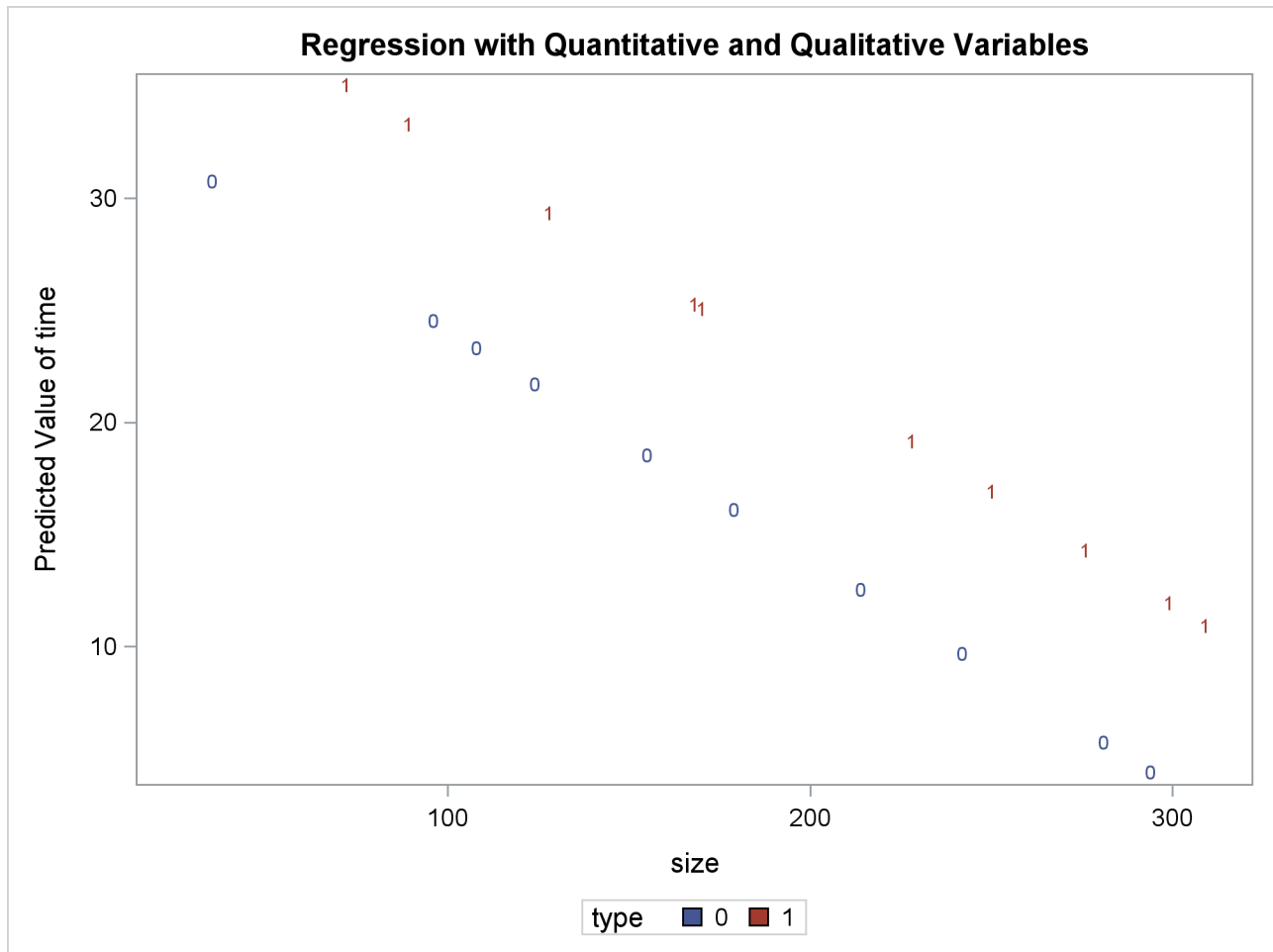
Output 85.4.4 Plot of Predicted vs. Size
