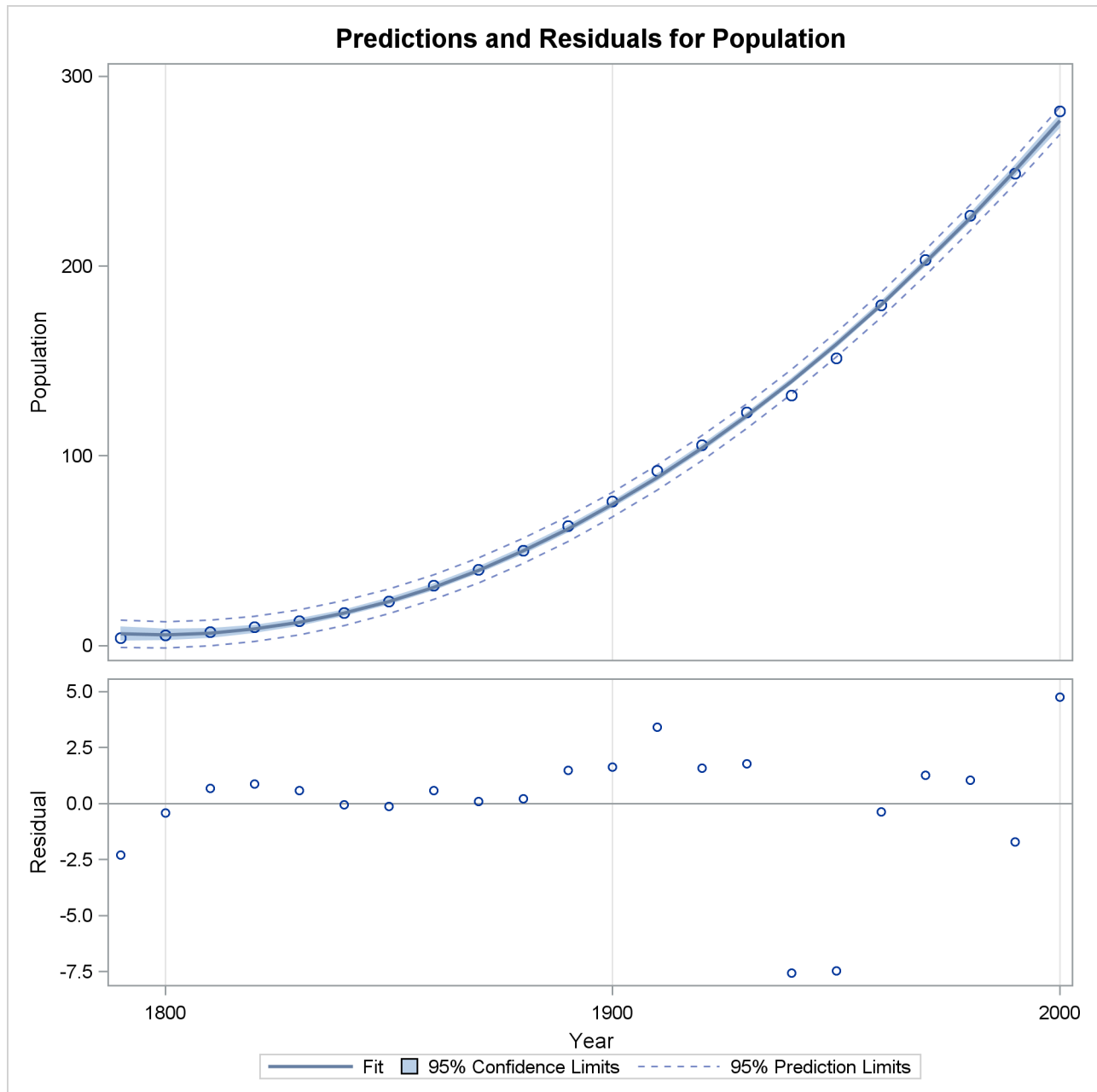
Figure 85.14 Predictions and Residuals by Year
