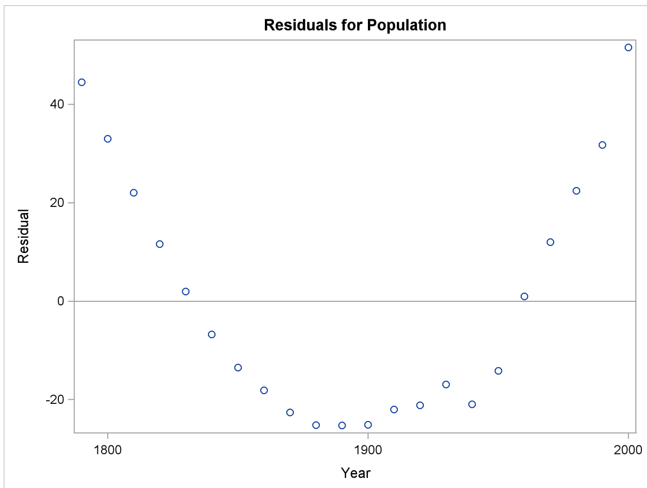
Figure 85.10 Residual Plot
