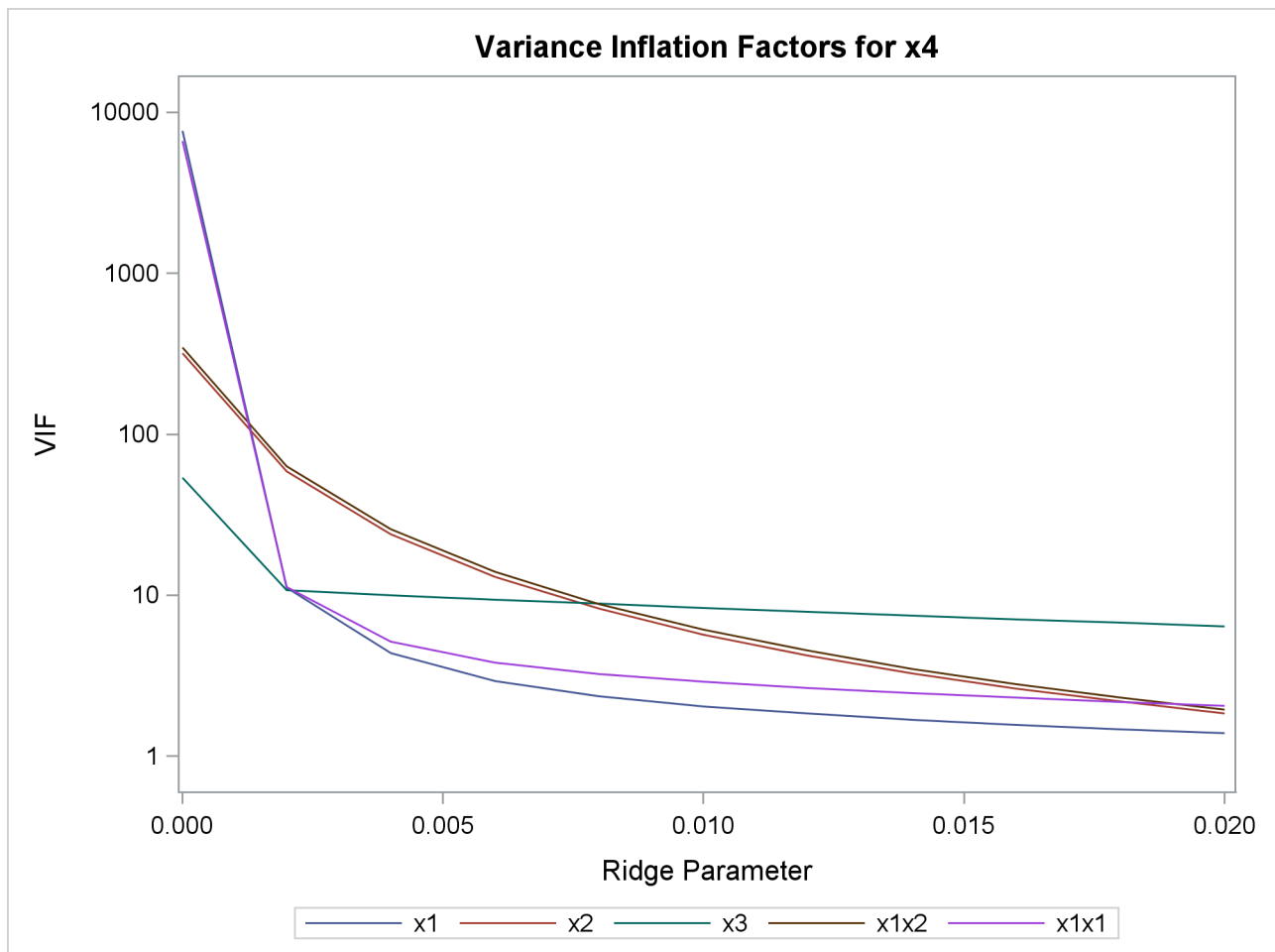
Output 85.5.3 VIF Traces
