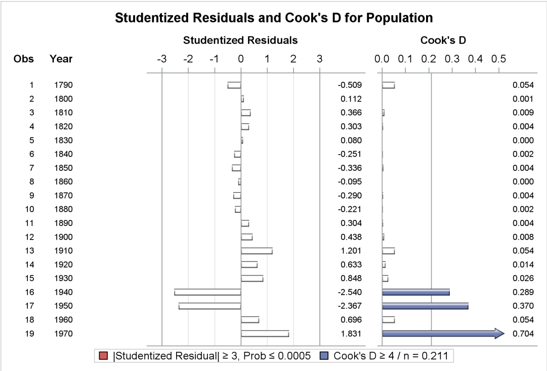
Figure 85.41 Studentized Residuals and Cook's D Chart
