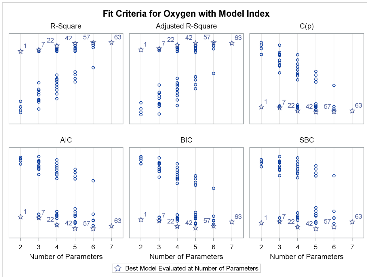
Output 85.2.8 Fit Criteria
