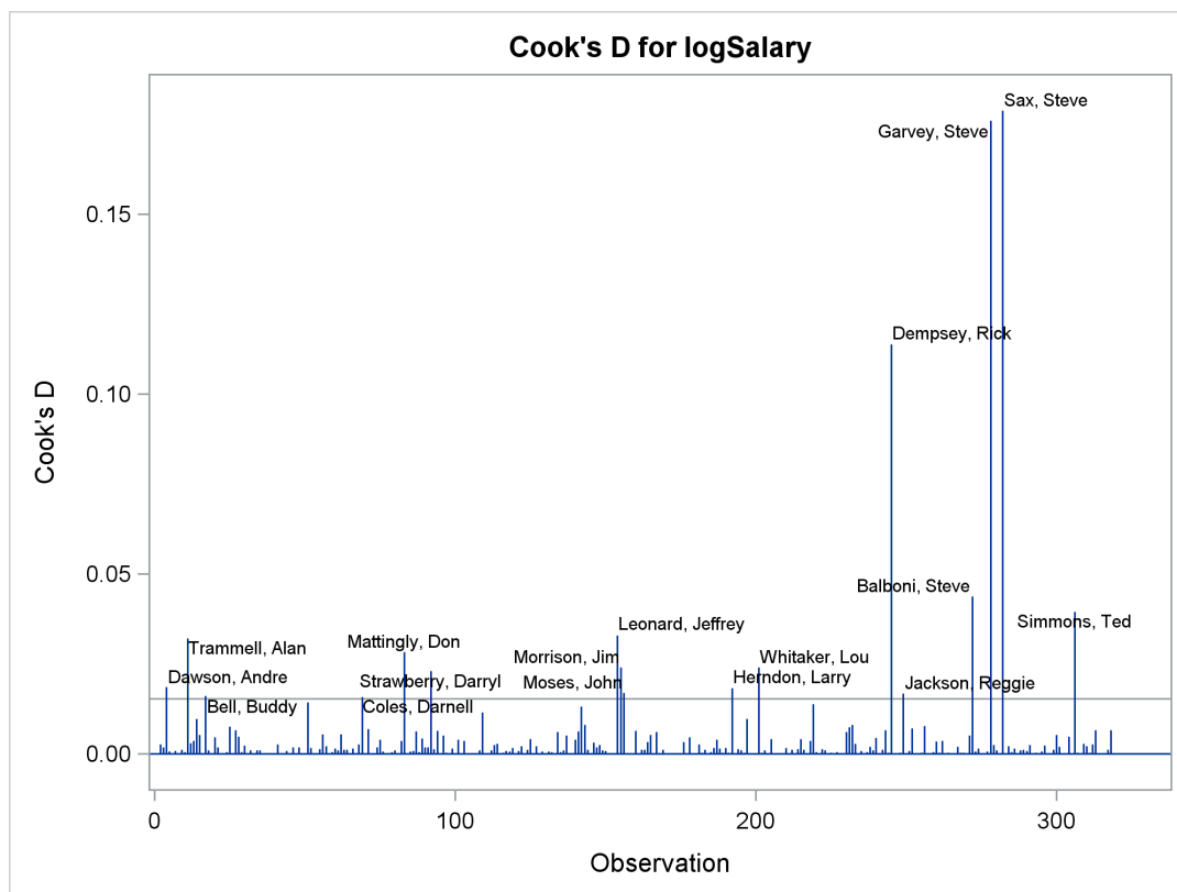
Output 85.1.14 Cook's D
