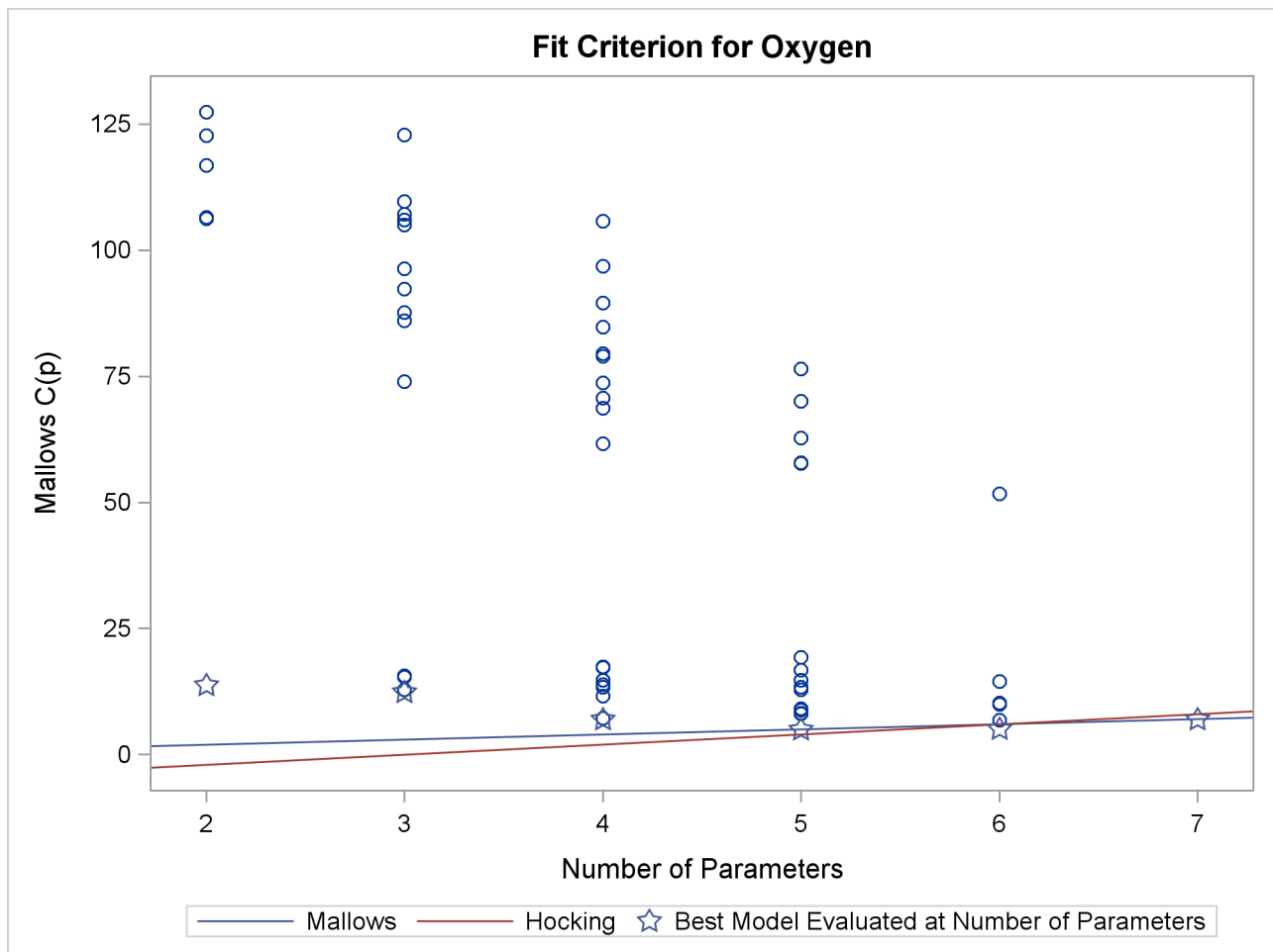
Output 85.2.9 C_p Criterion
