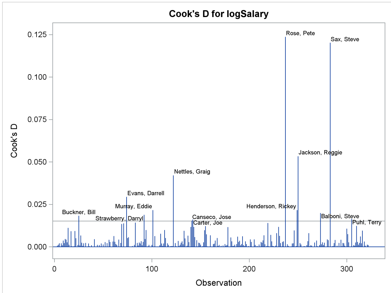
Output 85.1.5 Cook's D
