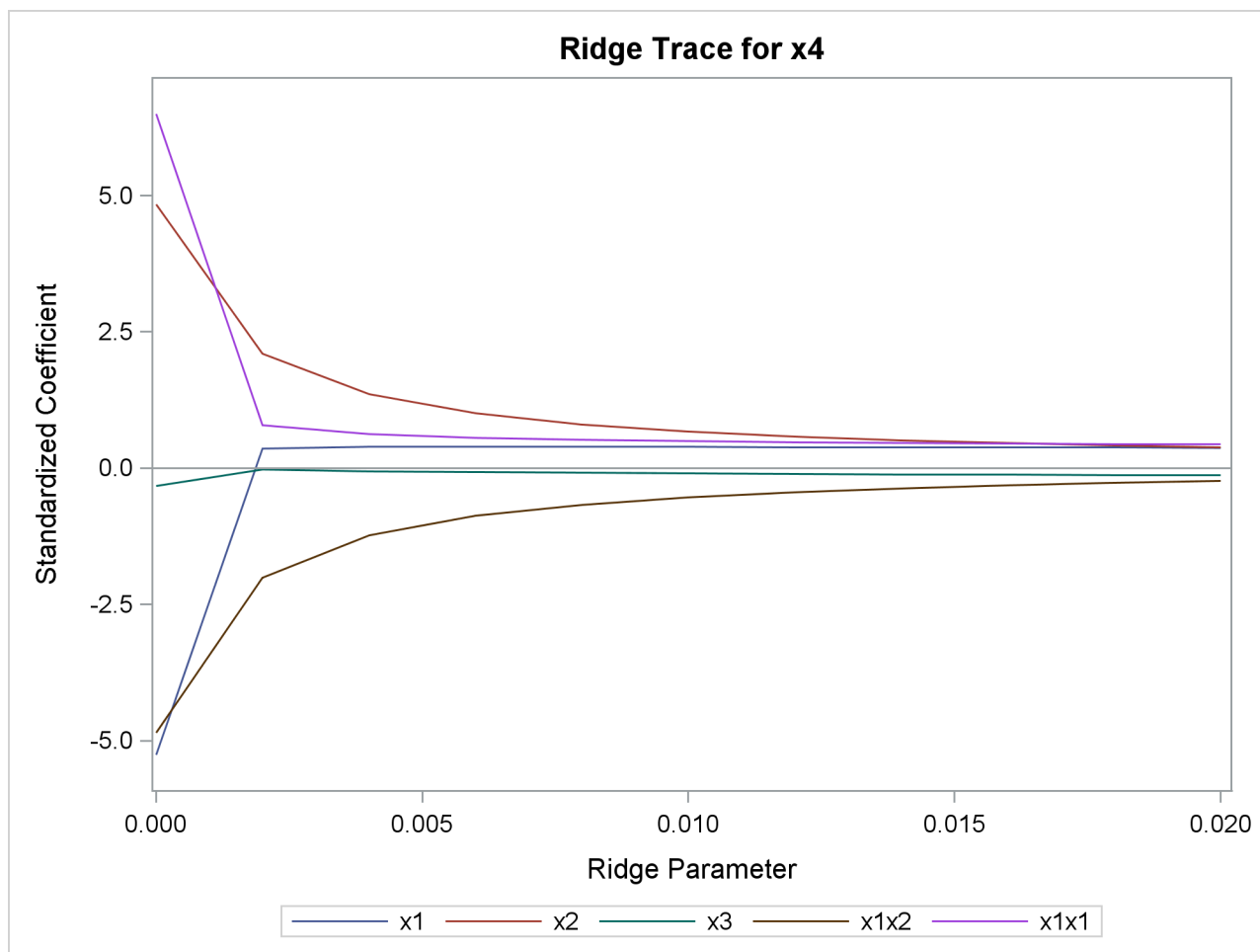
Output 85.5.4 Ridge Traces
