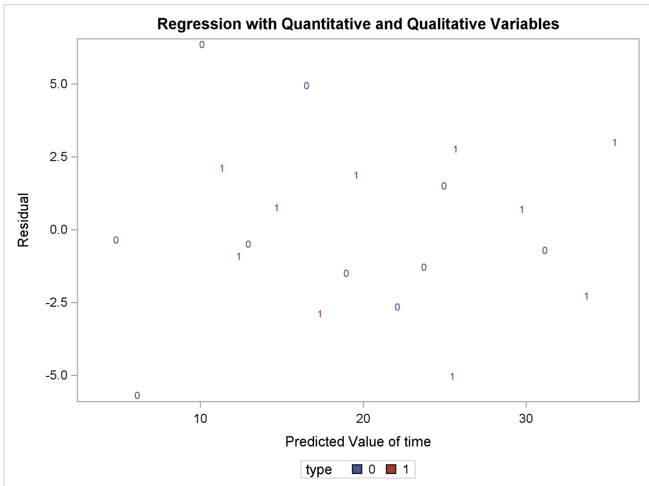
Output 85.4.3 Plot of Residual vs. Predicted Values
