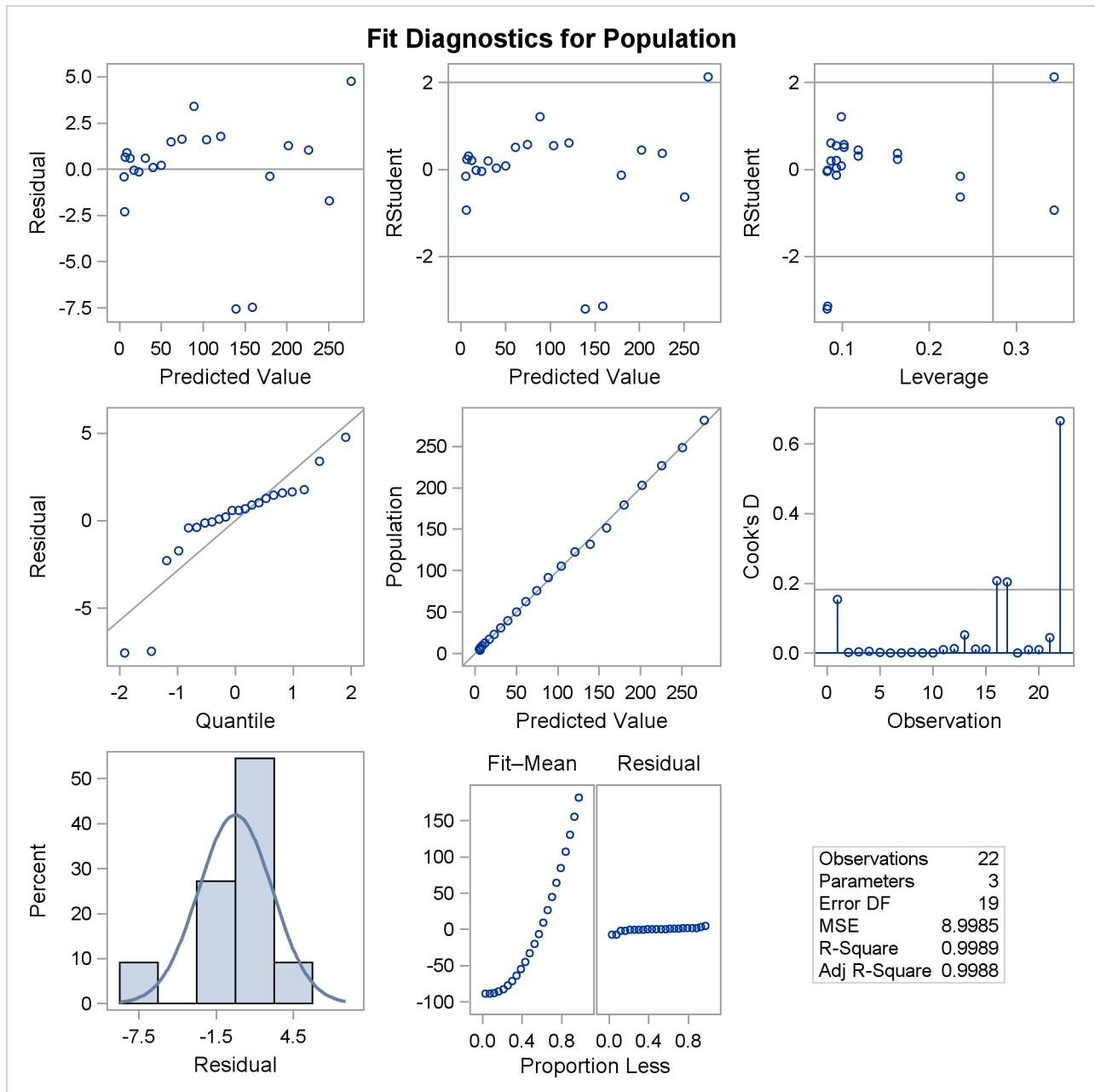
Figure 85.13 Diagnostics Panel
