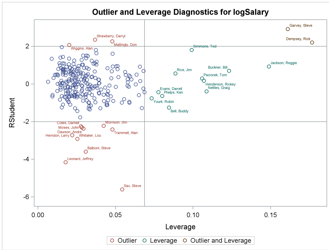
Output 85.1.12 Outlier and Leverage Diagnostics
