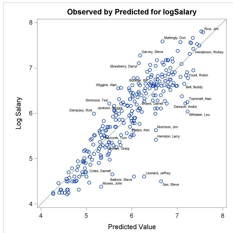
Output 85.1.13 Observed by Predicted Values
