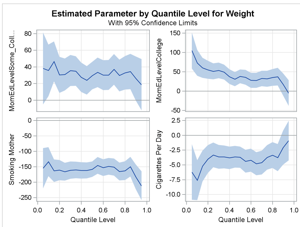
Output 83.3.5 Quantile Processes with 95% Confidence Bands
