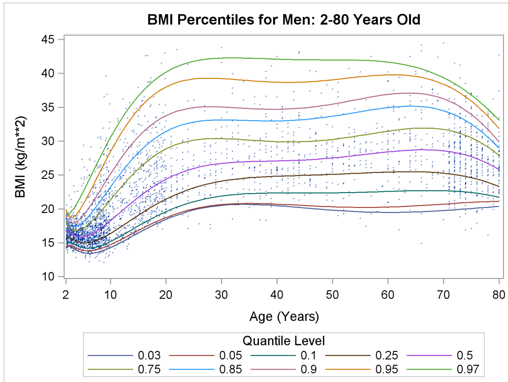
Figure 83.2 Percentiles for Body Mass Index
