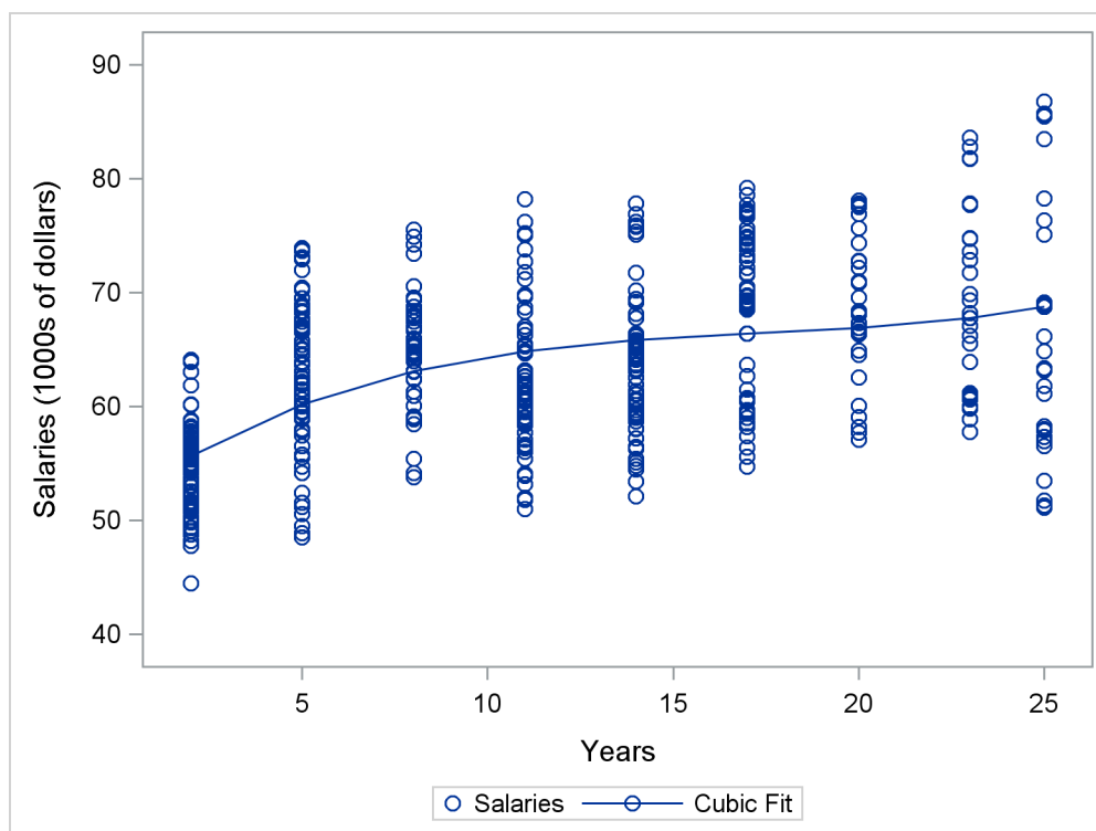
Output 83.5.1 Salary and Years as Professor: Cubic Fit
