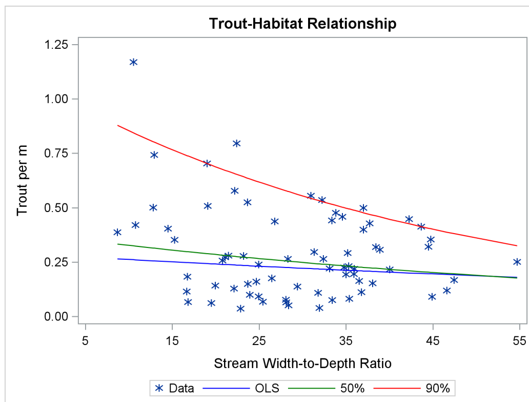
Figure 83.1 Trout Density in Streams
