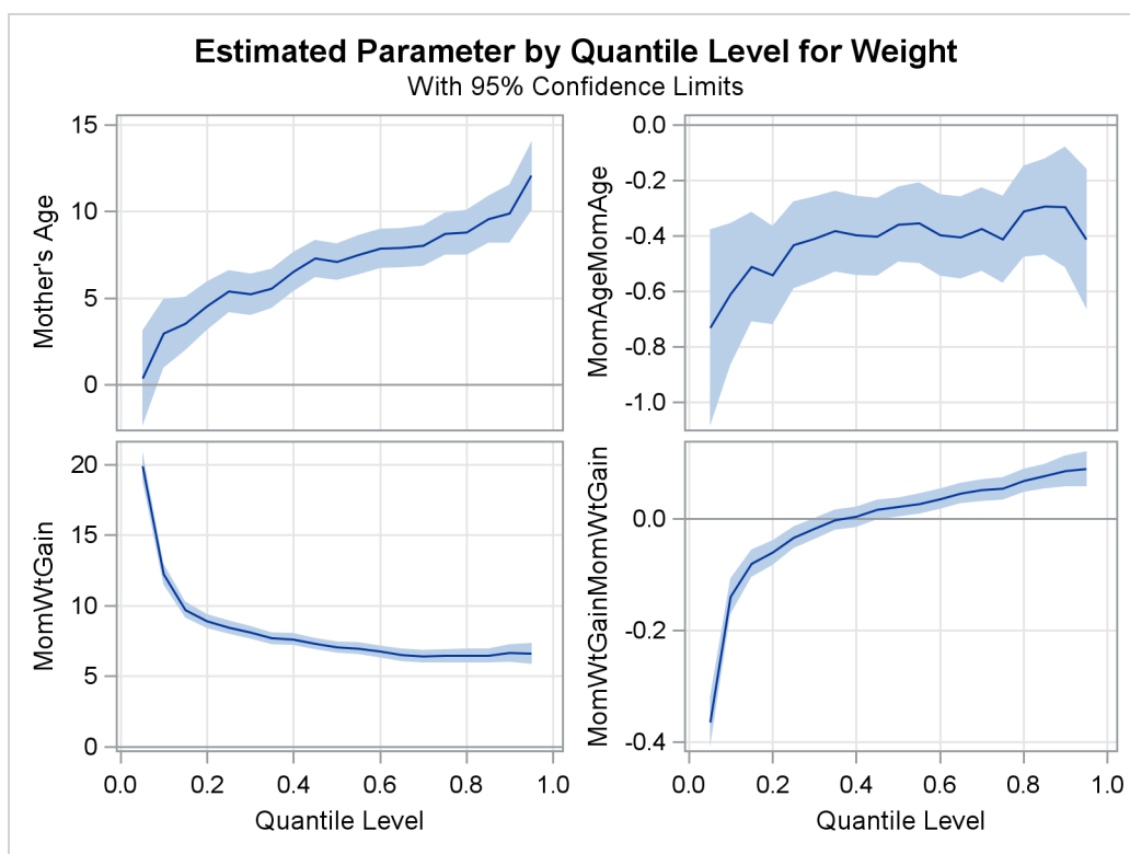
Output 83.3.6 Quantile Processes with 95% Confidence Bands
