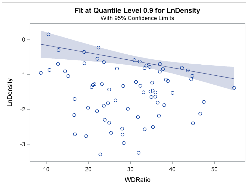
Figure 83.14 Fit Plot with Confidence Limits
