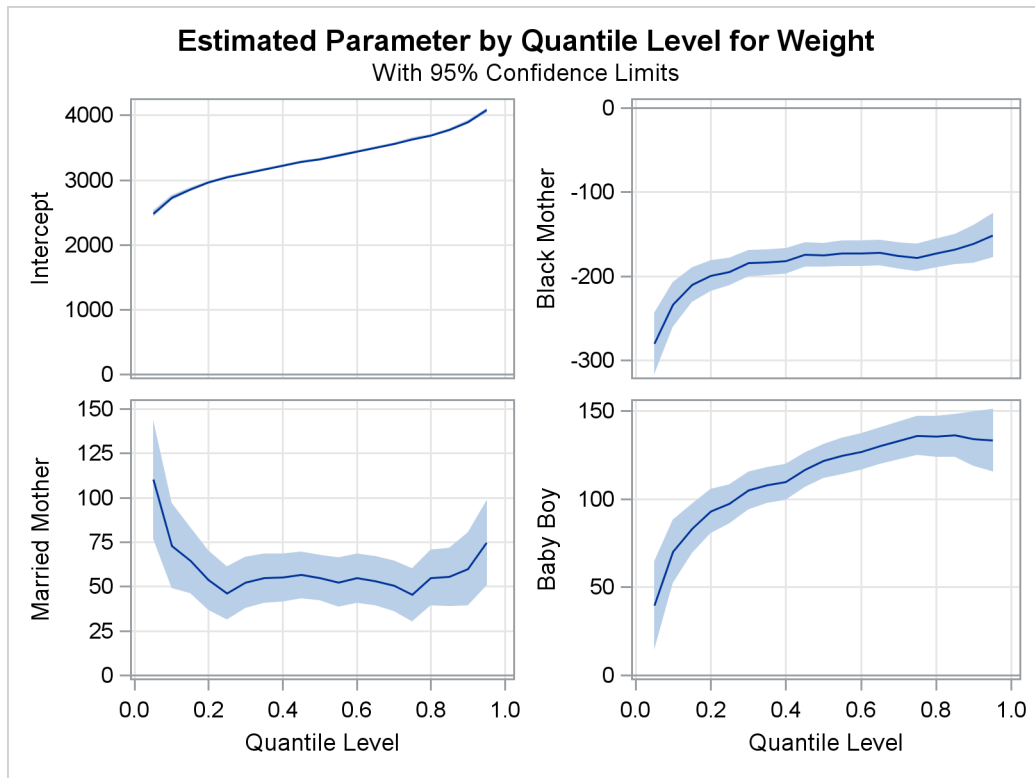
Output 83.3.3 Quantile Processes with 95% Confidence Bands
