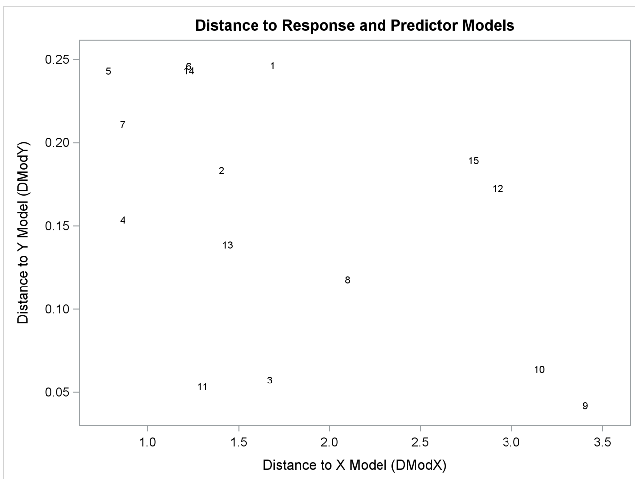
Output 76.2.2 Predictor versus Response Distances to the Model
