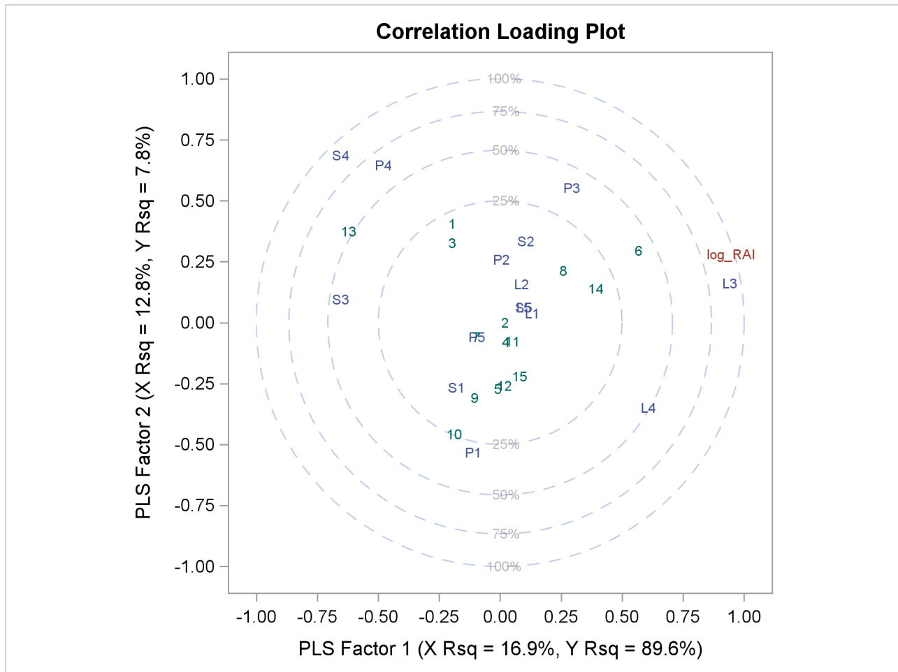
Output 76.1.3 Correlation Loading Plot
