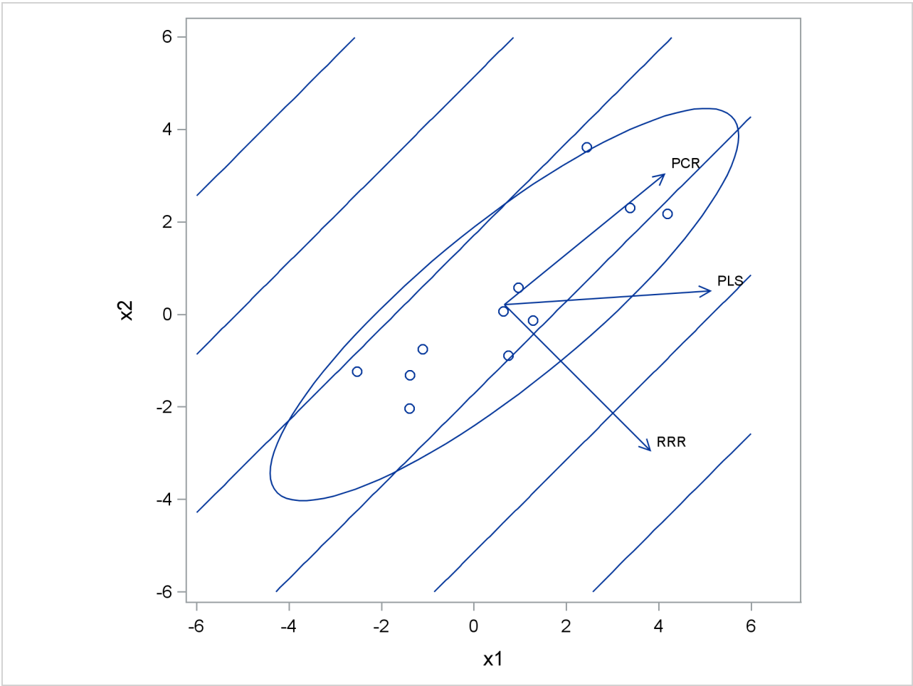
Figure 76.13 Depiction of First Factors for Three Different Regression Methods
