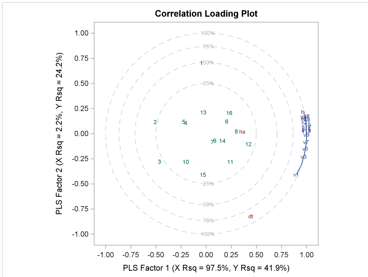
Figure 76.8 Correlation Loading Plot
