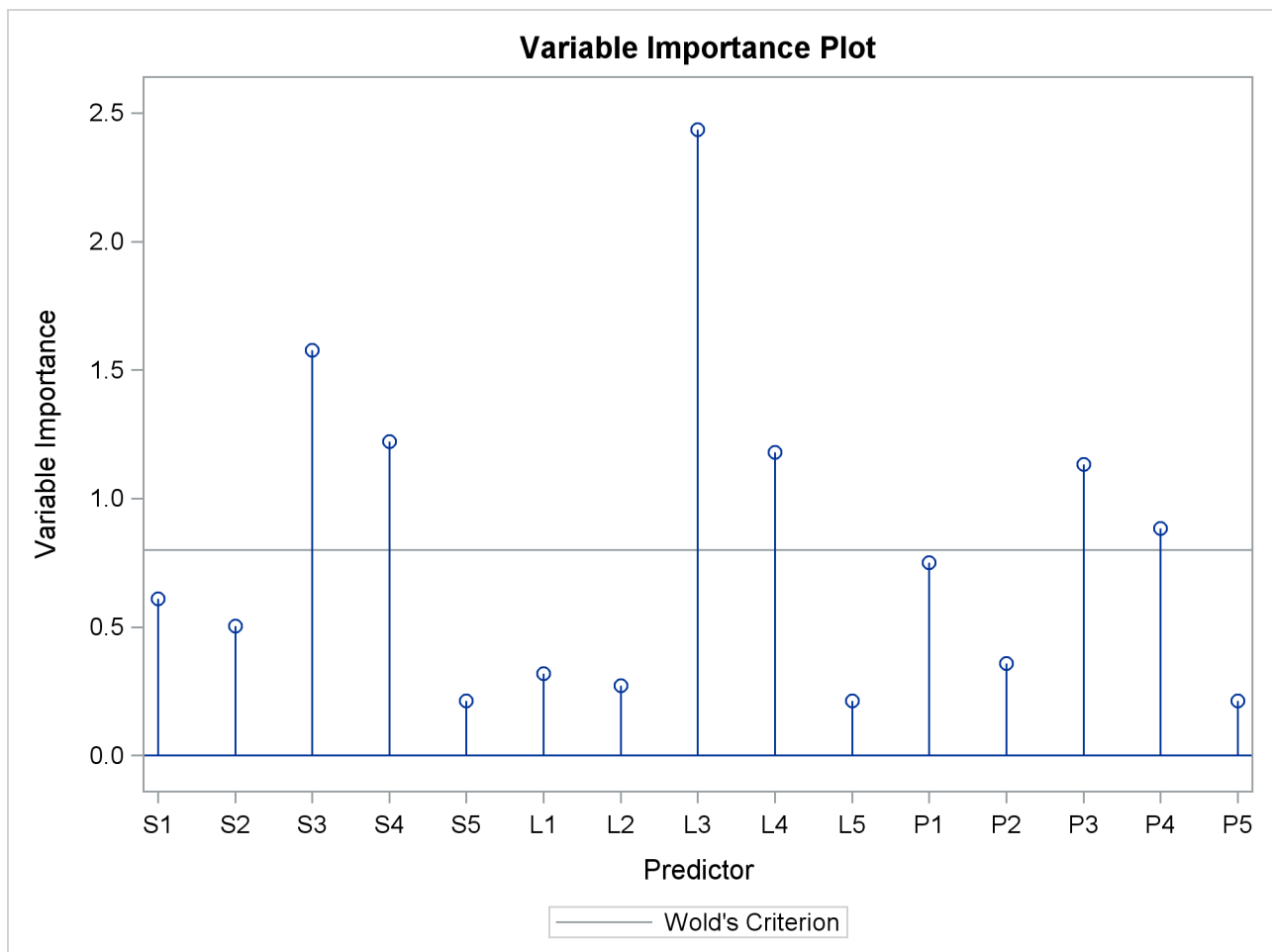
Output 76.1.5 Variable Importance Plots
