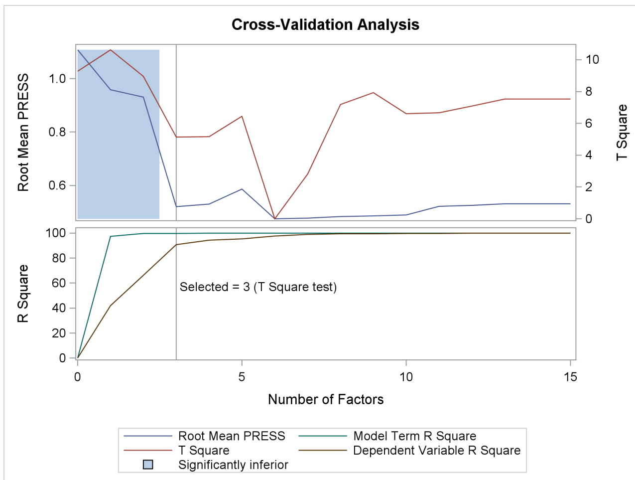
Figure 76.7 Split-Sample Cross Validation Plot
