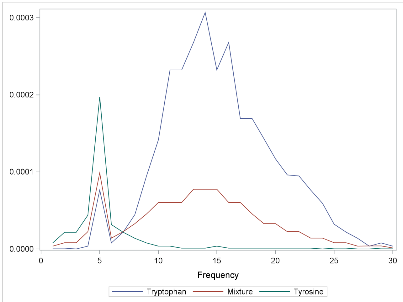
Output 76.3.1 Spectra for Three Samples of Tyrosine and Tryptophan
