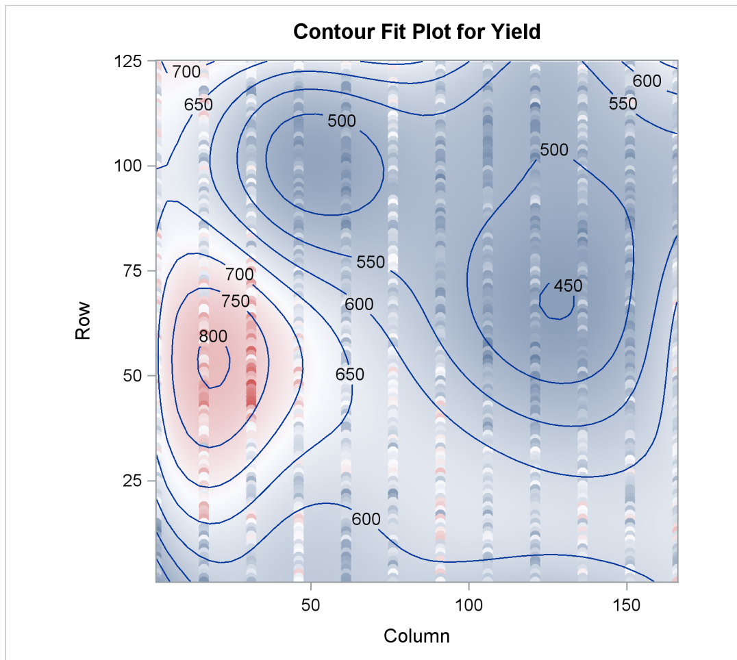
Output 76.4.4 Default Spline Basis: Smoothed Yield
