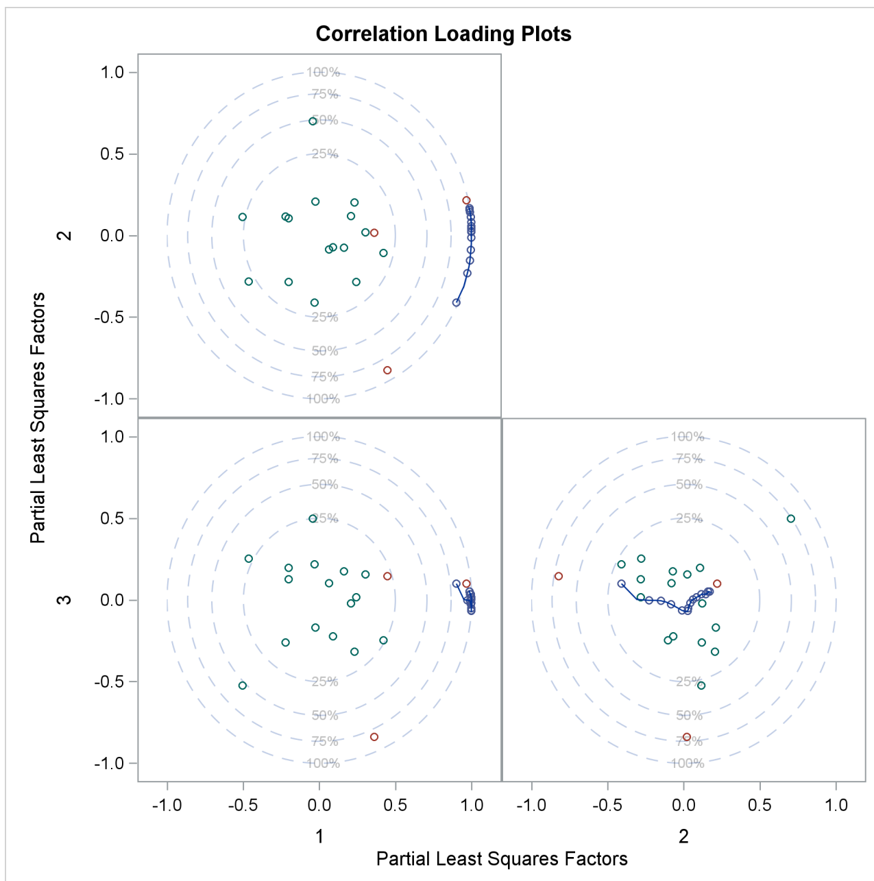
Figure 76.9 Correlation Loading Plot Matrix
