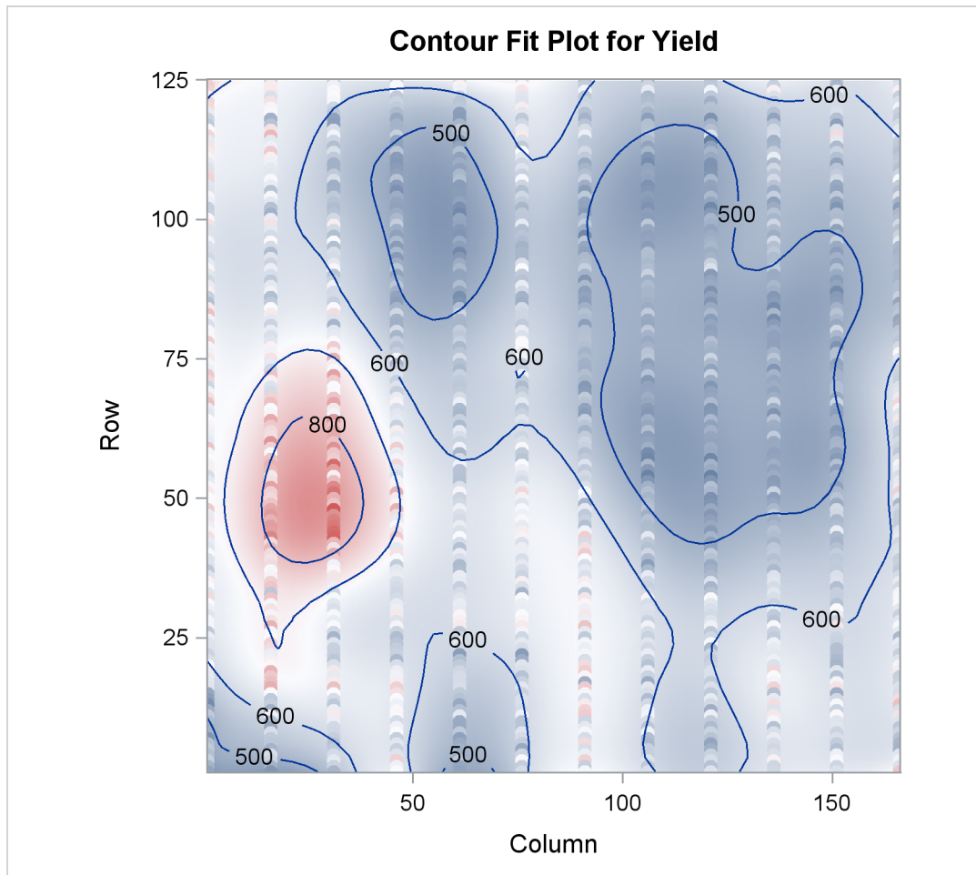
Output 76.4.8 More Granular Spline Basis: Smoothed Yield
