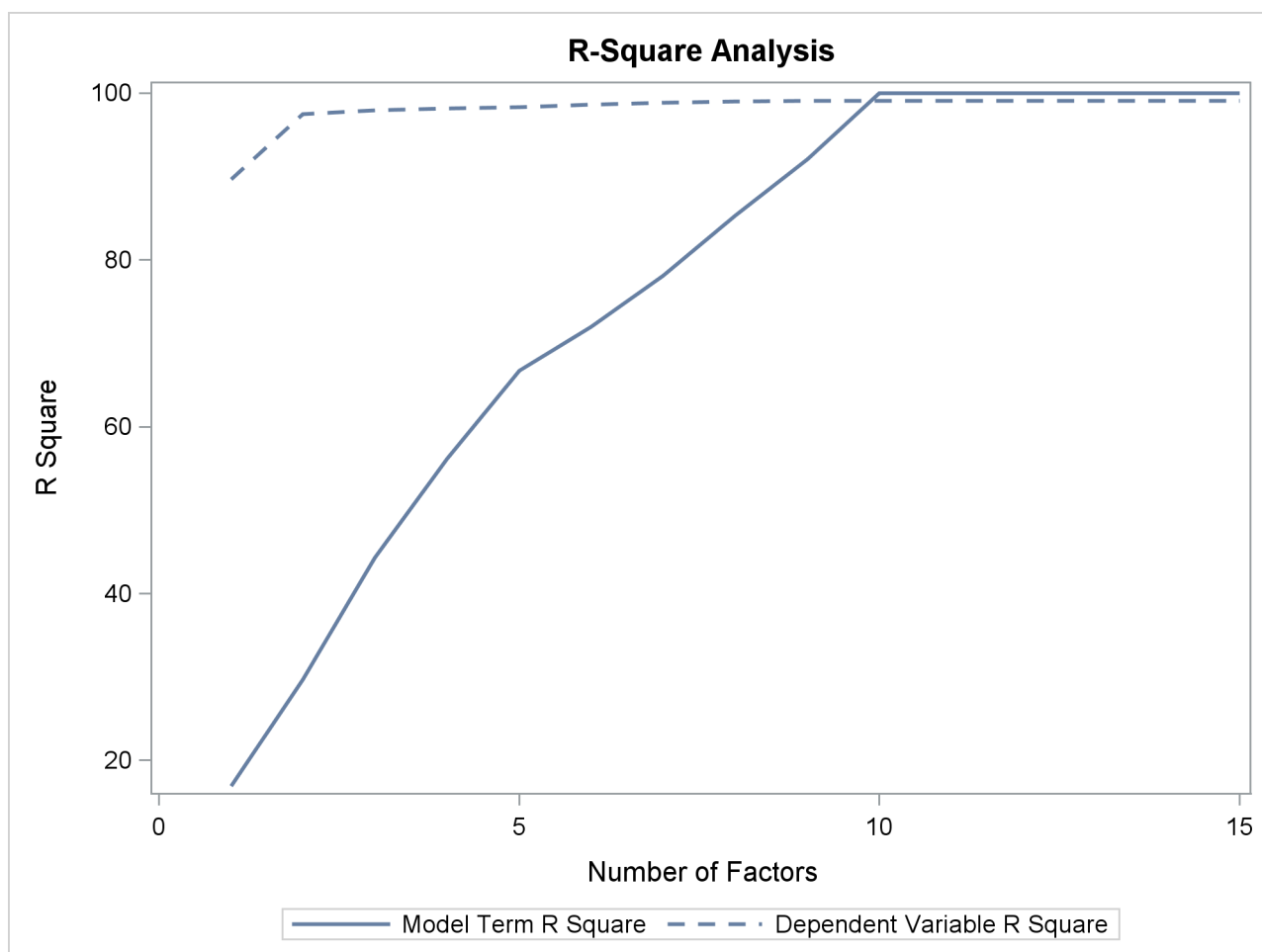
Output 76.1.2 Plot of Proportion of Variation Accounted For
