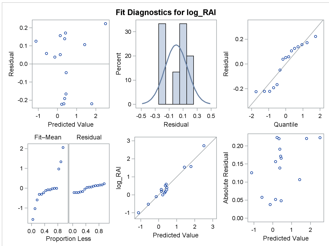
Output 76.2.1 Model Fit Diagnostics
