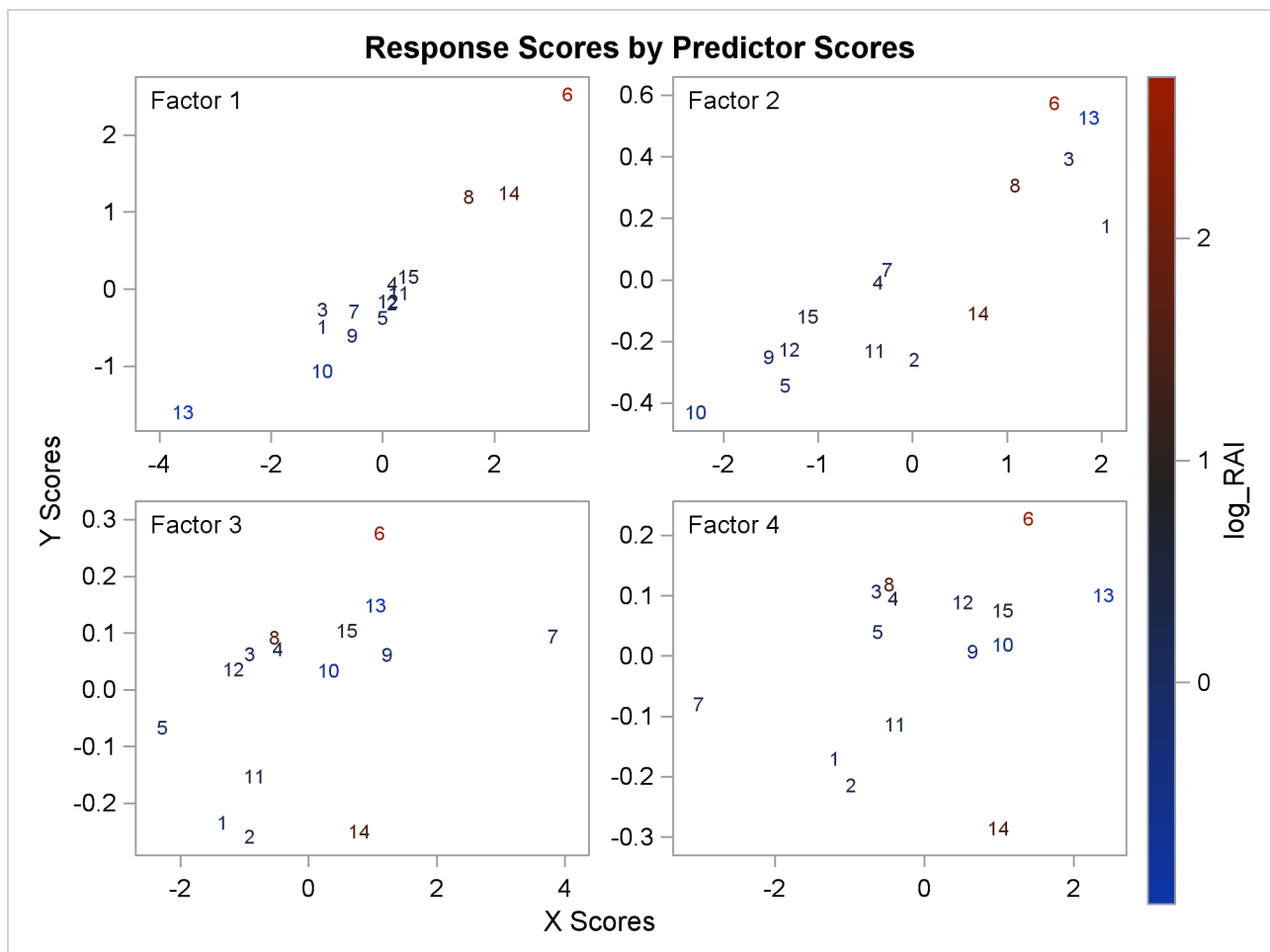
Output 76.1.4 X-Scores versus Y-Scores
