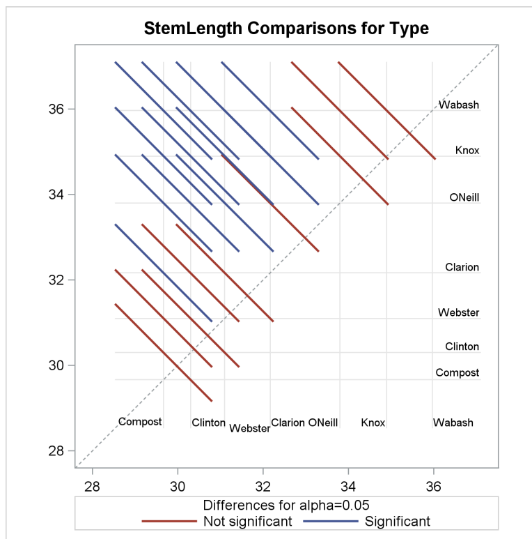
Figure 21.10 LS-Means Diffogram
