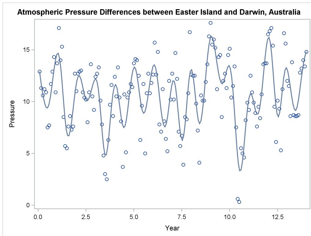
Figure 21.61 Penalized B-Spline Fit with PROC SGPLOT
