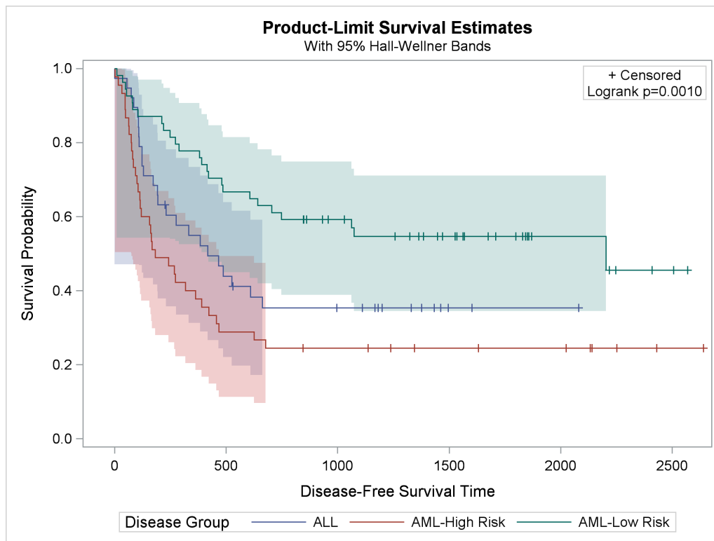
Figure 21.4 Survival Plot
