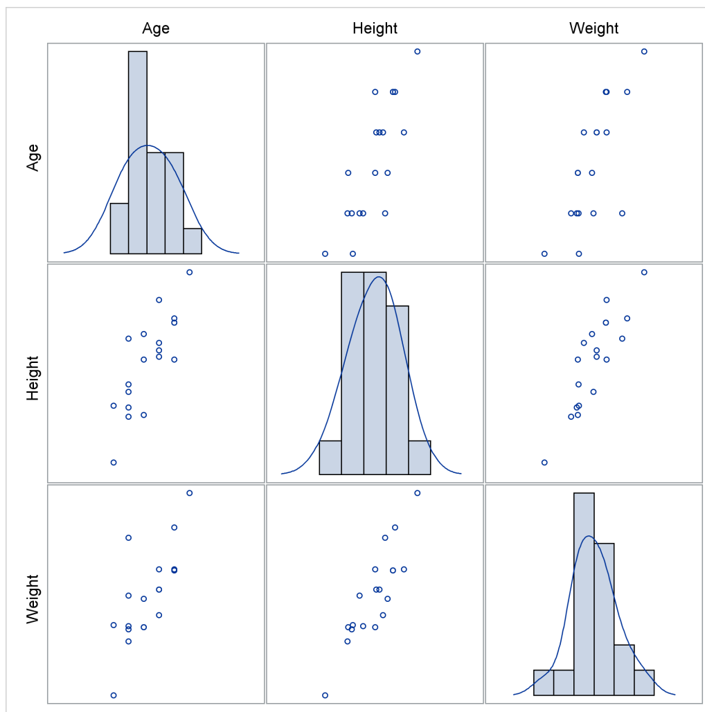
Figure 21.62 Scatter Plot Matrix with PROC SGSCATTER
