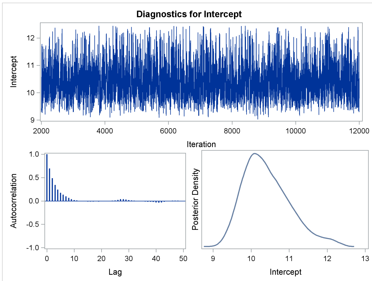
Figure 57.11 Diagnostic Plots
