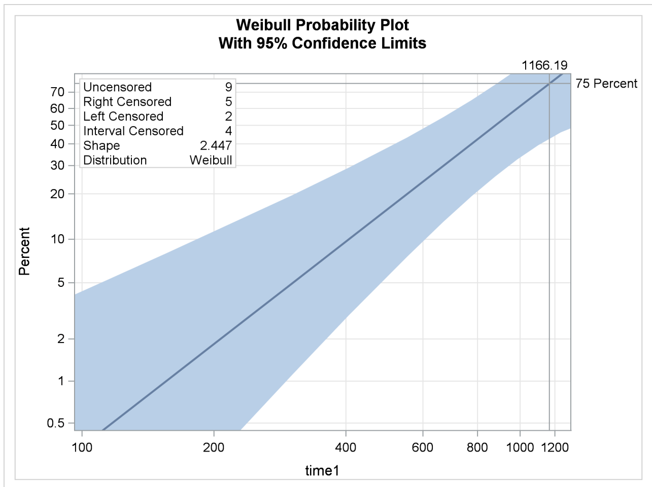
Output 57.4.3 Probability Plot for Recovery Time with sex = 2, age = 60.6
