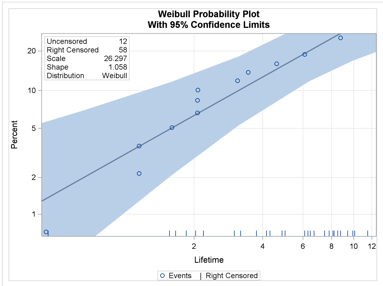
Output 57.5.1 Probability Plot for the Fan Data
