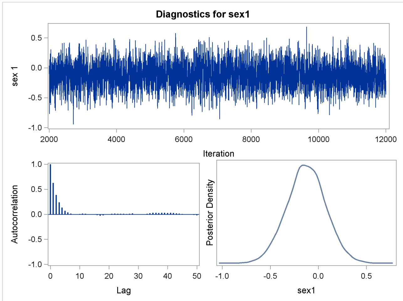
Output 57.7.8 Diagnostic Plots
