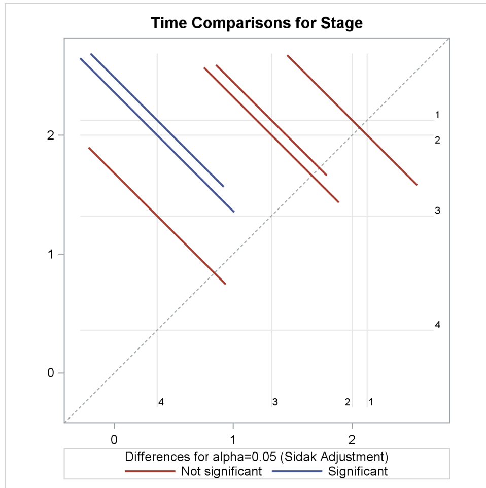
Output 57.8.2 Plot of Pairwise LS-Means Differences
