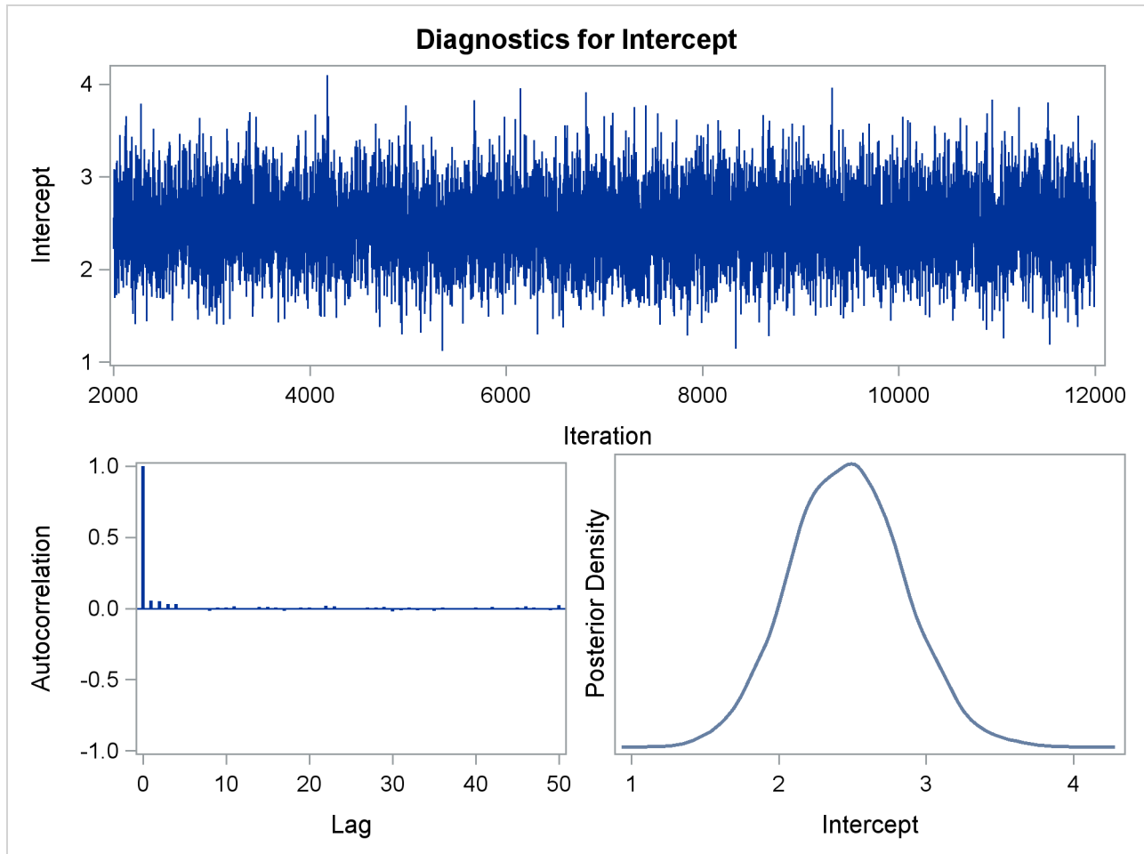
Output 57.7.6 Diagnostic Plots
