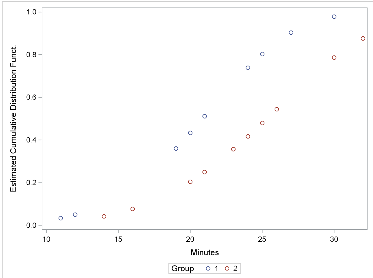
Figure 57.5 Plot of the Estimated Cumulative Distribution Function
