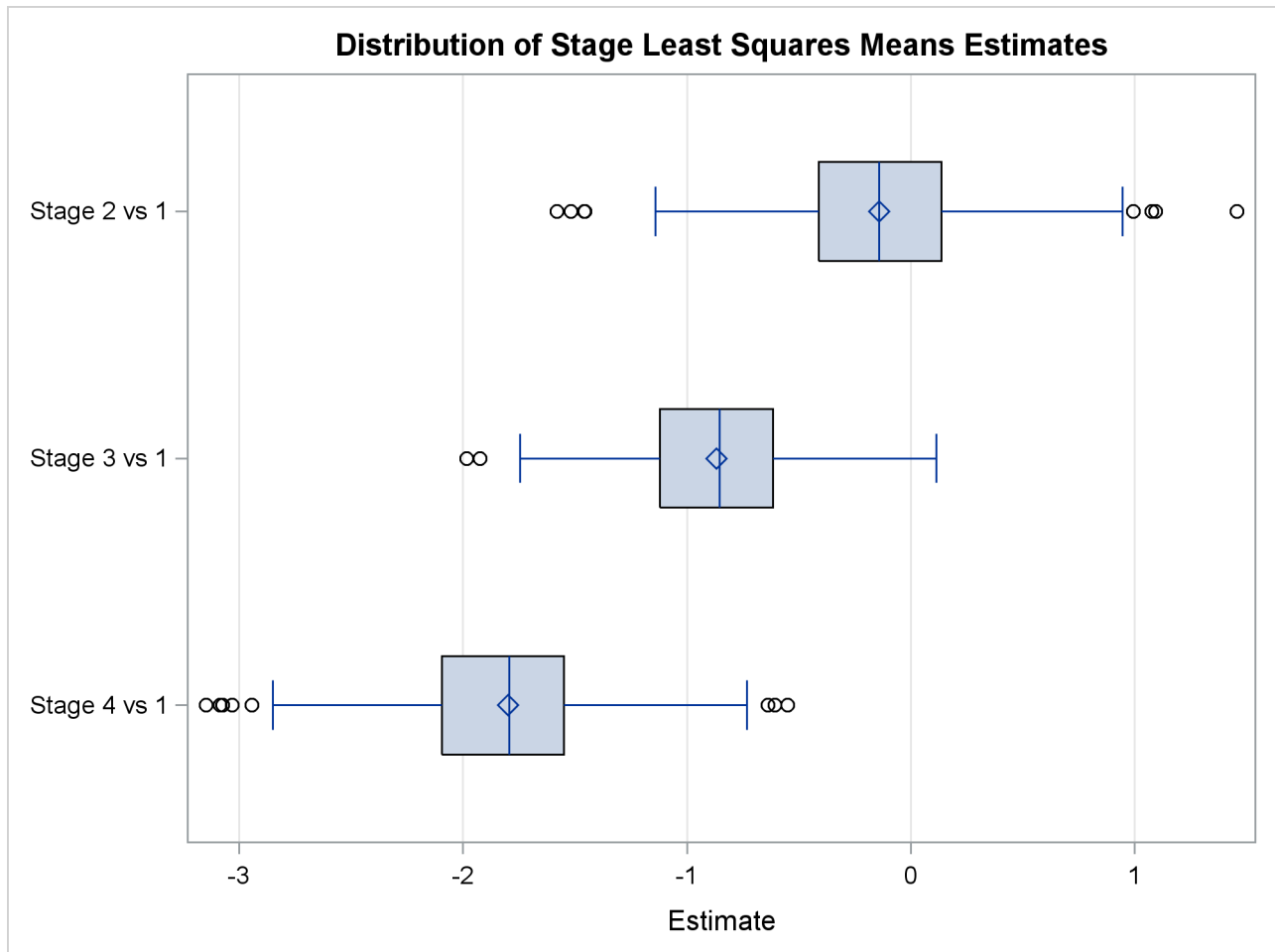
Output 57.8.8 Box Plot of Sampled LS-Means Differences
