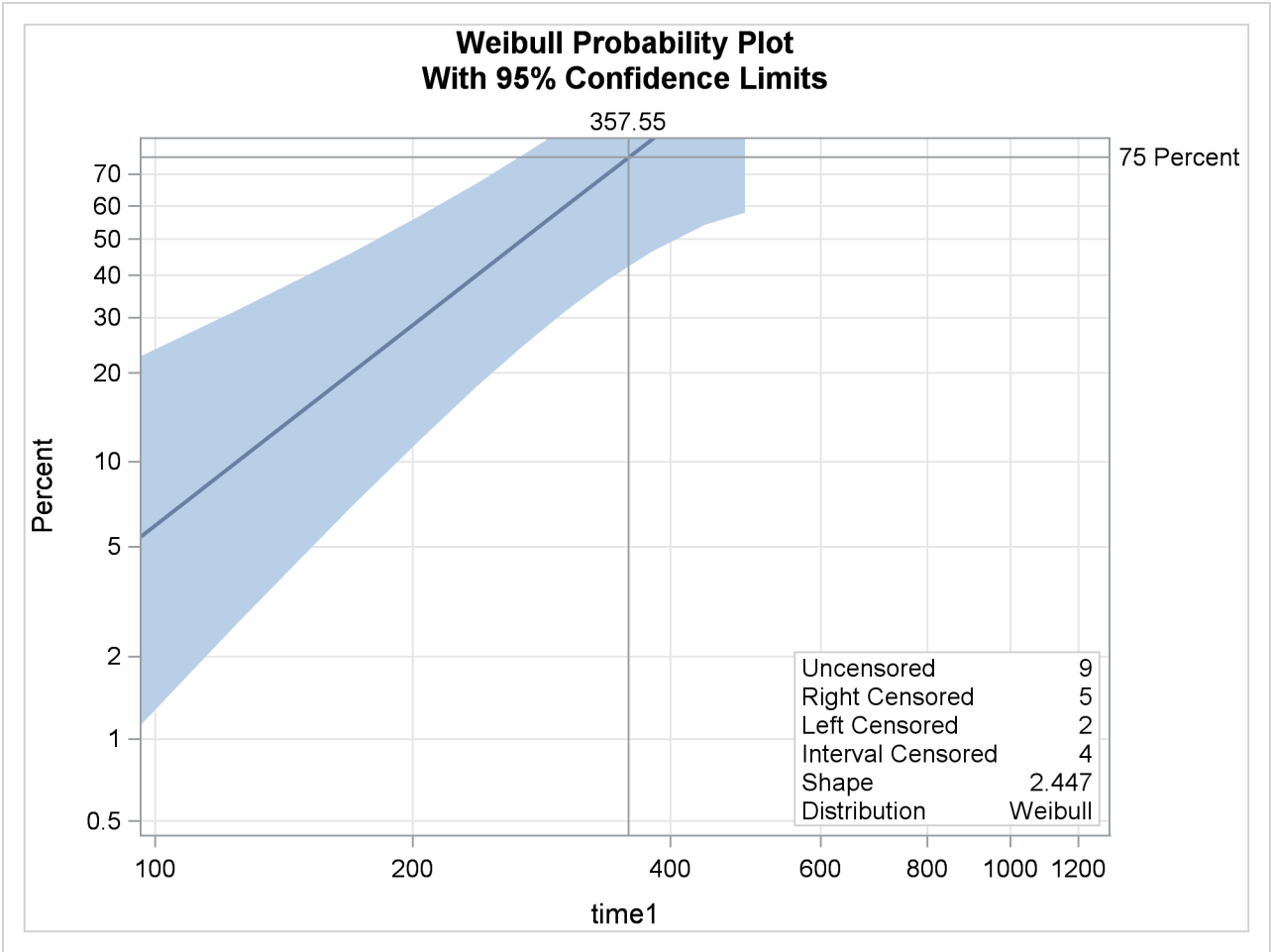
Output 57.4.2 Probability Plot for Recovery Time with sex = 1, age = 50
