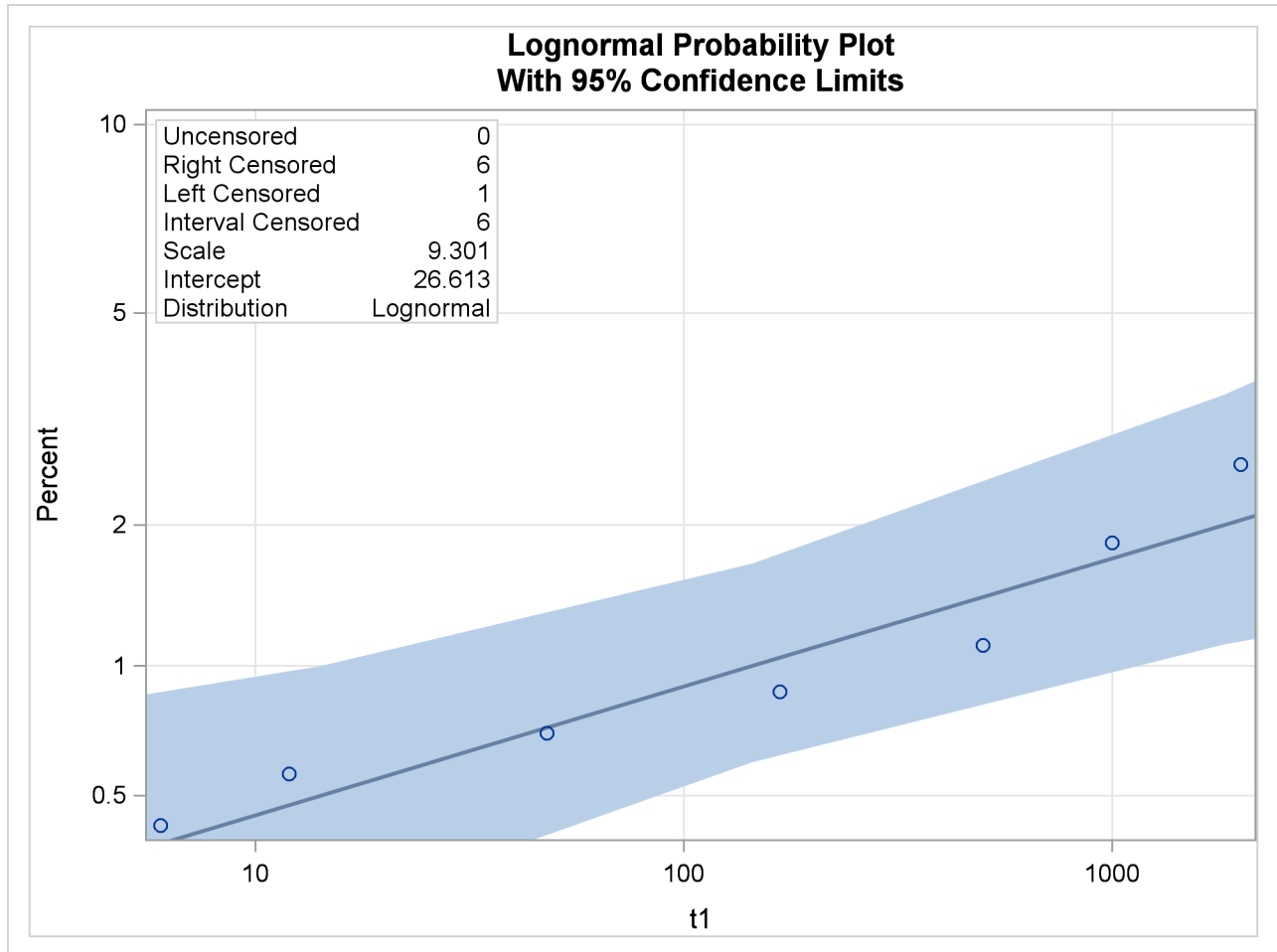
Output 57.6.4 Lognormal Probability Plot for the Microprocessor Data
