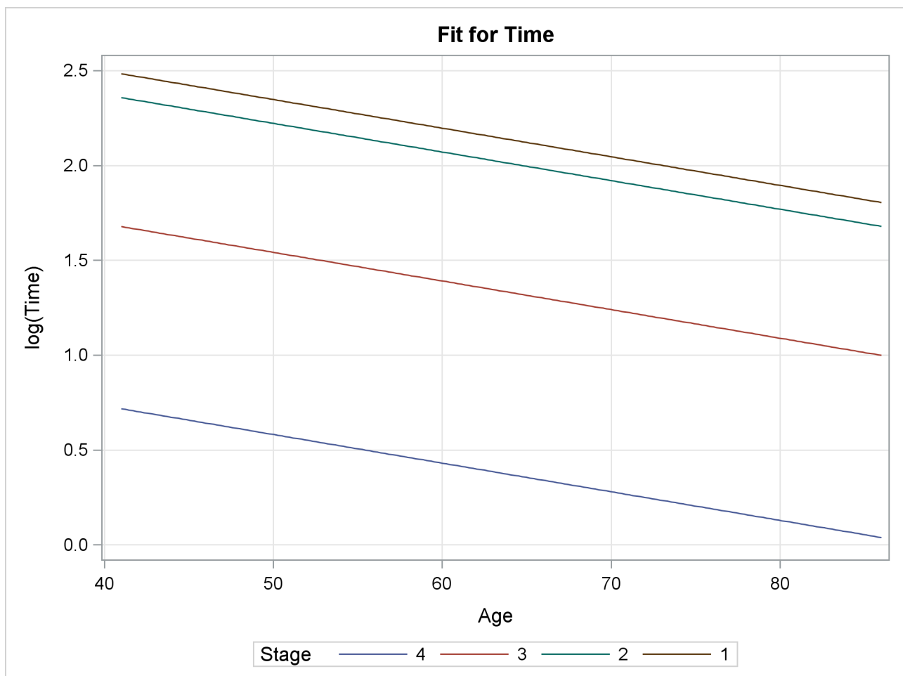
Output 57.8.4 Age Effects by Disease Stages
