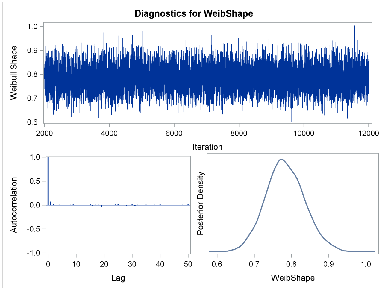
Output 57.7.10 Diagnostic Plots
