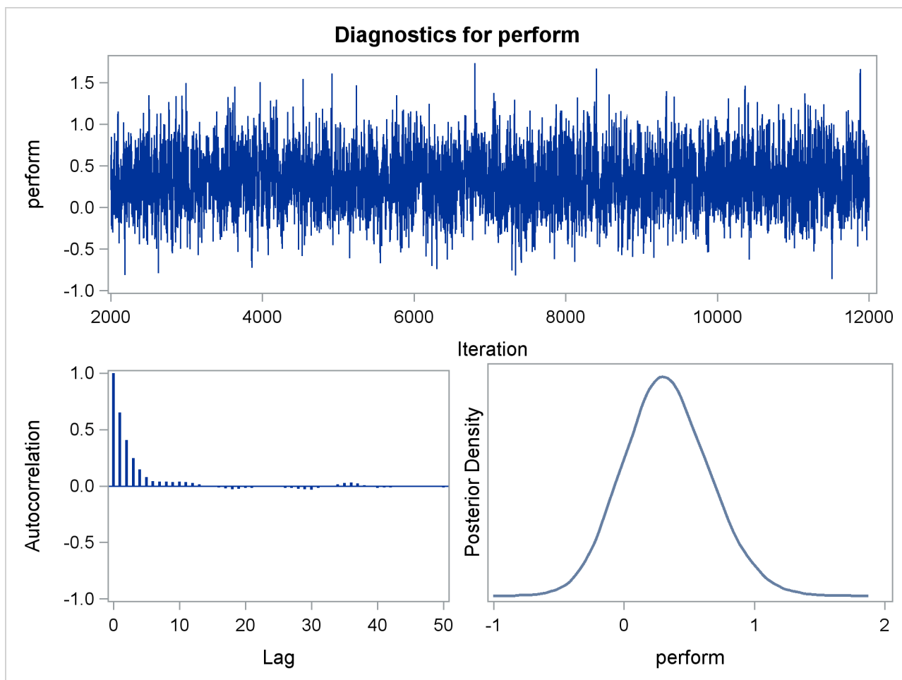
Output 57.7.9 Diagnostic Plots
