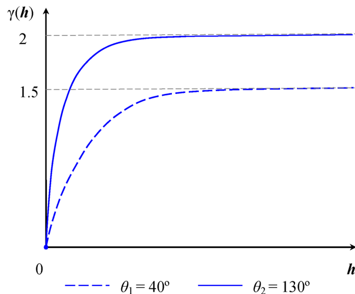
Figure 55.15 Zonal Anisotropy in Two Directions
