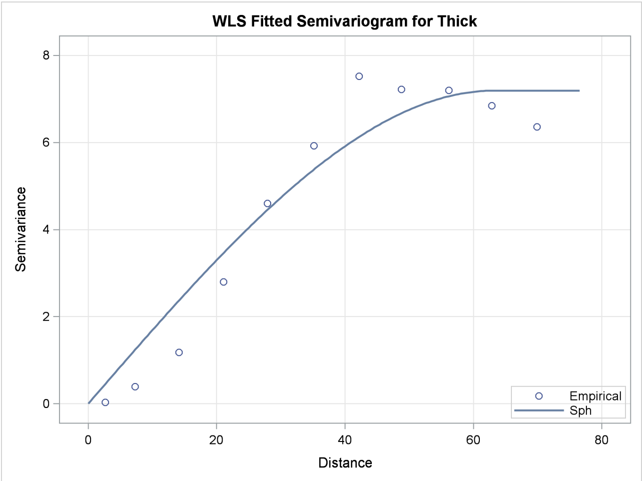
Output 55.2.3 Fitted Spherical and Empirical Thick Semivariogram
