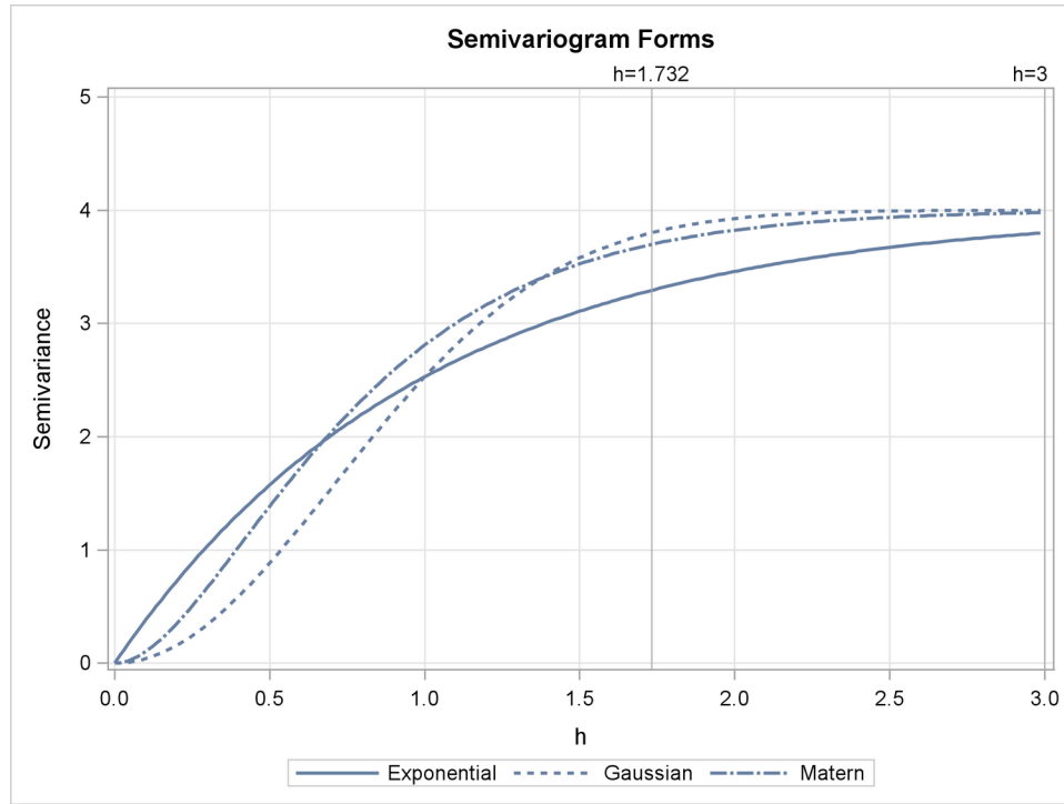
Figure 55.6 Gaussian, Exponential, and Matérn Semivariograms with Parameters a_0 = 1 , c_0 = 4 , and \nu = 1.5
