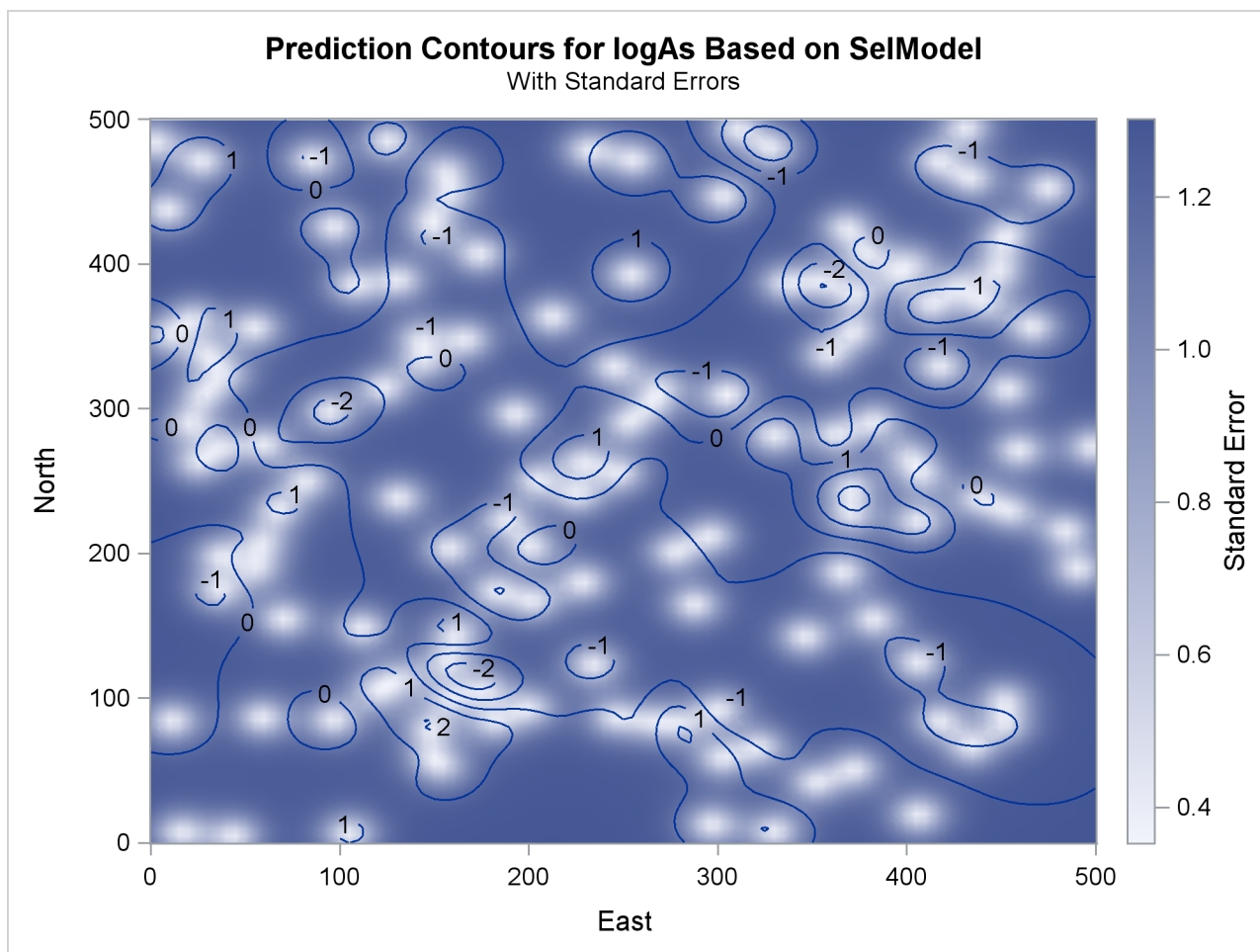
Output 55.1.7 Predicted Arsenic Logarithm Values with Gaussian-Gaussian Covariance
