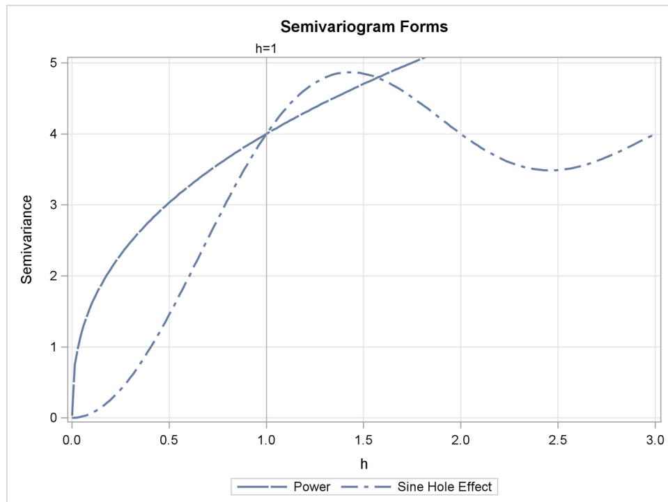
Figure 55.8 Sine Hole Effect Semivariogram with Range a_0 = 1 and Scale c_0 = 4 , and Power Semivariogram with Exponent a_0 = 0.4 and Slope c_0 = 4
