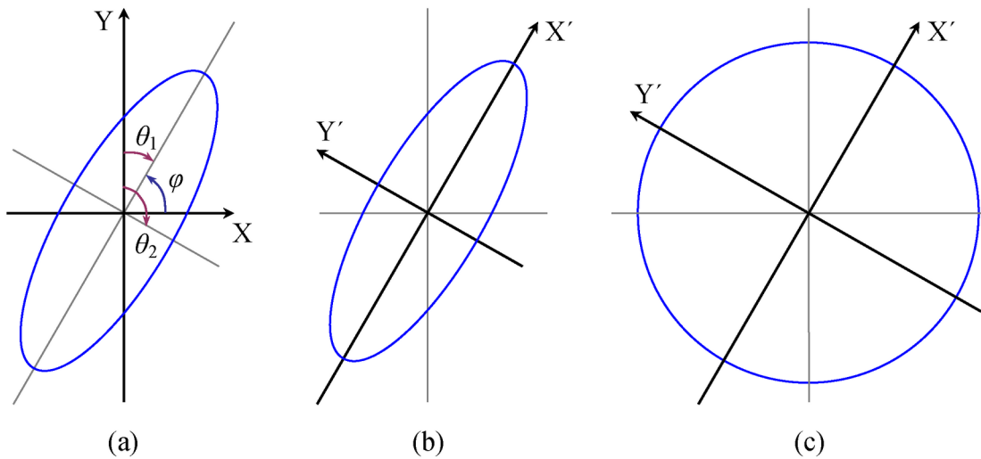
Figure 55.13 Transformation Applied to Geometric Anisotropy
