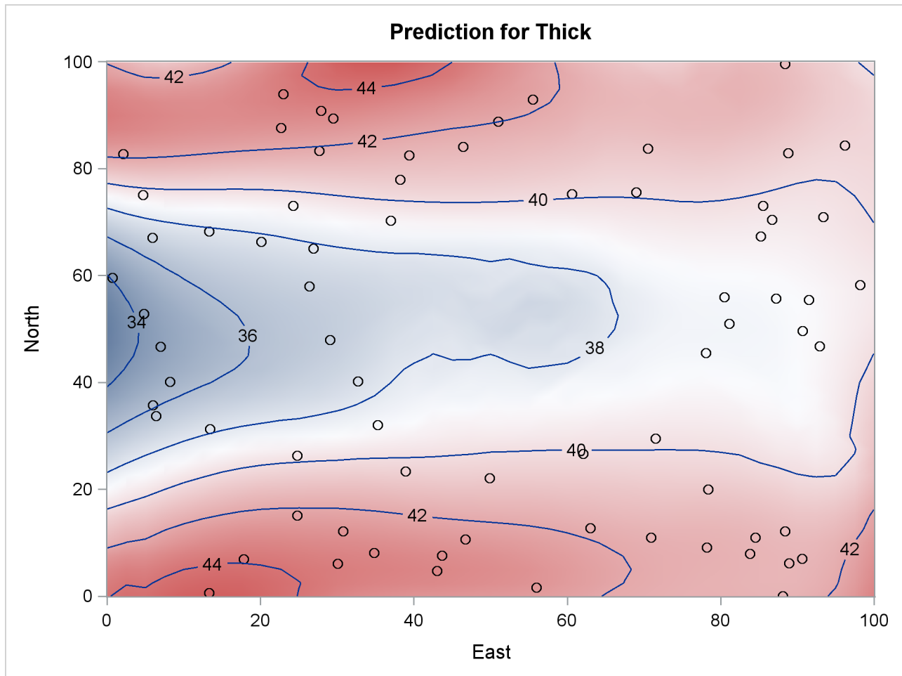
Output 55.3.3 Surface Plot and Contours of Kriged Coal Seam Thickness
