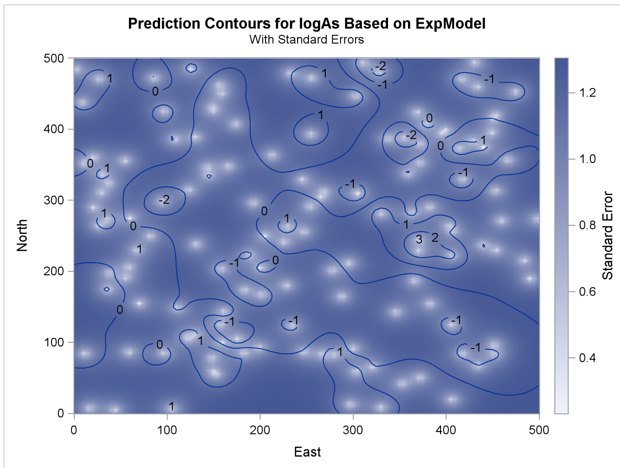
Output 55.1.10 Predicted Arsenic Logarithm Values with Exponential Covariance
