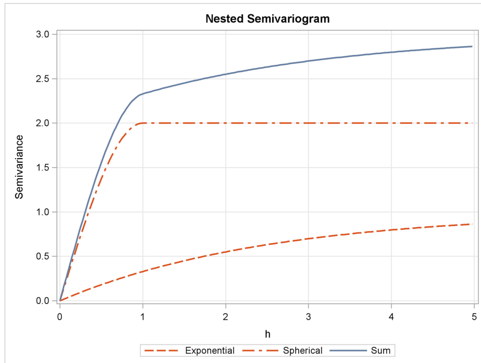
Figure 55.10 Sum of Exponential and Spherical Structures at Different Scales
