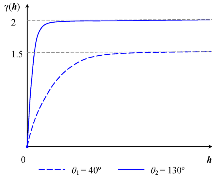
Figure 55.14 Zonal Anisotropy in Two Directions
