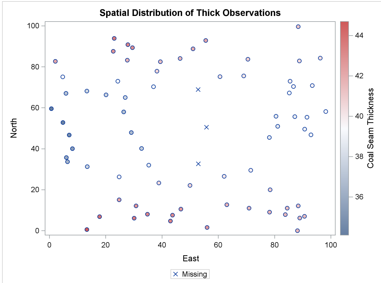
Output 55.3.2 Scatter Plot of the Observations Spatial Distribution
