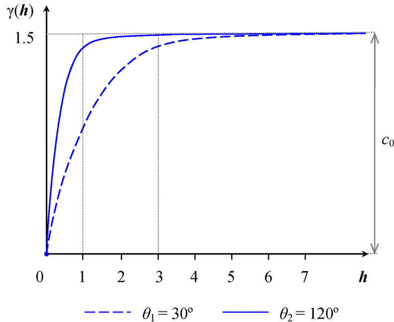
Figure 55.12 Geometric Anisotropy with Major Axis in the Direction \theta_1 = 30^\circ
