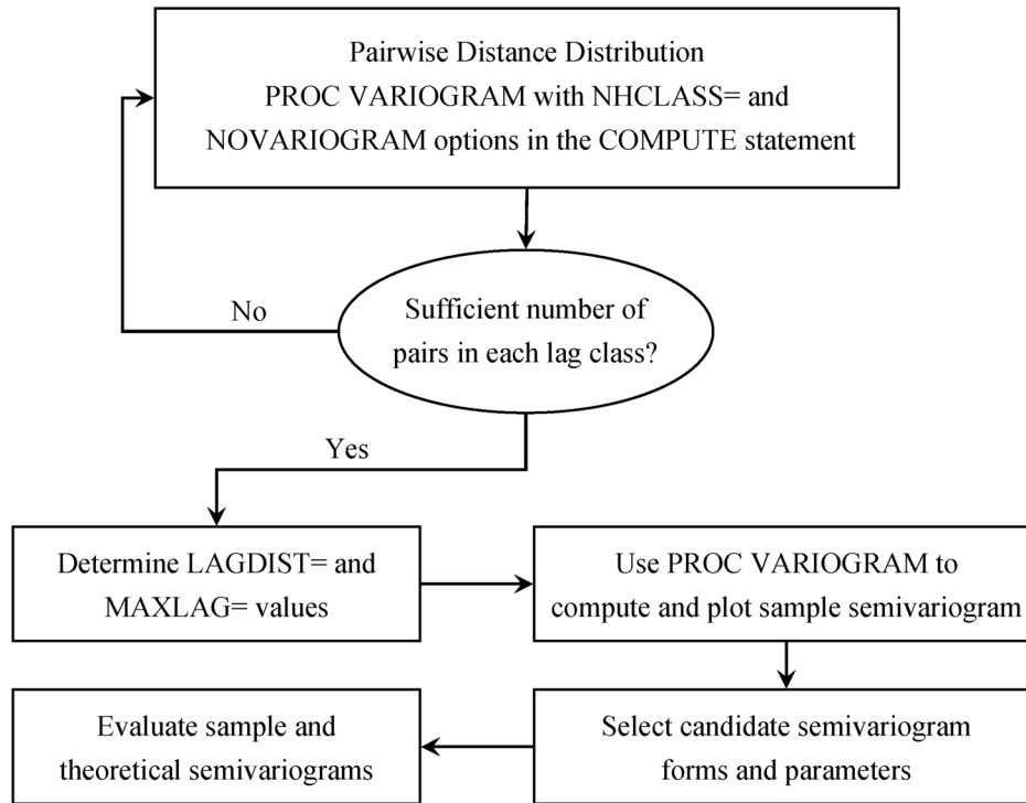
Figure 55.5 Flowchart for Semivariogram Selection
