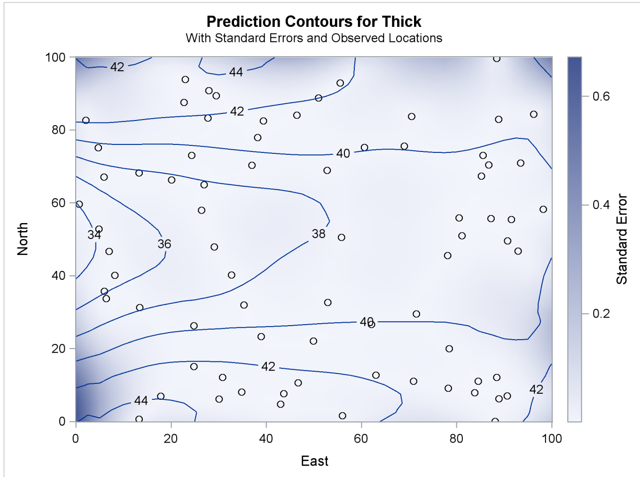
Figure 55.4 Contour Plot of Kriged Coal Seam Thickness
