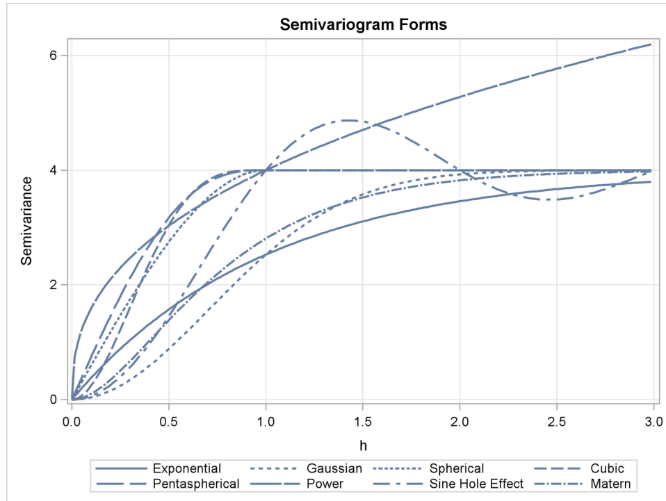
Figure 55.9 Semivariogram Forms Used in PROC KRIGE2D
