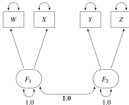
Figure 17.23 H3: Congeneric (One-Factor) Model for Lord Data
