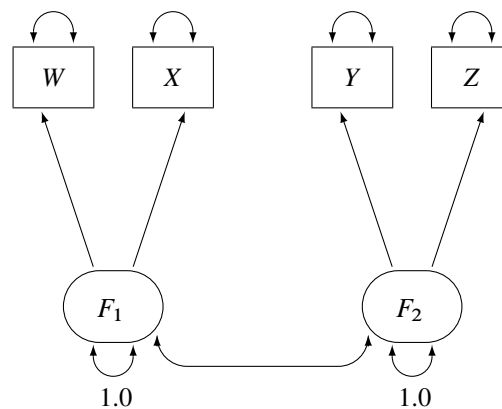
Figure 17.20 Simplified Path Diagram: Lord Data
