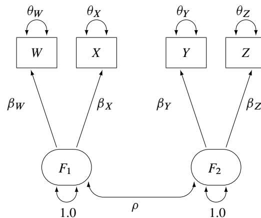
Figure 17.19 Path Diagram: Lord Data
