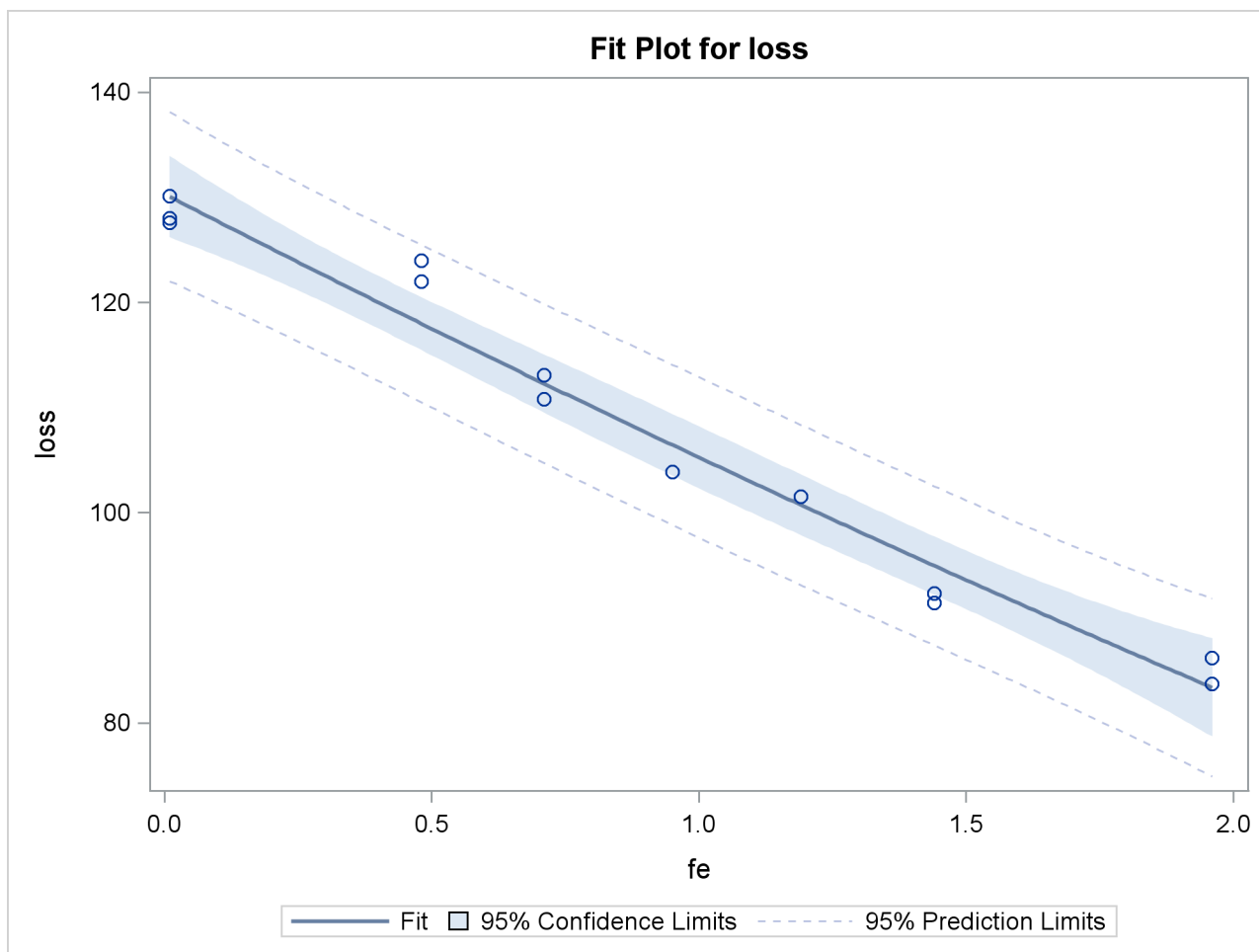
Figure 45.8 Plot of Observed and Fit Corrosion Resistance by Iron Content, Quadratic Model
