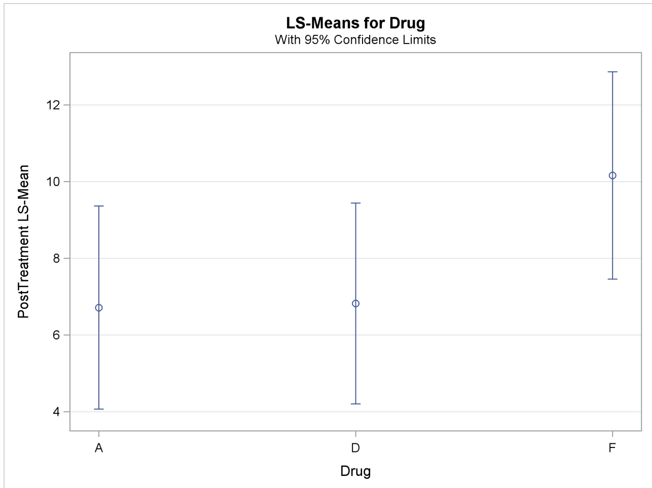
Output 45.4.7 LS-Means for PostTreatment Score by Drug
