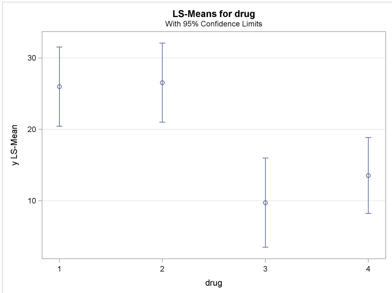
Output 45.3.6 Plot of Response LS-Means for Drug
