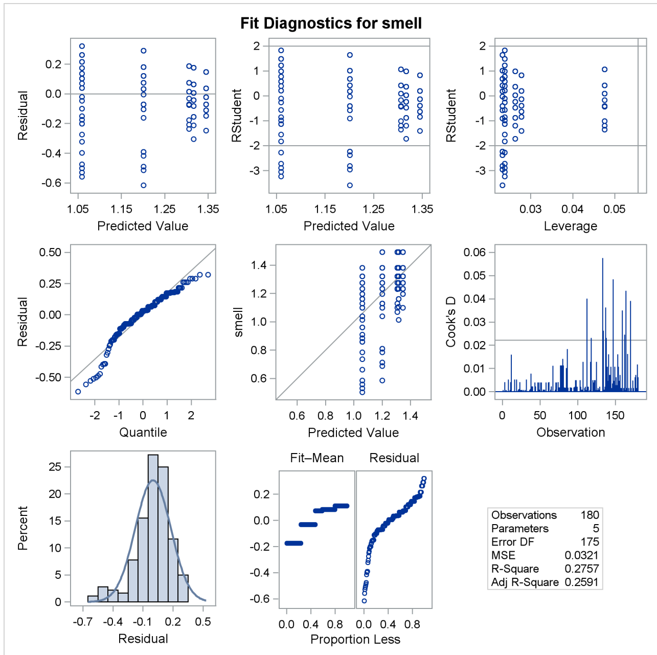
Output 45.10.5 Diagnostics for One-Way ANOVA of Olfactory Index by Age Group
