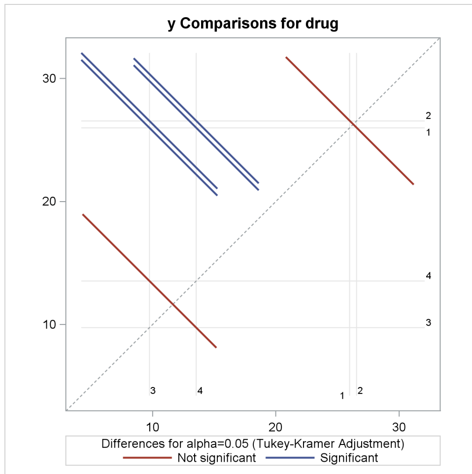
Output 45.3.7 Plot of Response LS-Mean Differences for Drug
