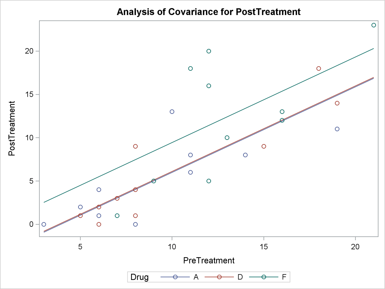
Output 45.4.6 Analysis of Covariance Plot of PostTreatment Score by Drug and PreTreatment Score
