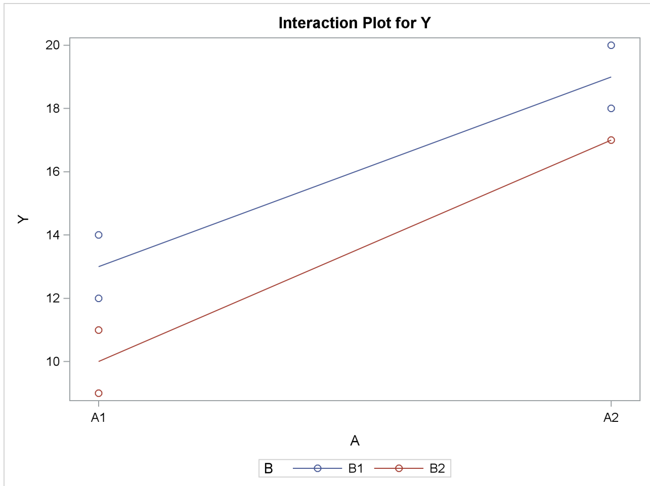
Figure 45.3 Plot of Y by A and B
