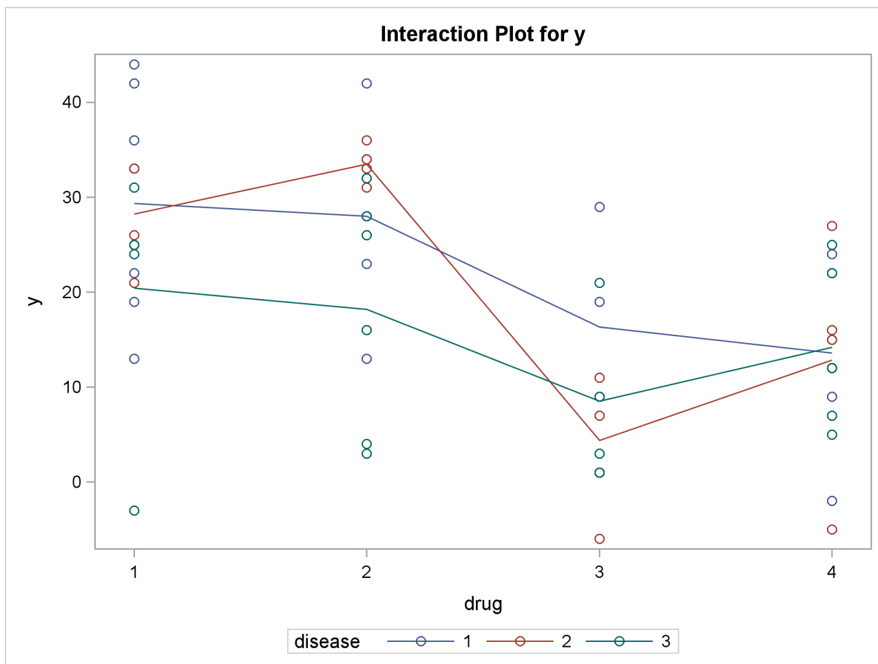
Output 45.3.5 Plot of Response by Drug and Disease
