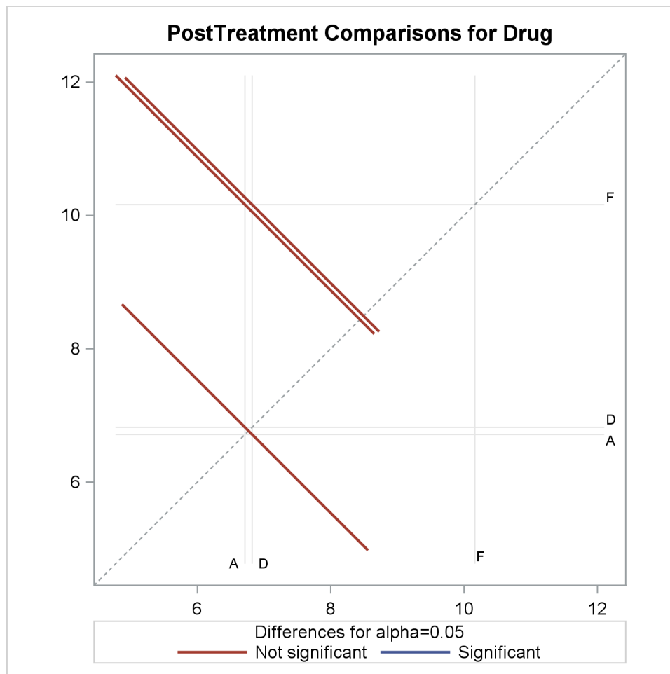
Output 45.4.8 Plot of Differences between Drug LS-Means for PostTreatment Scores
