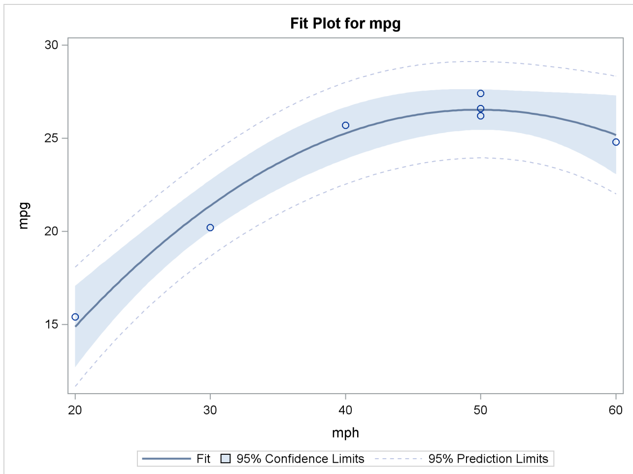
Output 45.2.4 Plot of Mileage Data
