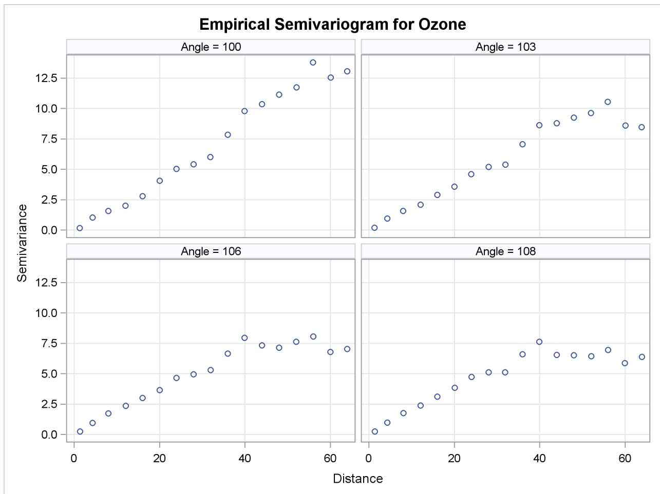
Output 106.3.2 Ozone Empirical Semivariograms in 100^\circ , 103^\circ , 106^\circ , and 108^\circ
