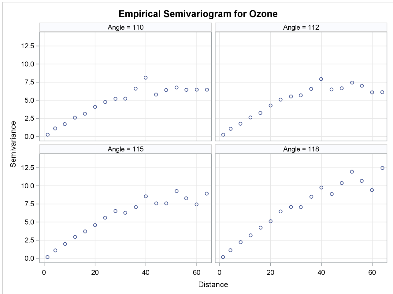
Output 106.3.3 Ozone Empirical Semivariograms in 110°, 112°, 115°, and 118°
