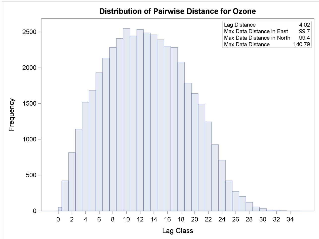
Output 106.2.3 Distribution of Pairwise Distances for Ozone Observation Data
