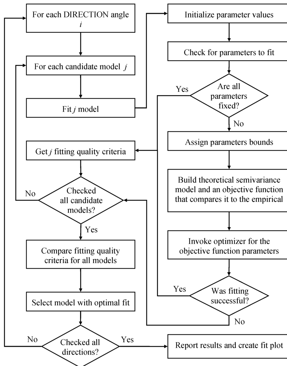
Figure 106.25 Semivariogram Fitting Process Flowchart
