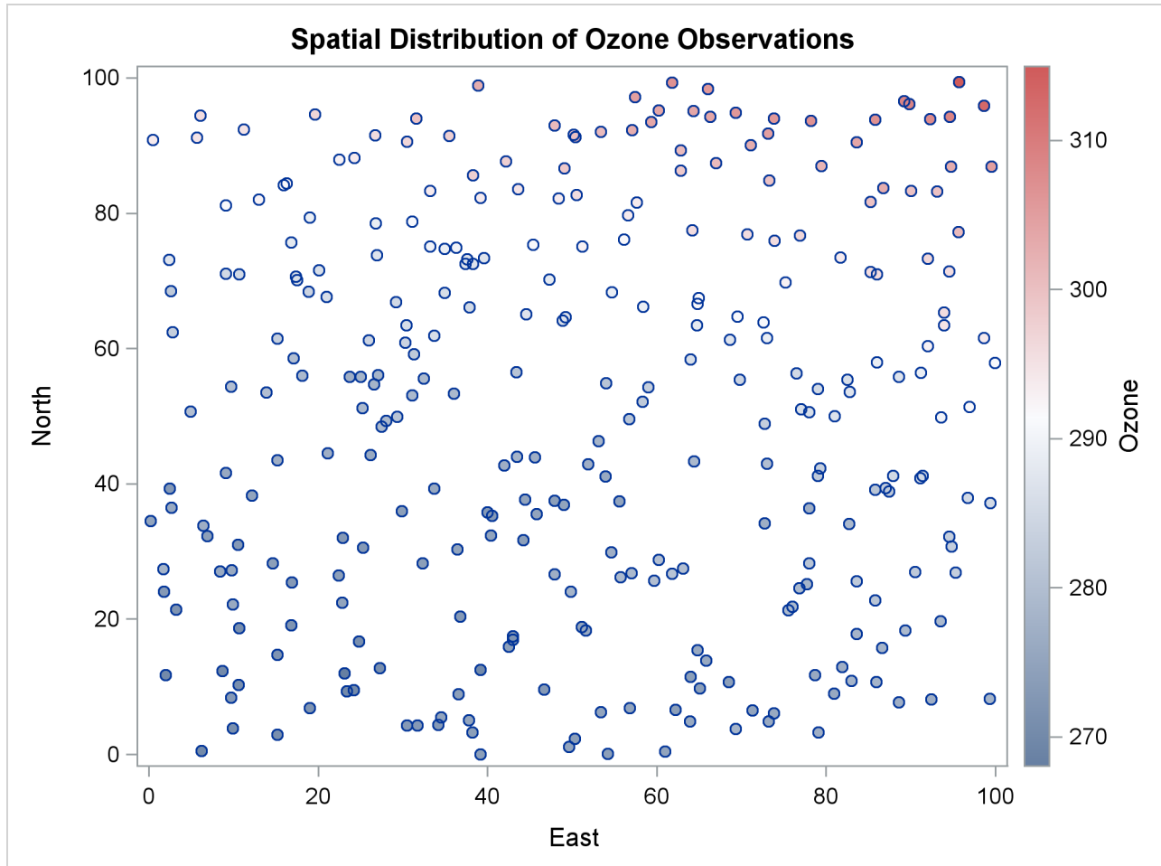
Output 106.2.1 Ozone Observation Data Scatter Plot
