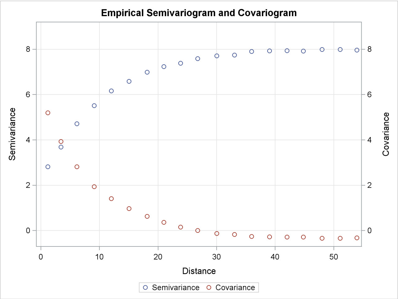
Output 106.4.1 Average Empirical Semivariogram and Covariogram from 500 Simulations
