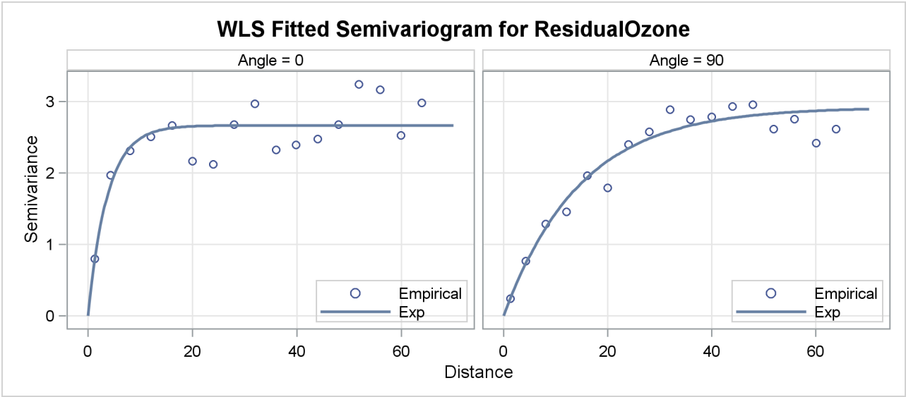
Output 106.2.12 Fitted Theoretical and Empirical Semivariogram for the Ozone Data in the \theta = 0^\circ and \theta = 90^\circ Directions
