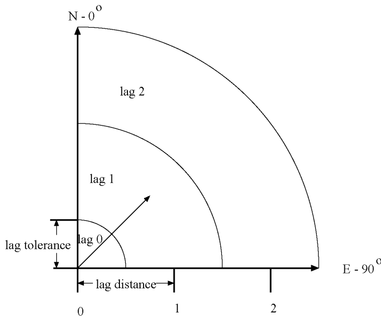
Figure 106.21 Selected Pair P_1P_2 Falls within the First Lag Class
