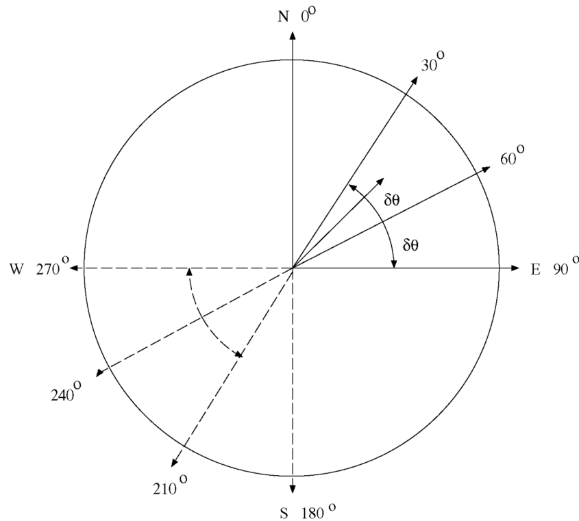
Figure 106.20 Selected Pair P_1 P_2 Falls within the Second Angle Class
