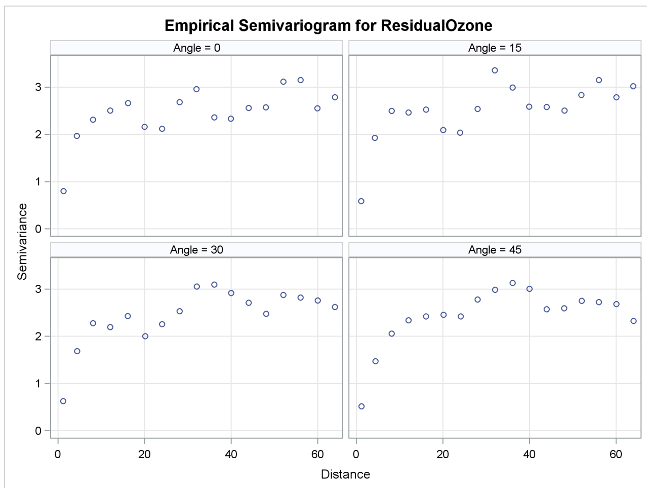
Output 106.2.6 Ozone Empirical Semivariograms with 0^\circ \leq \theta < 180^\circ and \delta\theta = 15^\circ
