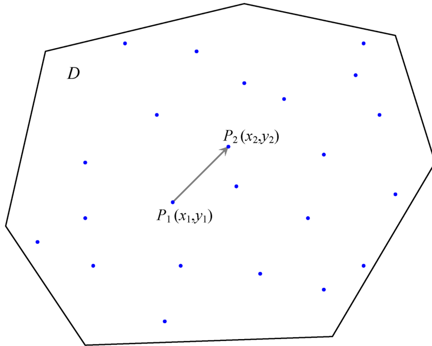
Figure 106.19 Selection of Points P_1 and P_2 in Spatial Domain D
