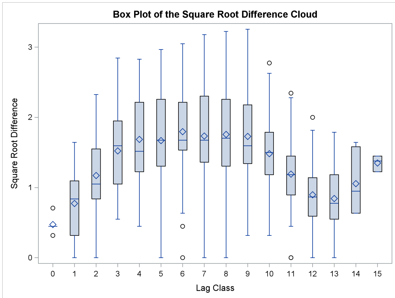
Output 106.5.2 Box Plot of the Square Root Difference Cloud
