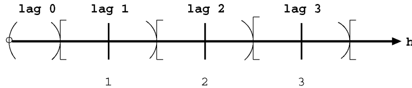
Figure 106.22 Lag Distance Axis Showing Lag Classes
