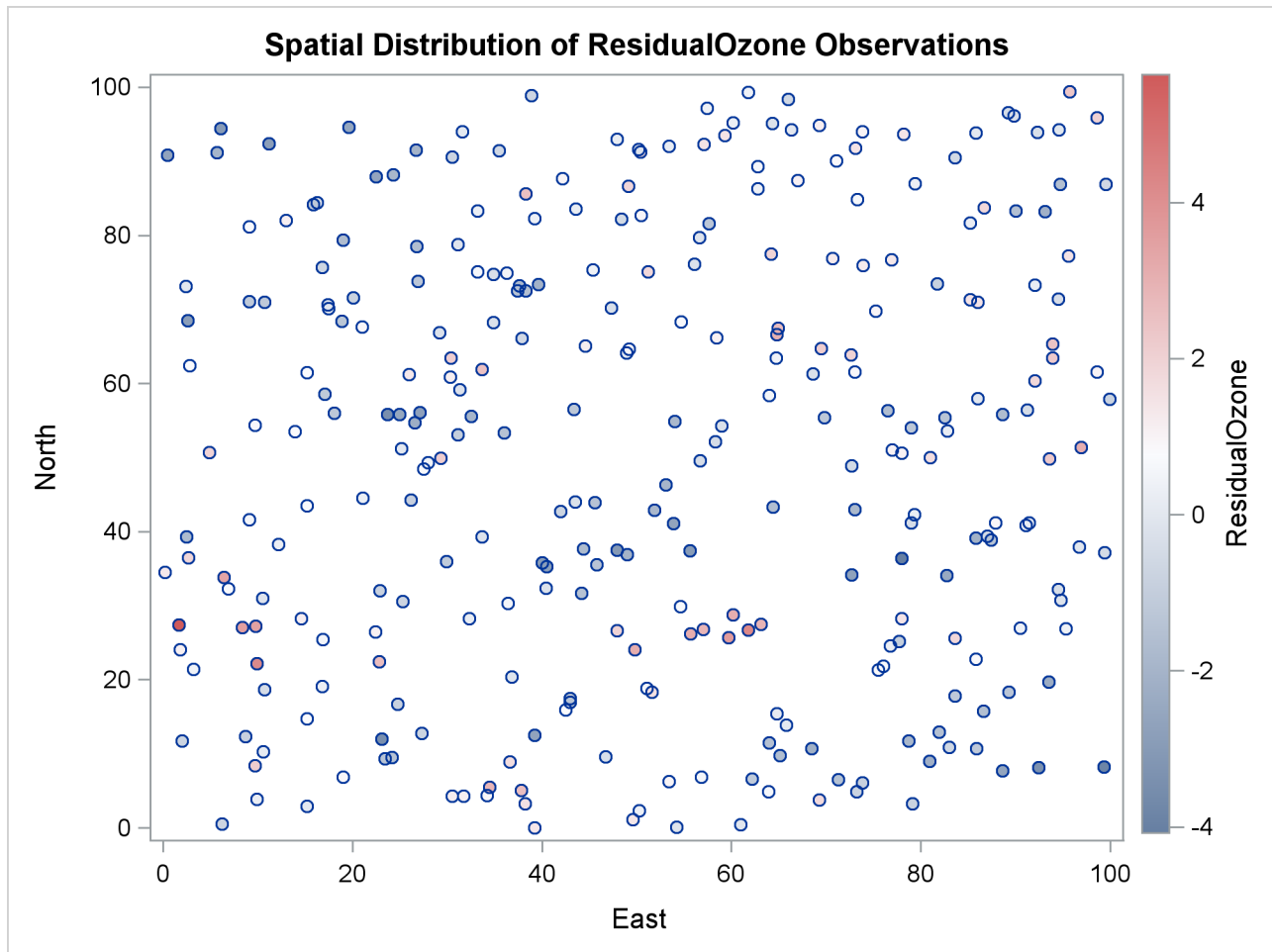
Output 106.2.5 Ozone Residual Observation Data Scatter Plot
