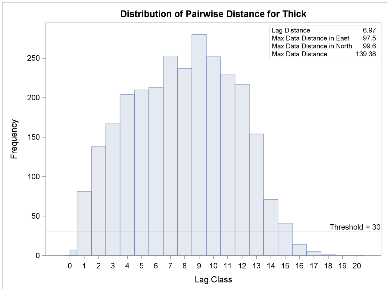
Figure 106.4 Distribution of Pairwise Distances
