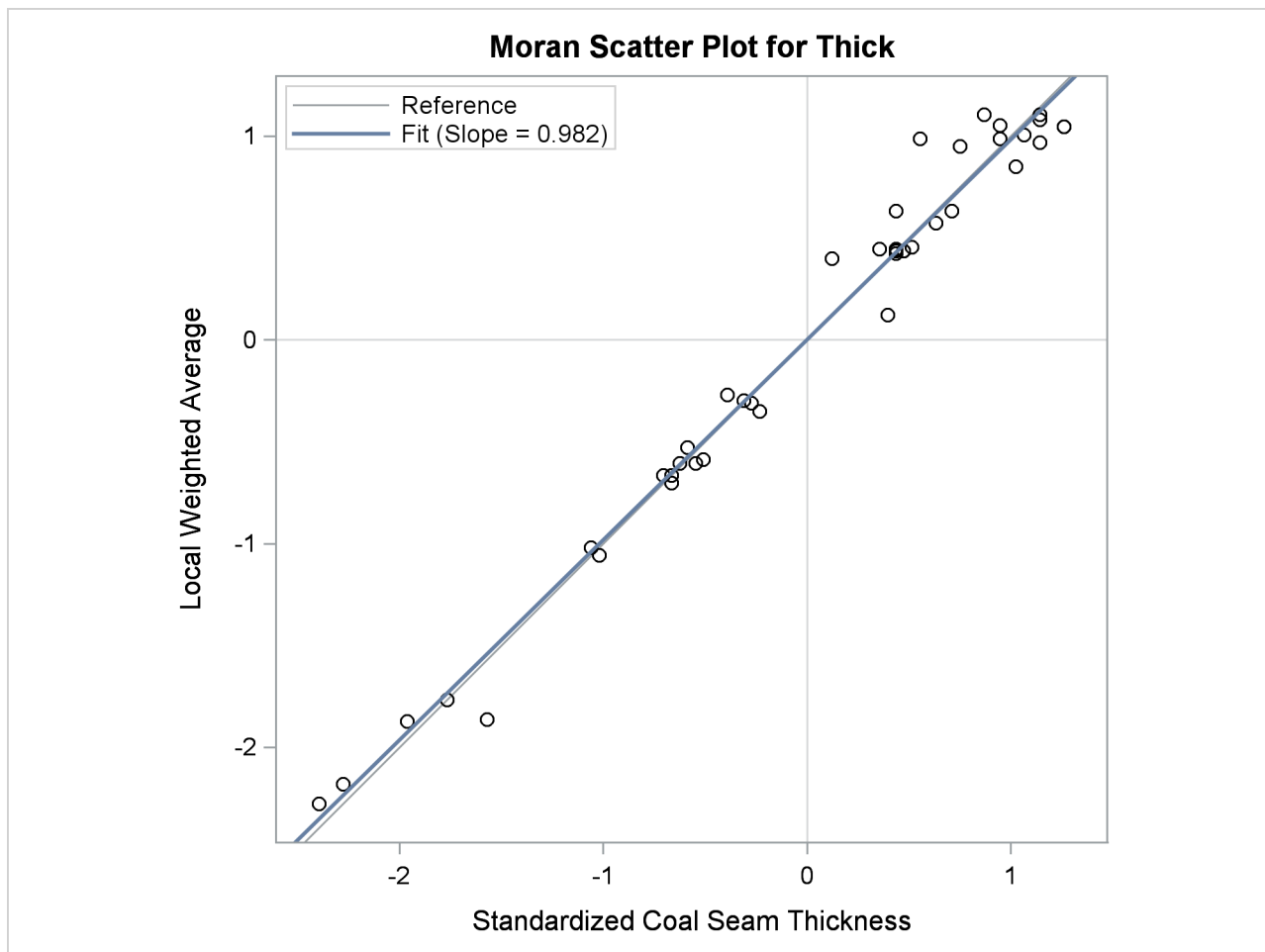
Figure 106.9 Moran Scatter Plot for Coal Seam Thickness Data
