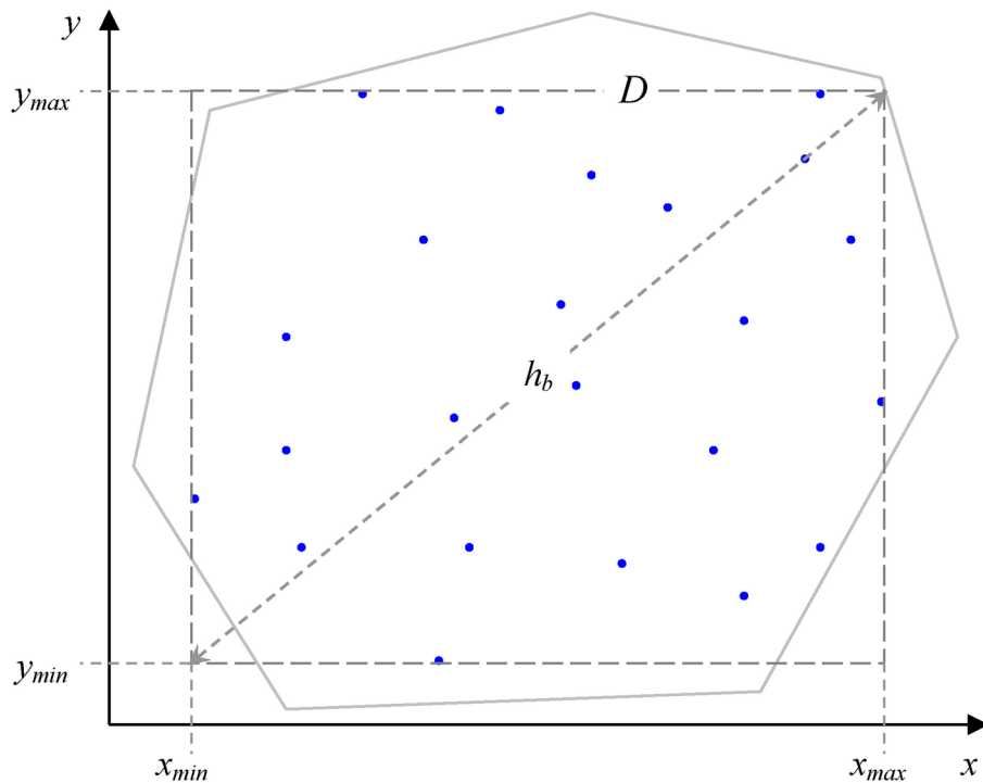
Figure 106.24 Bounding Rectangle to Determine Maximum Pairwise Distance in Domain D
