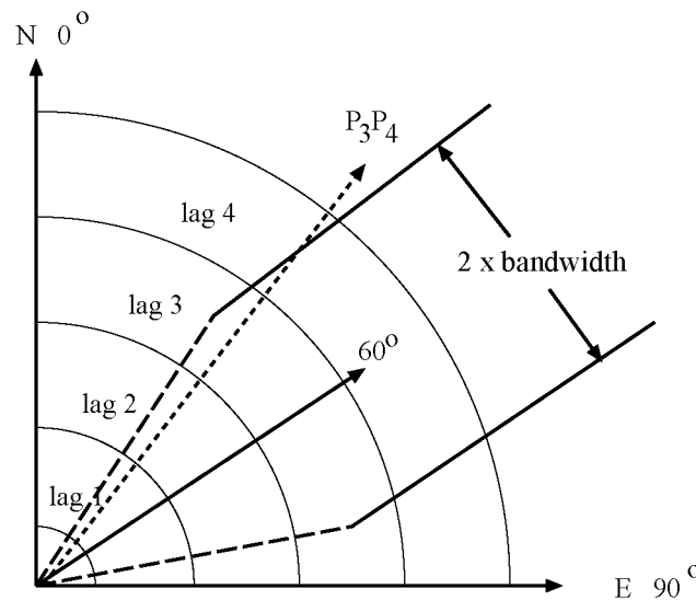
Figure 106.23 Selected Pair P_3P_4 Falls outside Bandwidth Limit
