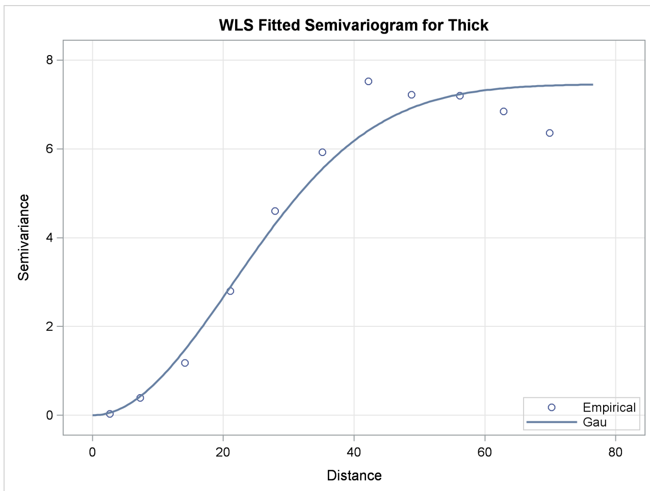
Figure 106.16 Fitted Theoretical and Empirical Semivariogram for Coal Seam Thickness
