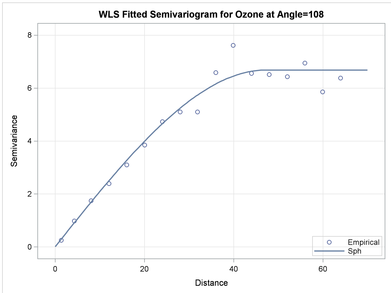
Output 106.3.6 Fitted Theoretical and Empirical Semivariogram for the Ozone Data in \theta = 108^\circ
