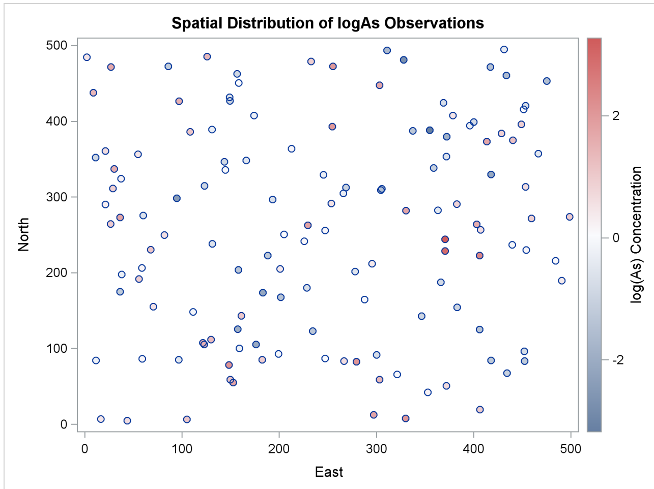
Output 106.1.1 logAs Observation Data Scatter Plot
