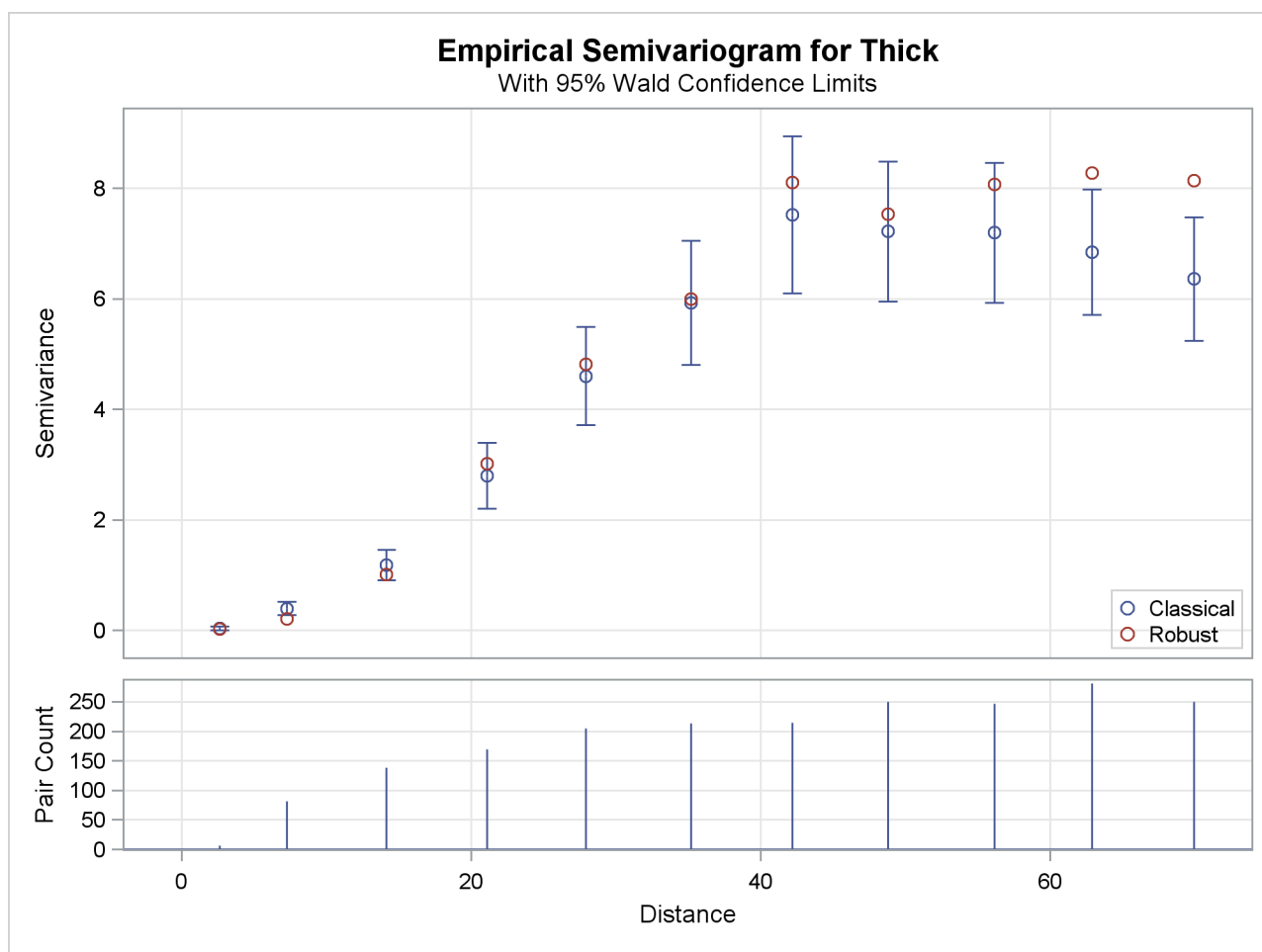
Figure 106.7 Classical and Robust Empirical Semivariograms for Coal Seam Thickness Data
