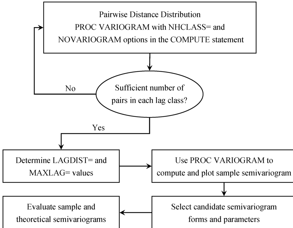
Figure 106.17 Flowchart for Semivariogram Selection
