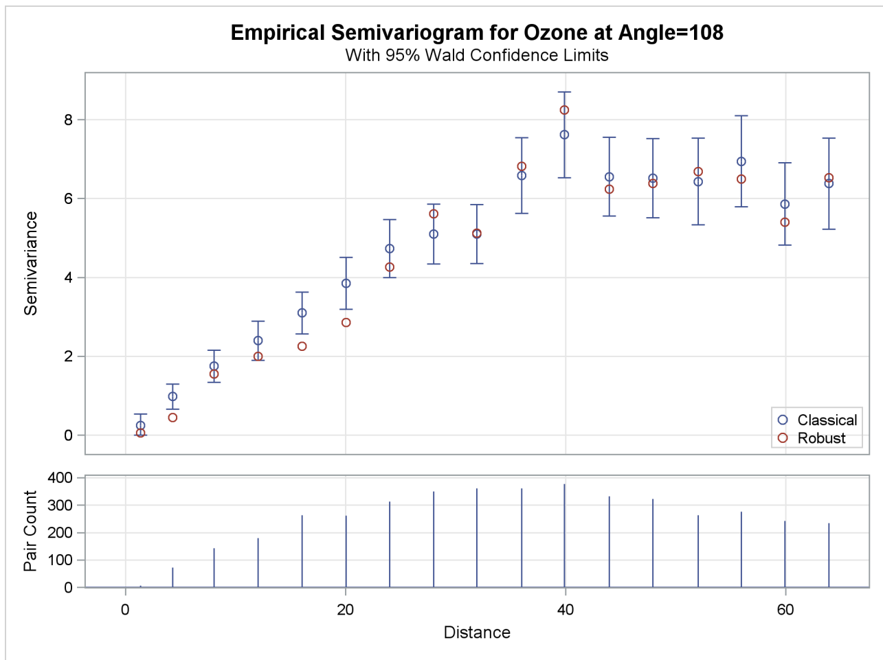
Output 106.3.4 Ozone Classical and Robust Empirical Semivariograms in \theta = 108^\circ
