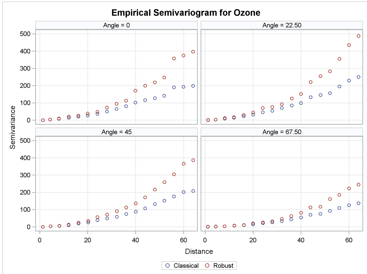
Output 106.3.1 Ozone Empirical Semivariograms with 0^\circ \leq \theta < 180^\circ and \delta\theta = 22.5^\circ
