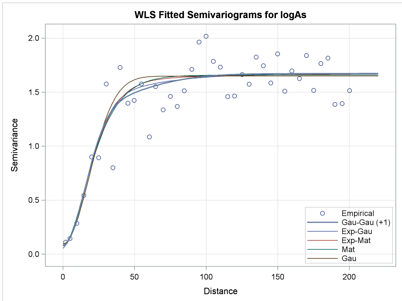
Output 106.1.9 Fitted Theoretical and Empirical logAs Concentration Semivariograms for the Specified Models
