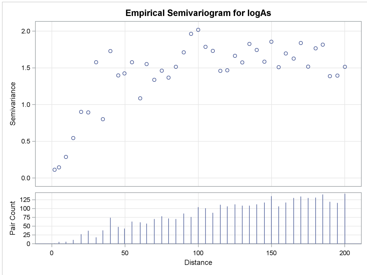
Output 106.1.4 Empirical Semivariogram for logAs Data
