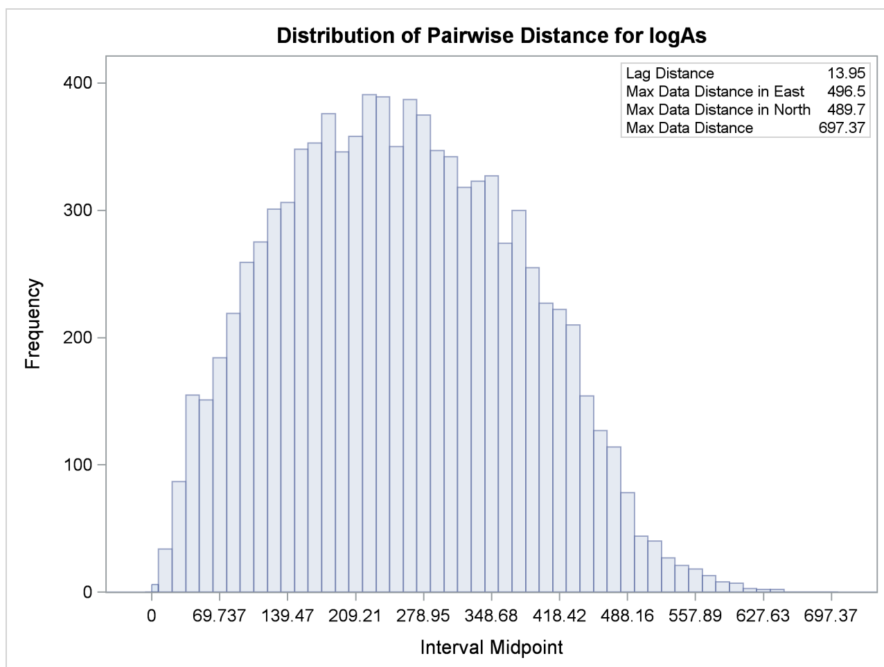
Output 106.1.2 Distribution of Pairwise Distances for logAs Data
