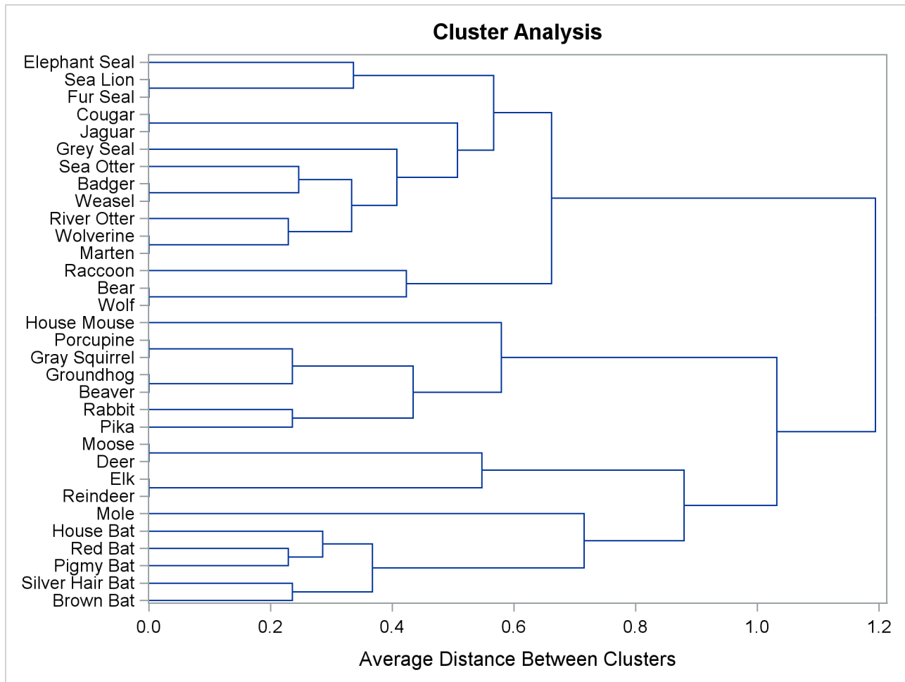
Output 102.1.2 Dendrogram from PROC CLUSTER
