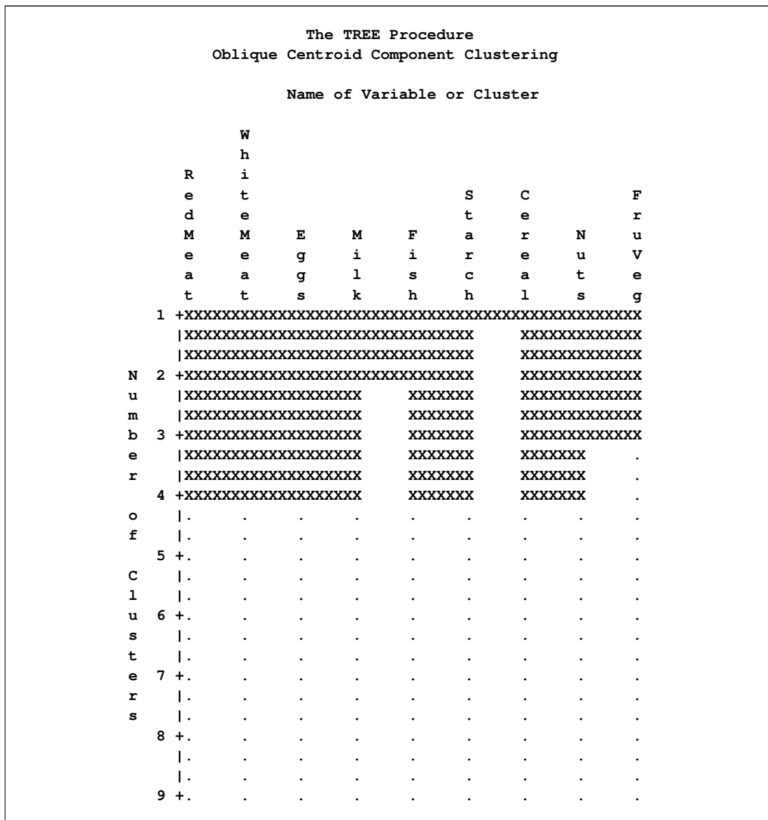
Figure 102.3 Line Printer Representation of the Tree Diagram
