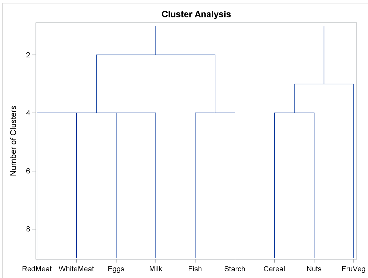
Figure 102.1 Dendrogram from PROC VARCLUS and ODS Graphics
