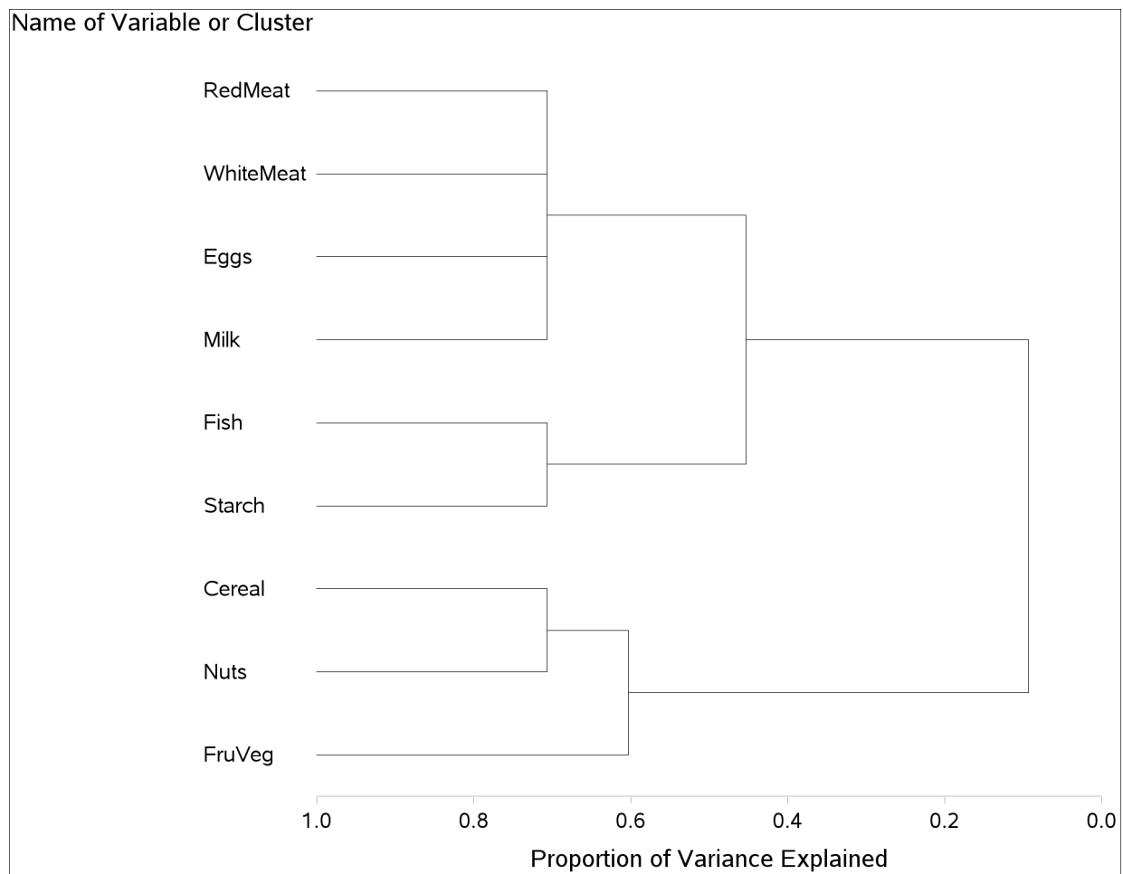
Figure 102.4 Horizontal Tree Diagram with _PROPOR_ as the HEIGHT Variable
