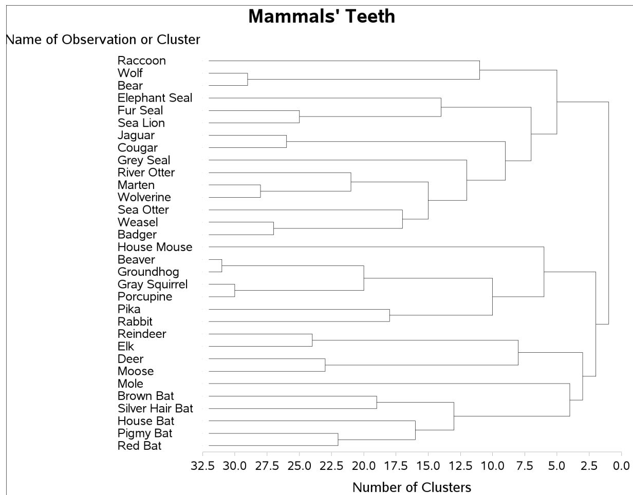
Output 102.1.5 PROC TREE with SORT and HEIGHT= Options
