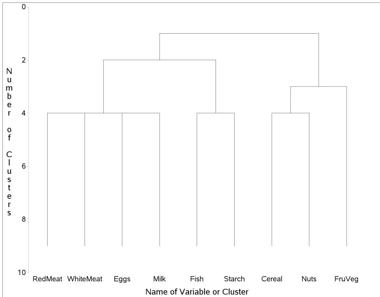
Figure 102.2 Graphical Tree Diagram from PROC TREE
