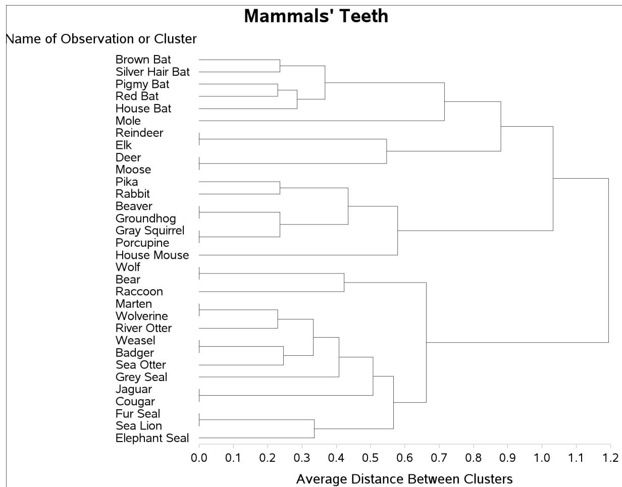
Output 102.1.3 Tree Diagram of Mammal Teeth Clusters
