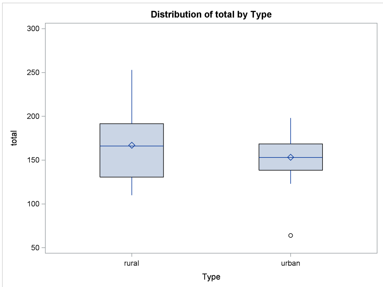
Figure 91.1 Schematic Plots from PROC BOXPLOT
