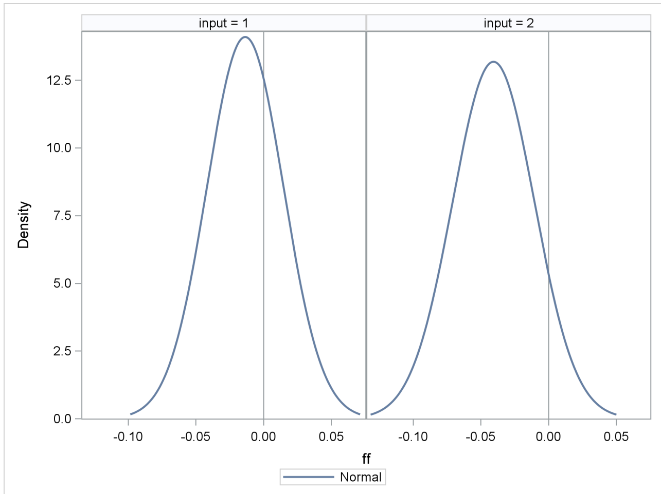
Figure 90.5 Frequency Plot for ff for Each Set of Input Values
