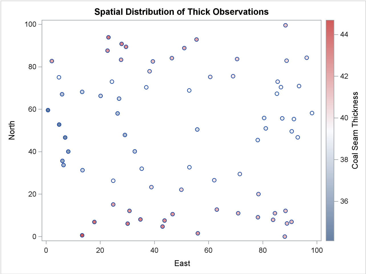
Figure 89.2 Scatter Plot of the Observations Spatial Distribution
