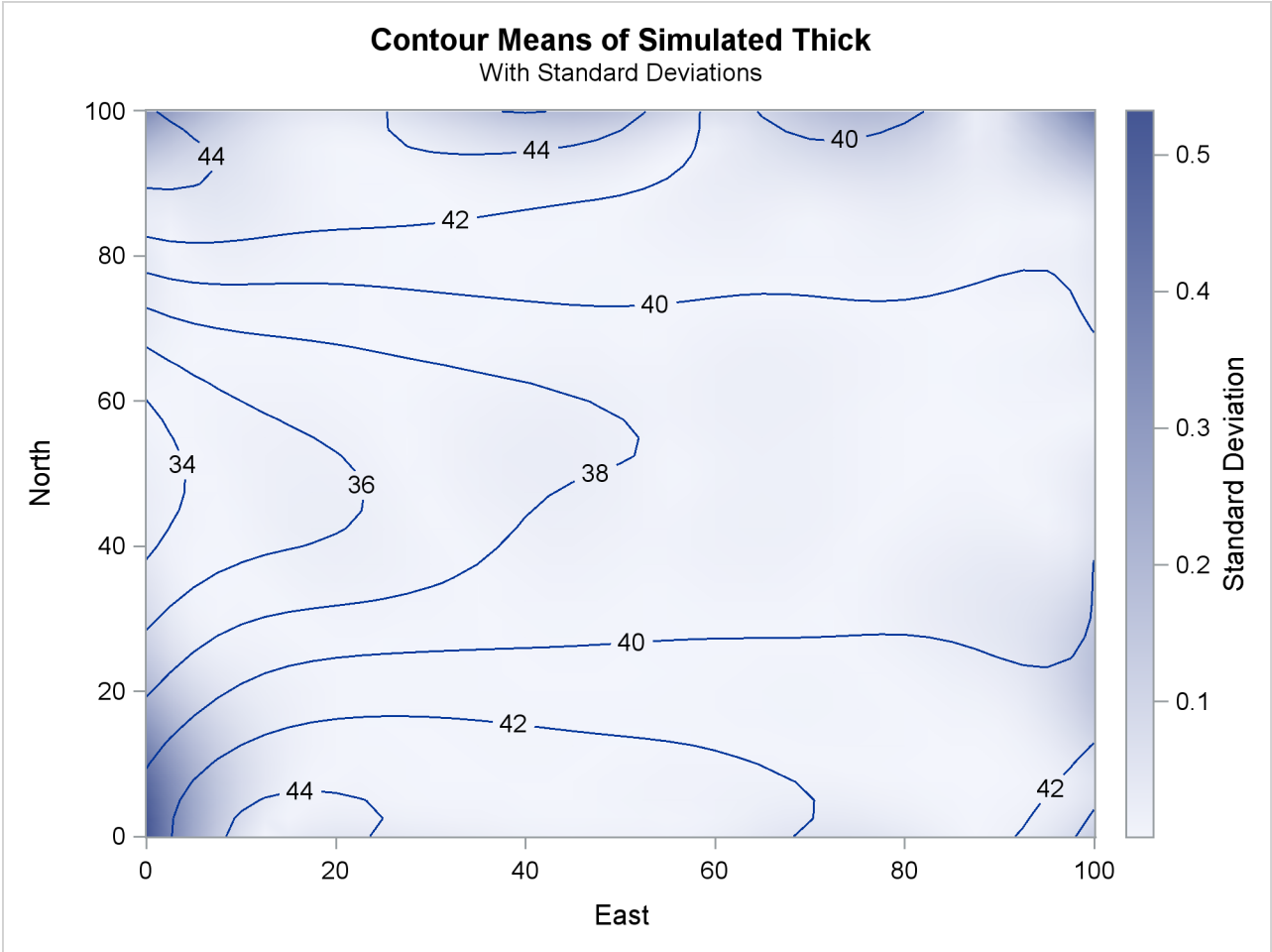
Figure 89.5 Contour Plot of Conditionally Simulated Coal Seam Thickness
