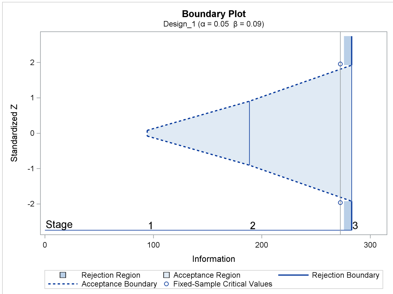
Output 87.10.4 Boundary Plot
