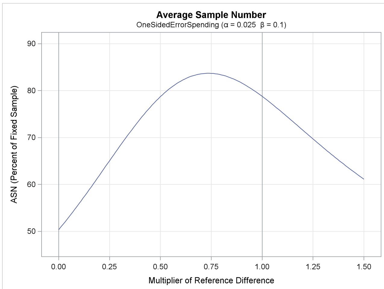
Output 87.8.5 ASN Plot
