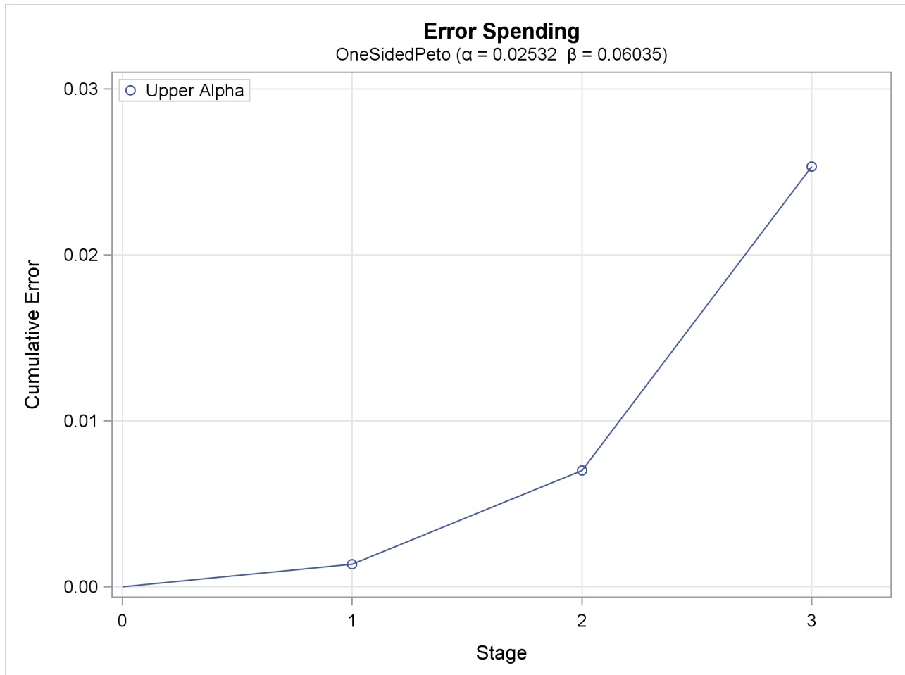
Output 87.5.14 Error Spending Plot
