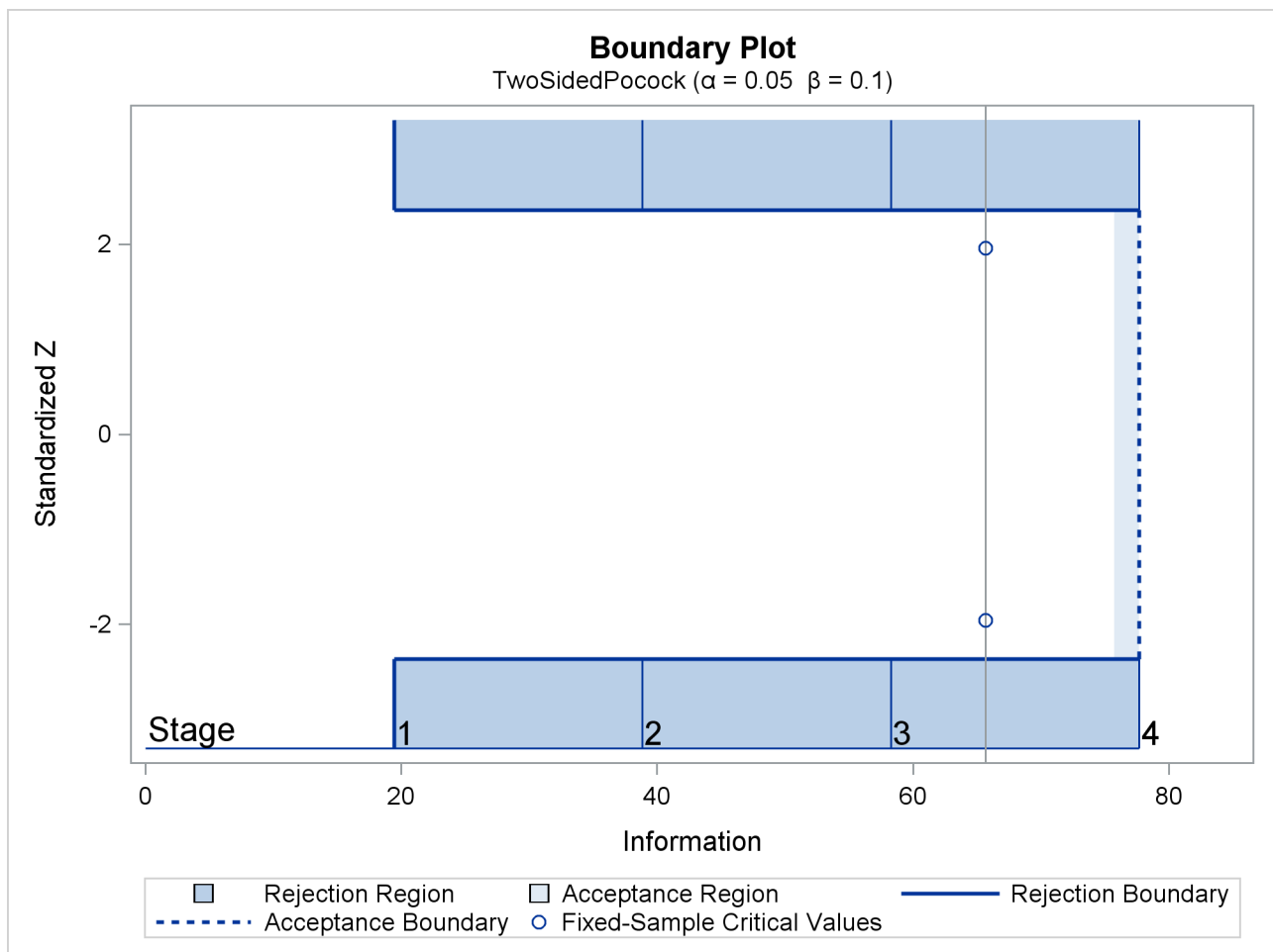
Output 87.4.1 Pocock Boundary Plot
