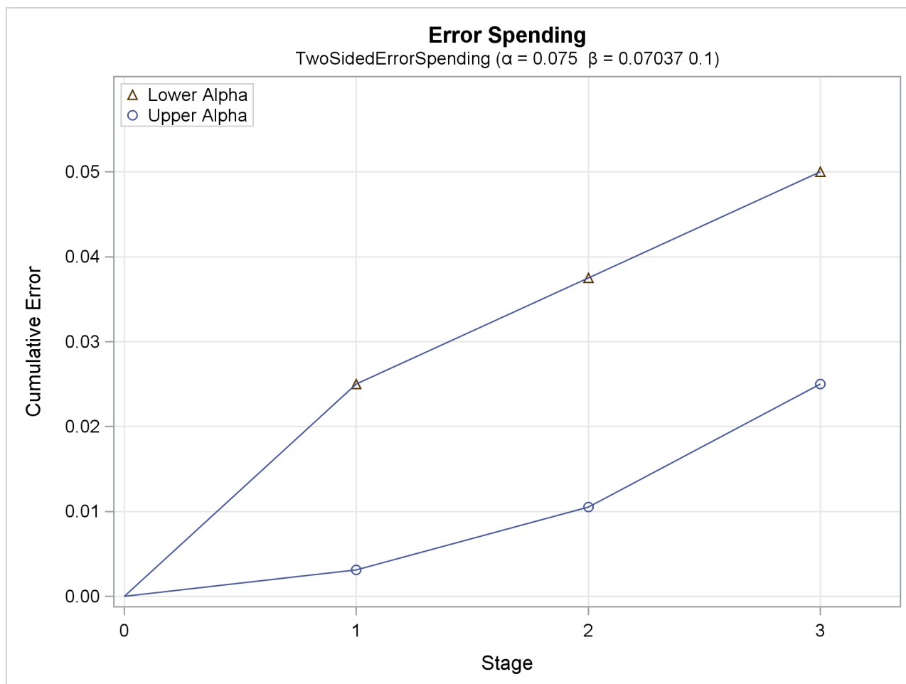
Output 87.11.10 Error Spending Plot
