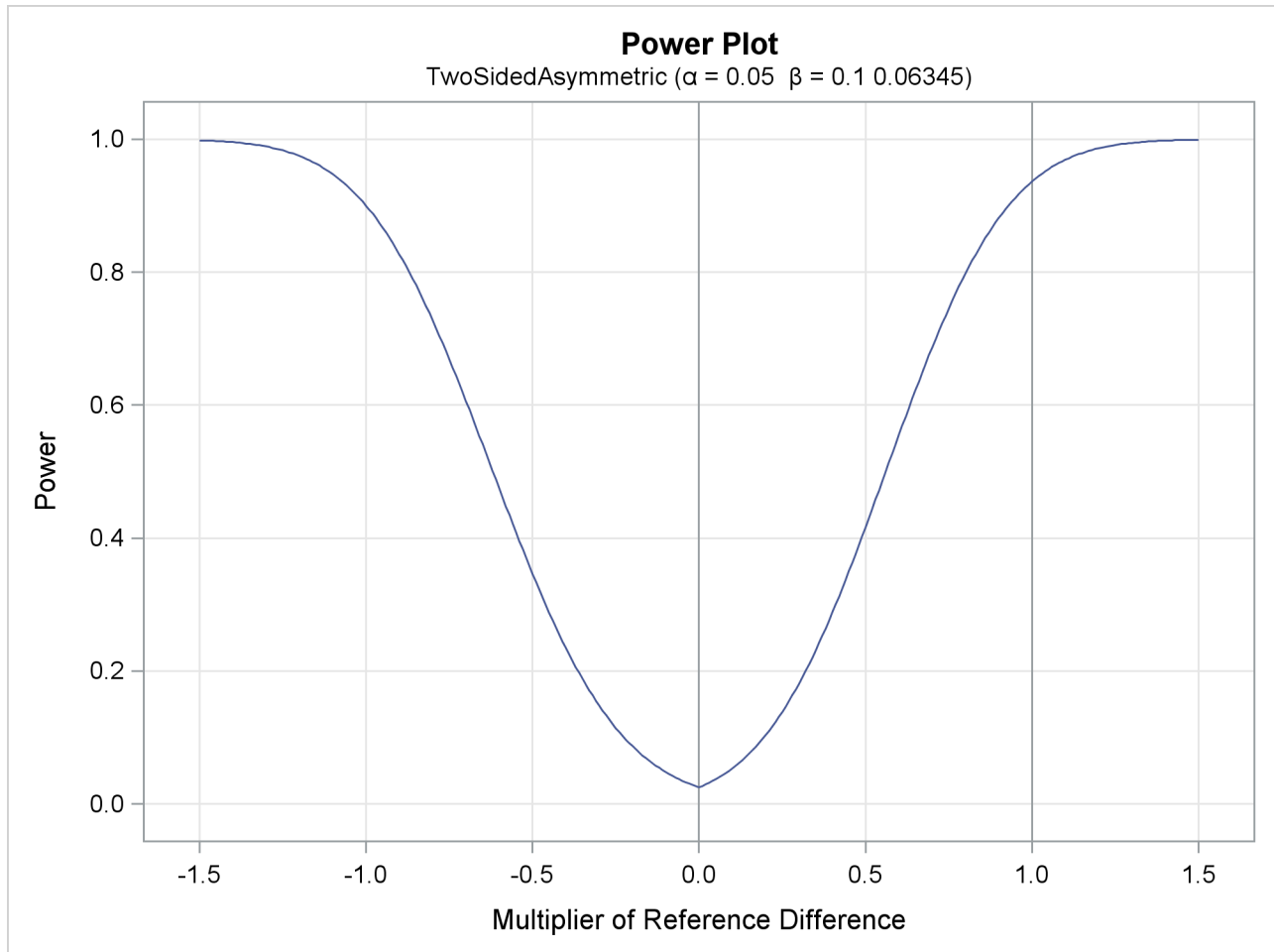
Output 87.12.5 Power Plot
