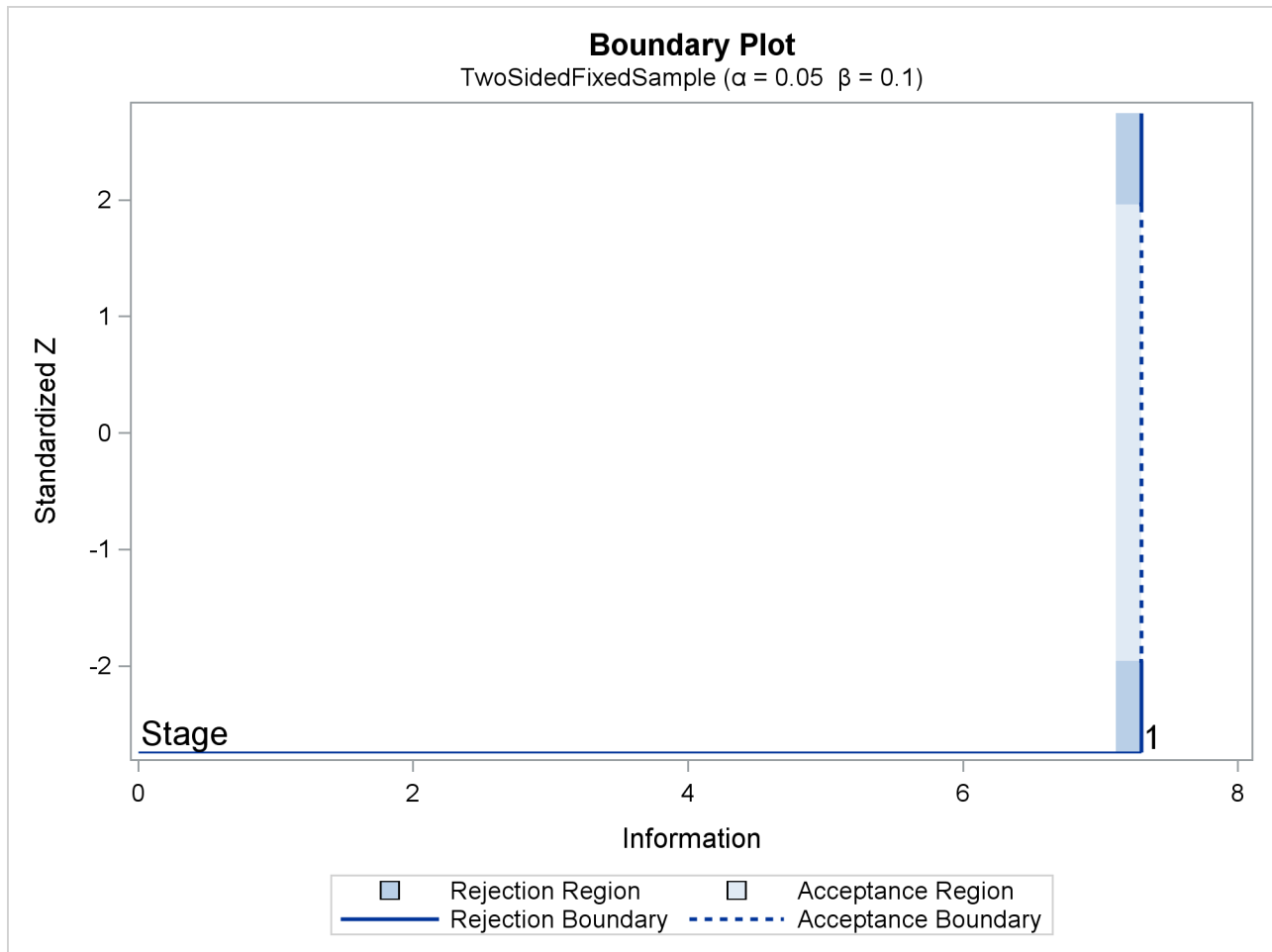
Output 87.1.10 Boundary Plot
