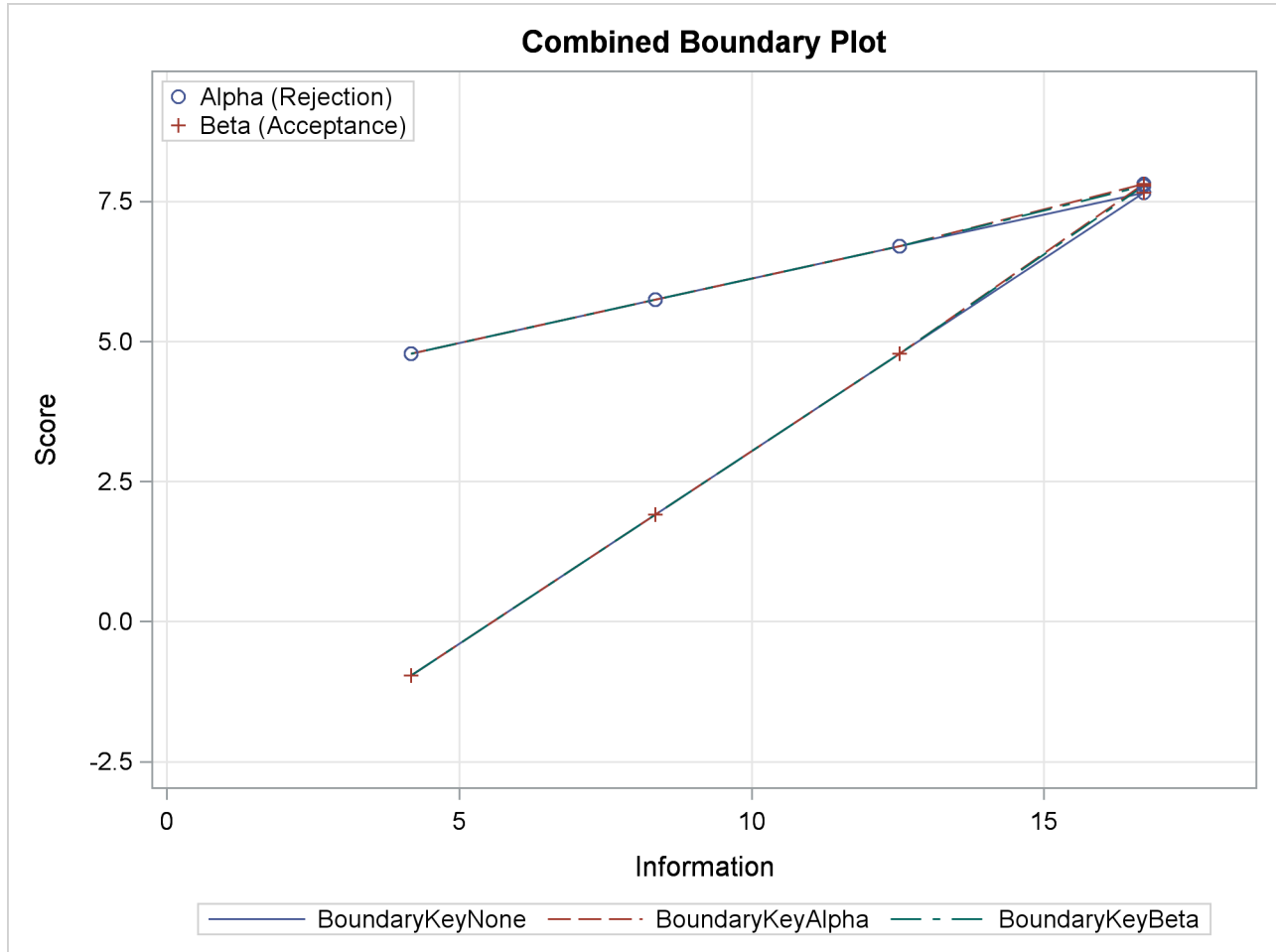
Output 87.7.13 Combined Boundary Plot
