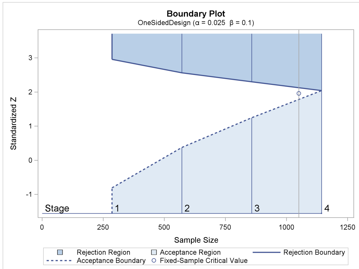
Figure 87.10 Boundary Plot for One-Sided Test
