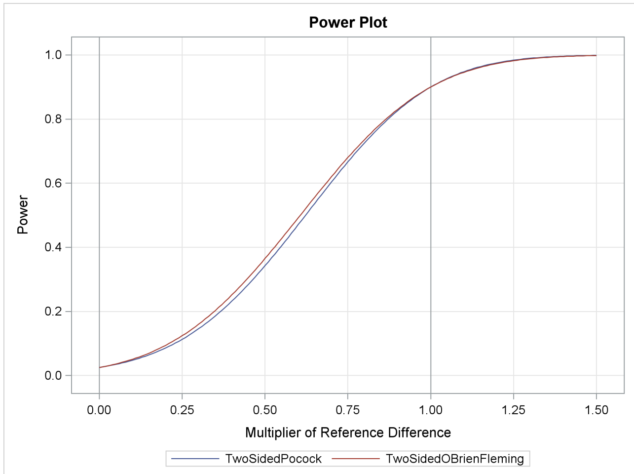
Output 87.4.4 Power Plot
