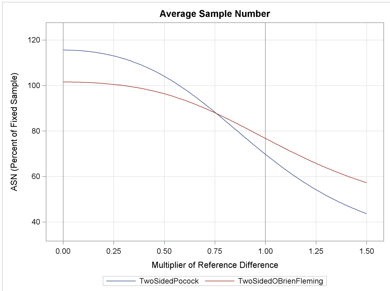
Output 87.4.3 ASN Plot
