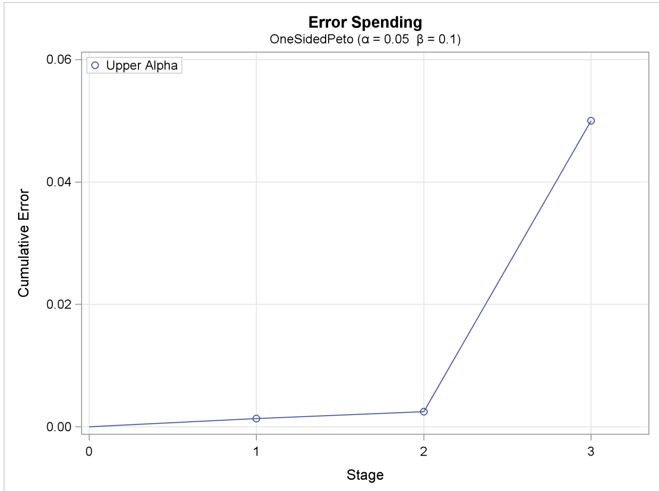
Output 87.5.7 Error Spending Plot
