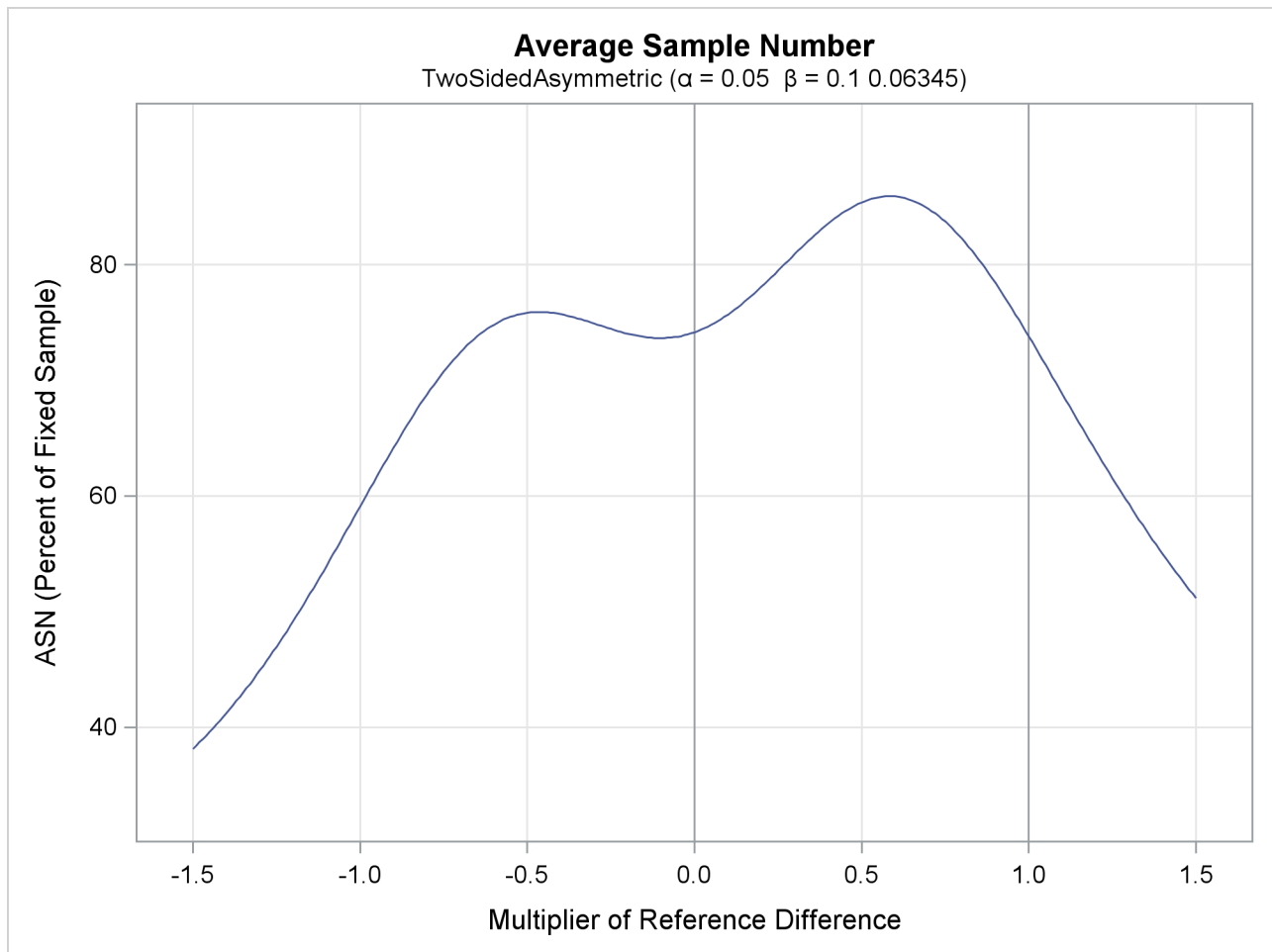
Output 87.12.6 ASN Plot
