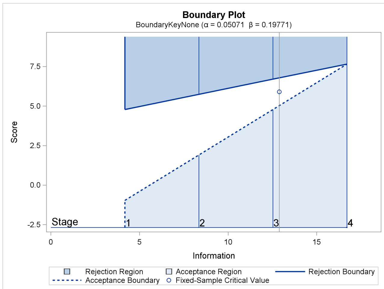
Output 87.7.4 Boundary Plot
