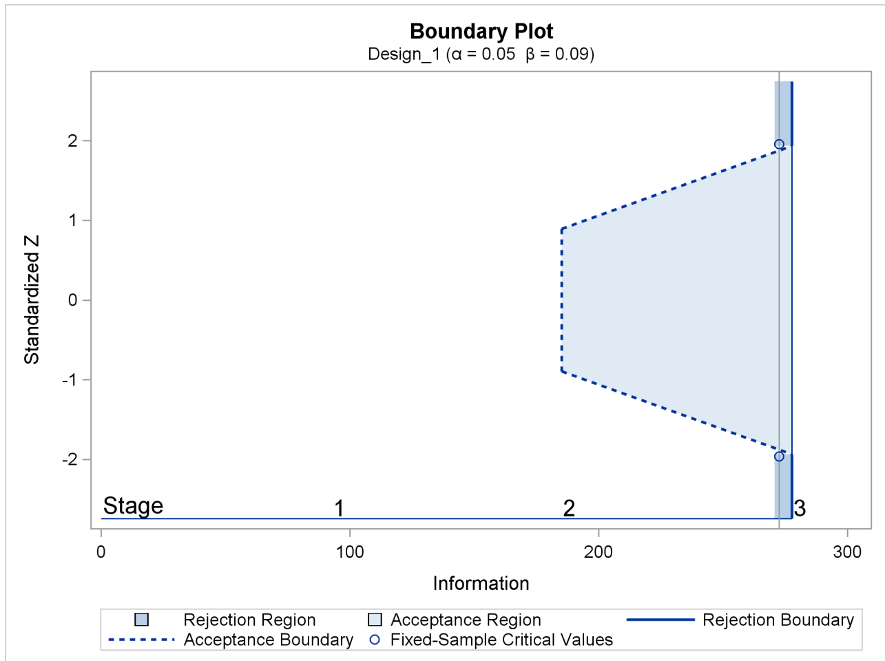
Output 87.10.8 Boundary Plot
