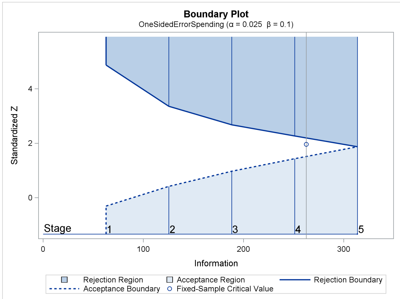
Output 87.8.8 Boundary Plot
