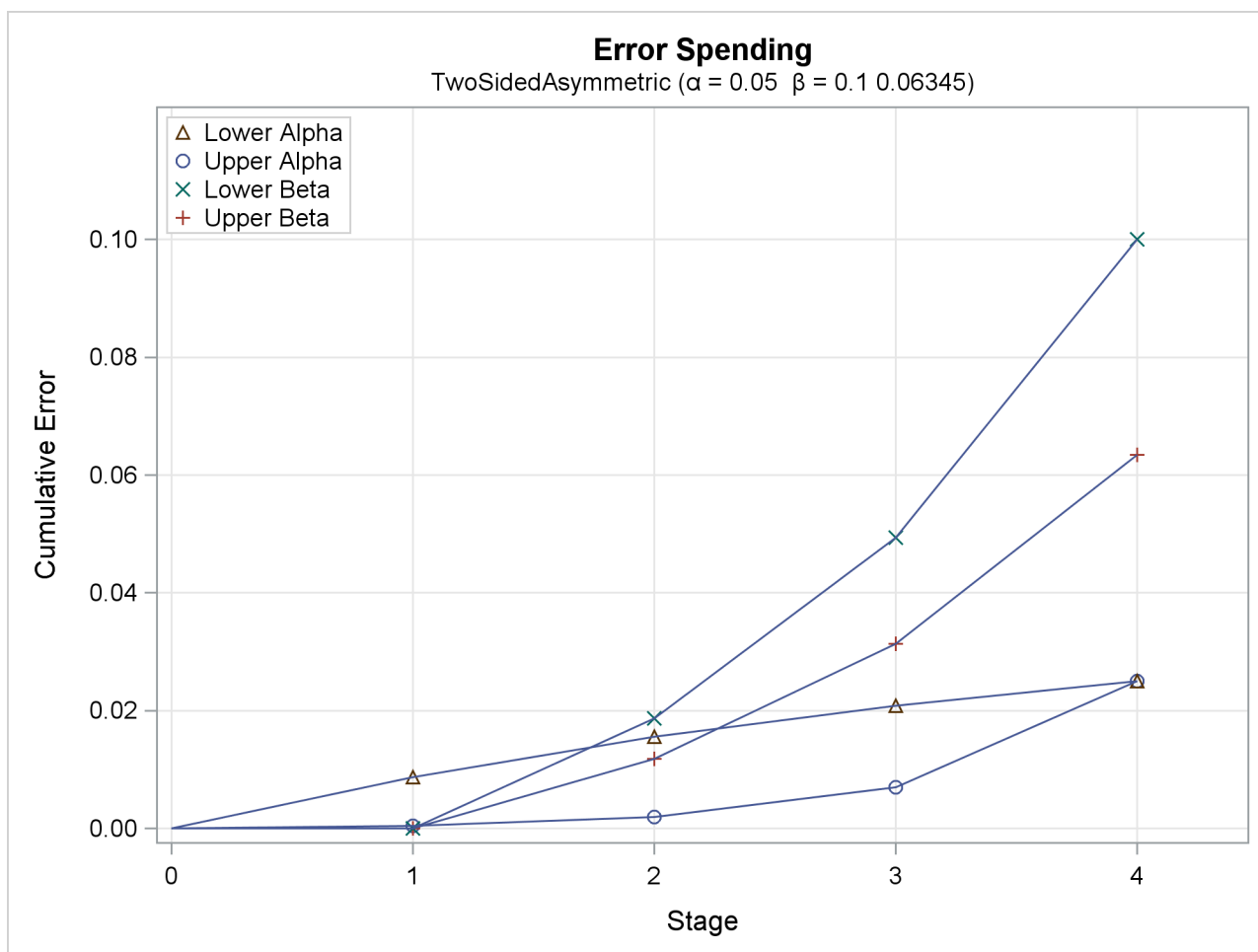
Output 87.12.10 Error Spending Plot
