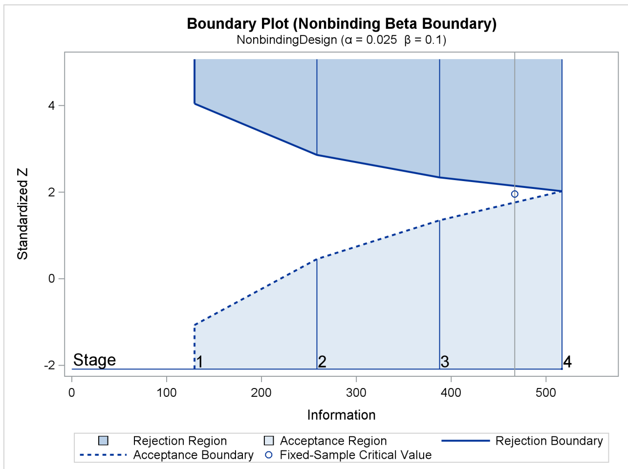
Output 87.13.4 Boundary Plot
