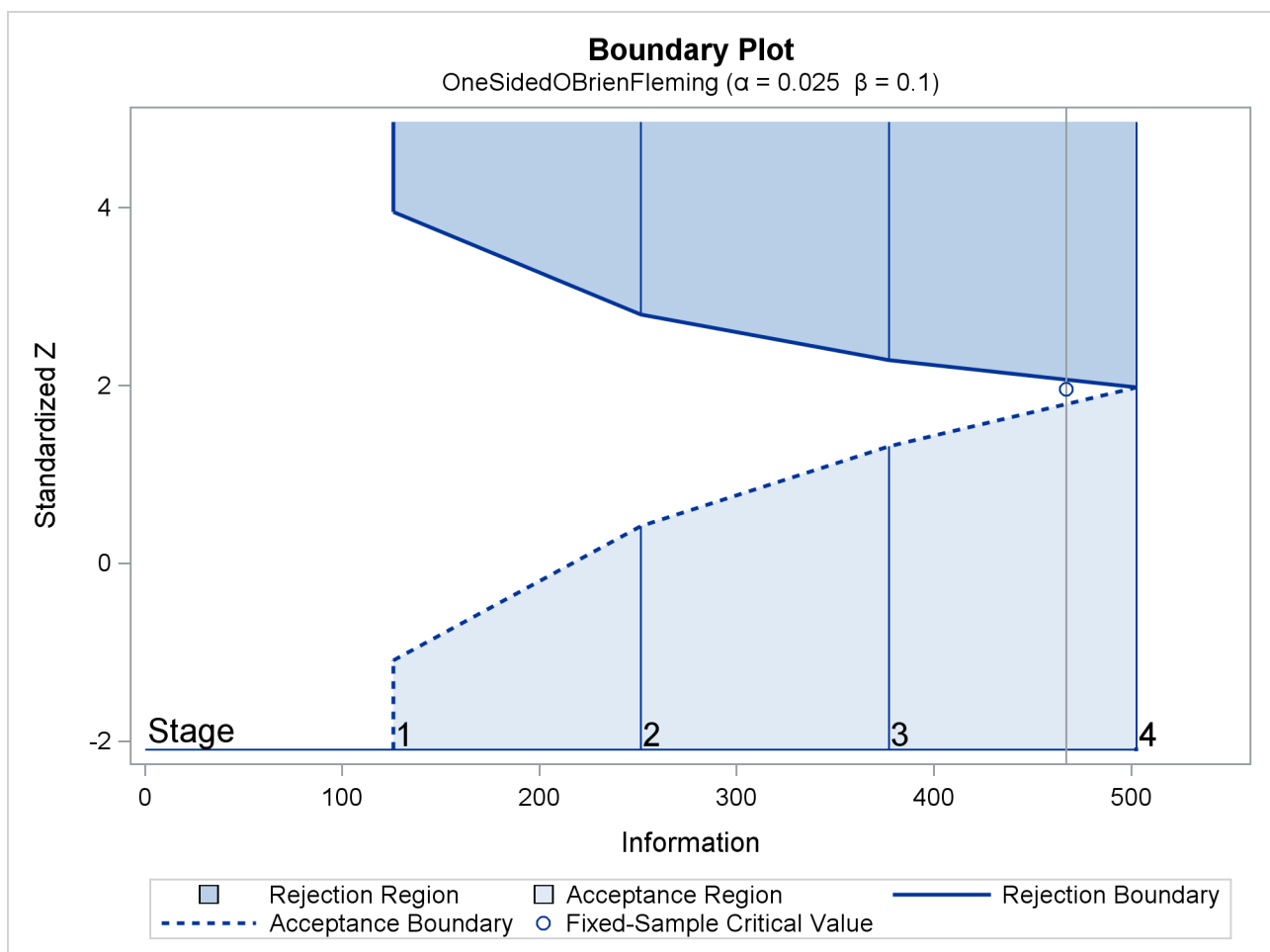
Output 87.2.4 Boundary Plot
