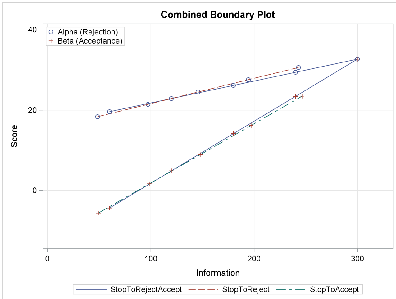
Output 87.6.16 Combined Boundary Plot with Score Scale
