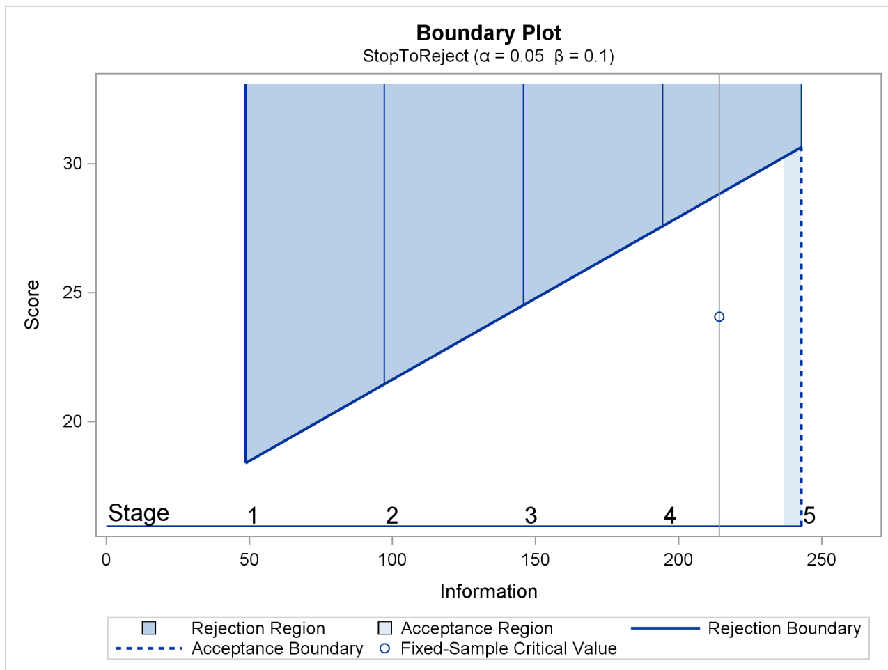
Output 87.6.10 Boundary Plot with Score Statistics
