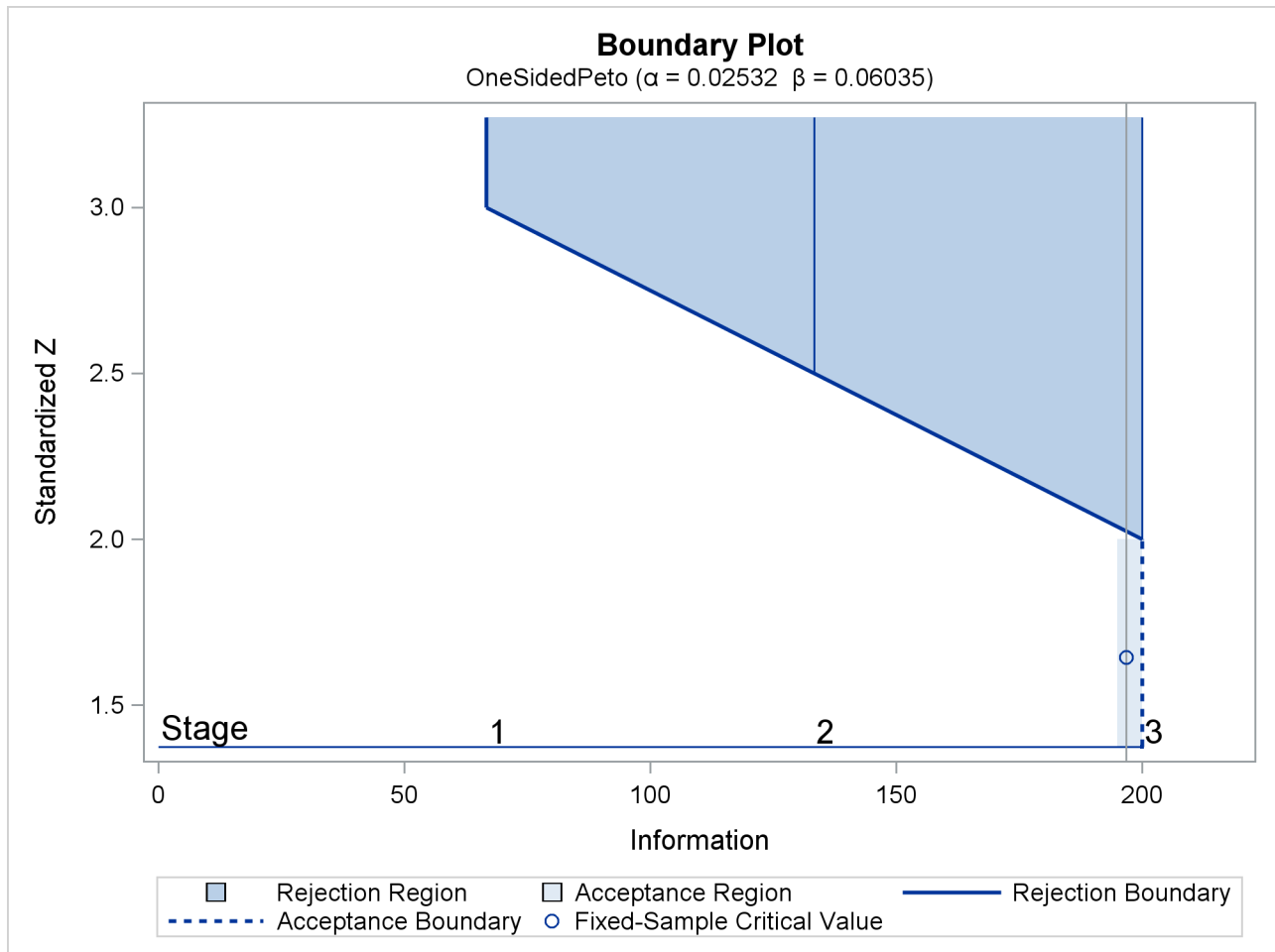
Output 87.5.13 Boundary Plot
