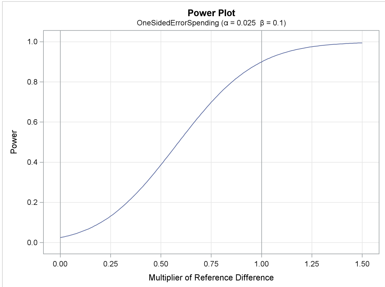
Output 87.8.6 Power Plot
