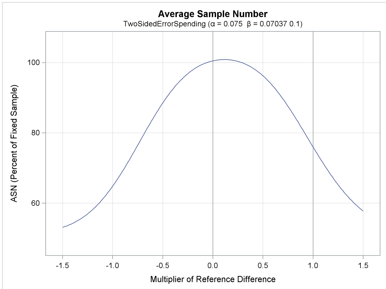
Output 87.11.6 ASN Plot
