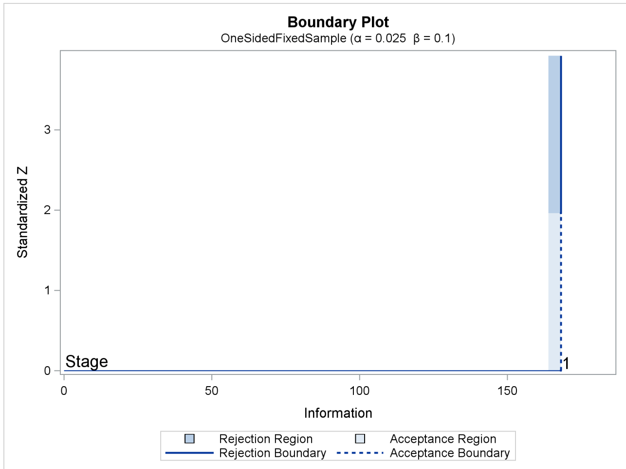
Output 87.1.4 Boundary Plot
