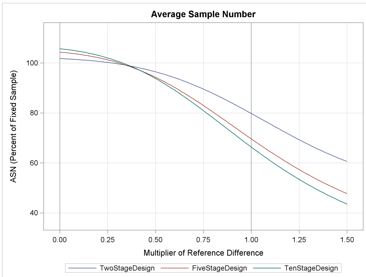
Output 87.9.7 ASN Plot
