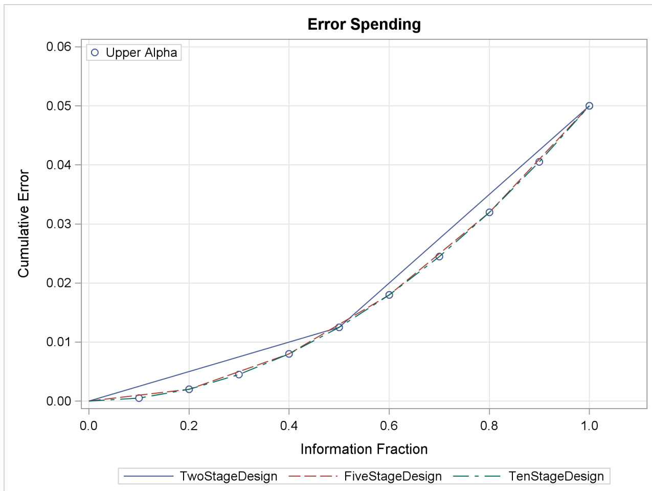
Output 87.9.10 Error Spending Plot
