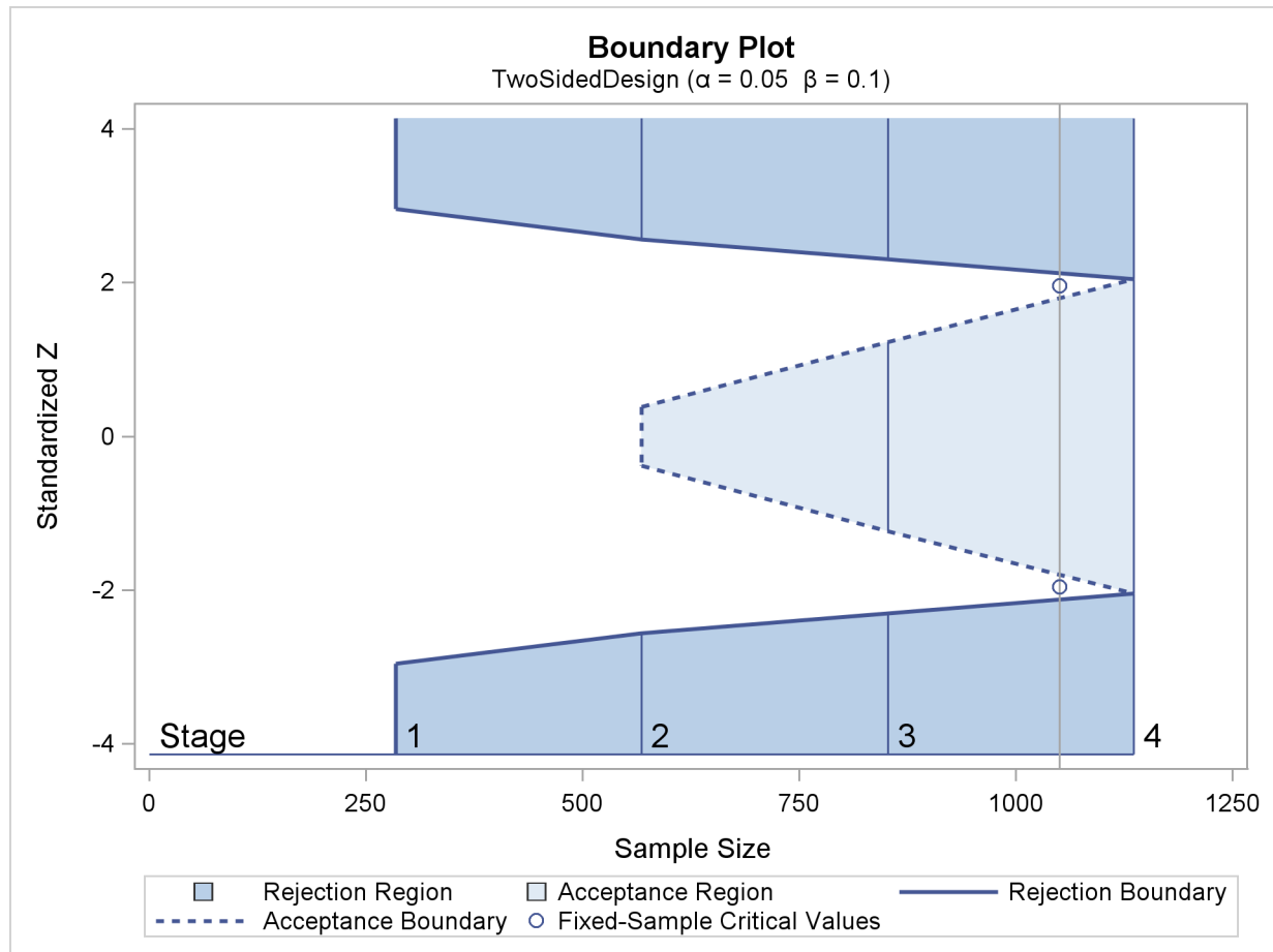
Figure 87.11 Boundary Plot for Two-Sided Test
