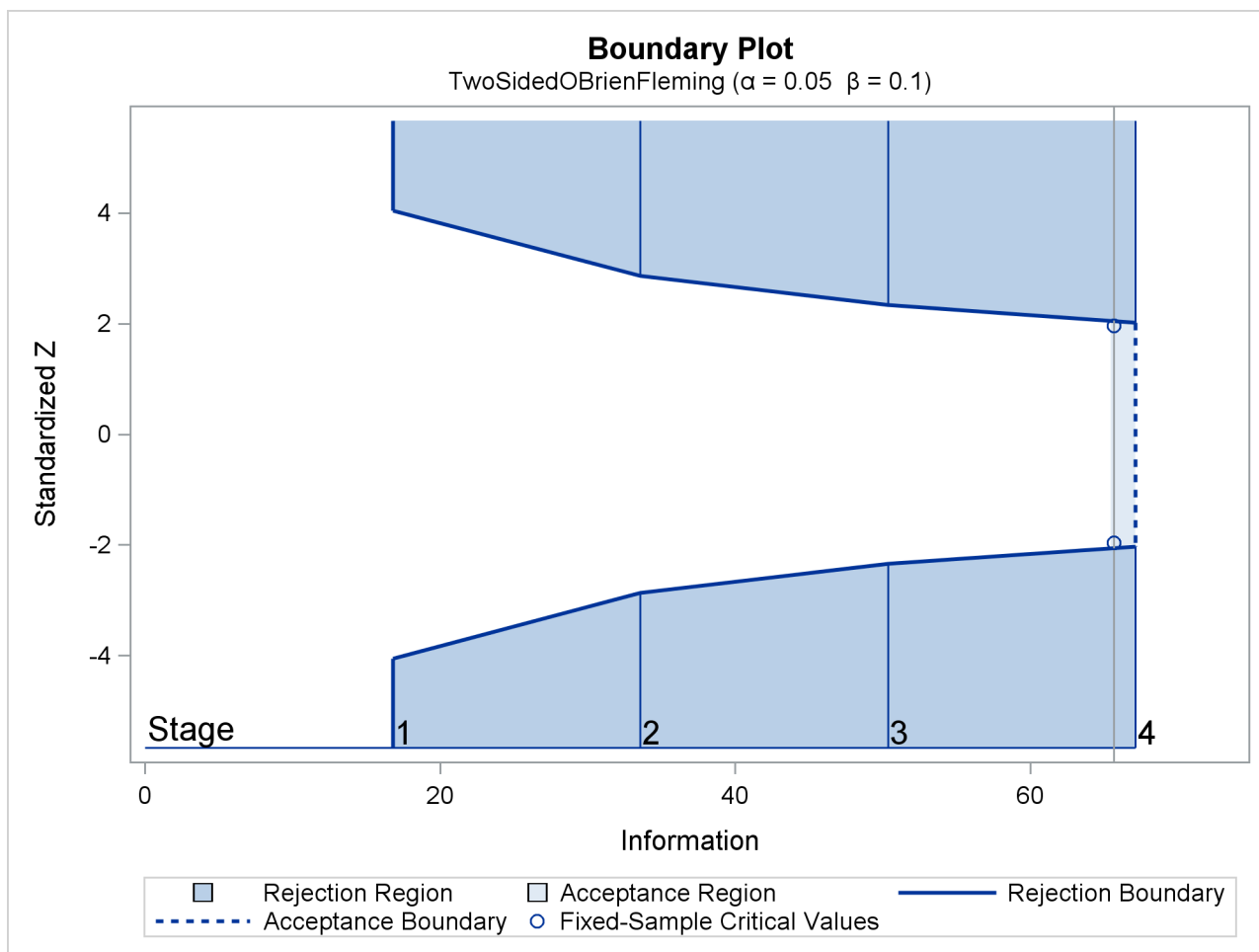
Output 87.4.2 O'Brien-Fleming Boundary Plot
