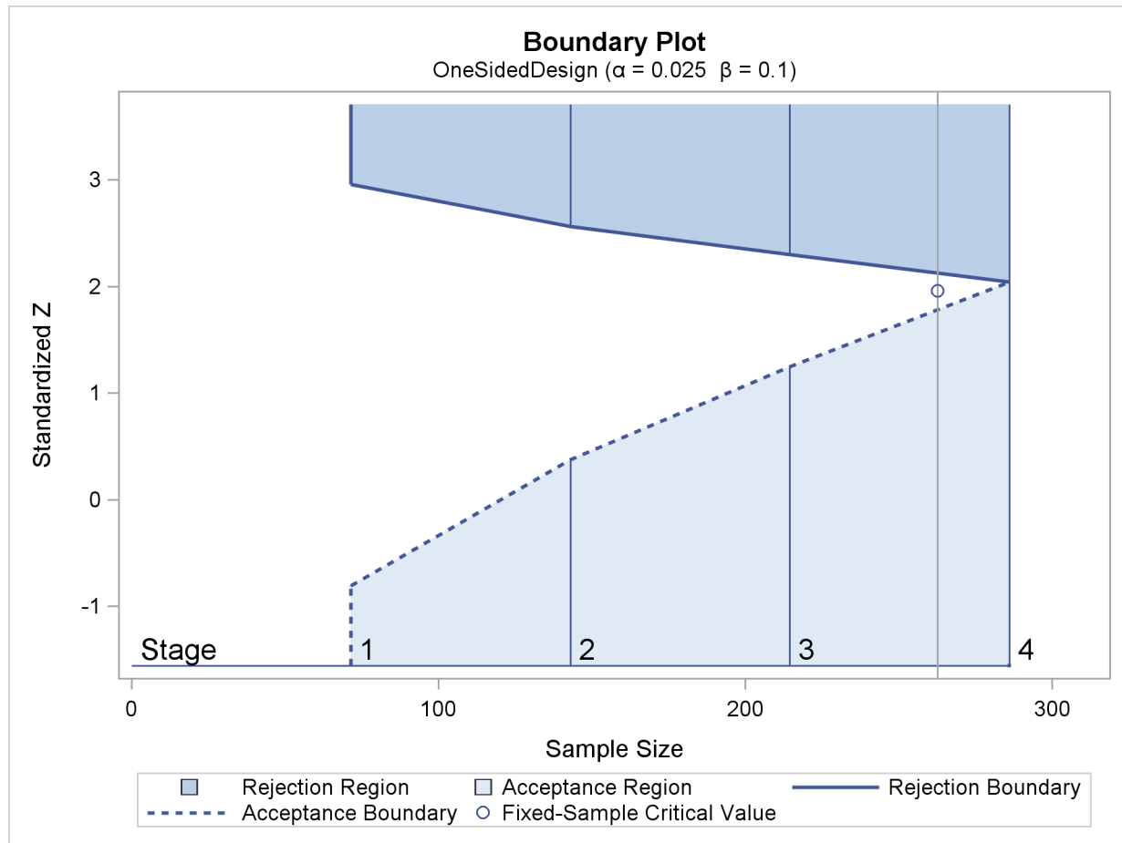
Figure 87.3 Boundary Plot for One-Sided Design
