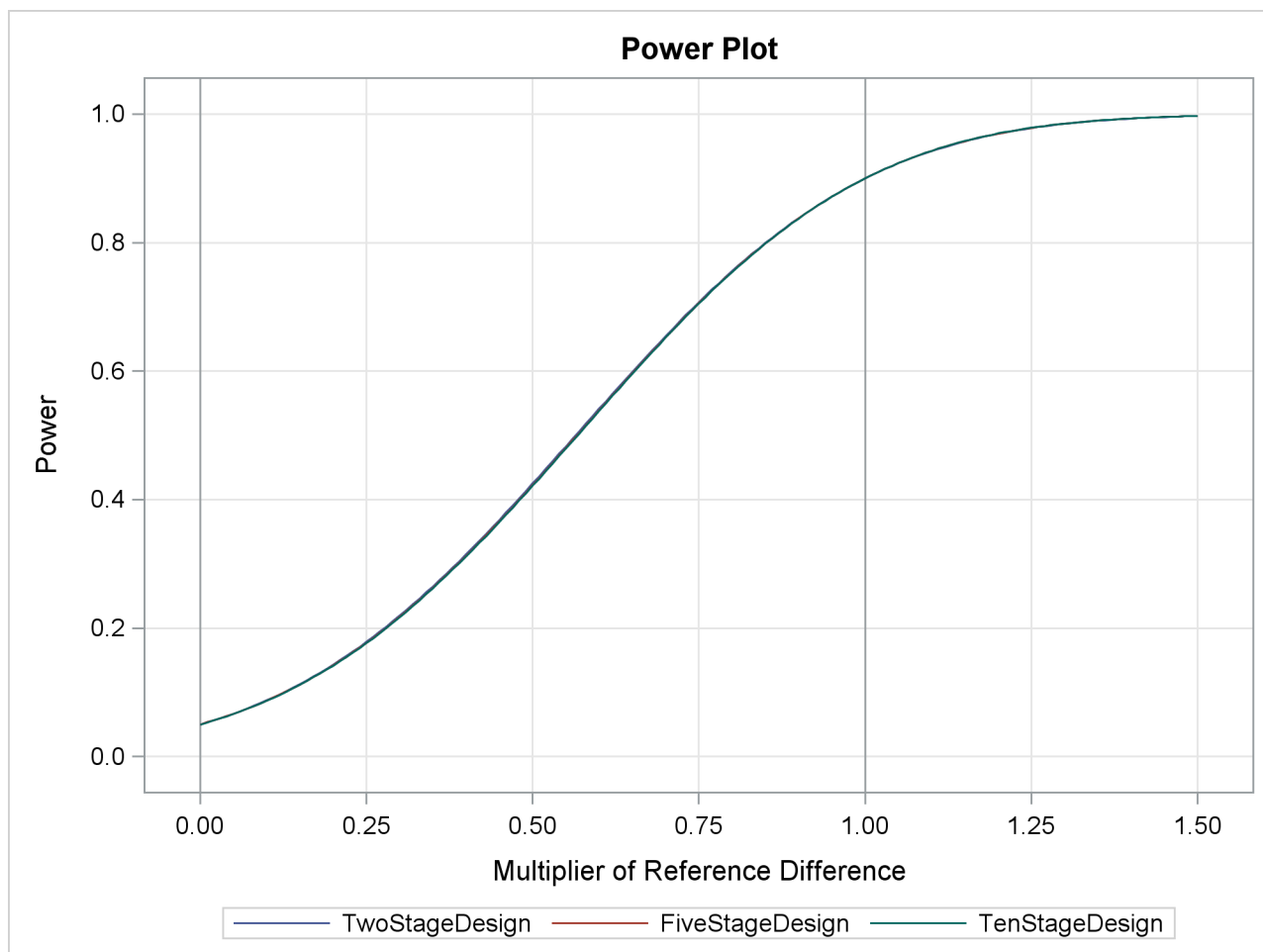
Output 87.9.8 Power Plot
