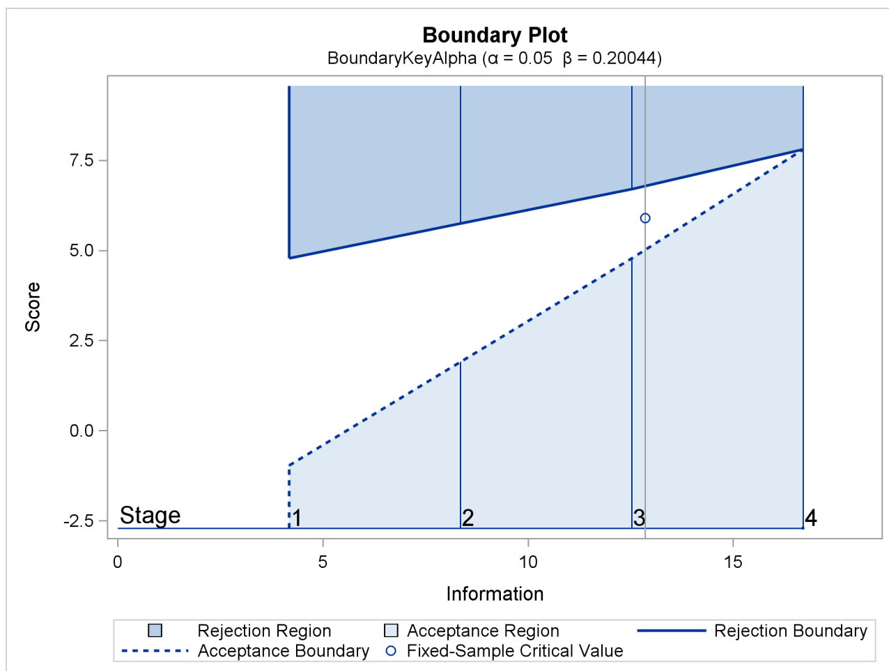
Output 87.7.8 Boundary Plot
