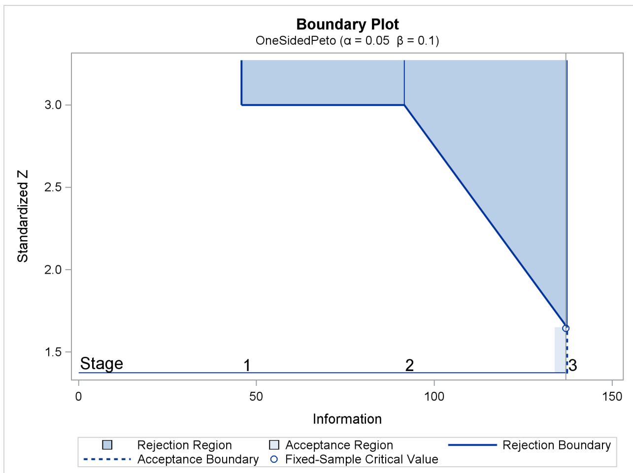
Output 87.5.6 Boundary Plot
