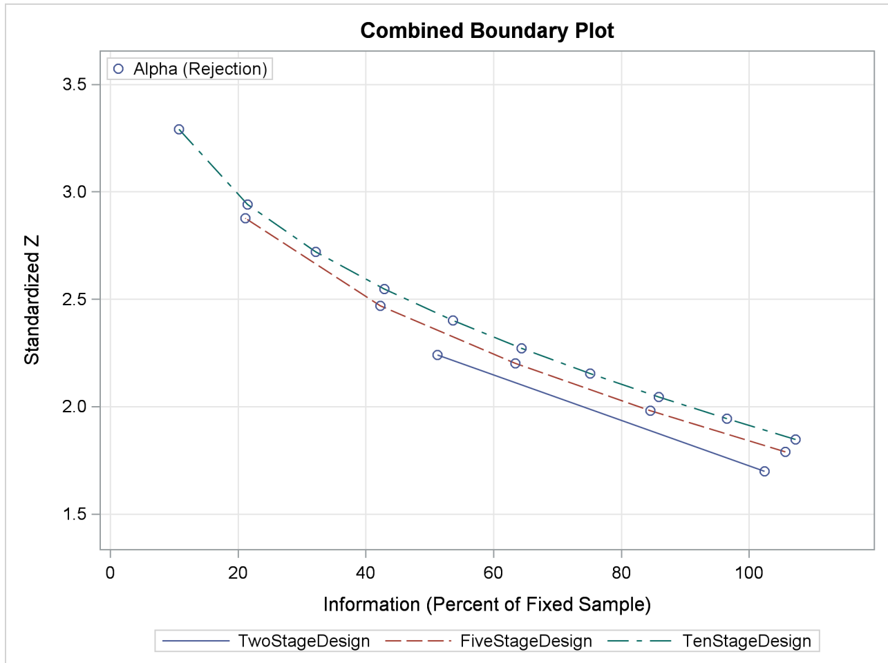
Output 87.9.9 Combined Boundary Plot
