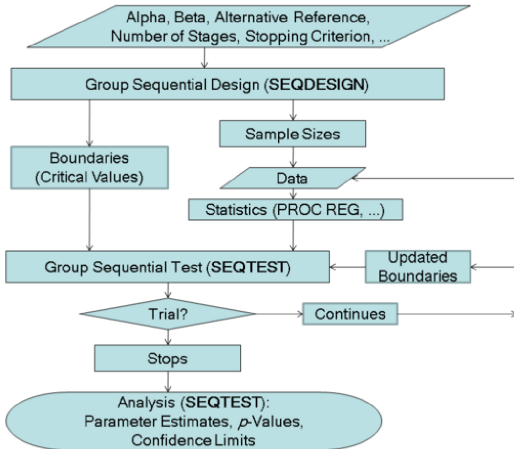
Figure 87.2 Group Sequential Trial
