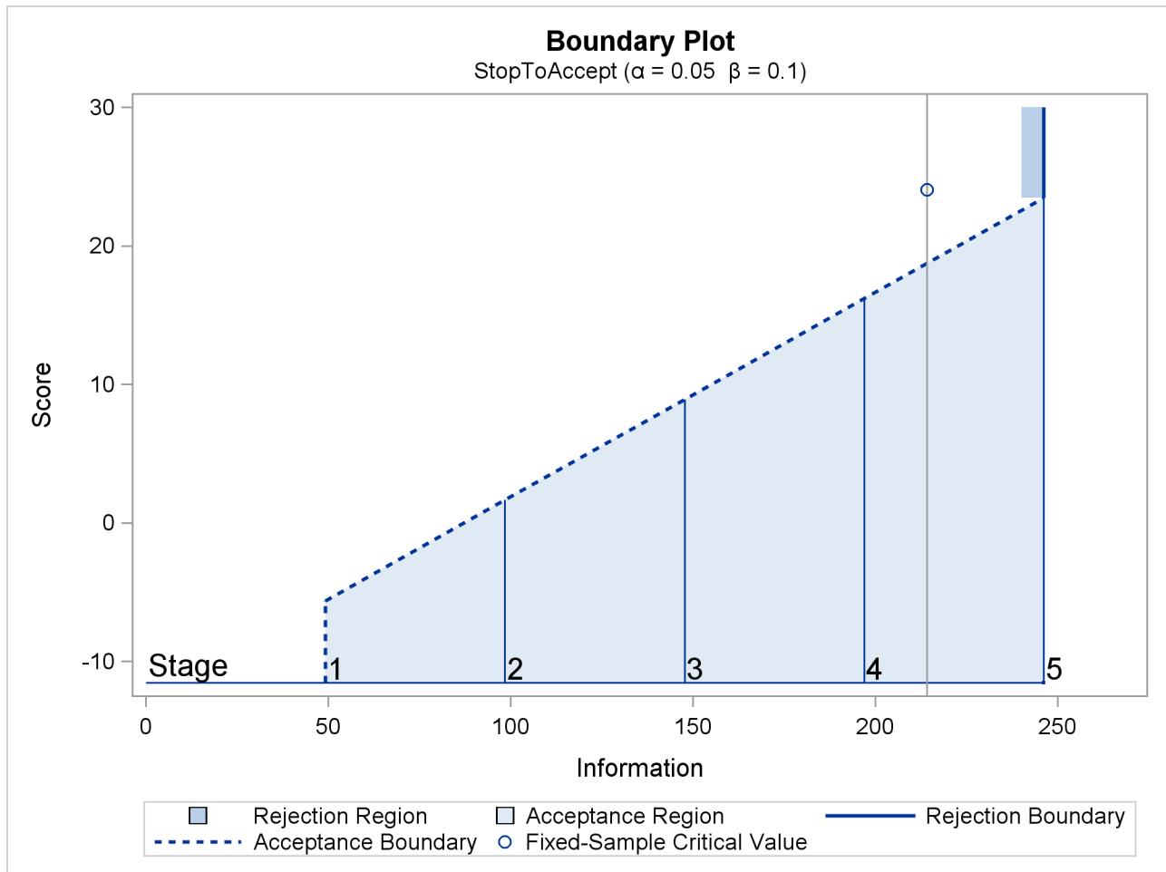
Output 87.6.15 Boundary Plot with Score Scale
