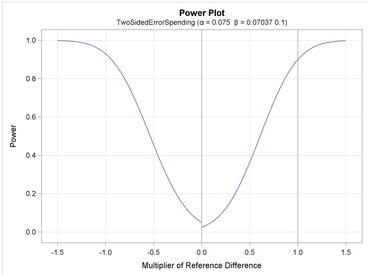
Output 87.11.5 Power Plot
