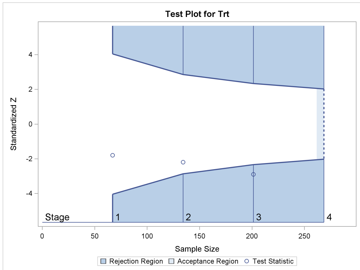
Figure 87.1 Sequential Plot for Two-Sided Test
