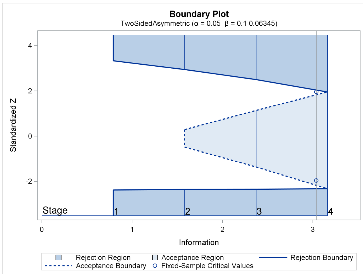
Output 87.12.8 Boundary Plot
