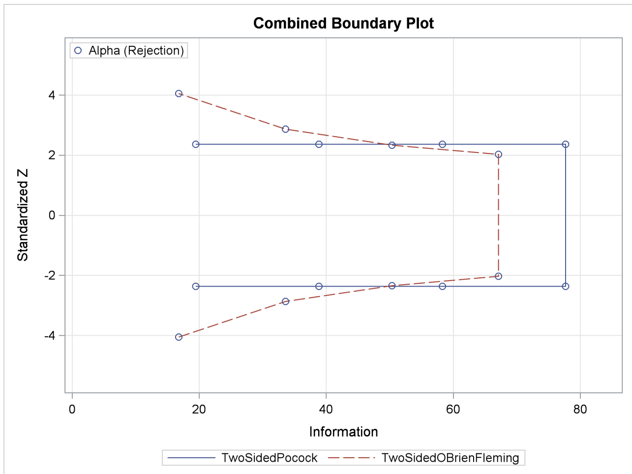
Output 87.4.5 Combined Boundary Plot
