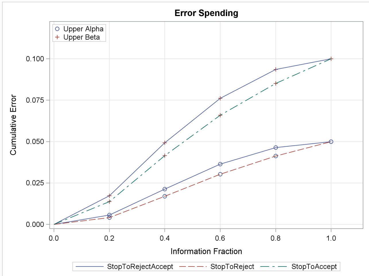
Output 87.6.17 Error Spending Plot
