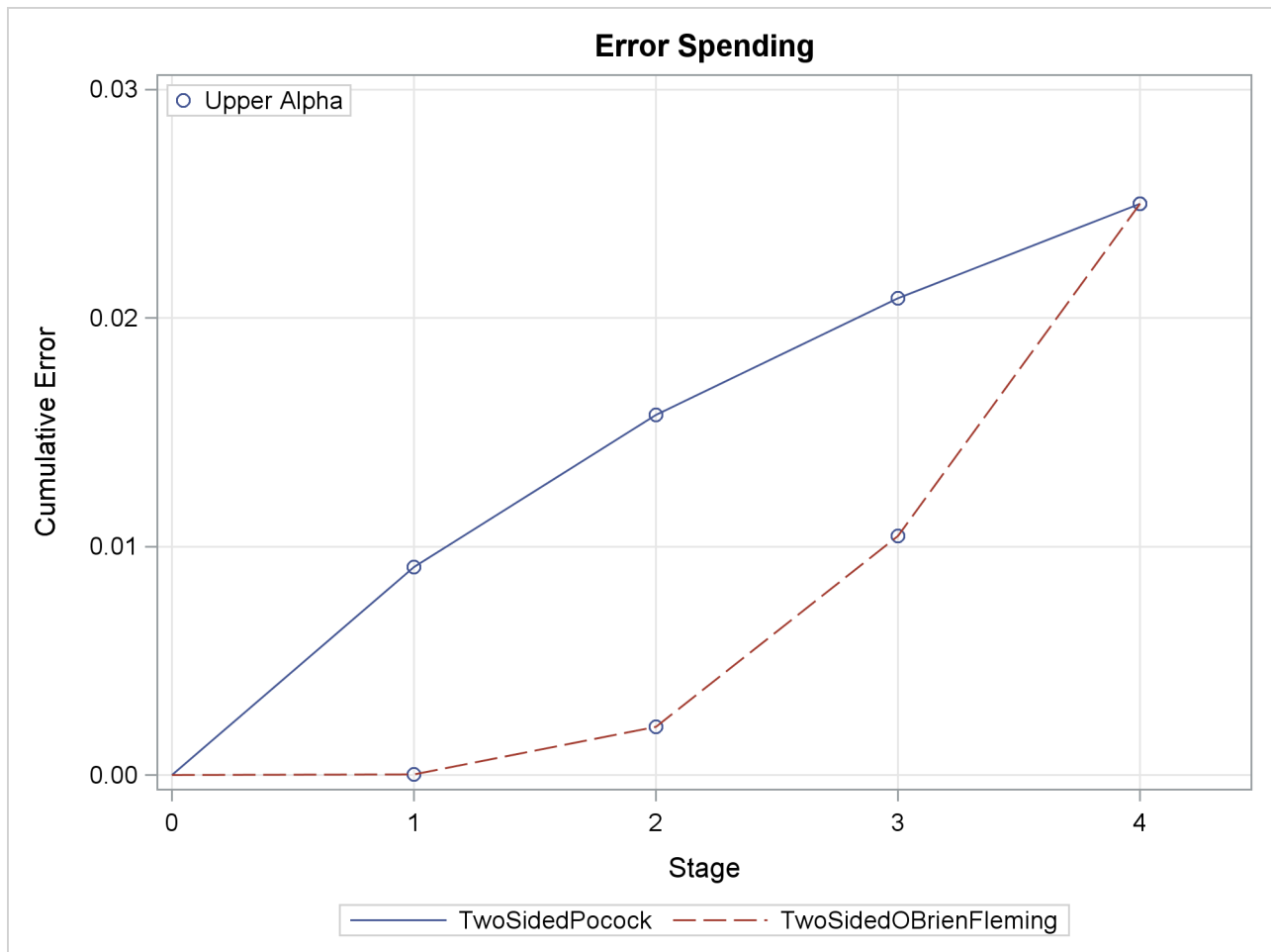
Output 87.4.6 Error Spending Plot
