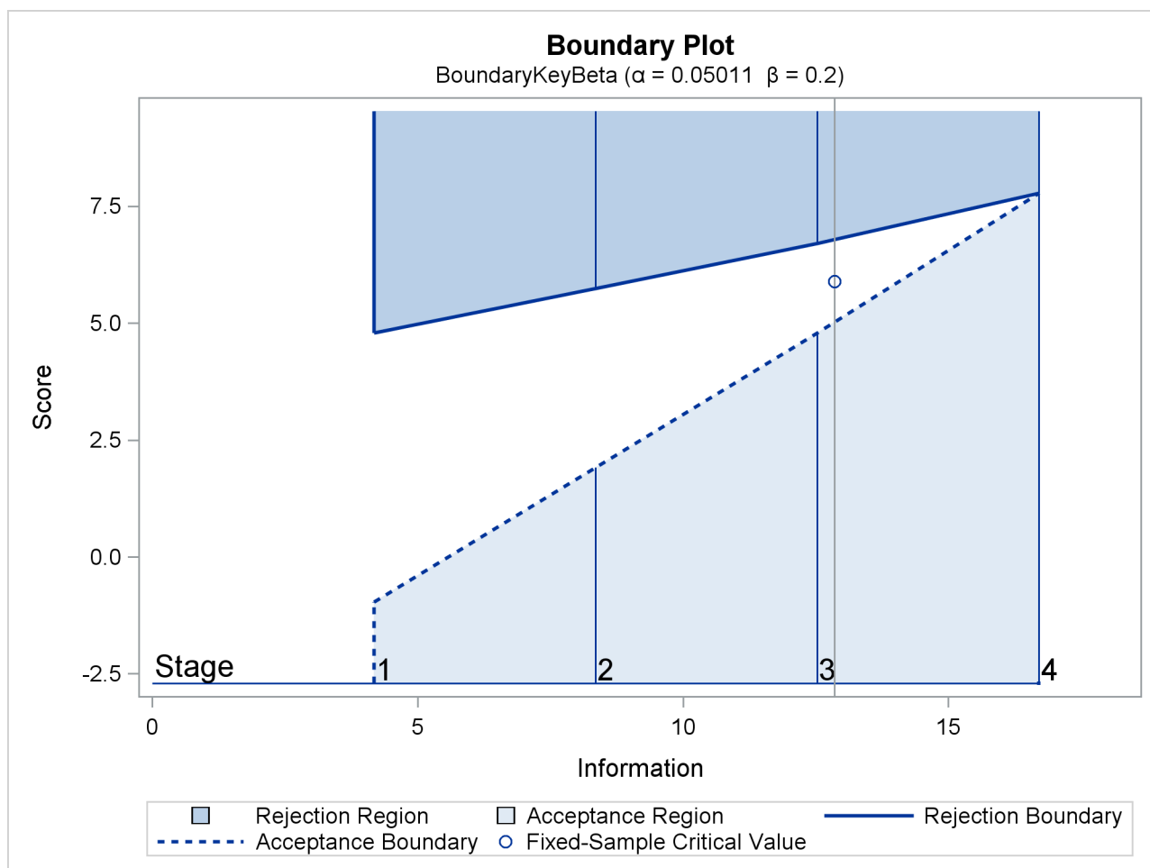
Output 87.7.12 Boundary Plot
