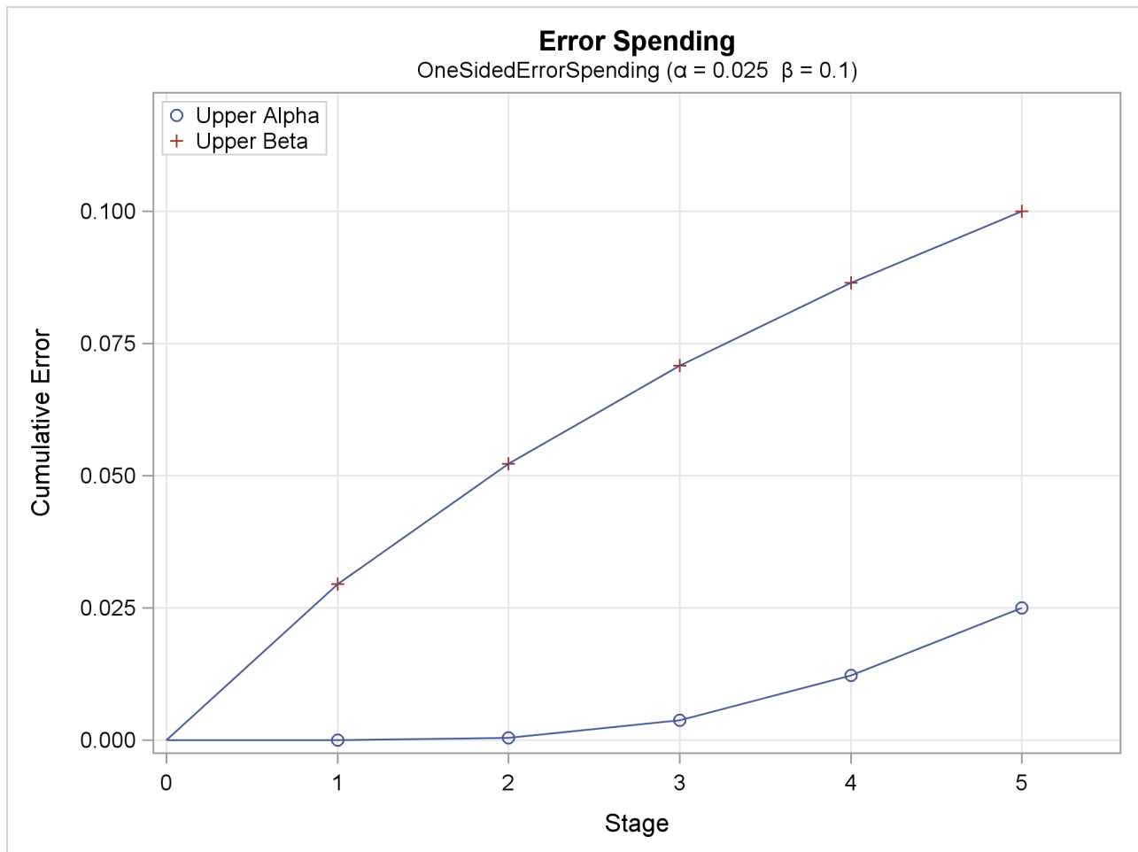
Output 87.8.10 Error Spending Plot
