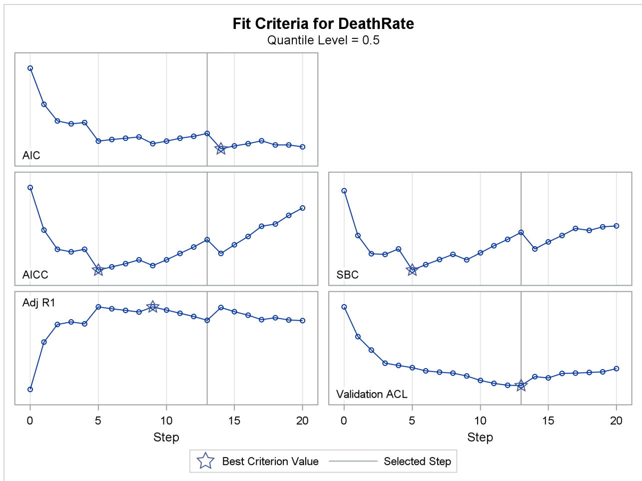
Output 82.3.5 Criterion Panel
