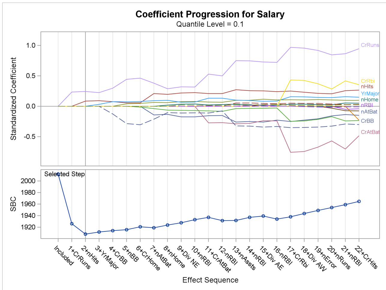
Figure 82.12 Coefficient Panel: \tau = 0.1
