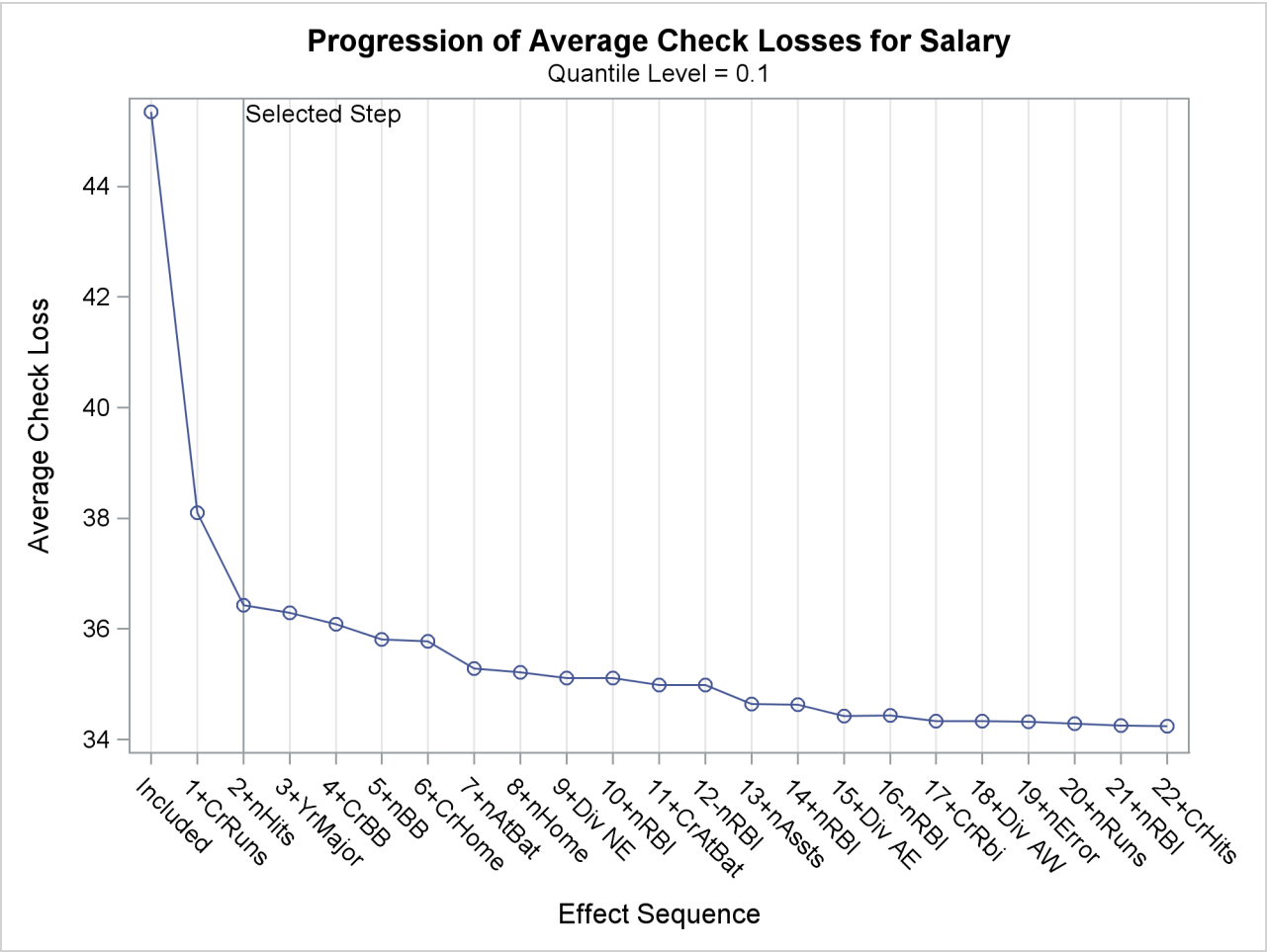
Figure 82.13 Average Check Loss Plot: \tau = 0.1
