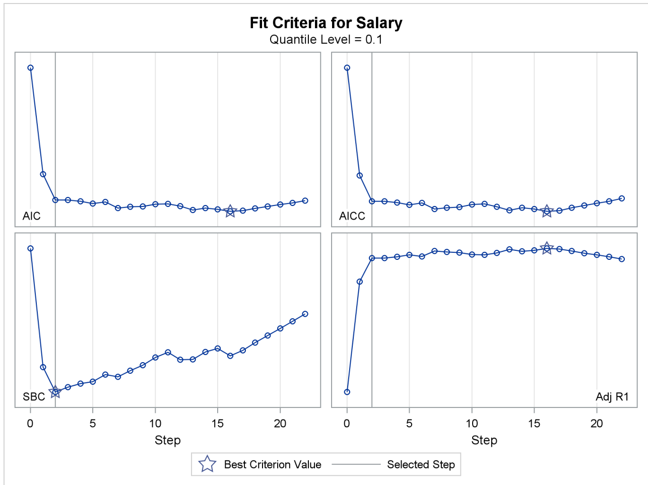
Figure 82.14 Criterion Panel: \tau = 0.1
