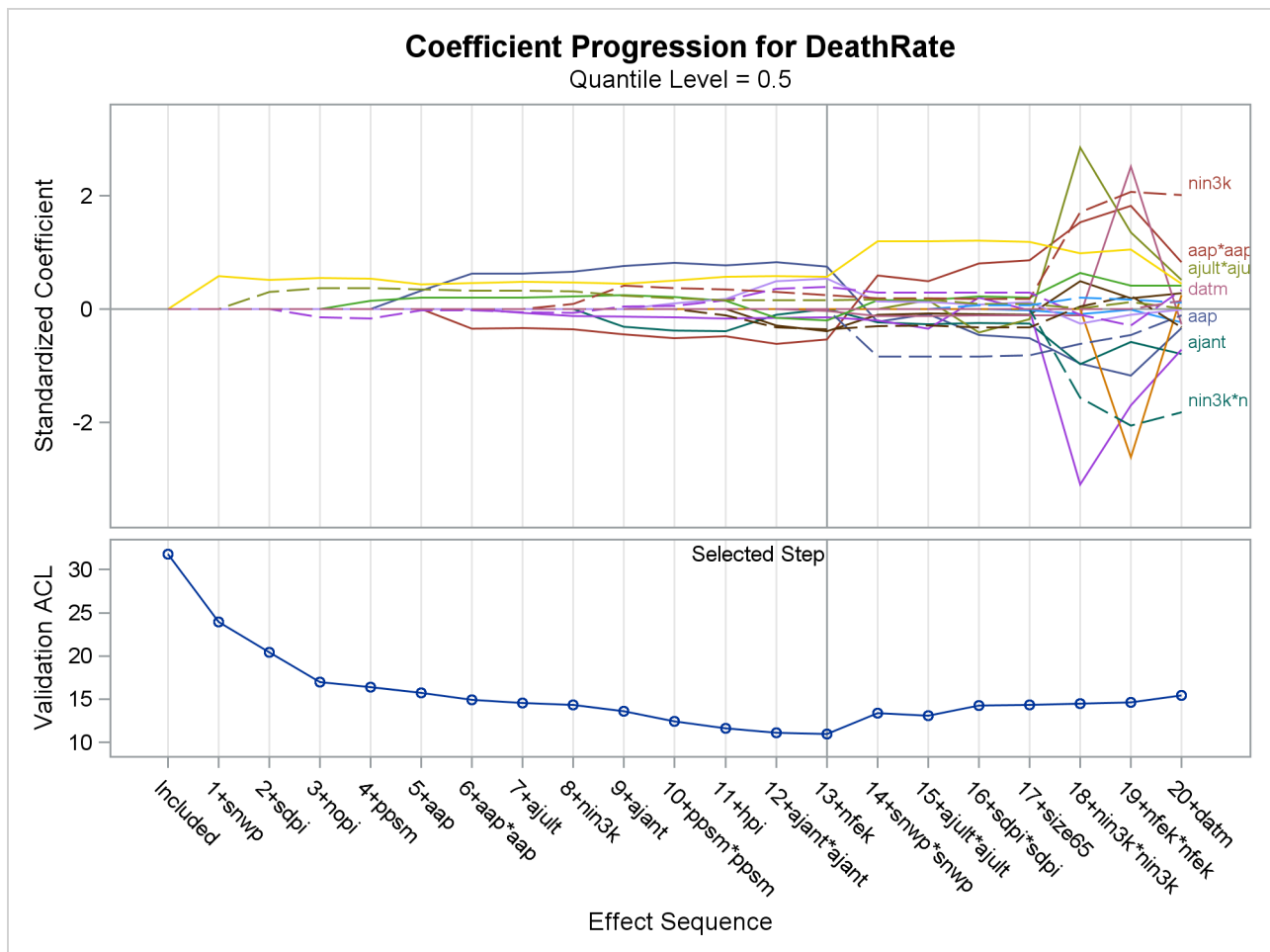
Output 82.3.3 Coefficient Panel
