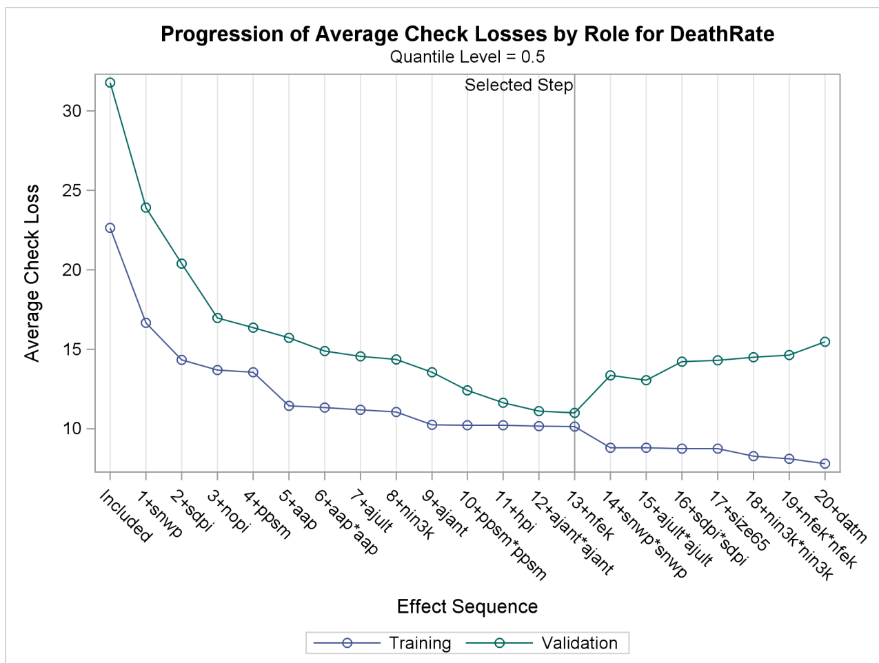
Output 82.3.4 Average Check Loss Plot
