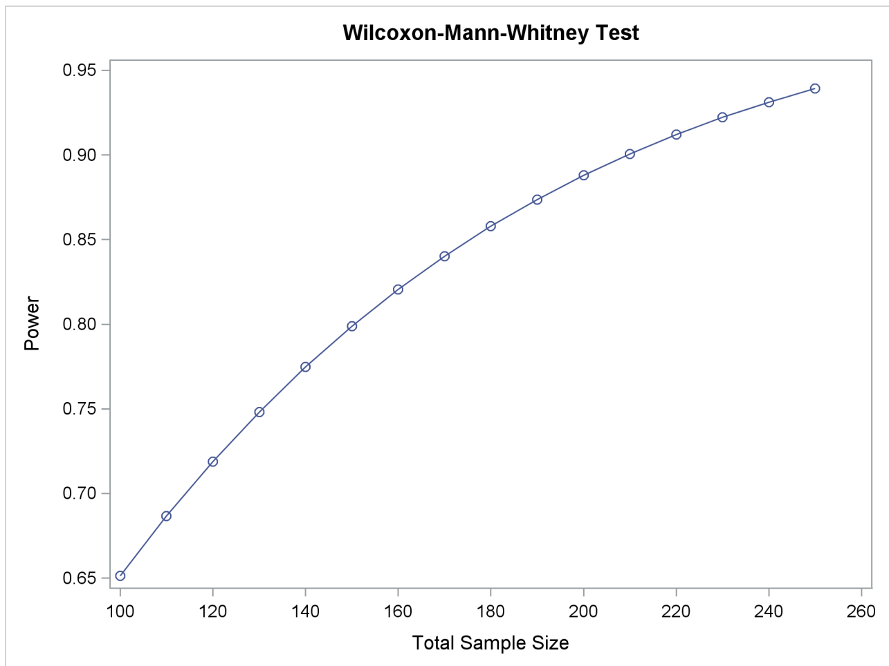
Output 75.10.2 Plot of Power versus Sample Size for Wilcoxon Power Analysis
