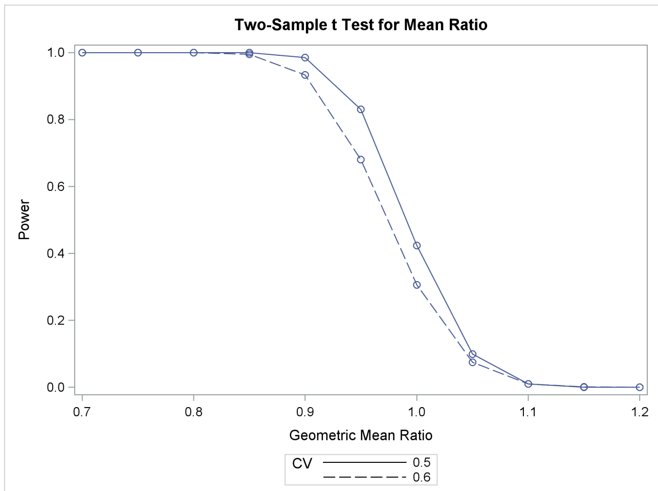
Output 75.4.2 Plot of Power versus Mean Ratio for Noninferiority Test
