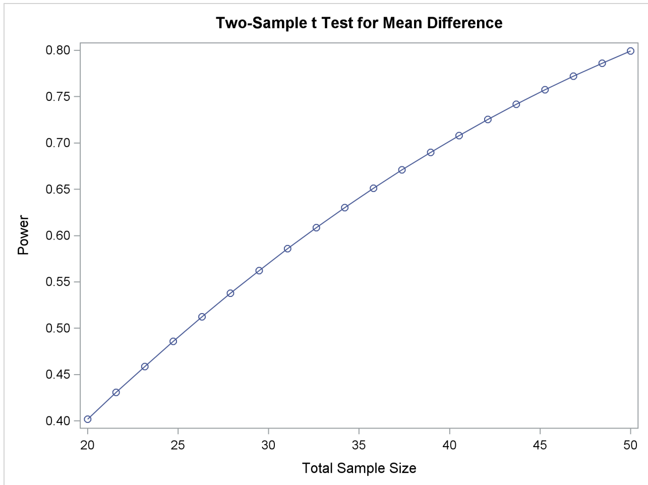
Output 75.8.10 Plot with Fractional Sample Sizes
