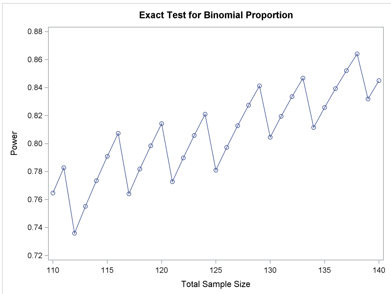
Output 75.2.6 Plot of Power versus Sample Size for Another One-sided Test
