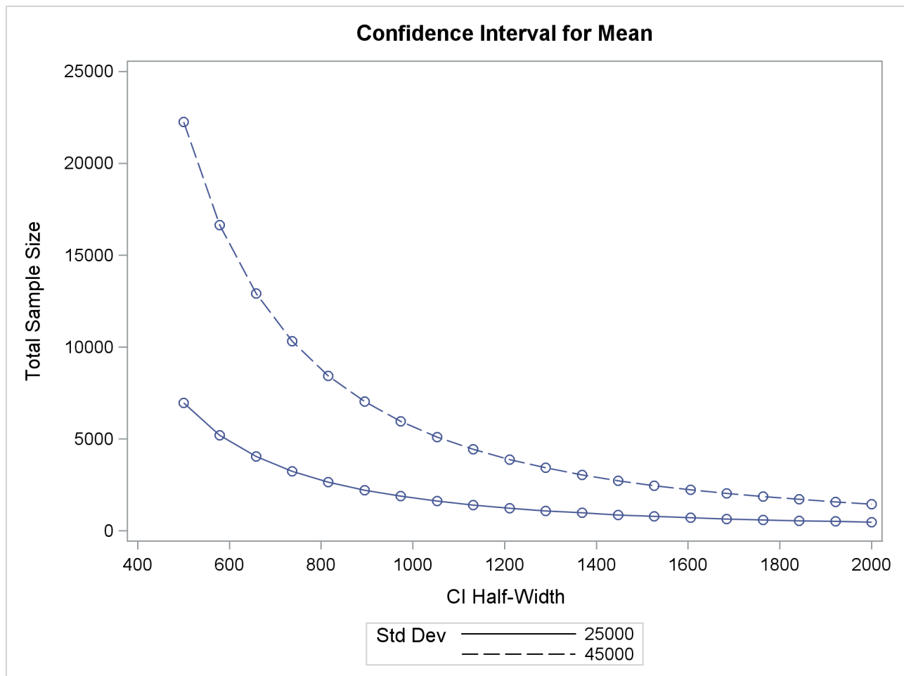
Output 75.7.2 Plot of Sample Size versus Confidence Interval Half-Width
