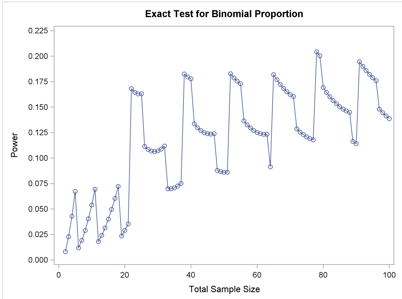
Output 75.2.7 Plot of Power versus Sample Size for a Two-Sided Test
