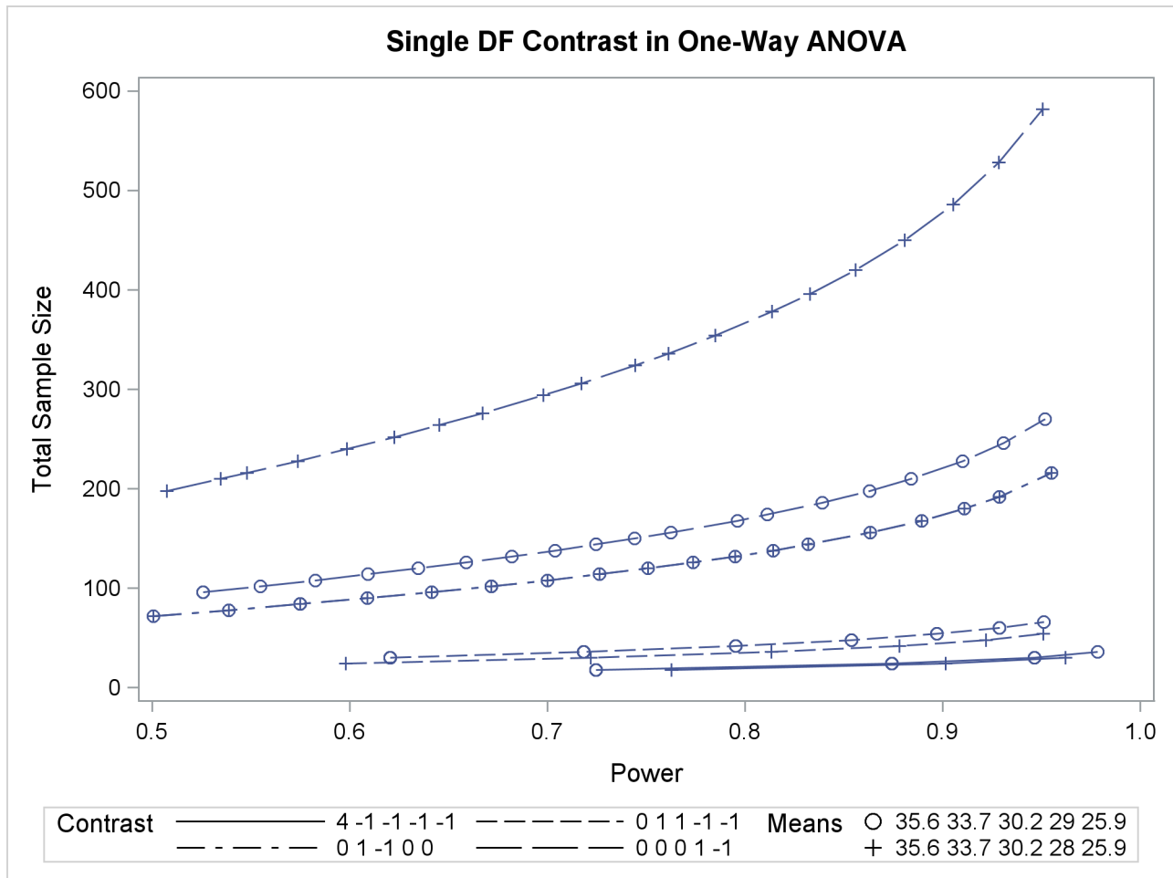
Output 75.1.2 Plot of Sample Size versus Power for One-Way ANOVA Contrasts
