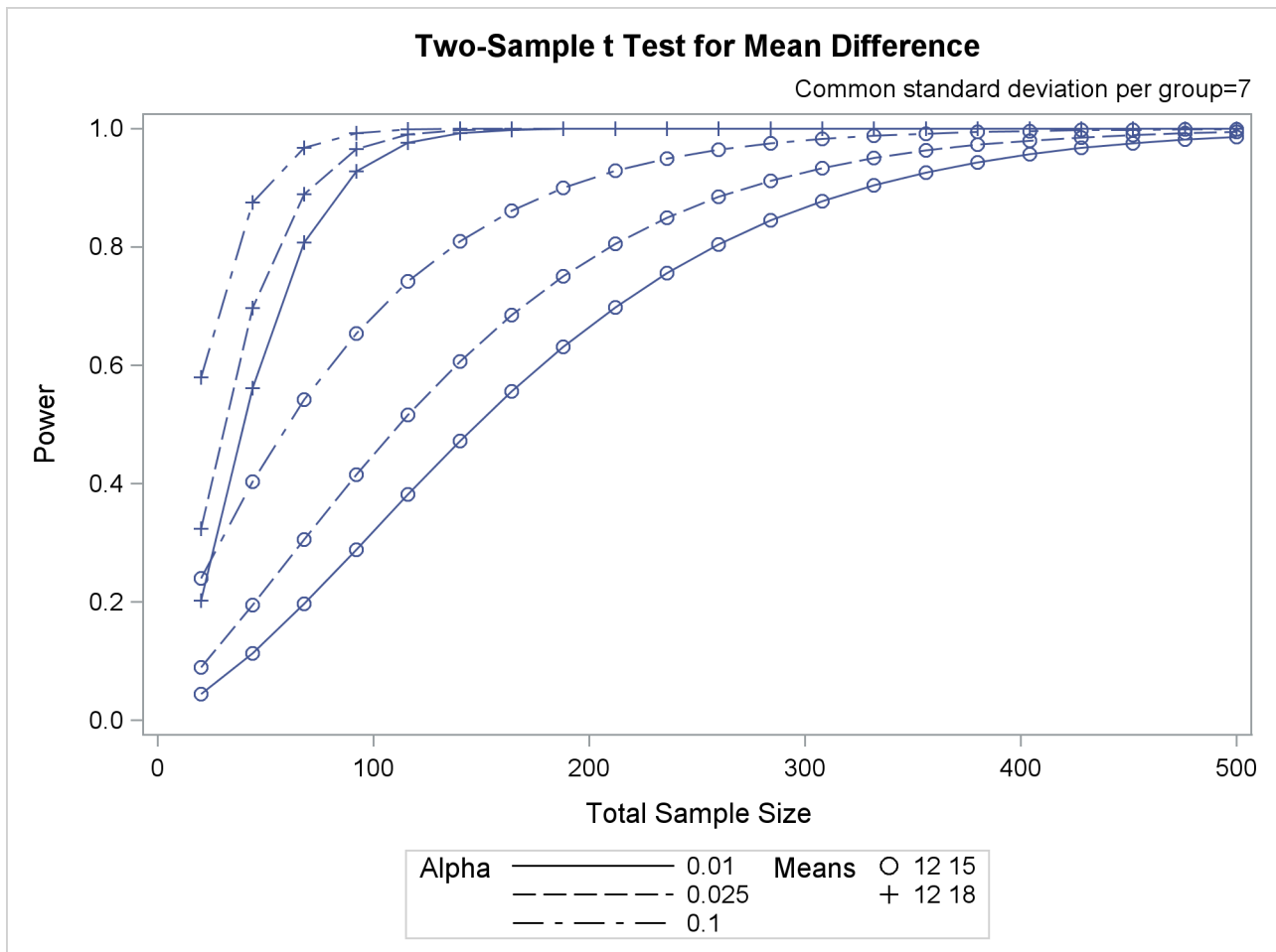
Output 75.8.14 Plot with Default VARY Settings
