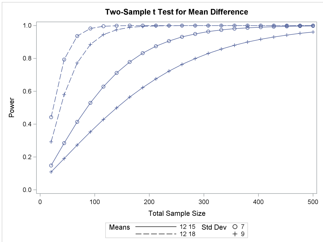
Output 75.8.5 Plot of Power versus Sample Size Using Second Strategy
