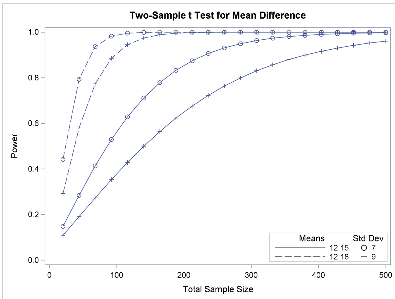
Output 75.8.17 Plot with a By-Feature Key inside the Plotting Region
