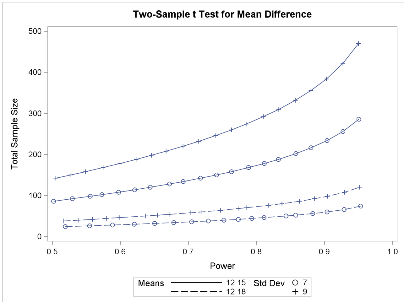
Output 75.8.2 Plot of Sample Size versus Power
