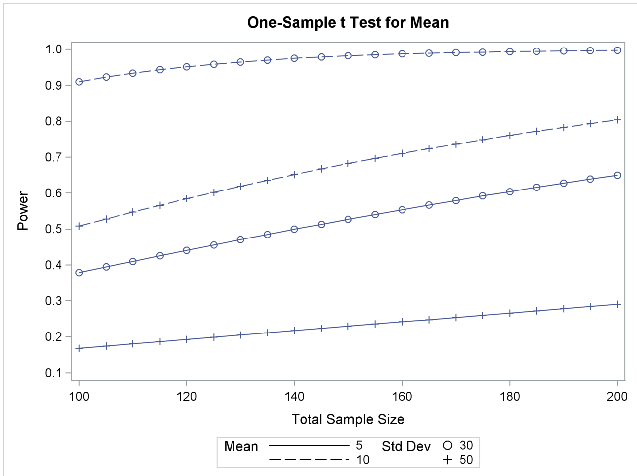
Figure 75.3 Plot of Power versus Sample Size for One-Sample t Test with Input Ranges
