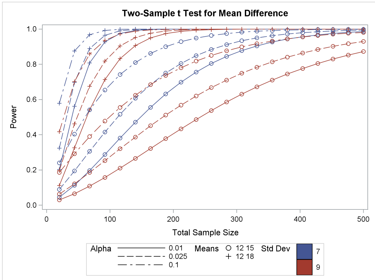
Output 75.8.15 Plot with Varying Color Instead of Panel
