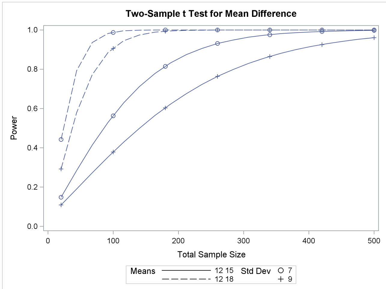
Output 75.8.22 Plot with MARKERS=NICE
