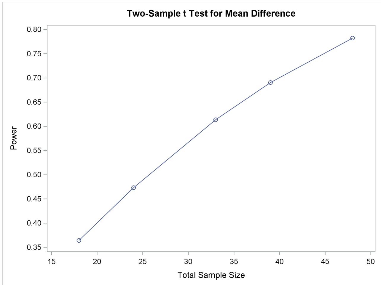
Output 75.8.9 Plot with Unequally Spaced Points
