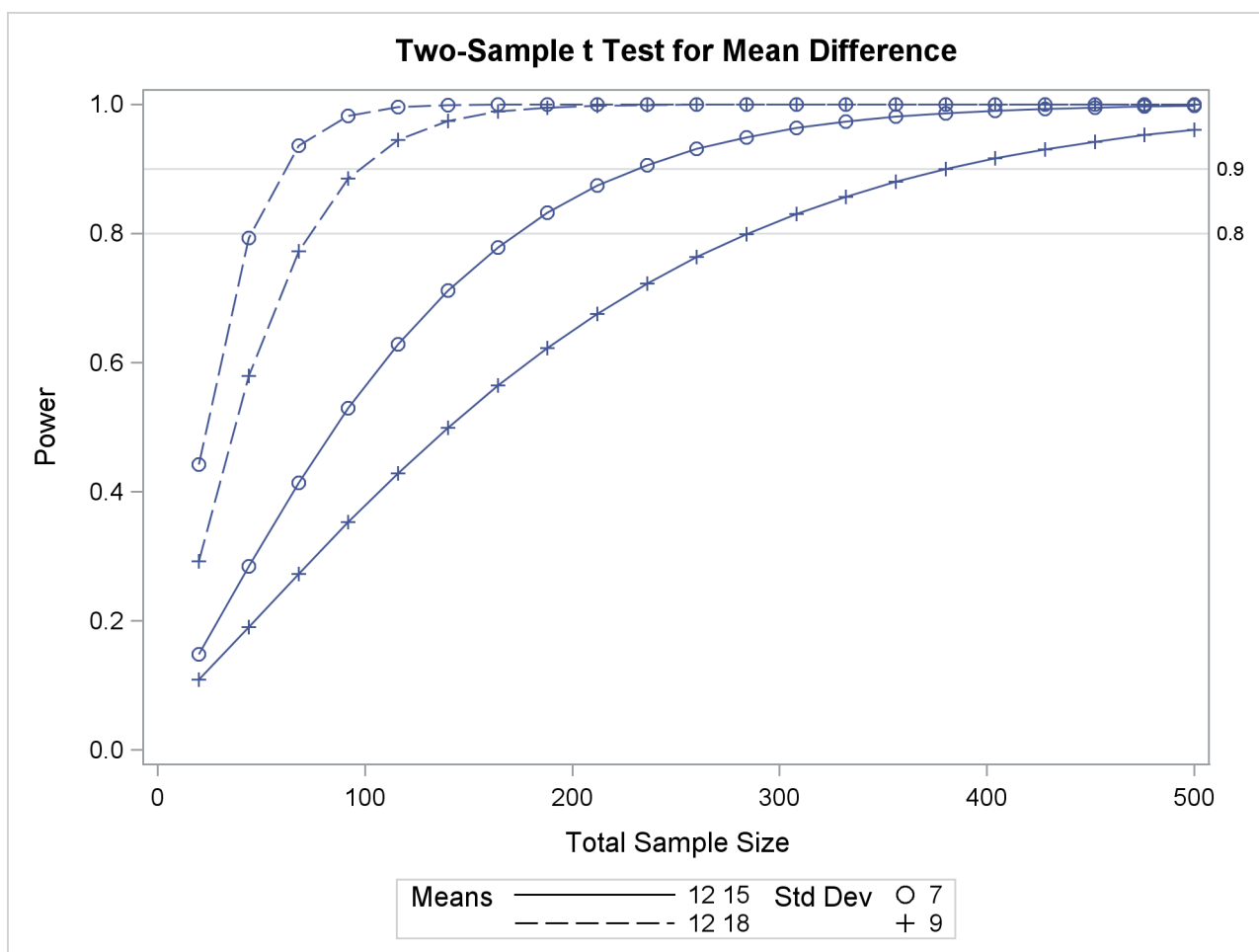
Output 75.8.11 Plot with Simple Reference Lines on Y Axis
