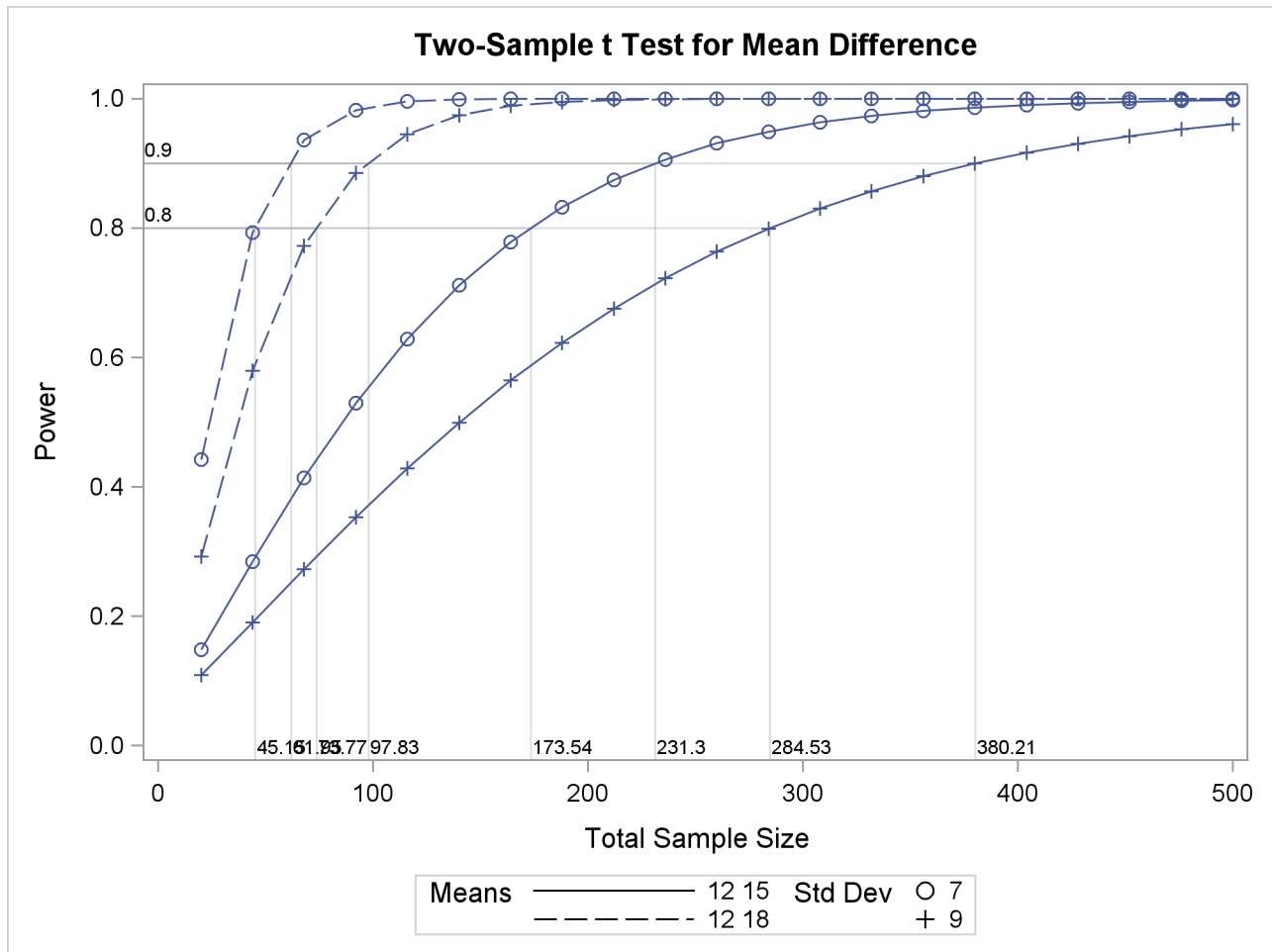
Output 75.8.12 Plot with CROSSREF=YES Style Reference Lines from Y Axis
