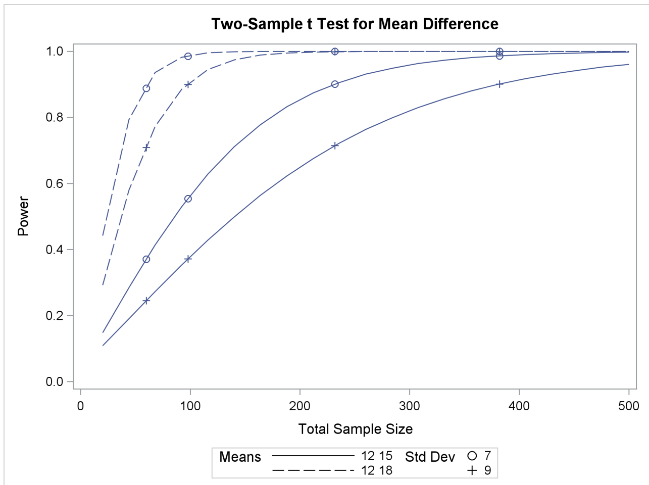
Output 75.8.21 Plot with MARKERS=ANALYSIS
