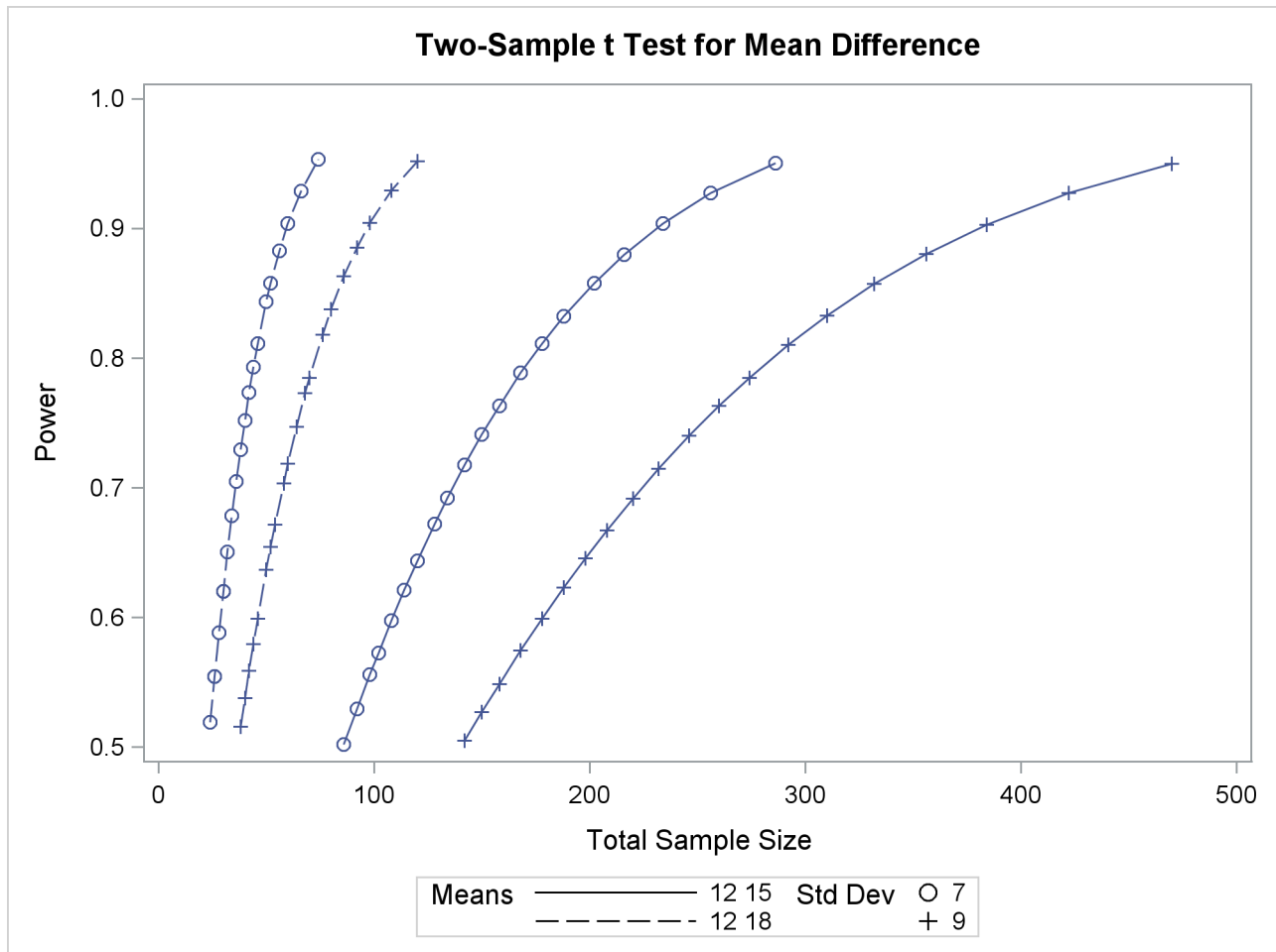
Output 75.8.3 Plot of Power versus Sample Size using First Strategy
