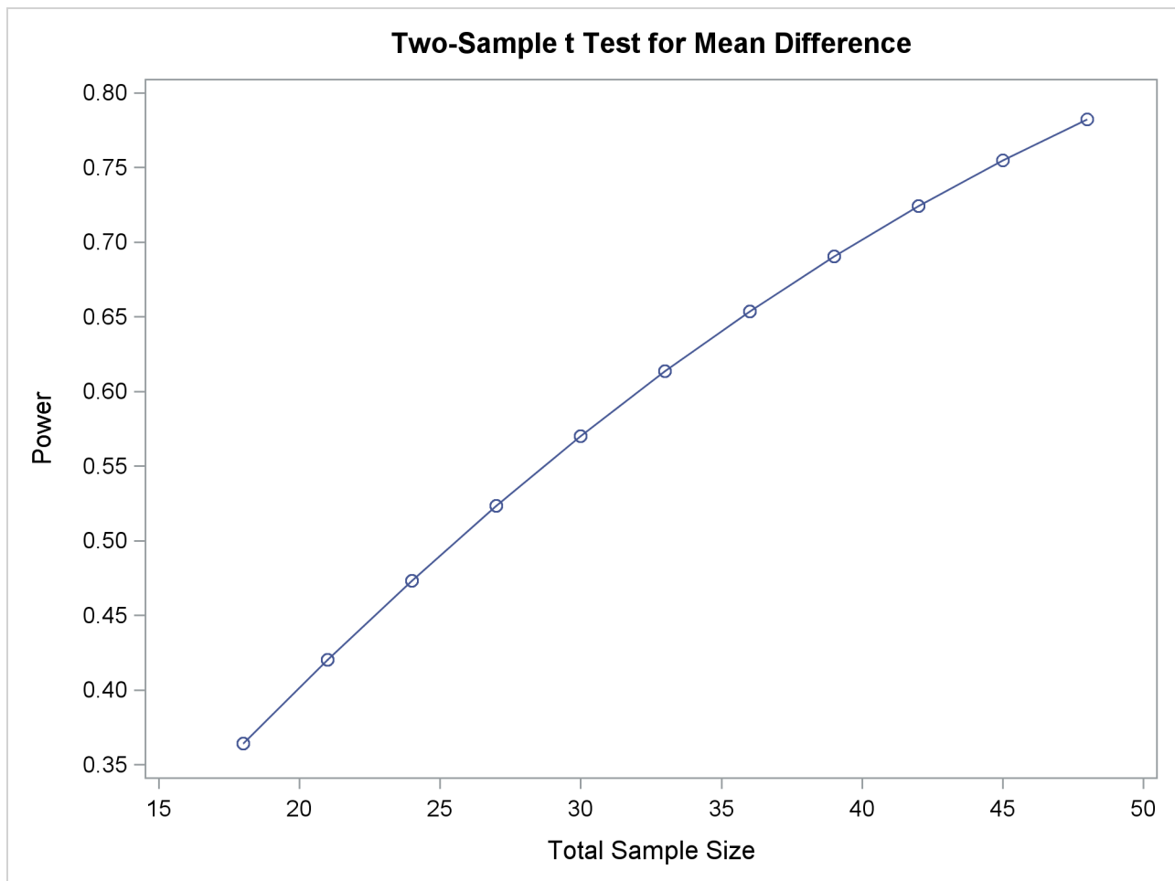
Output 75.8.7 Plot with Overlapping Points
