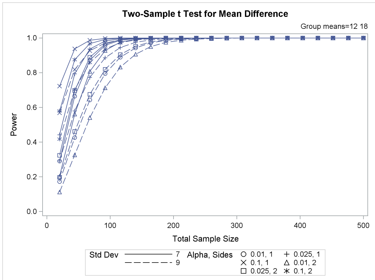
Output 75.8.16 Plot with Features Explicitly Linked to Parameters
