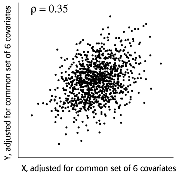
Figure 75.9 Partial Regression Plot
