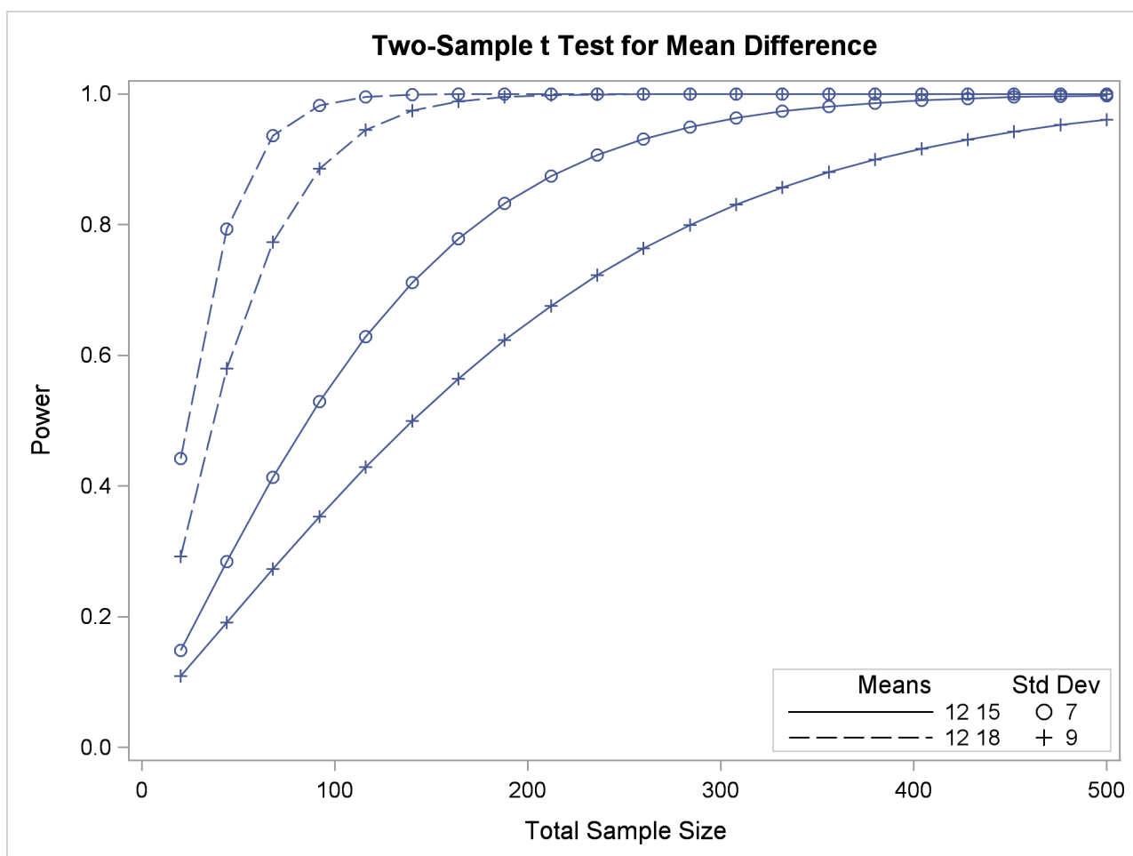
Output 75.8.19 Plot with a Nonnumbered By-Curve Key
