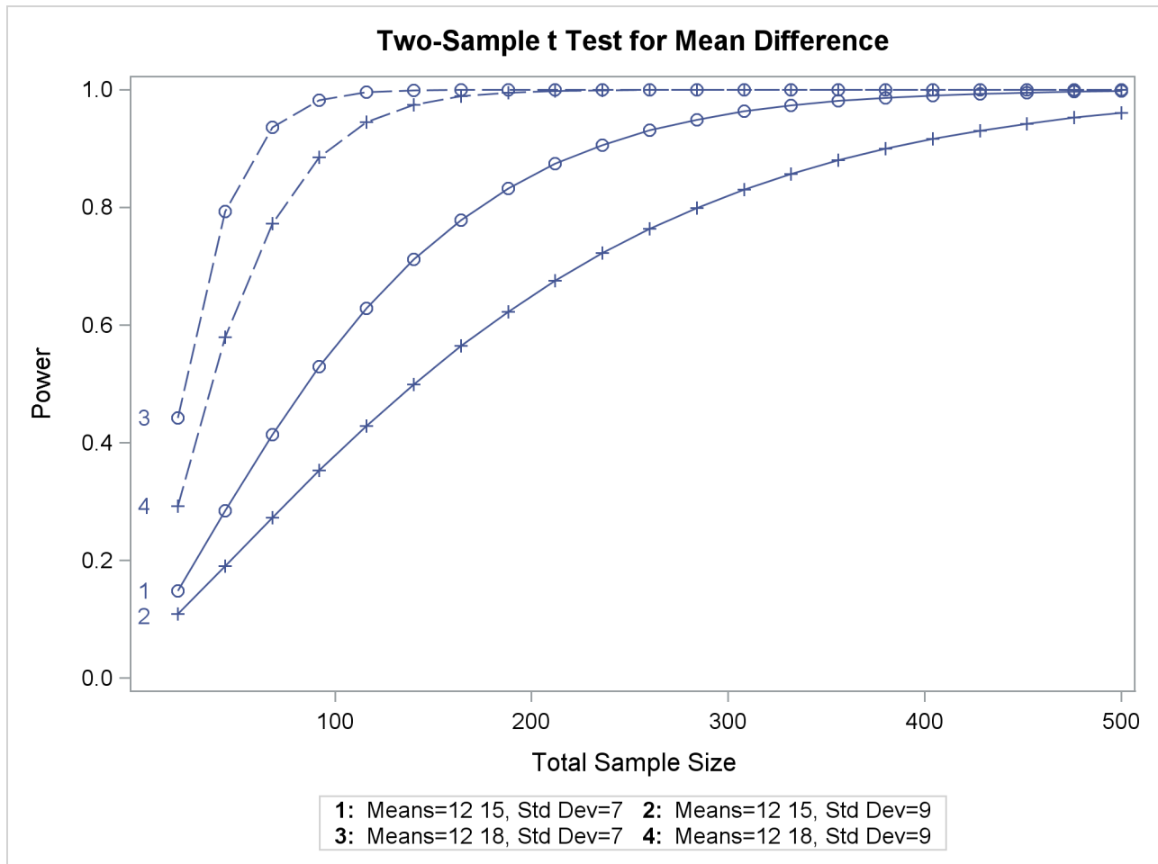
Output 75.8.18 Plot with a Numbered By-Curve Key
