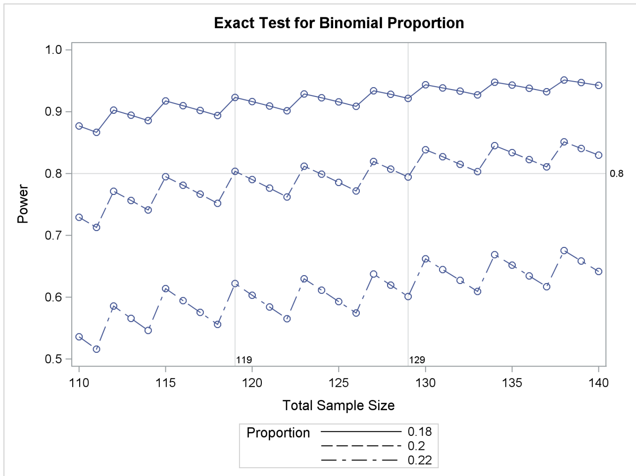
Output 75.2.4 Plot for Assessing Sensitivity to True Proportion Value
