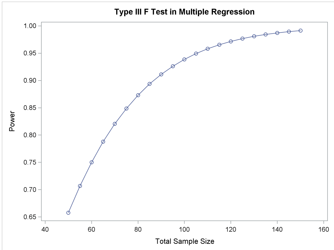
Output 75.5.2 Plot of Power versus Sample Size for Multiple Regression
