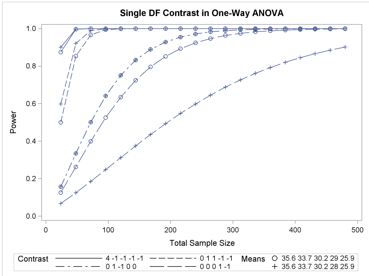
Output 75.1.3 Plot of Power versus Sample Size for One-Way ANOVA Contrasts
