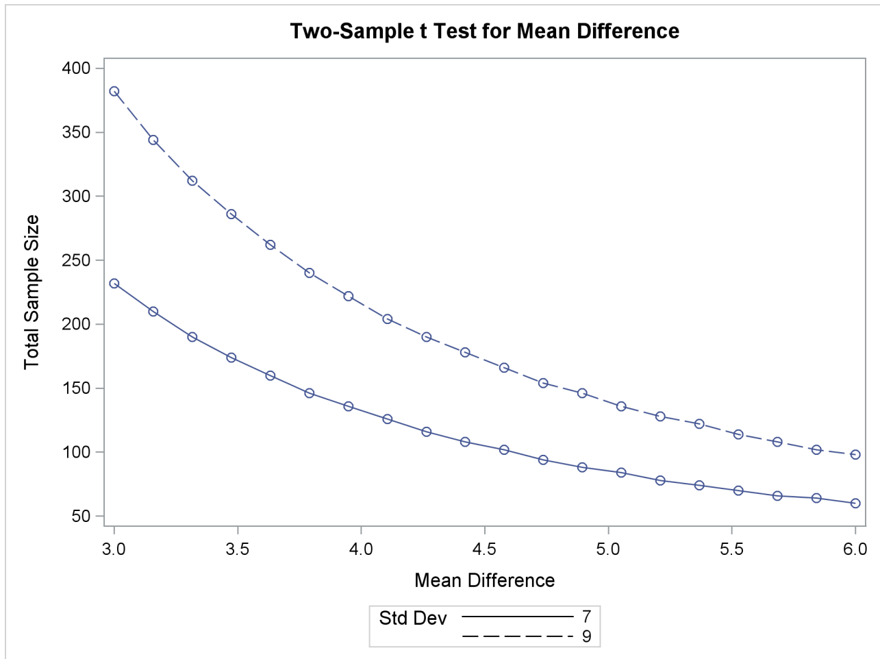
Output 75.8.6 Plot of Sample Size versus Mean Difference
