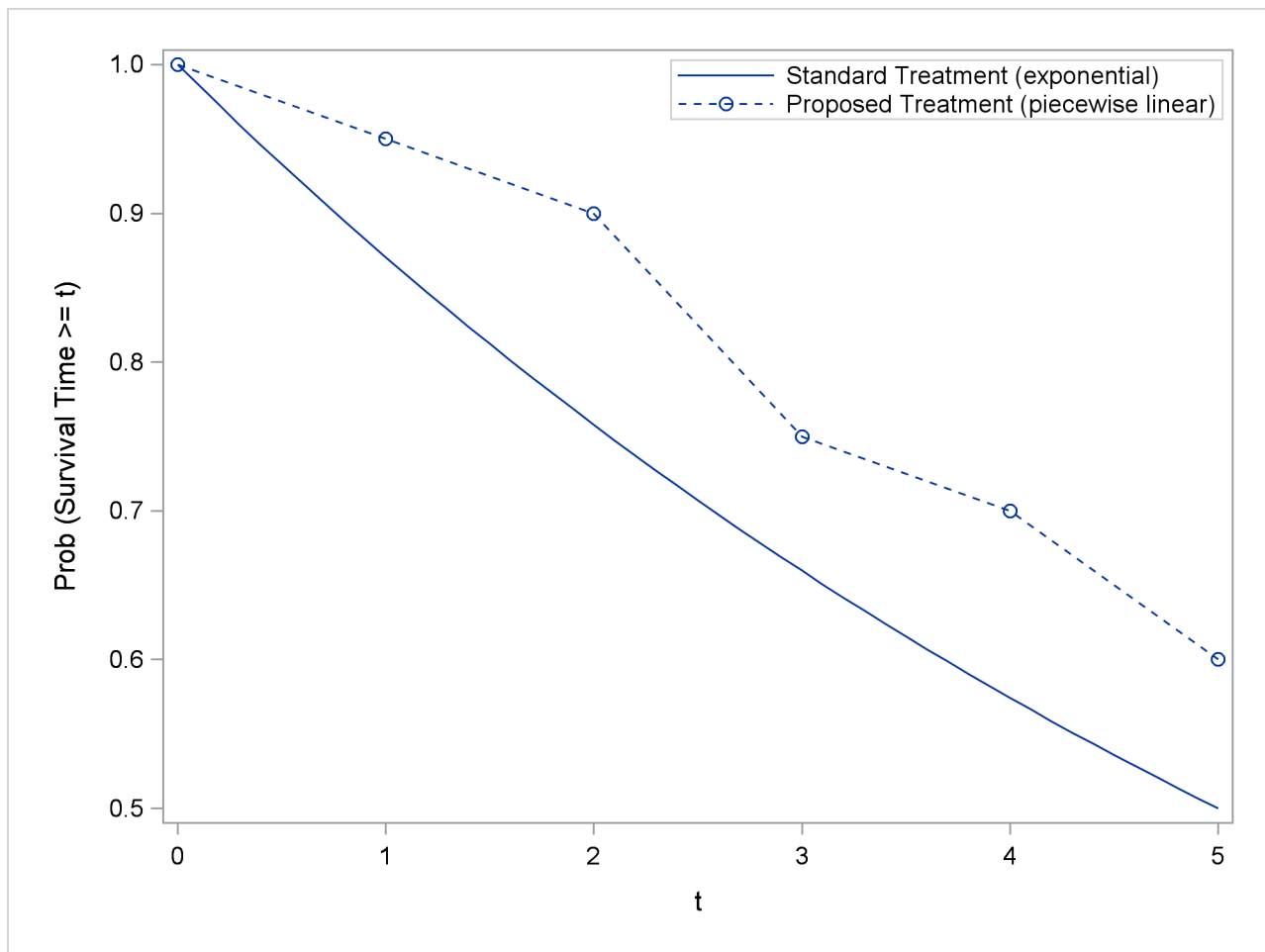
Output 75.6.1 Survival Curves
