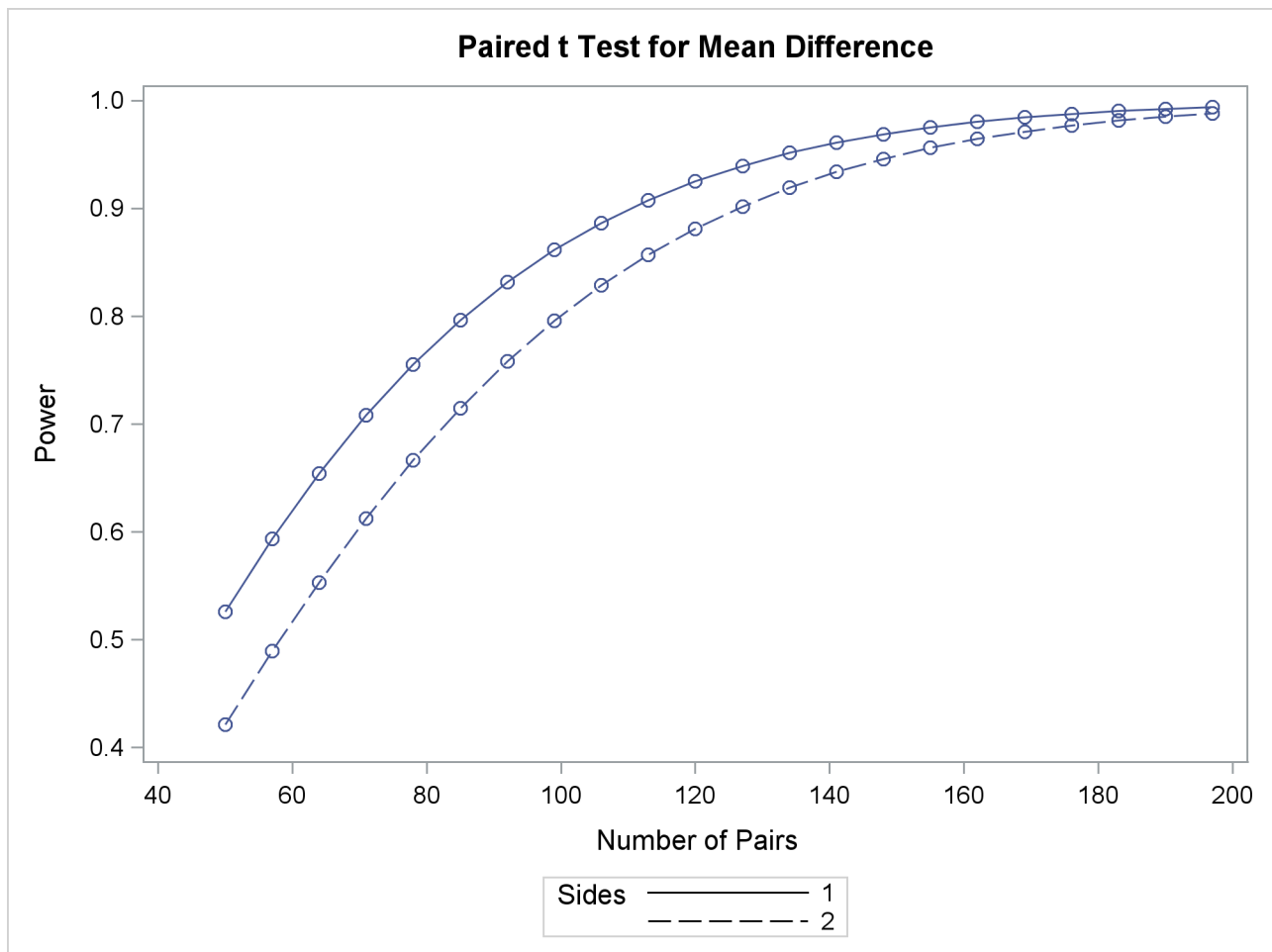
Output 75.3.2 Plot of Power versus Sample Size for Paired t Analysis of Crossover Design
