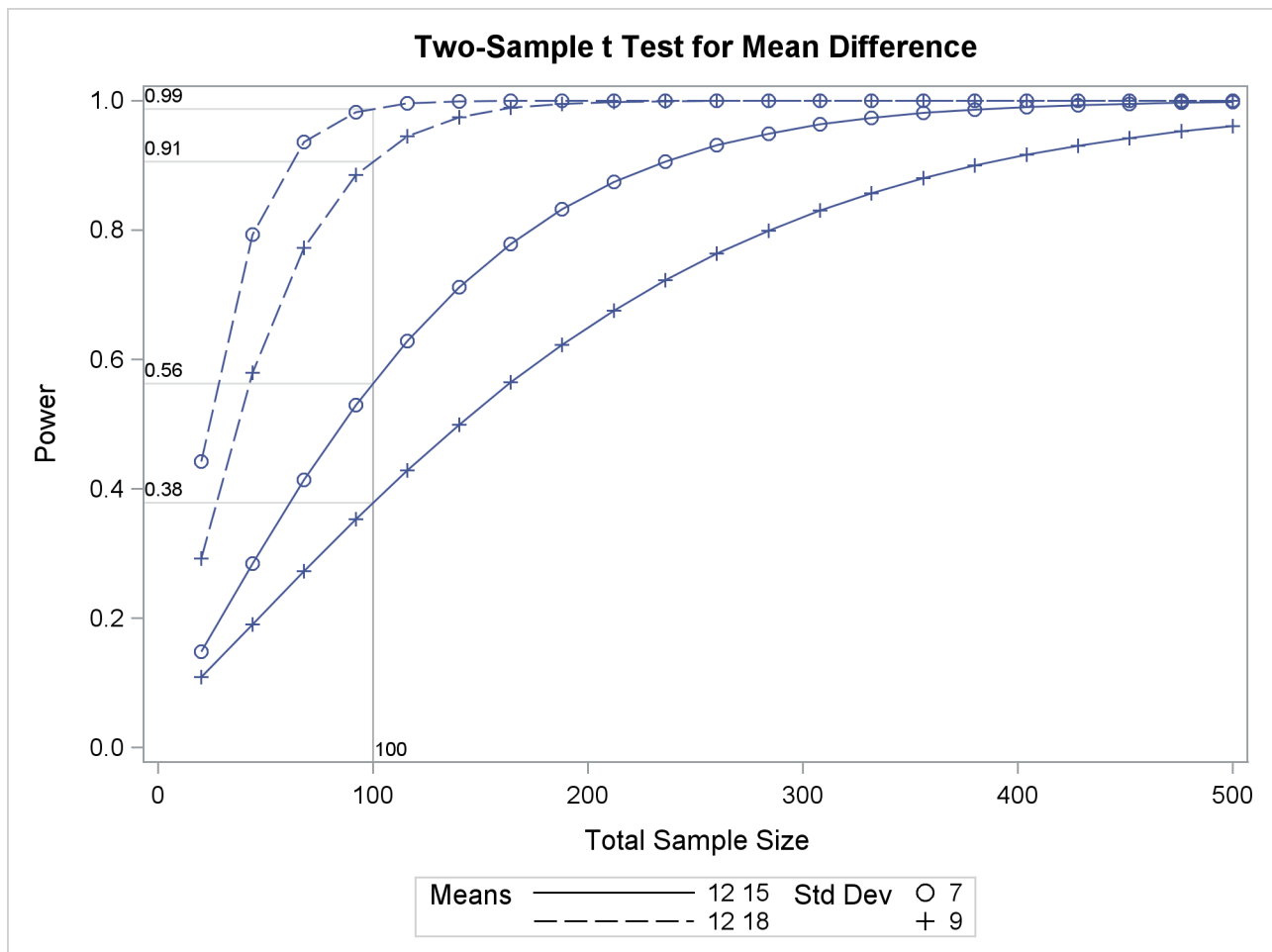
Output 75.8.13 Plot with CROSSREF=YES Style Reference Lines from X Axis
