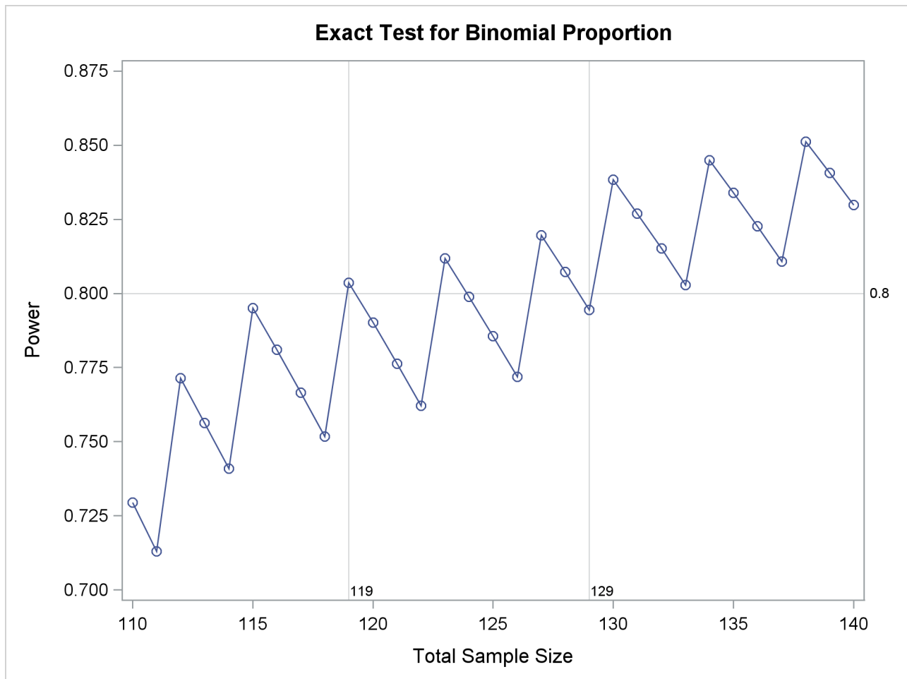
Output 75.2.3 Plot of Power versus Sample Size for Exact Binomial Test
