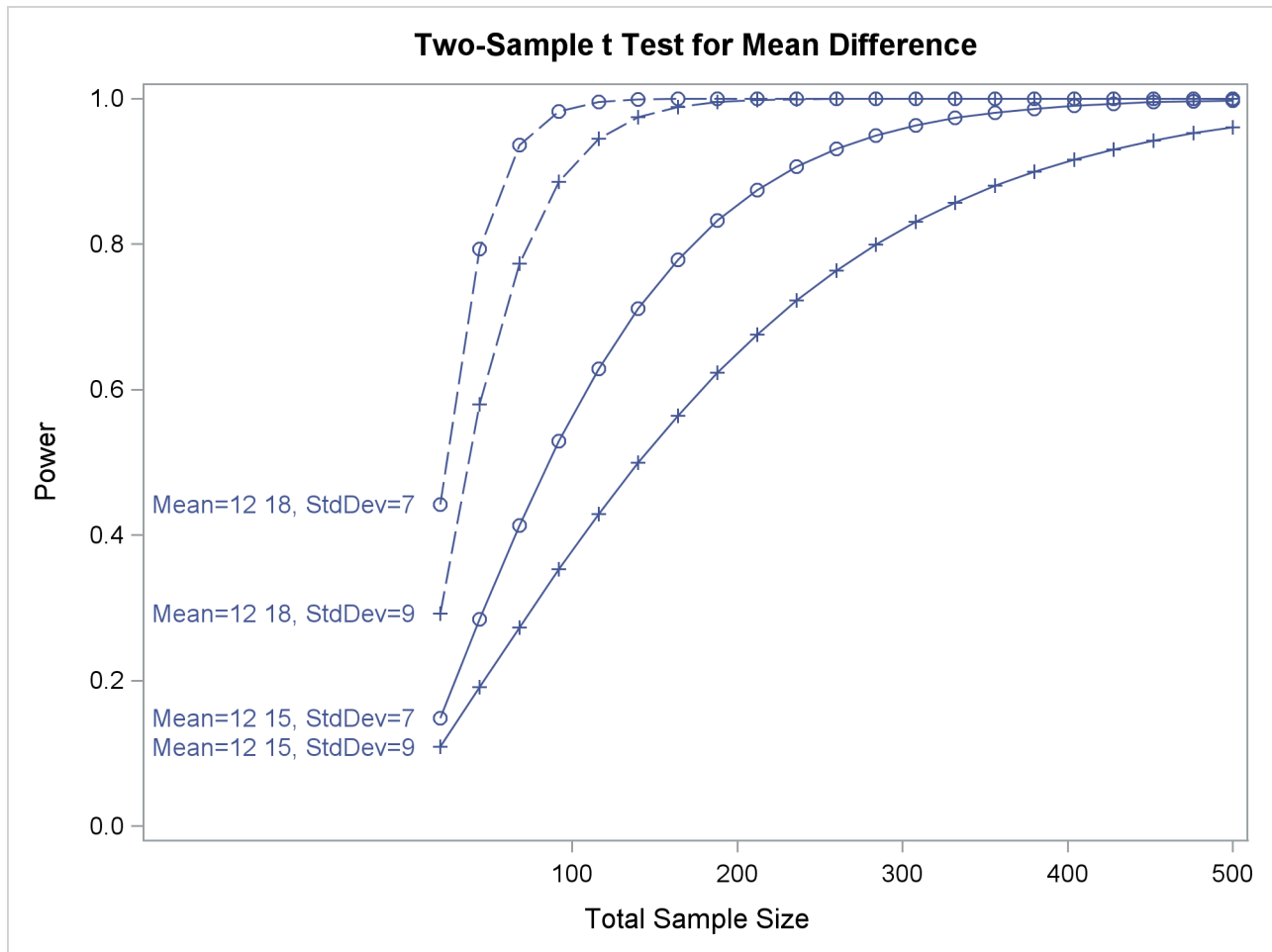
Output 75.8.20 Plot with Directly Labeled Curves
