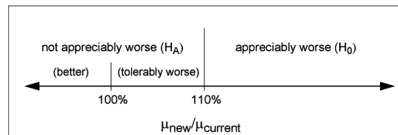
Figure 75.8 Hypotheses for the Pollutant Study
