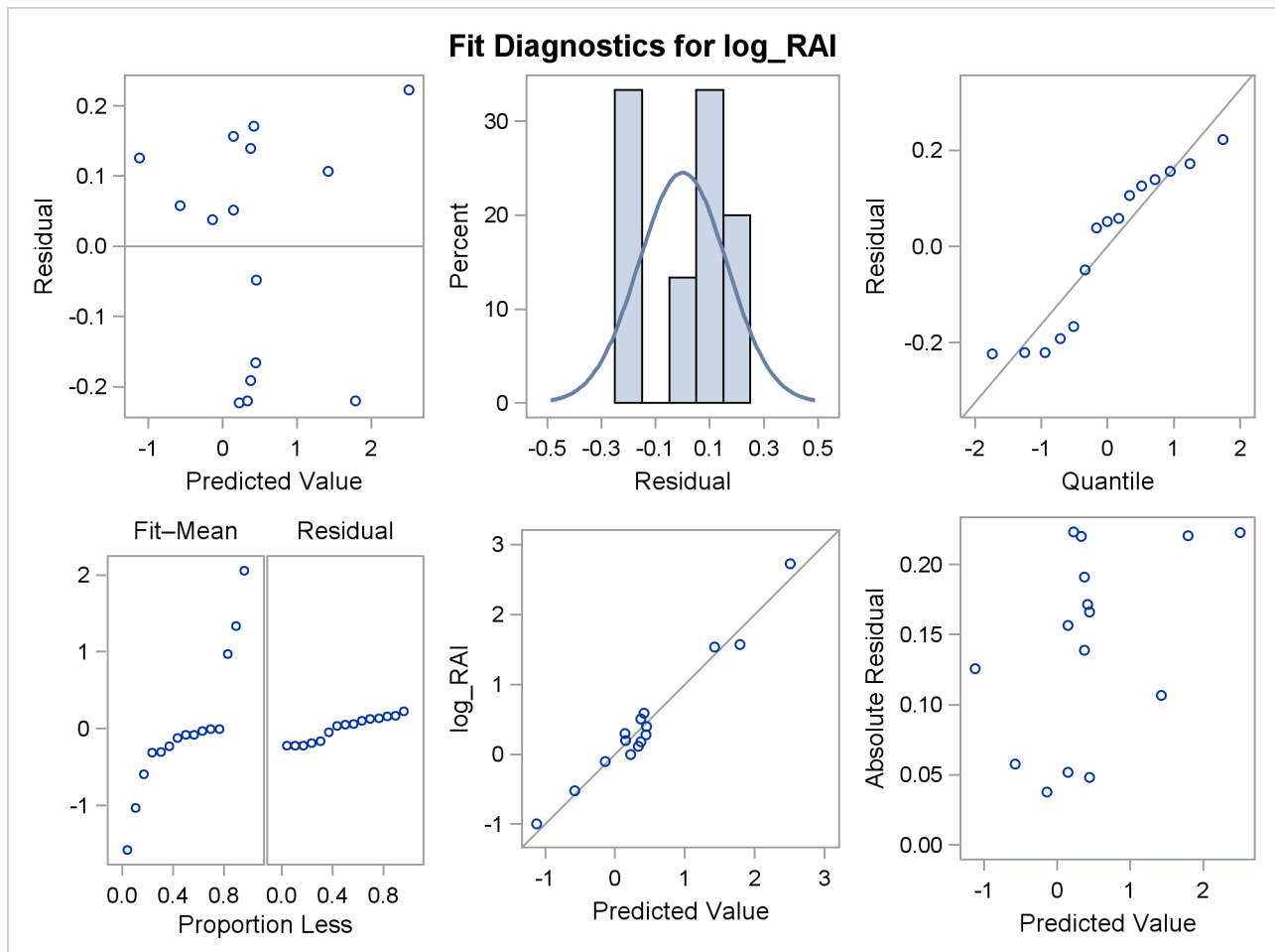
Output 74.2.1 Model Fit Diagnostics
