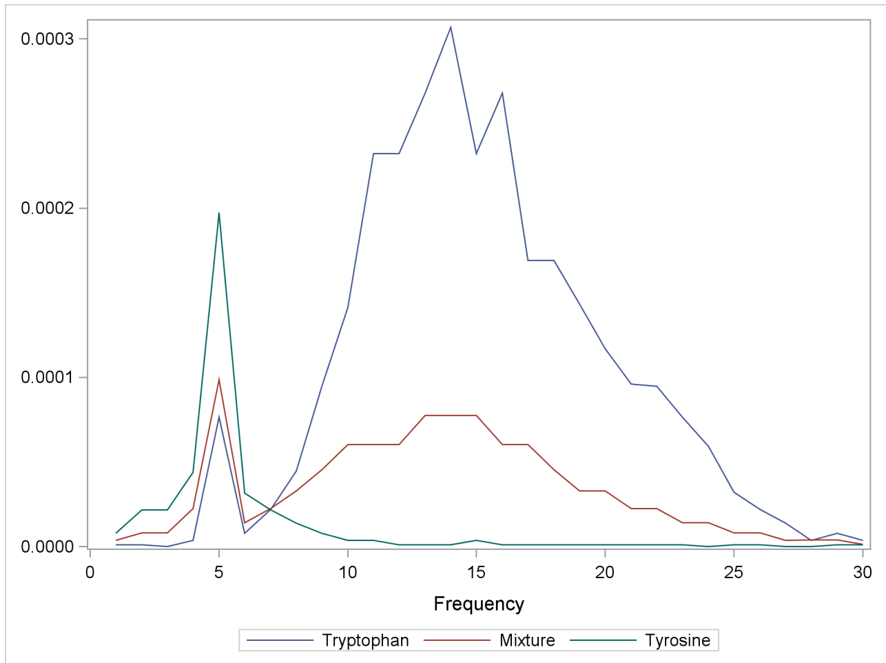
Output 74.3.1 Spectra for Three Samples of Tyrosine and Tryptophan
