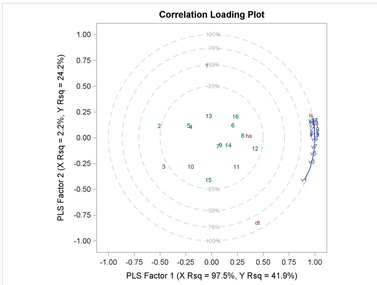
Figure 74.8 Correlation Loadings Plot
