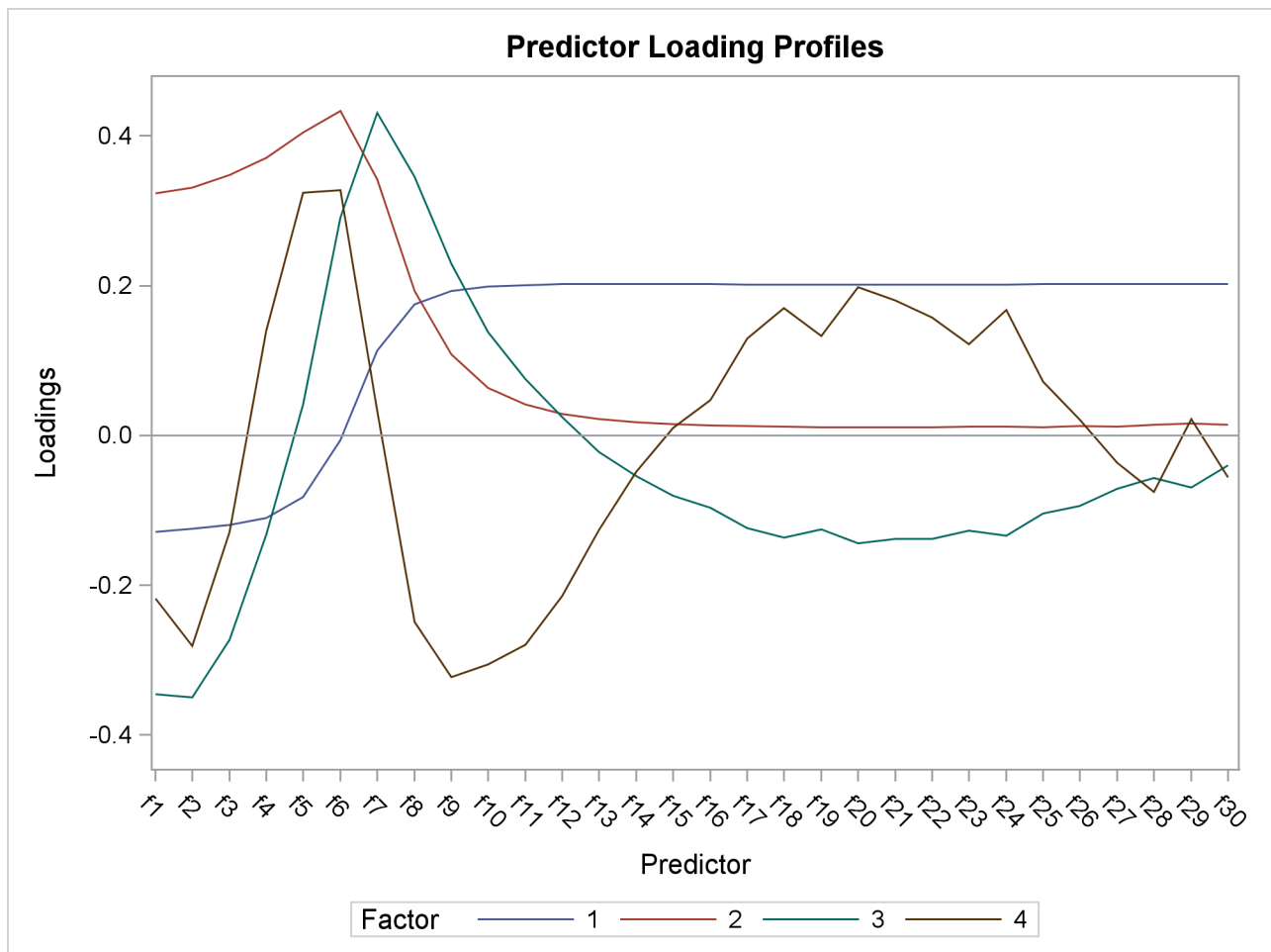
Output 74.3.5 Predictor Loadings across Frequencies
