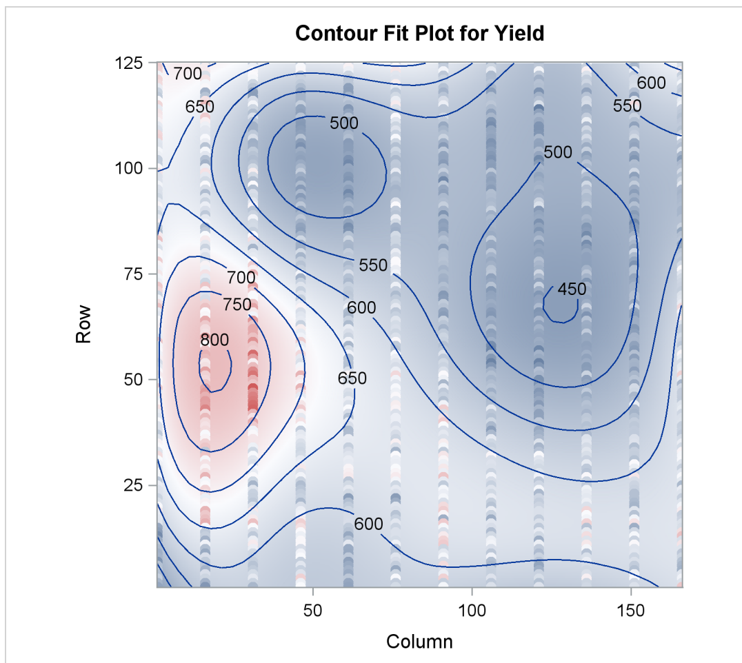
Output 74.4.4 Default Spline Basis: Smoothed Yield
