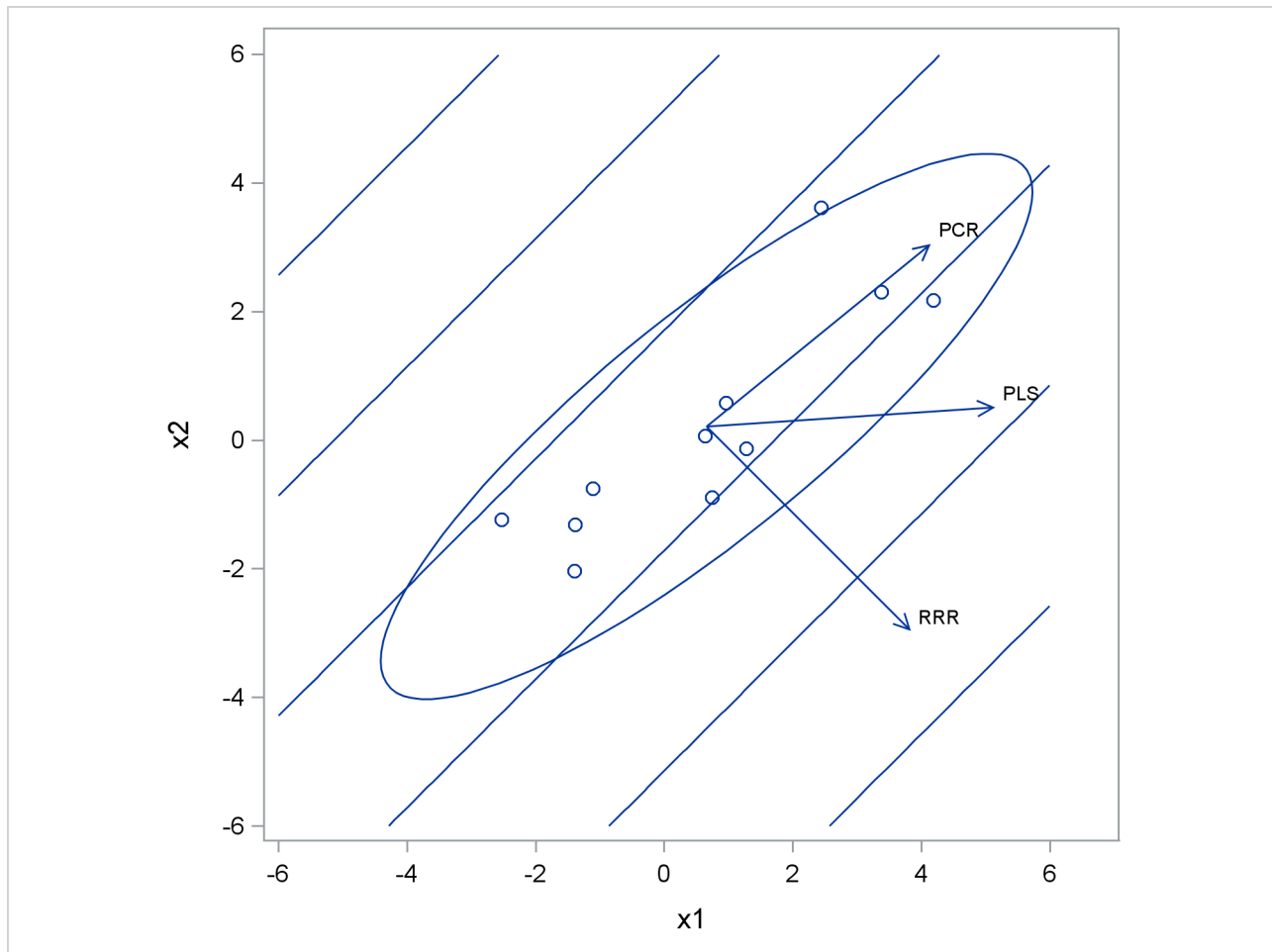
Figure 74.12 Depiction of First Factors for Three Different Regression Methods
