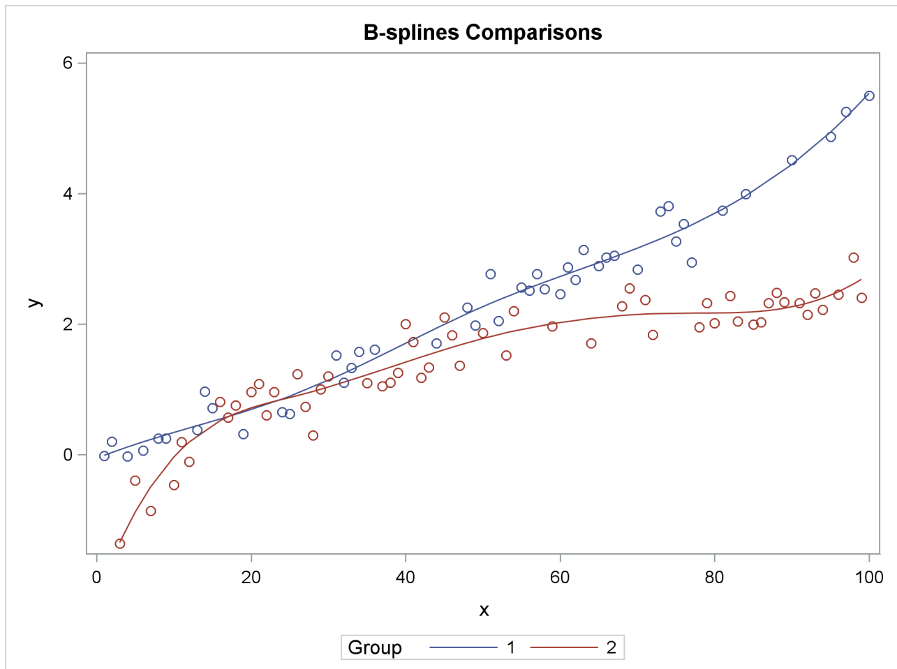
Output 73.6.2 Observed Data and Predicted Values by Group
