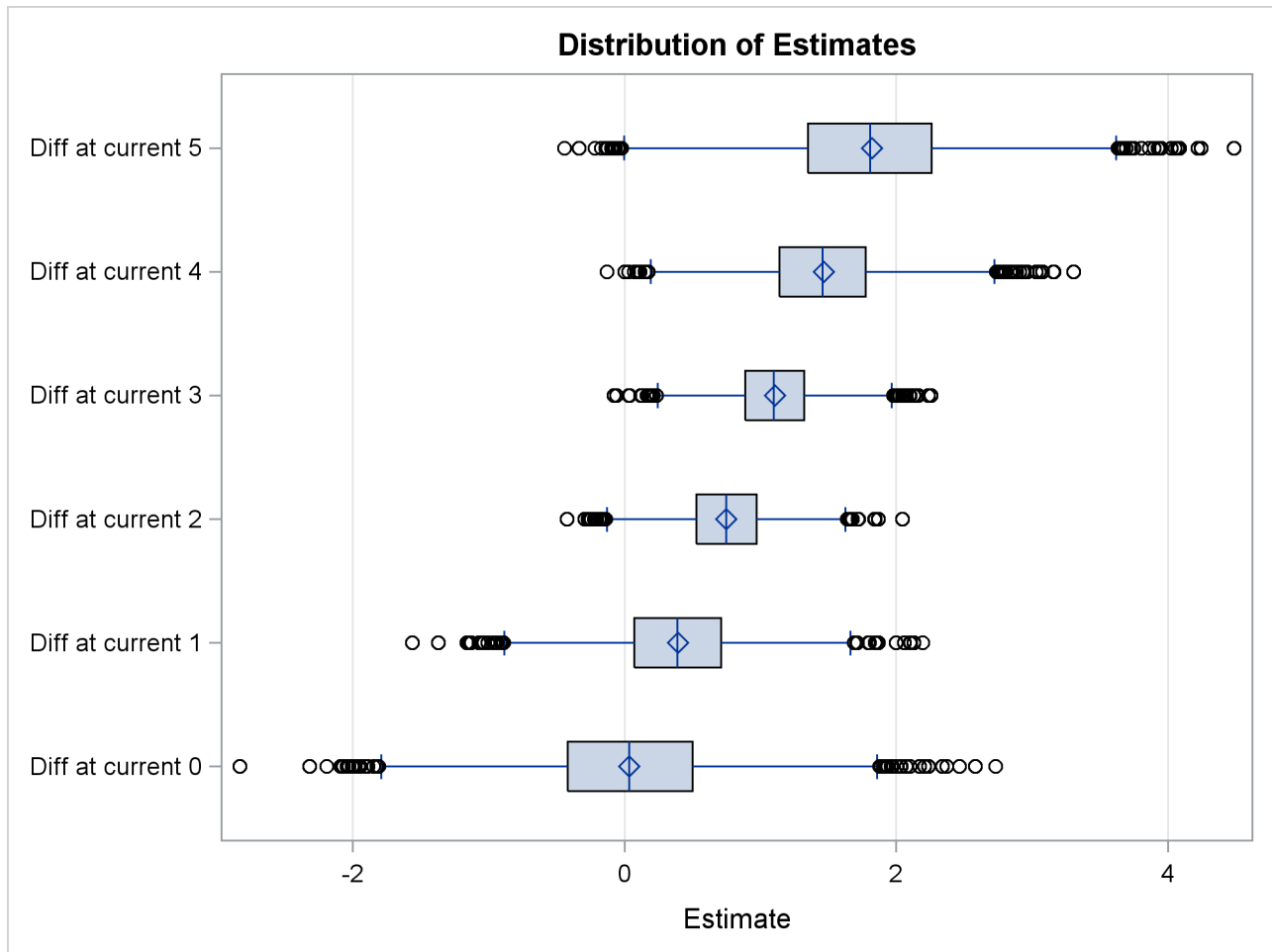
Output 73.4.3 Box Plot of Difference between Two Experiments
