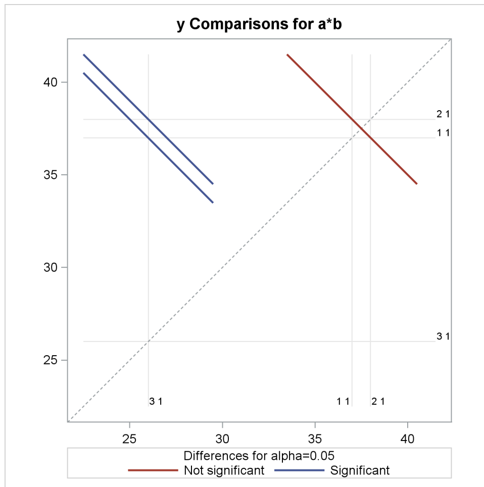
Figure 73.6 LS-Means Difference Diffogram
