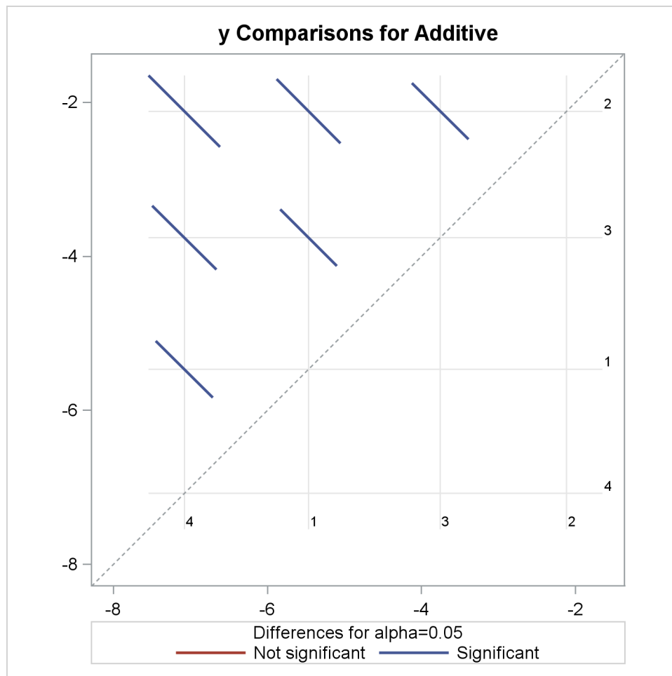
Output 73.3.2 LS-Means Plot of Pairwise Differences
