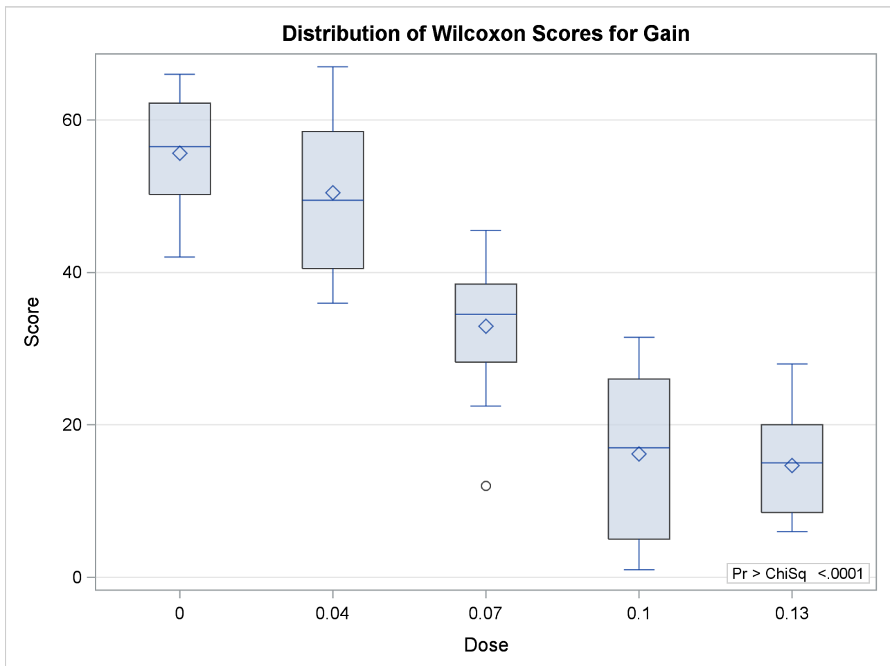
Figure 69.7 Box Plot of Wilcoxon Scores
