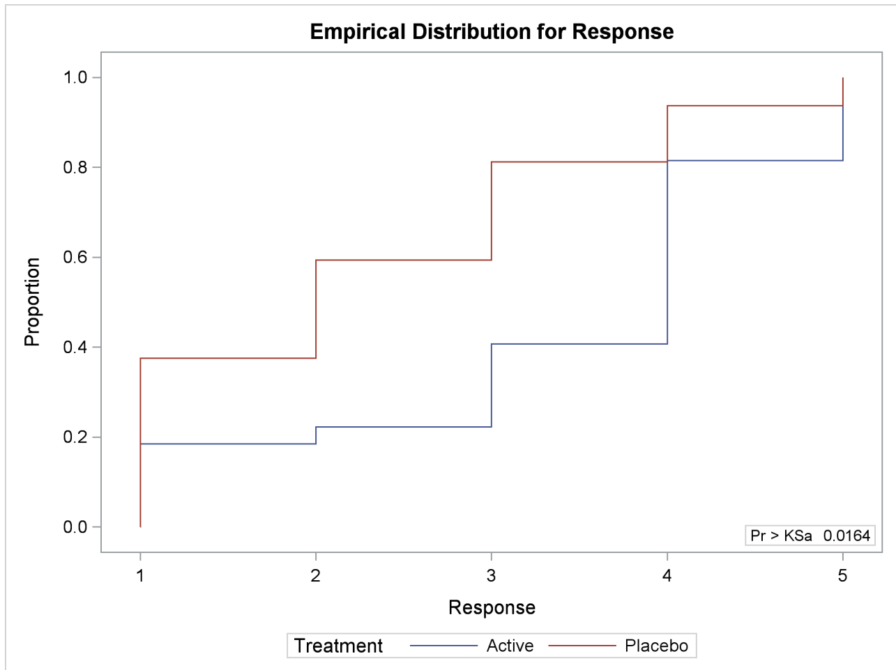
Output 69.2.2 Empirical Distribution Function Plot
