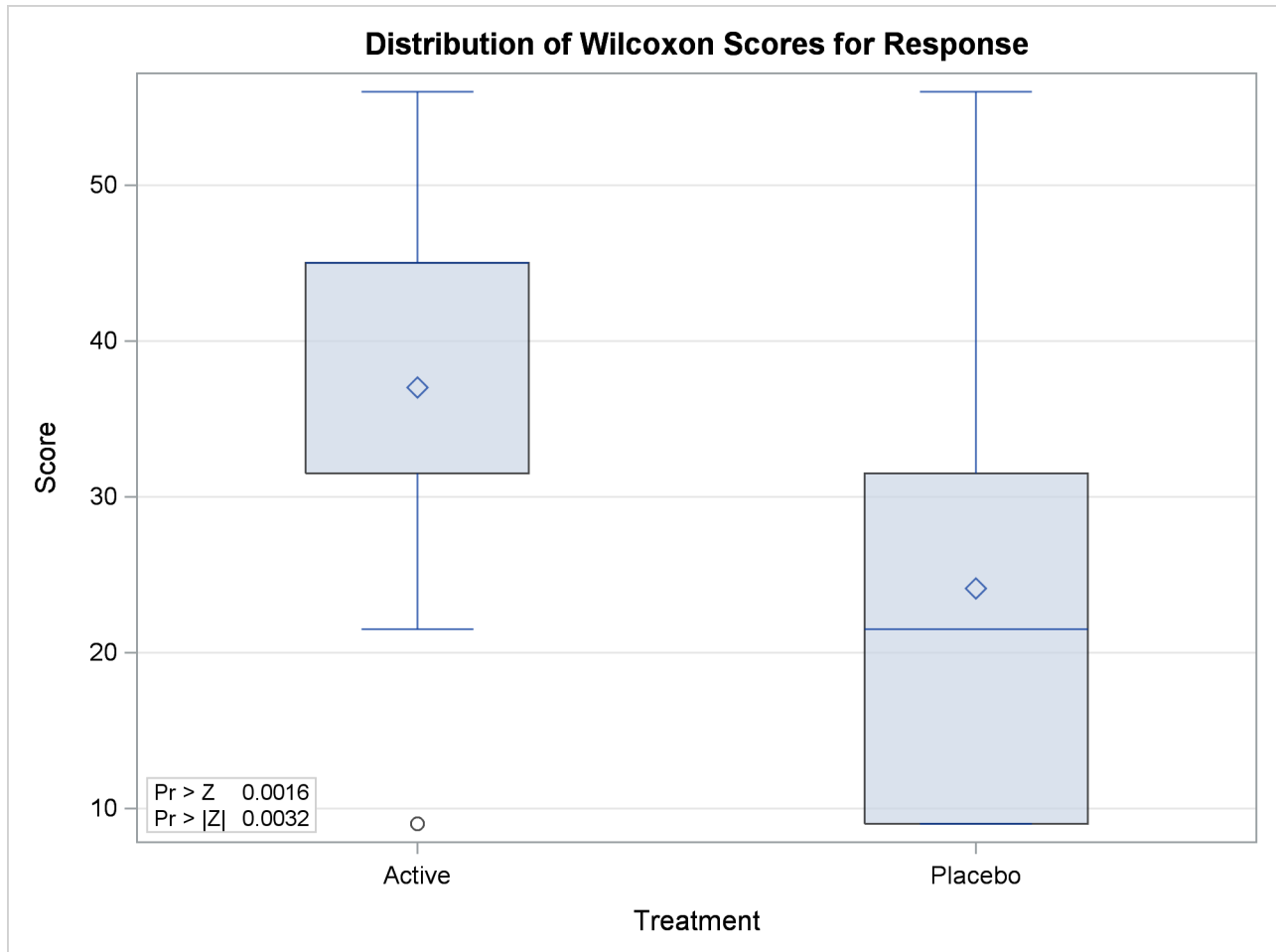
Output 69.1.2 Box Plot of Wilcoxon Scores
