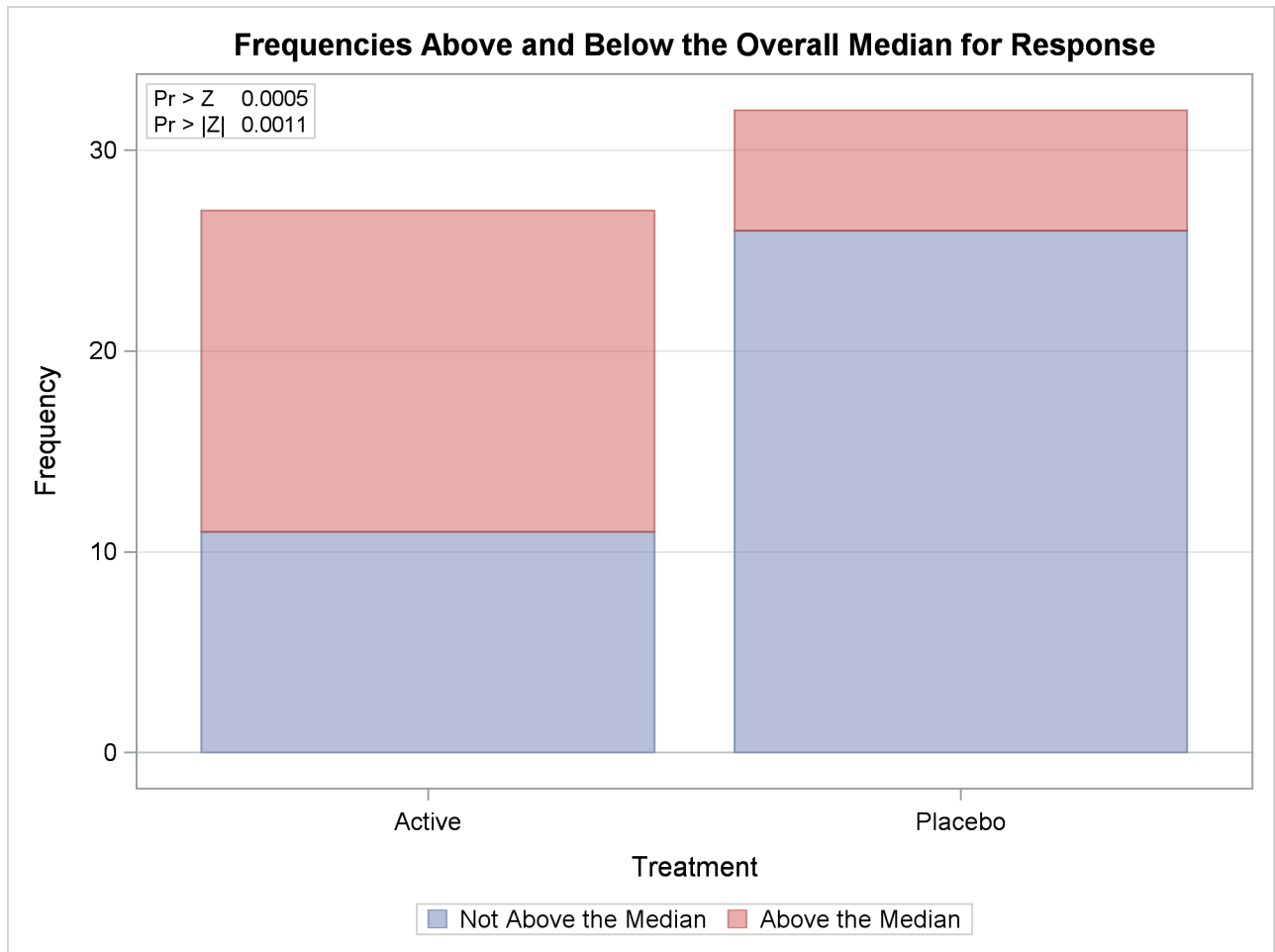
Output 69.1.4 Median Plot
