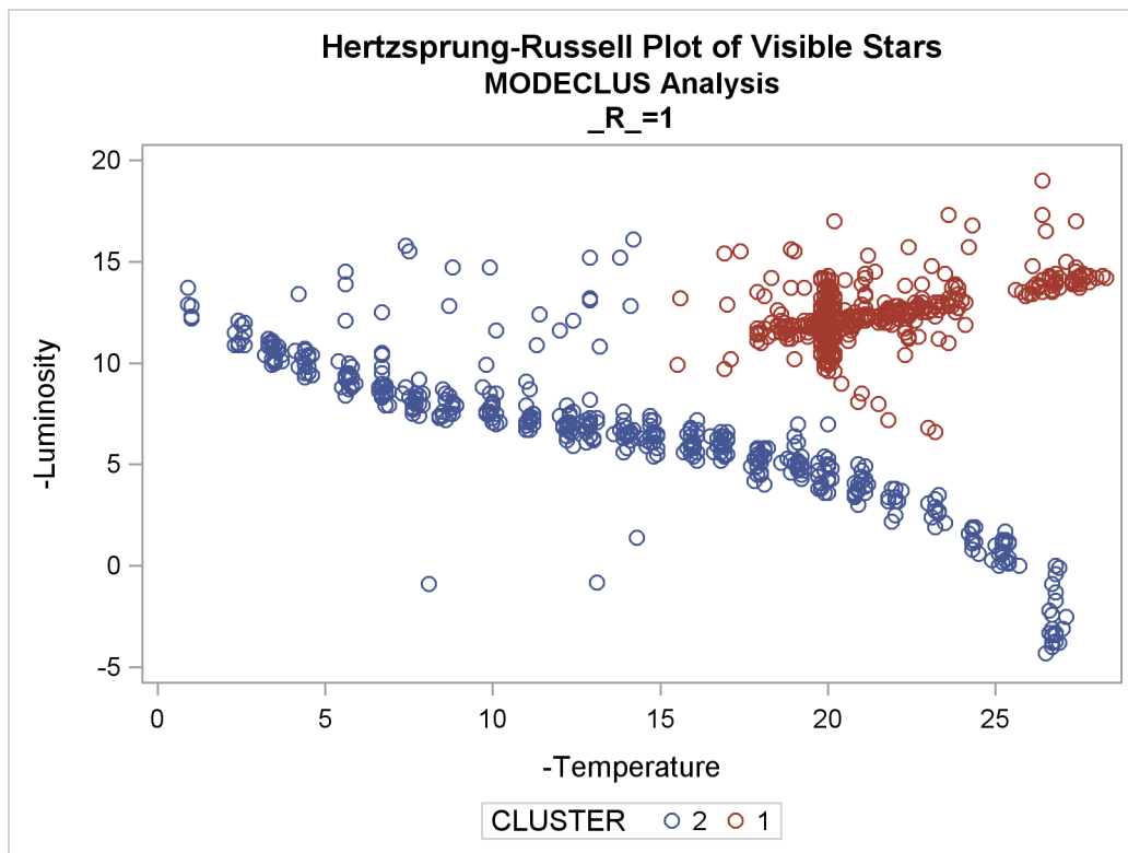
Output 64.4.3 Scatter Plots of Cluster Memberships by \_R\_ = 1
