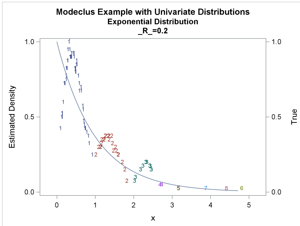
Output 64.1.8 True Density, Estimated Density, and Cluster Membership by Various _R Values
