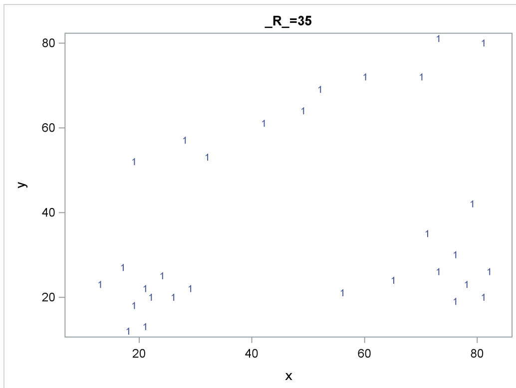
Figure 64.8 Scatter Plots of Cluster Memberships with _R_=35
