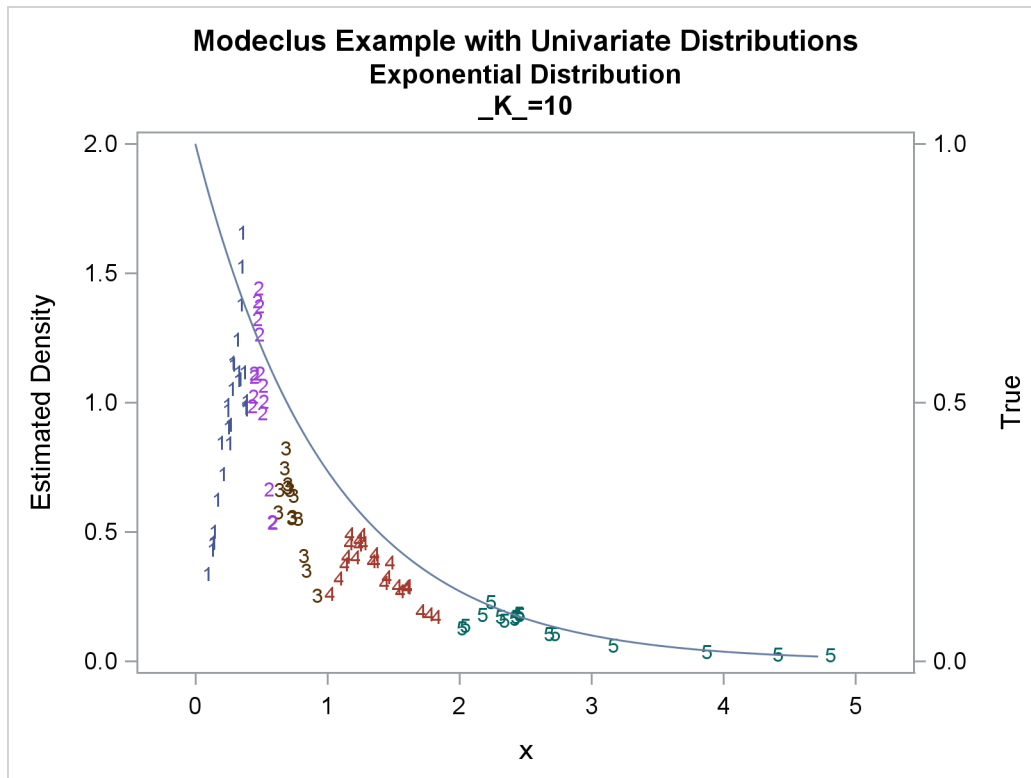
Output 64.1.6 True Density, Estimated Density, and Cluster Membership by Various _K_ Values
