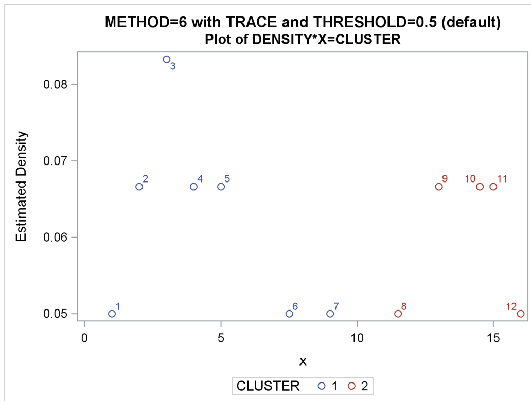
Output 64.5.2 Density Plot
