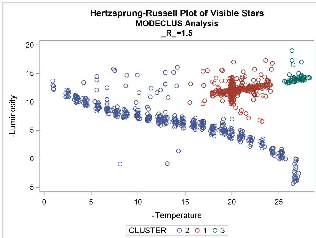
Output 64.4.4 Scatter Plots of Cluster Memberships by \_R\_ = 1.5
