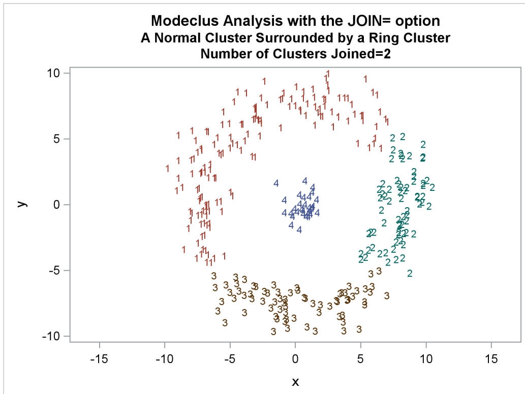
Output 64.3.5 Cluster Memberships When Number of Clusters Joined=2
