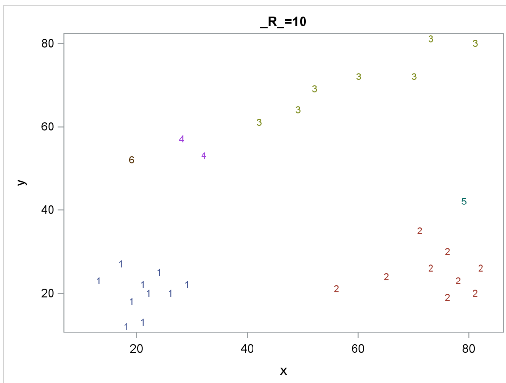
Figure 64.6 Scatter Plots of Cluster Memberships with _R_=10
