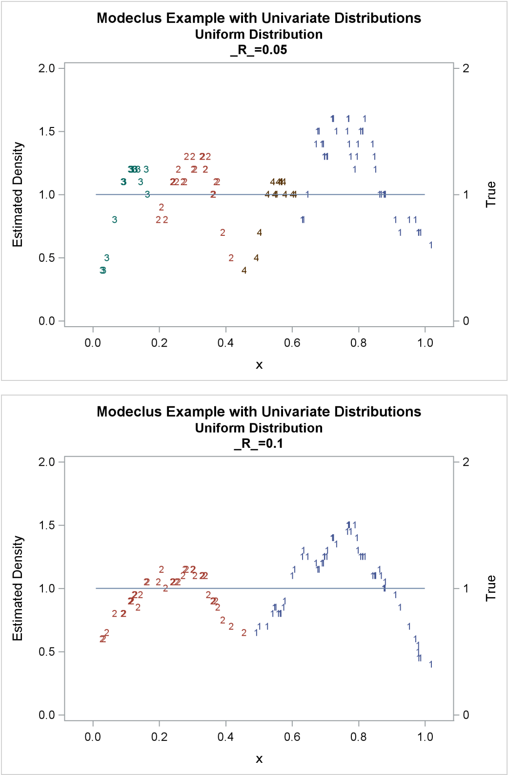
Output 64.1.4 True Density, Estimated Density, and Cluster Membership by Various _R_ Values
