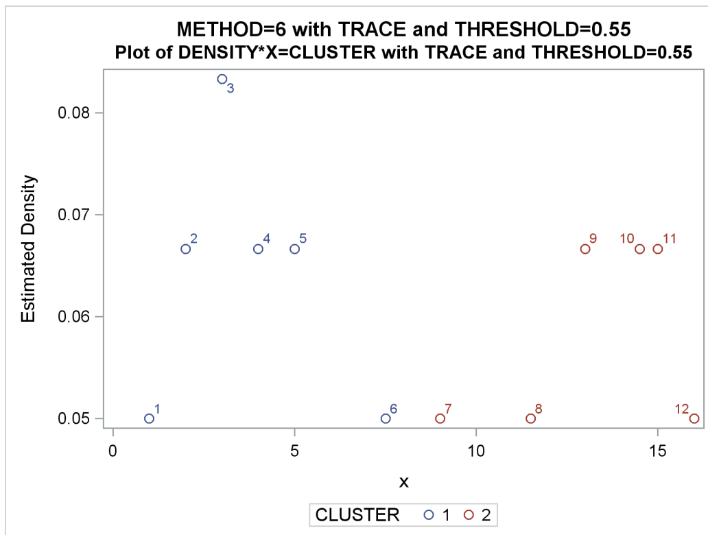
Output 64.5.4 Density Plot
