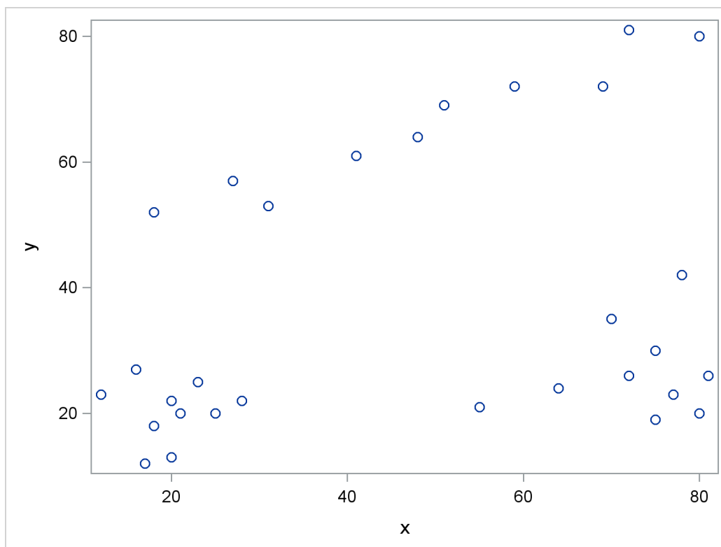
Figure 64.1 Scatter Plot of Data
