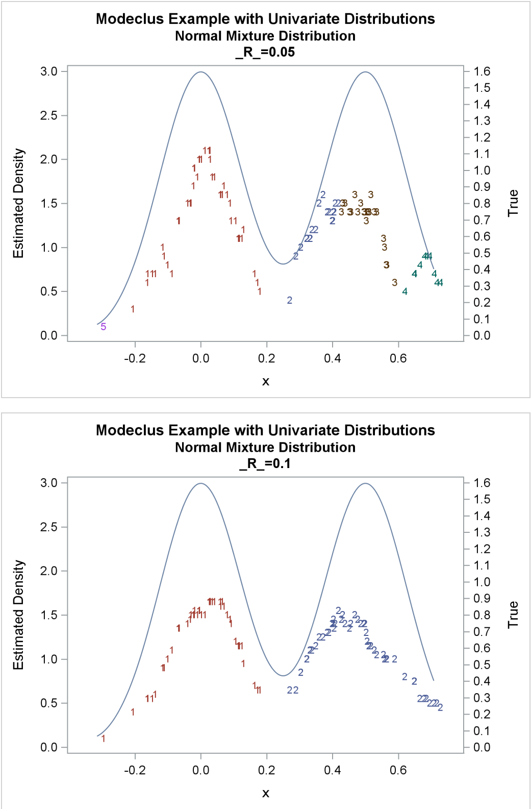
Output 64.1.16 True Density, Estimated Density, and Cluster Membership by Various \_R\_ = Values
