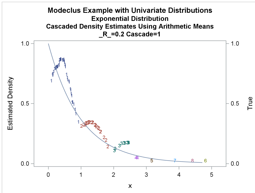
Output 64.1.12 True Density, Estimated Density, and Cluster Membership by \_R_=0.2 with Various \_CASCAD\_ Values
