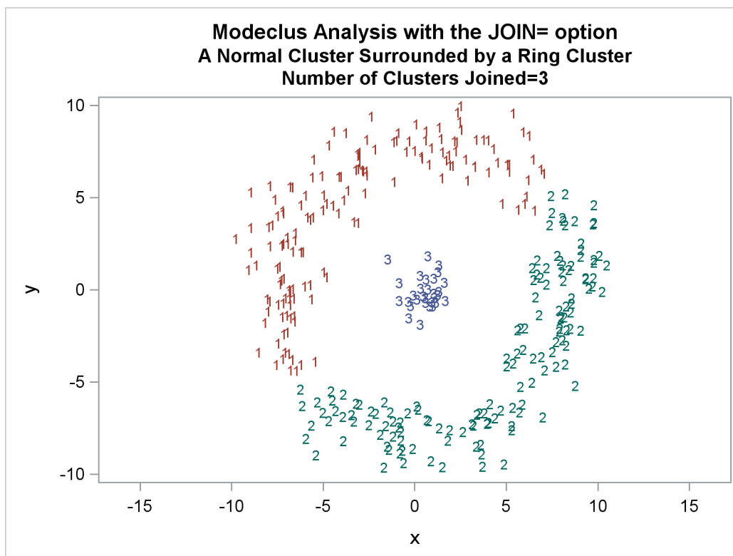
Output 64.3.6 Cluster Memberships When Number of Clusters Joined=3
