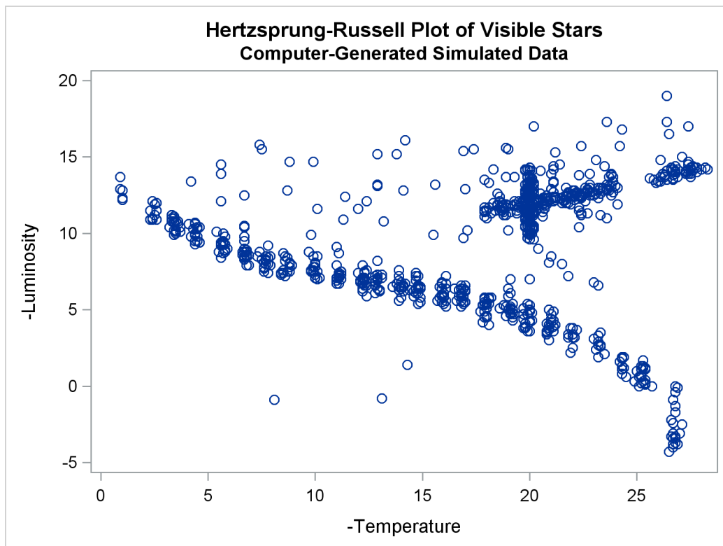
Output 64.4.1 Scatter Plot of Data
