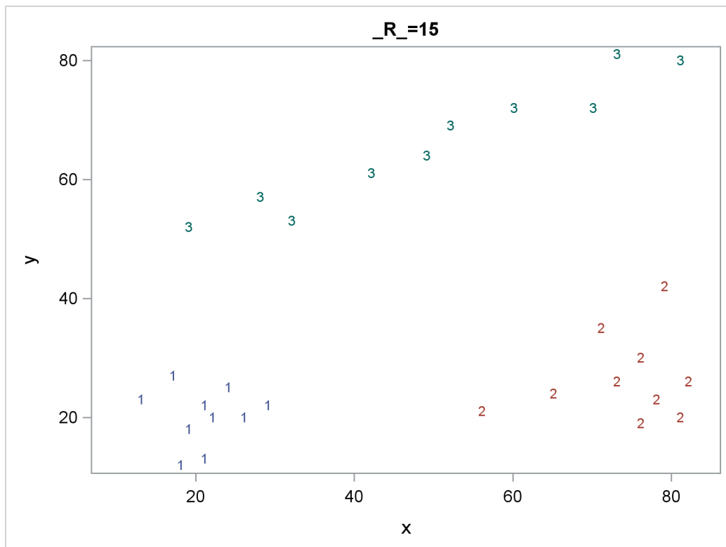
Figure 64.7 Scatter Plots of Cluster Memberships with _R_=15
