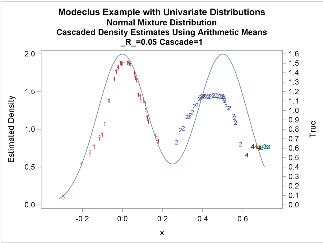
Output 64.1.18 True Density, Estimated Density, and Cluster Membership by _R_=0.05 with Various _CASCAD_ Values
