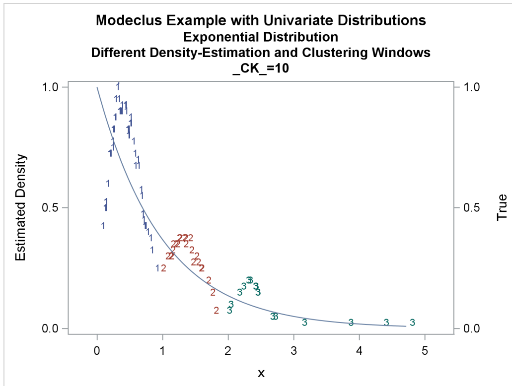
Output 64.1.10 True Density, Estimated Density, and Cluster Membership by \_R_=0.2 with Various \_CK\_ Values
