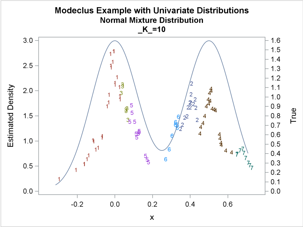
Output 64.1.14 True Density, Estimated Density, and Cluster Membership by Various _K_ Values
