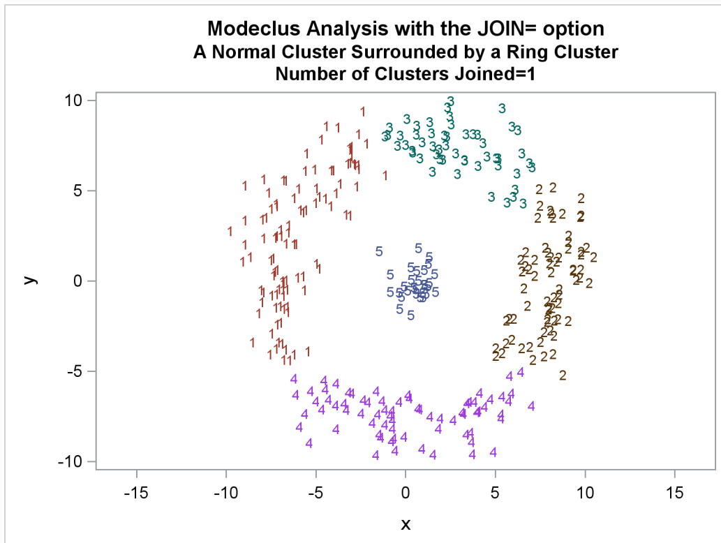
Output 64.3.4 Cluster Memberships When Number of Clusters Joined=1
