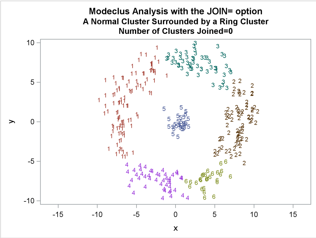
Output 64.3.3 Cluster Memberships When Number of Clusters Joined=0
