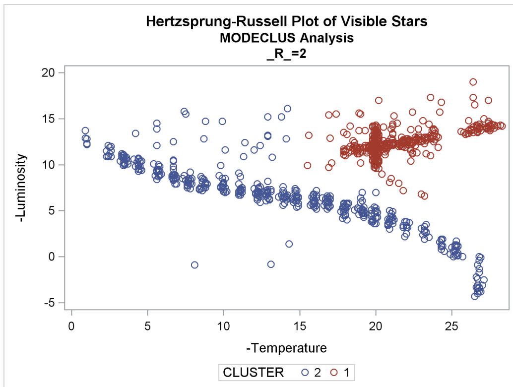
Output 64.4.5 Scatter Plots of Cluster Memberships by _R_=2
