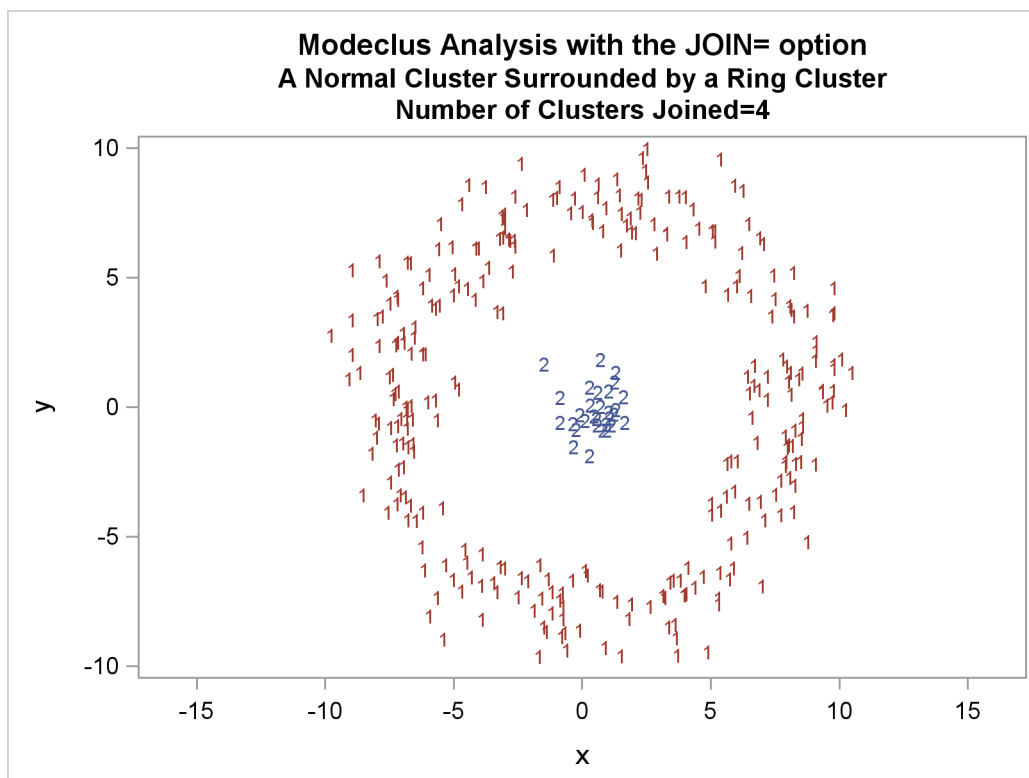
Output 64.3.7 Cluster Memberships When Number of Clusters Joined=4
