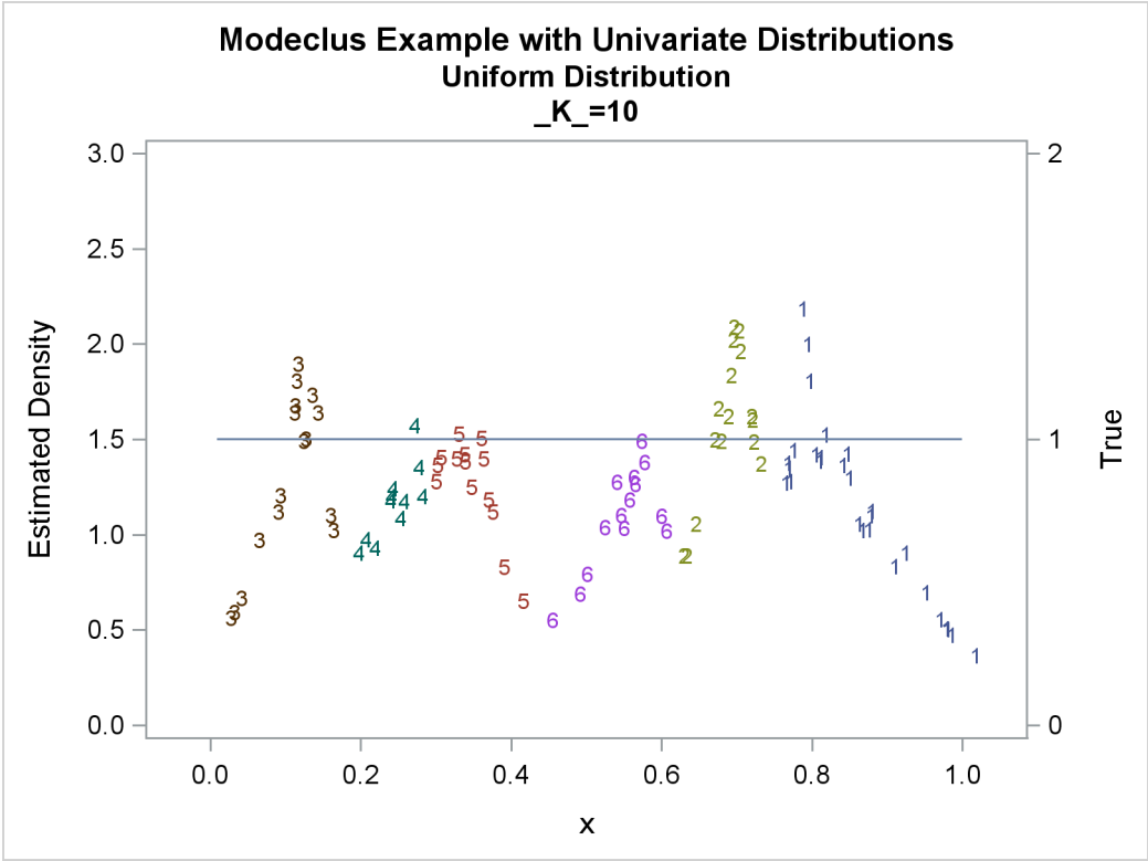
Output 64.1.2 True Density, Estimated Density, and Cluster Membership by Various _K_ Values
