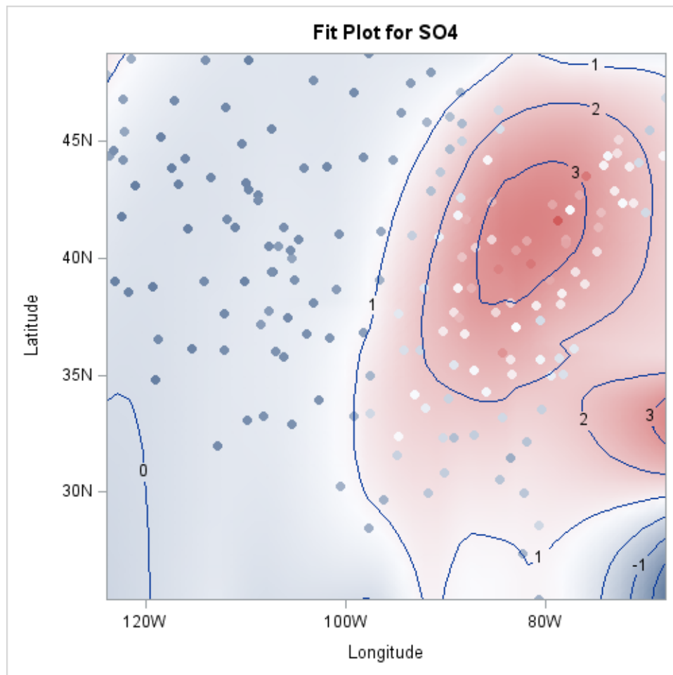
Output 57.2.2 Fit Plot for the SO 4 Data
