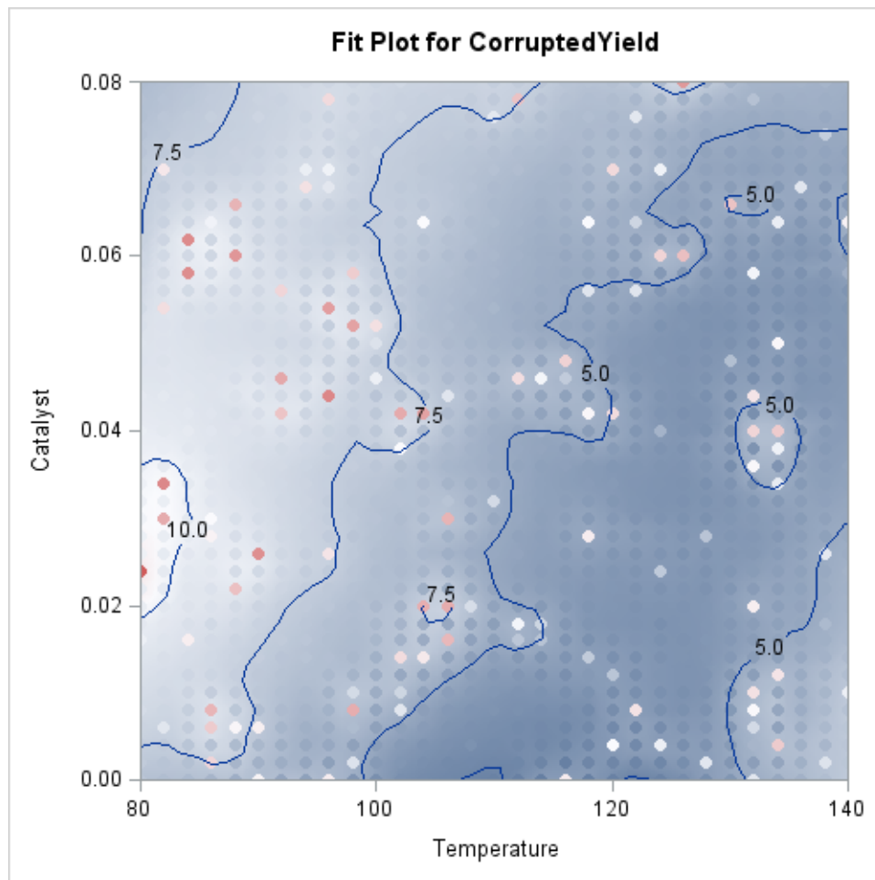
Output 57.3.4 Fit for CorruptedYield
