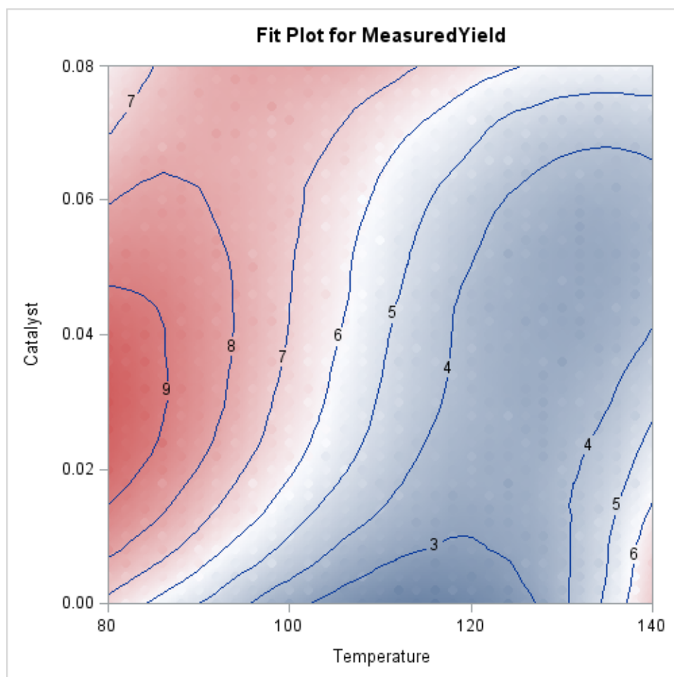
Output 57.3.3 Fit for MeasuredYield
