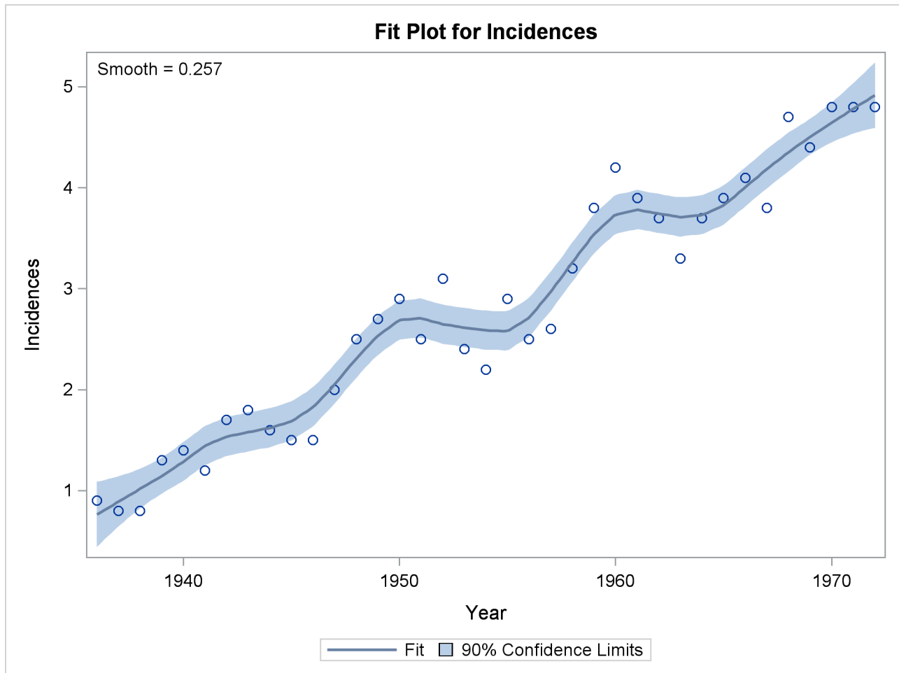
Figure 57.13 Loess Fit of Melanoma Data with 90% Confidence Limits
