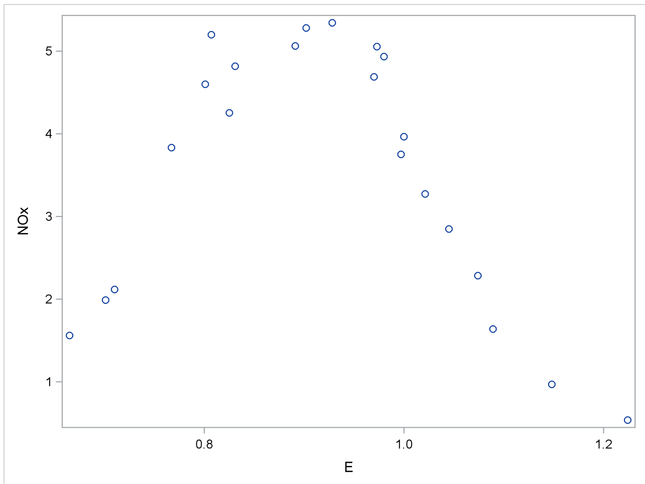
Output 57.1.1 Scatter Plot of the Gas Data
