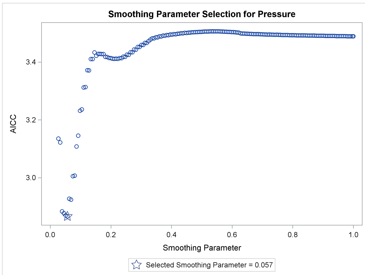
Output 57.4.5 AICC versus Smoothing Parameter Showing Local Minima
