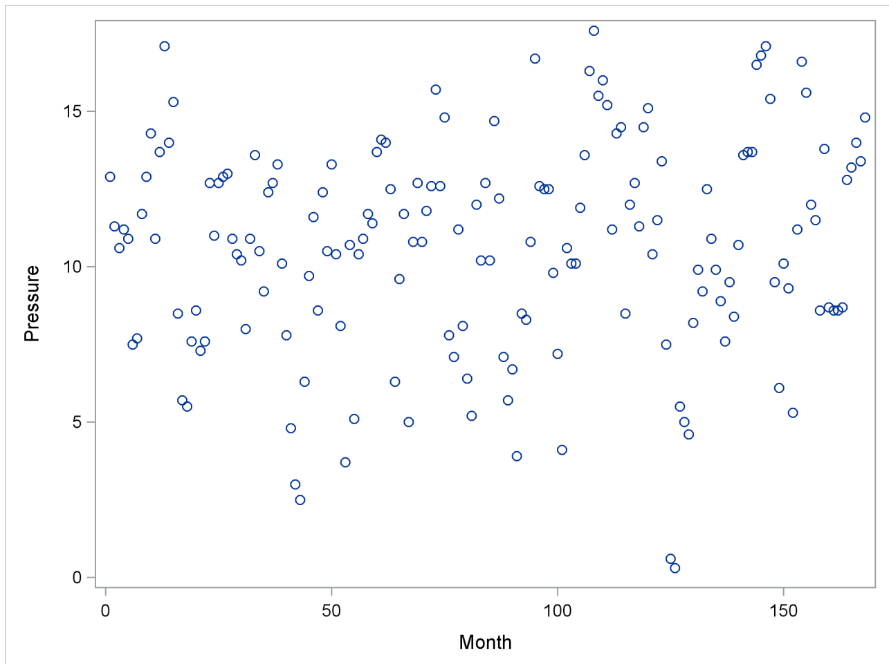
Output 57.4.1 Scatter Plot of ENSO Data
