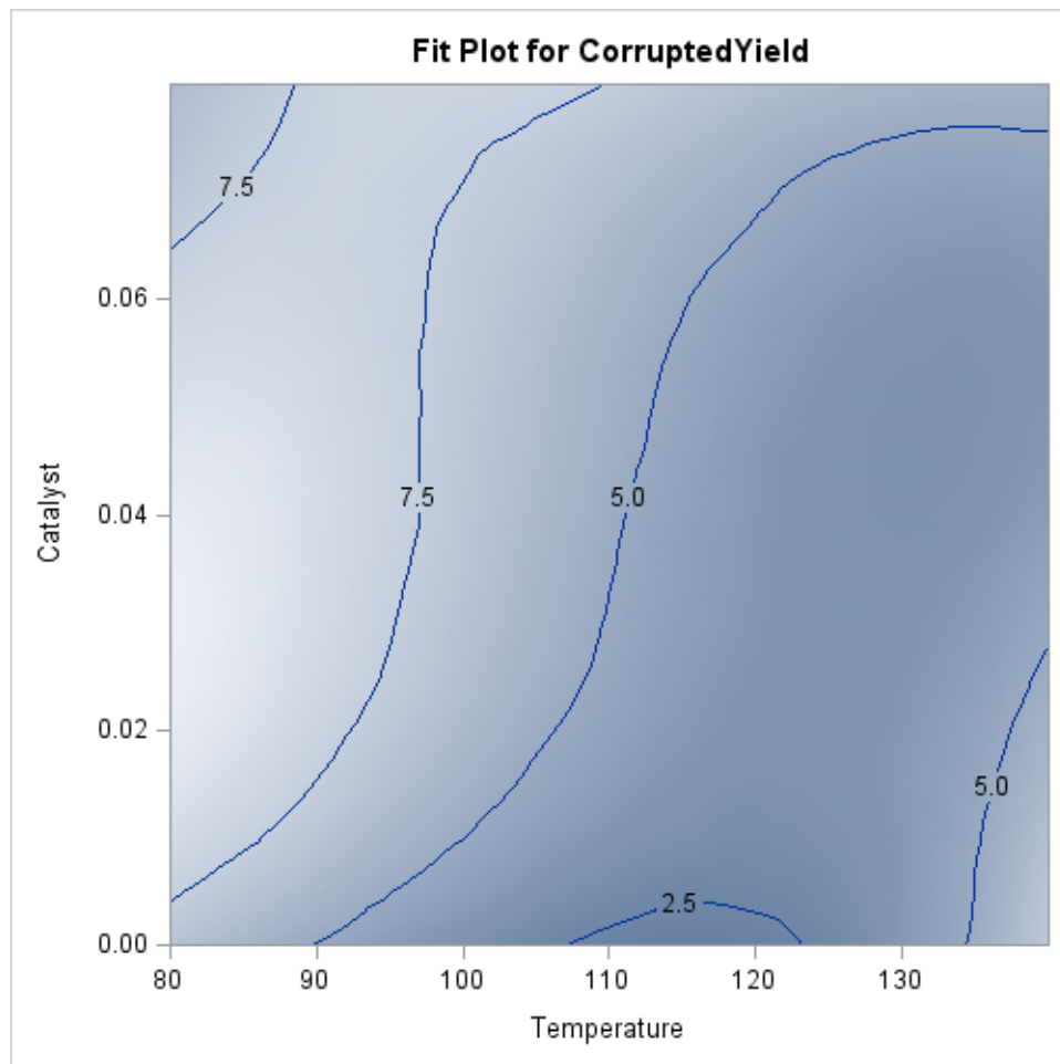
Output 57.3.6 Robust Fit for CorruptedYield with Observations Suppressed
