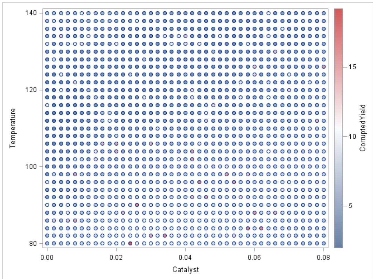
Output 57.3.1 Scatter Plot of Experiment Data Colored by CorruptedYield
