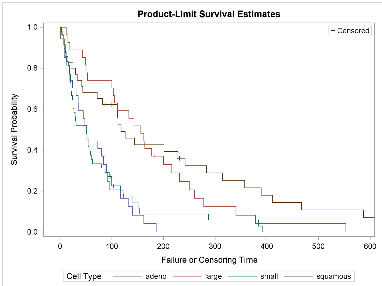
Output 56.1.6 Graph of the Estimated Survivor Functions
