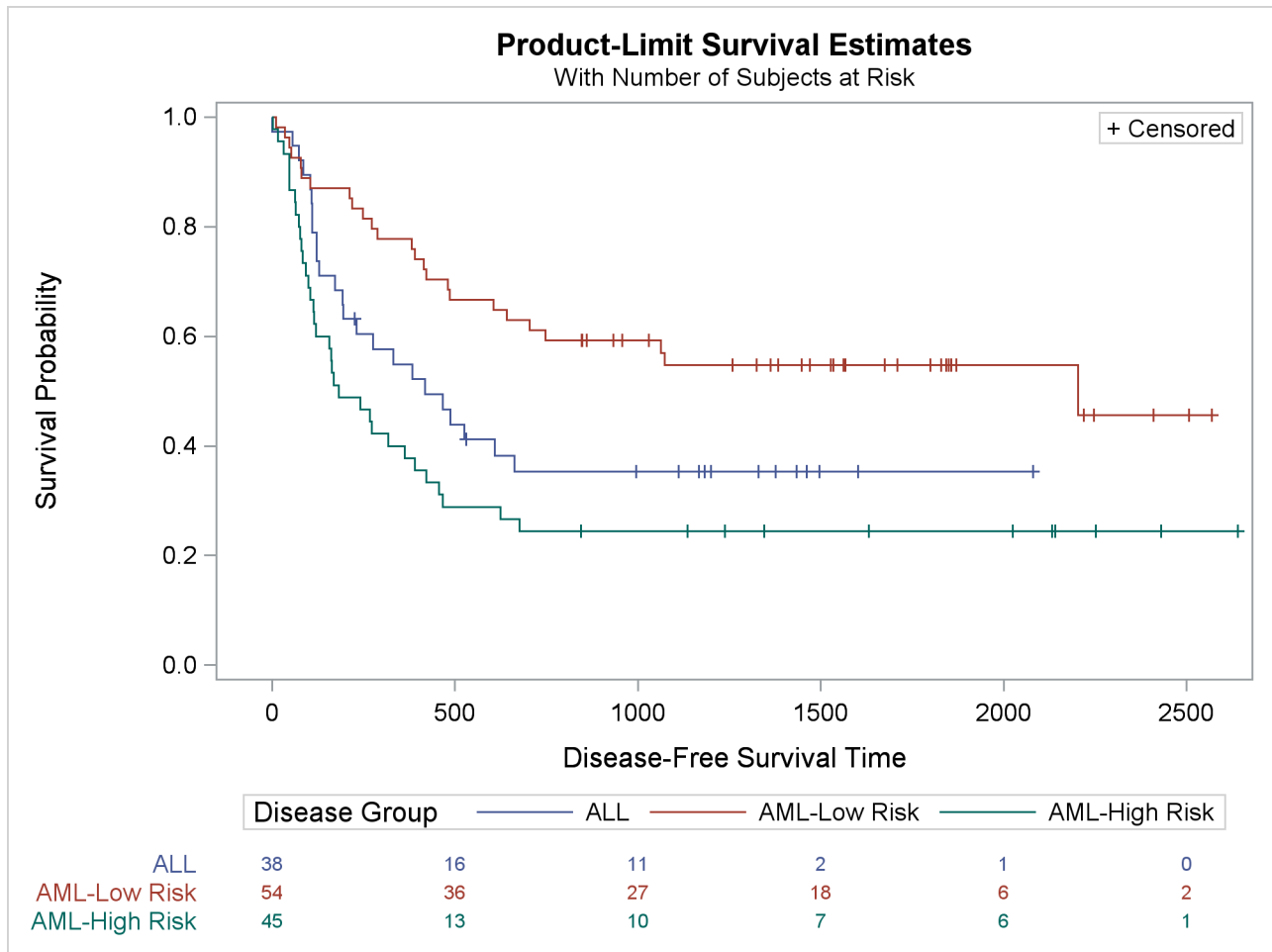
Output 56.2.6 Modified Disease-Free Survival for Bone Marrow Transplant Patients
