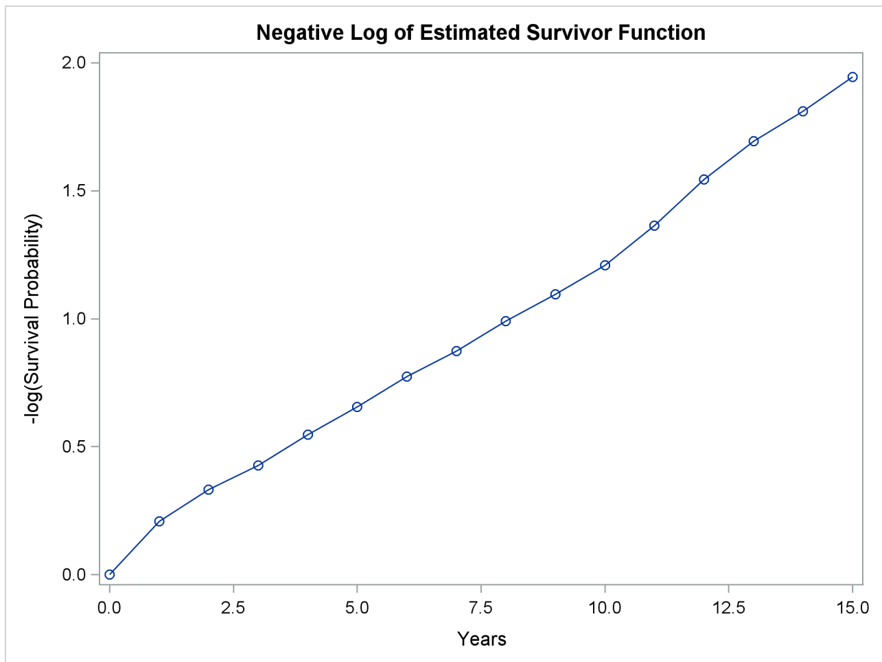
Output 56.3.4 Negative Log of Survivor Function Estimate
