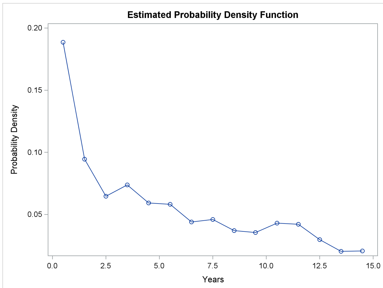
Output 56.3.7 Density Function Estimate
