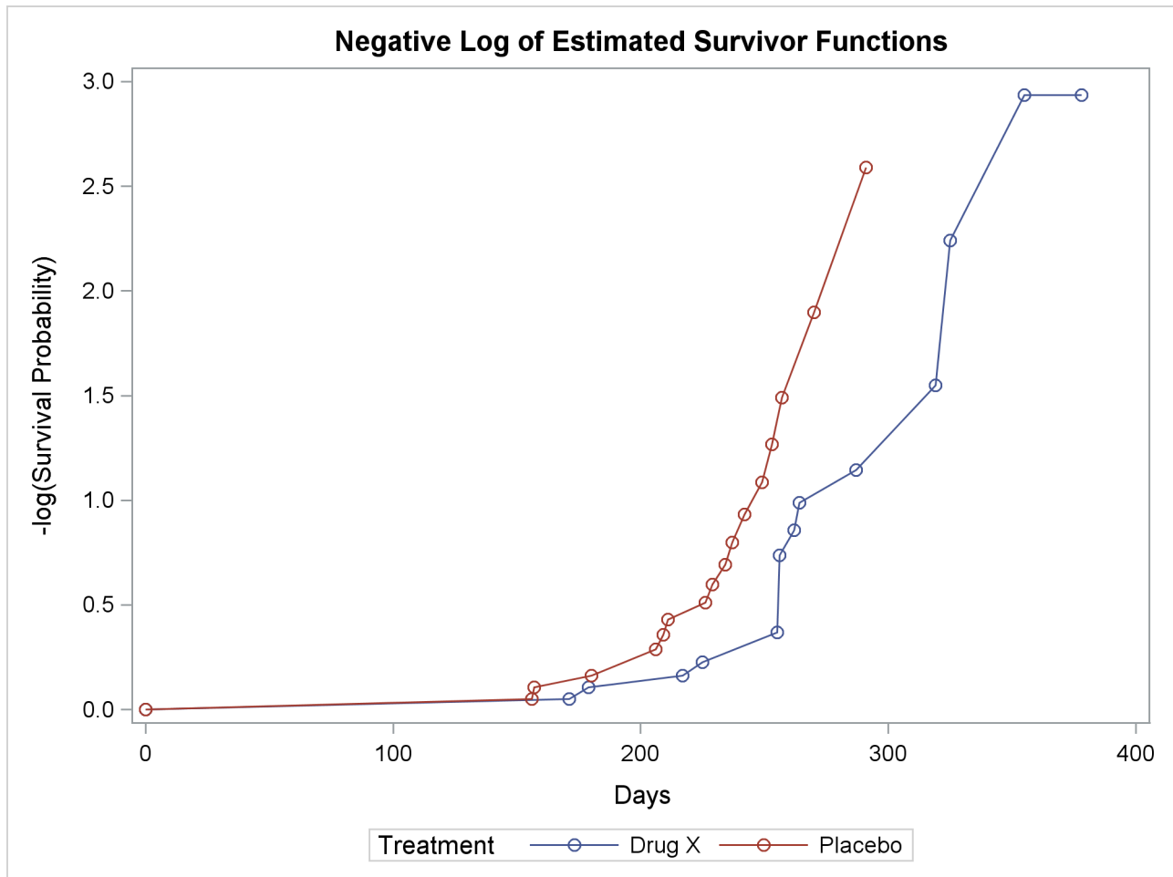
Figure 56.7 Plot of Estimated Negative Log Survivor Functions
