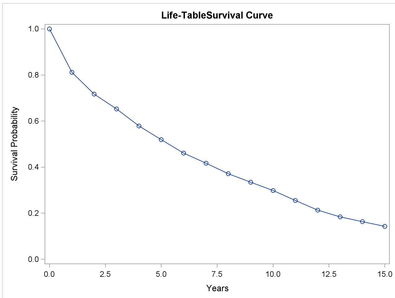
Output 56.3.3 Life-Table Survivor Function Estimate
