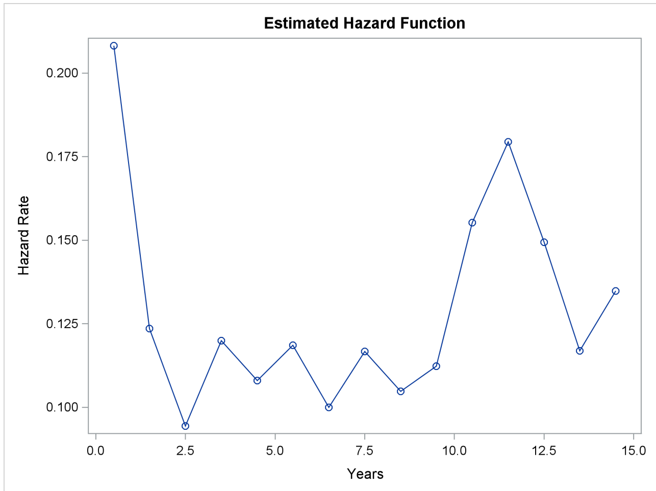
Output 56.3.6 Hazard Function Estimate
