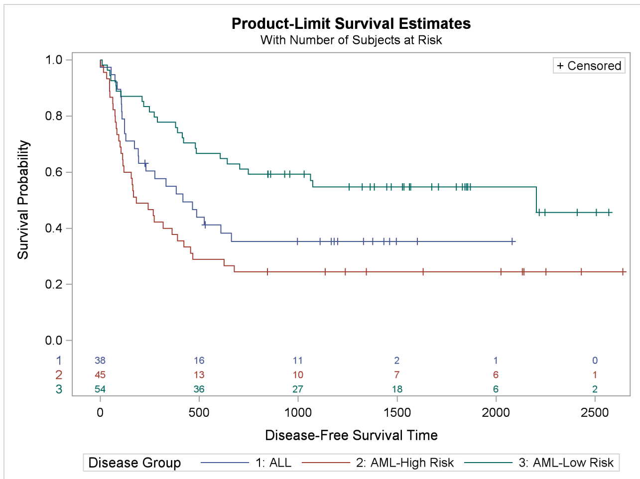
Output 56.2.2 Estimated Disease-Free Survival for 137 Bone Marrow Transplant Patients
