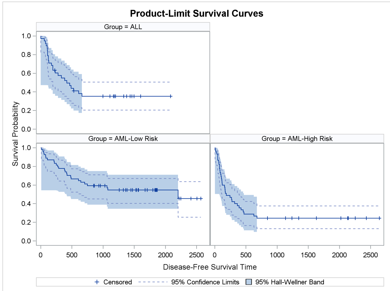
Output 56.2.7 Estimated Disease-Free Survivor Functions with Confidence Limits
