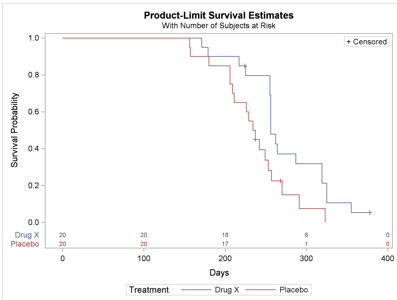
Figure 56.6 Plot of Estimated Survivor Functions
