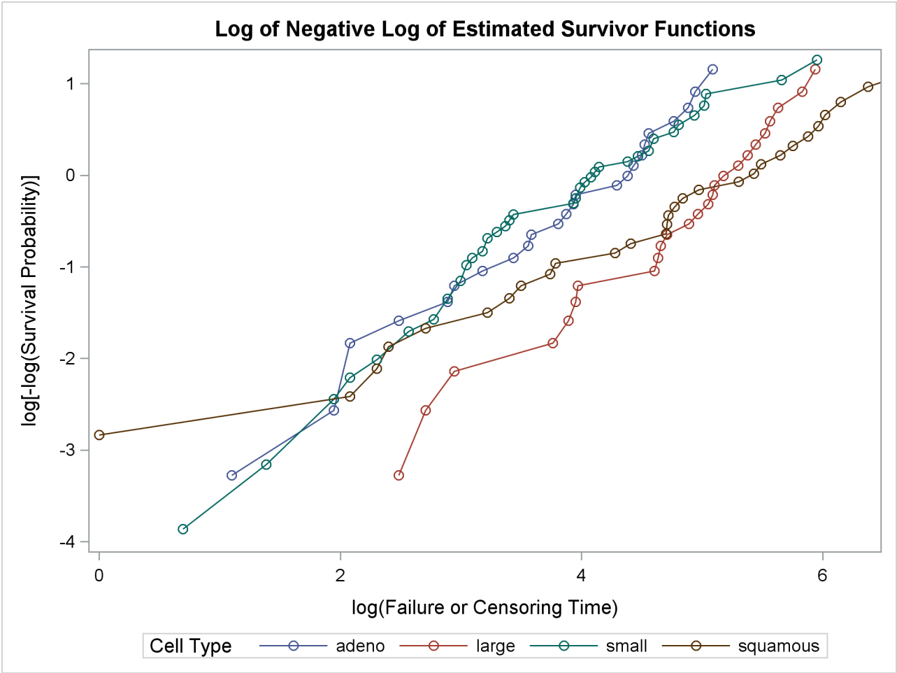
Output 56.1.8 Graph of Log of the Negative Log of the Estimated Survivor Functions
