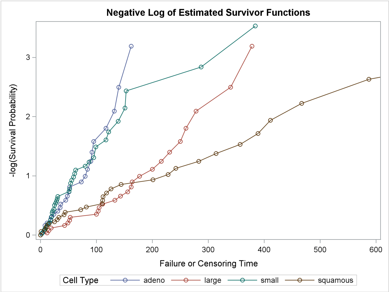
Output 56.1.7 Graph of Negative Log of the Estimated Survivor Functions
