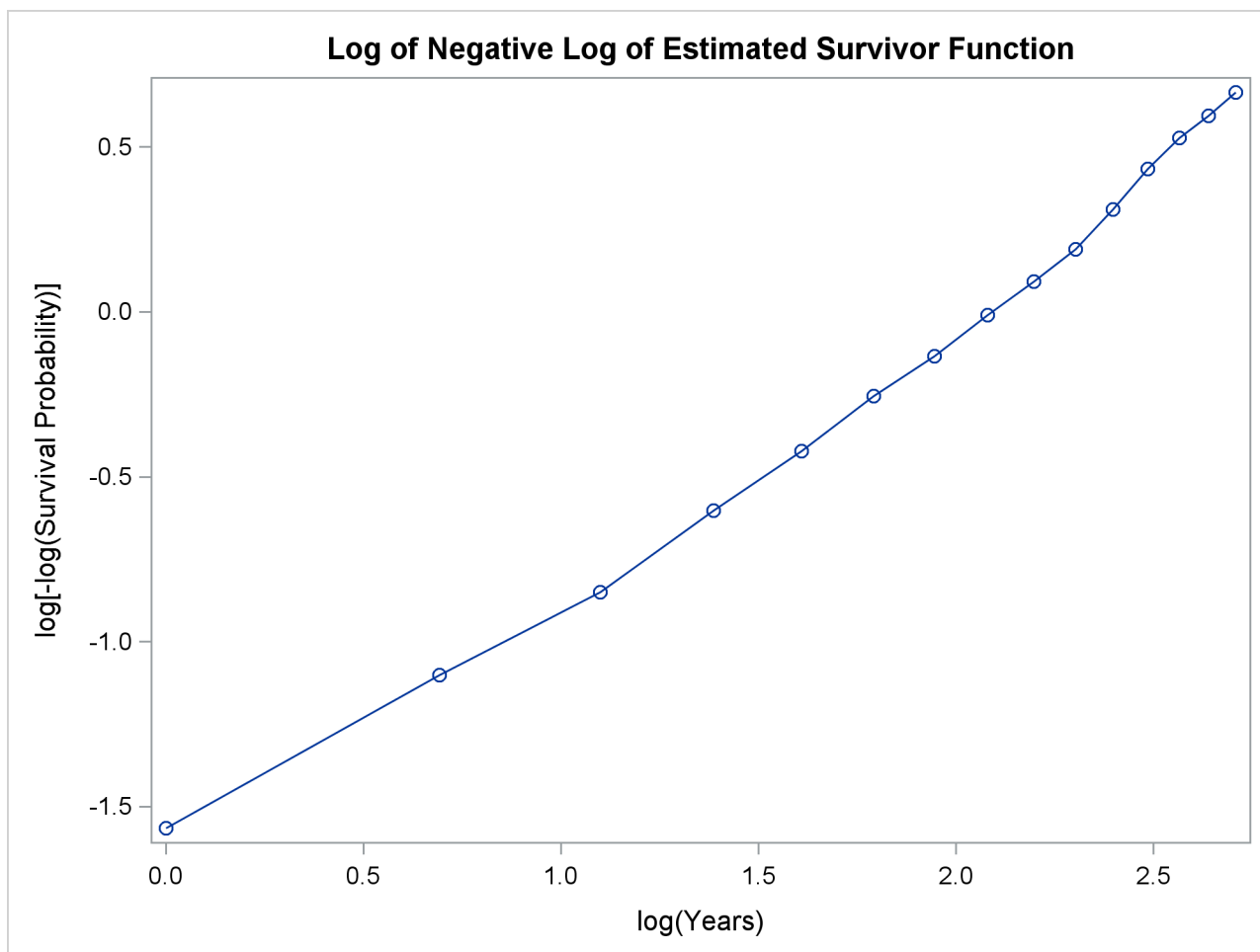
Output 56.3.5 Log of Negative Log of Survivor Function Estimate
