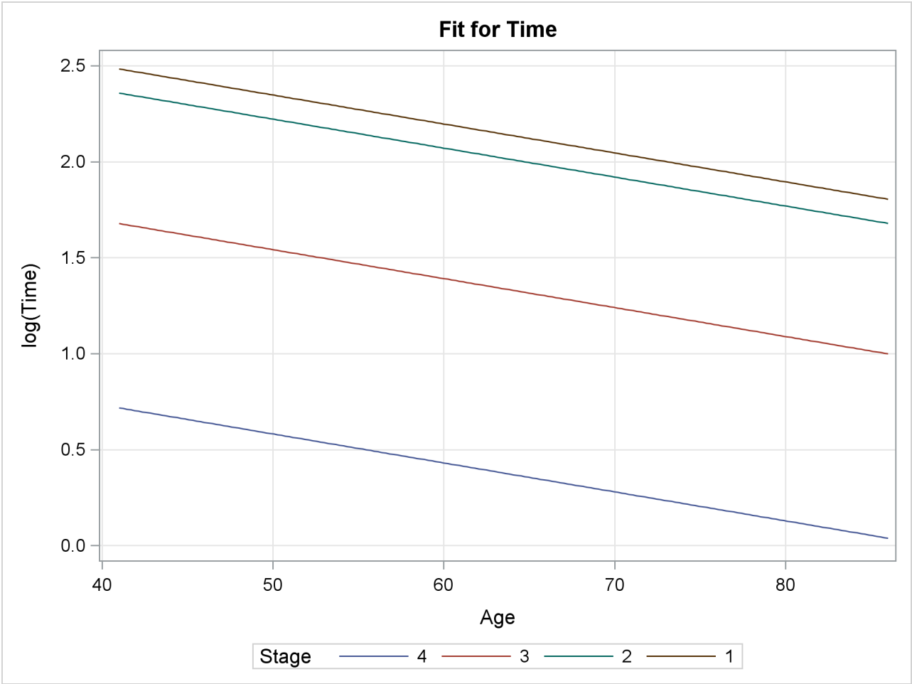
Output 55.8.4 Age Effects by Disease Stages
