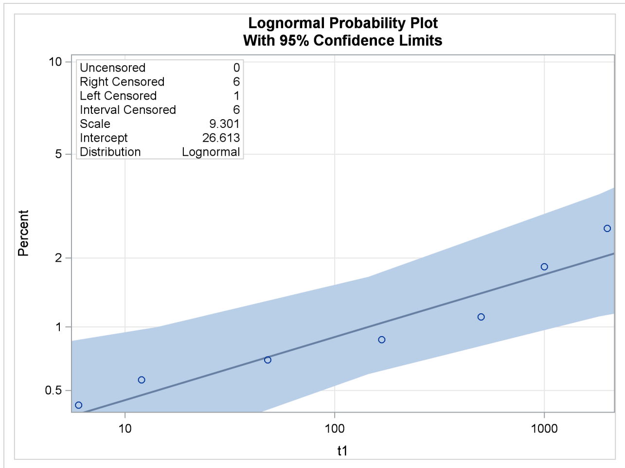
Output 55.6.4 Lognormal Probability Plot for the Microprocessor Data
