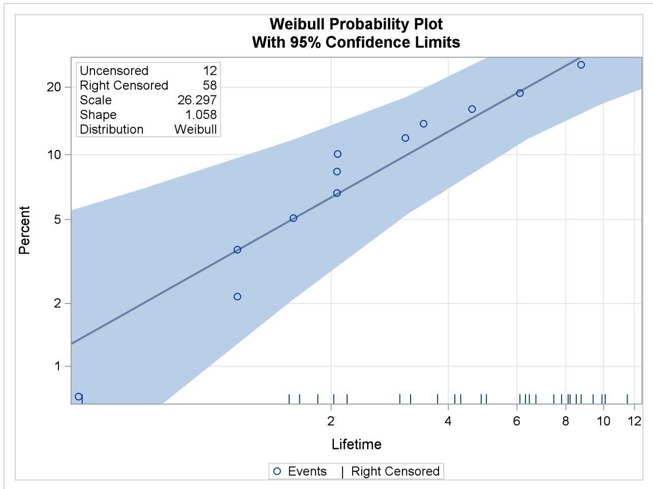
Output 55.5.1 Probability Plot for the Fan Data
