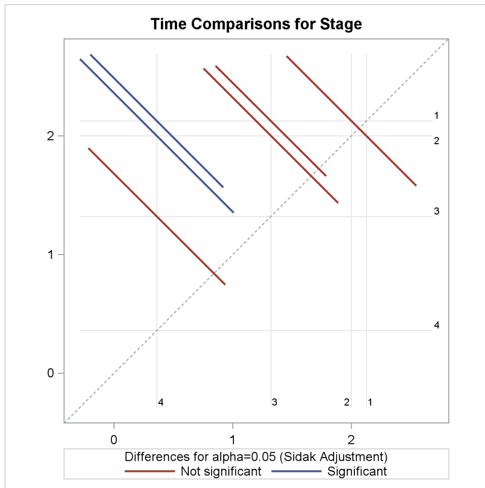
Output 55.8.2 Plot of Pairwise LS-Means Differences
