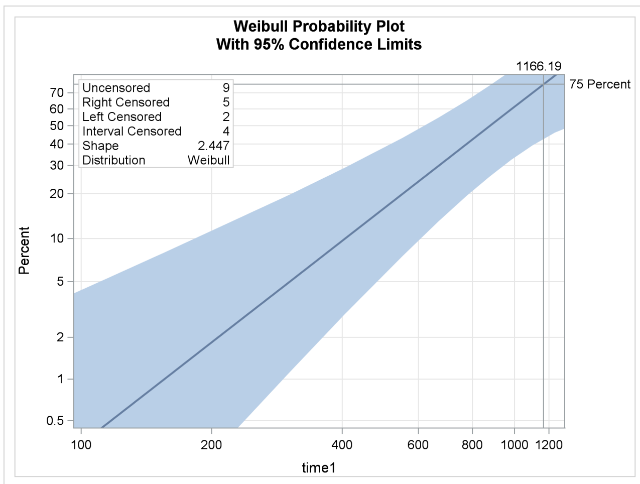
Output 55.4.3 Probability Plot for Recovery Time with sex = 2, age = 60.6
