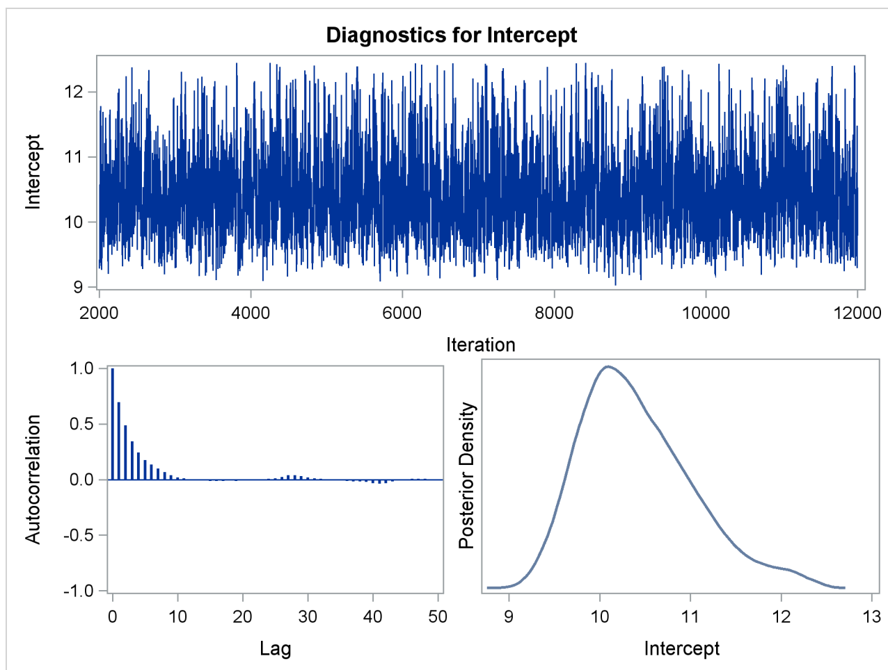
Figure 55.11 Diagnostic Plots
