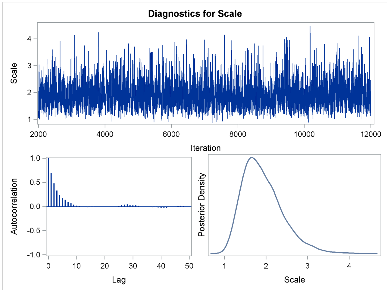
Figure 55.12 Diagnostic Plots
