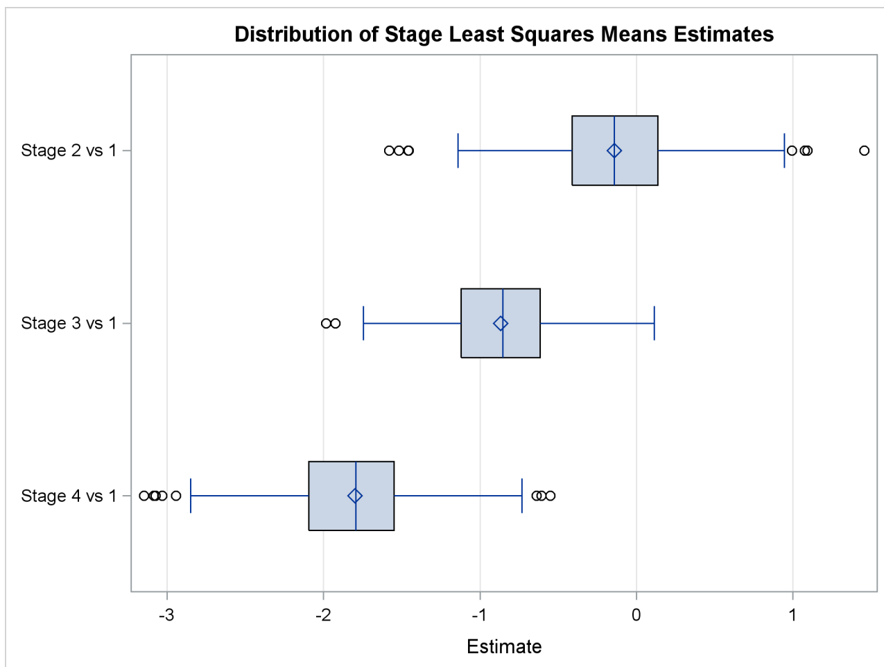
Output 55.8.8 Box Plot of Sampled LS-Means Differences
