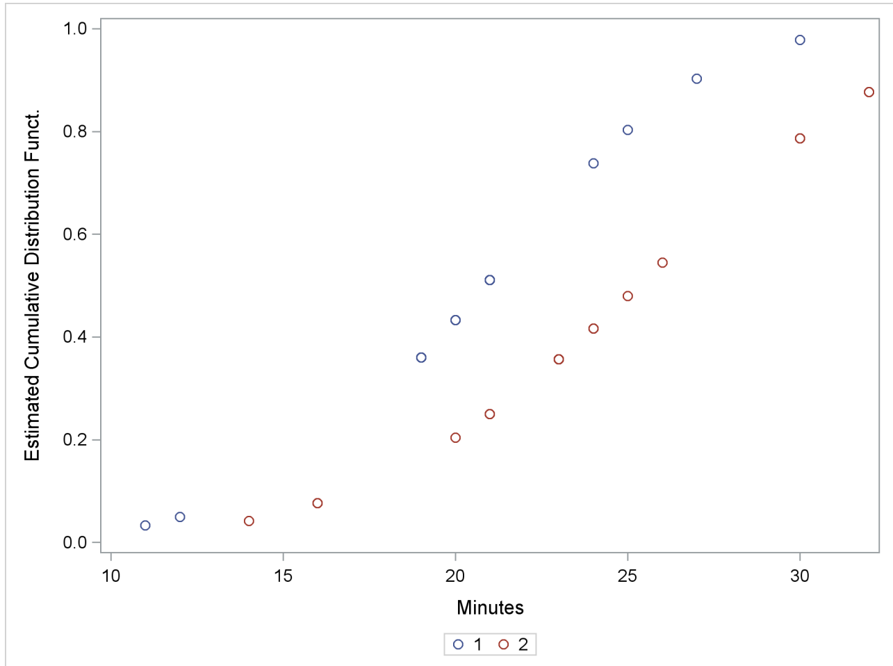
Figure 55.5 Plot of the Estimated Cumulative Distribution Function
