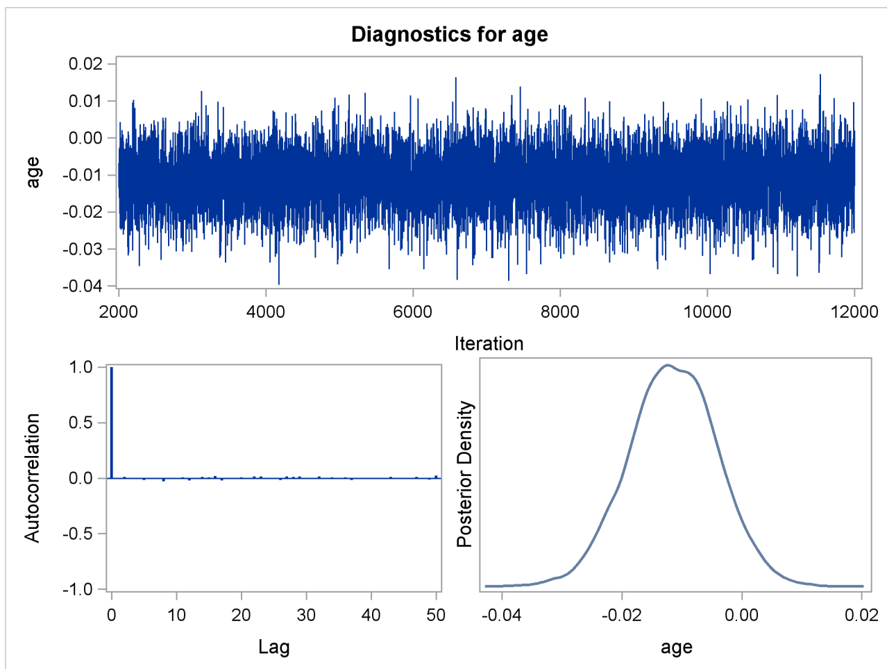
Output 55.7.7 Diagnostic Plots
