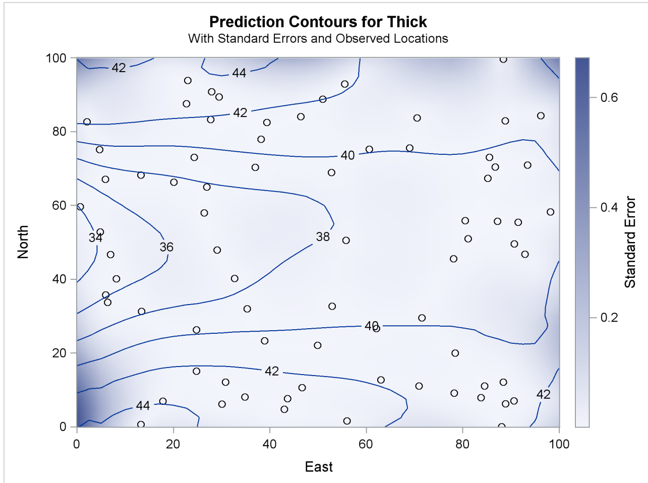
Figure 53.4 Contour Plot of Kriged Coal Seam Thickness
