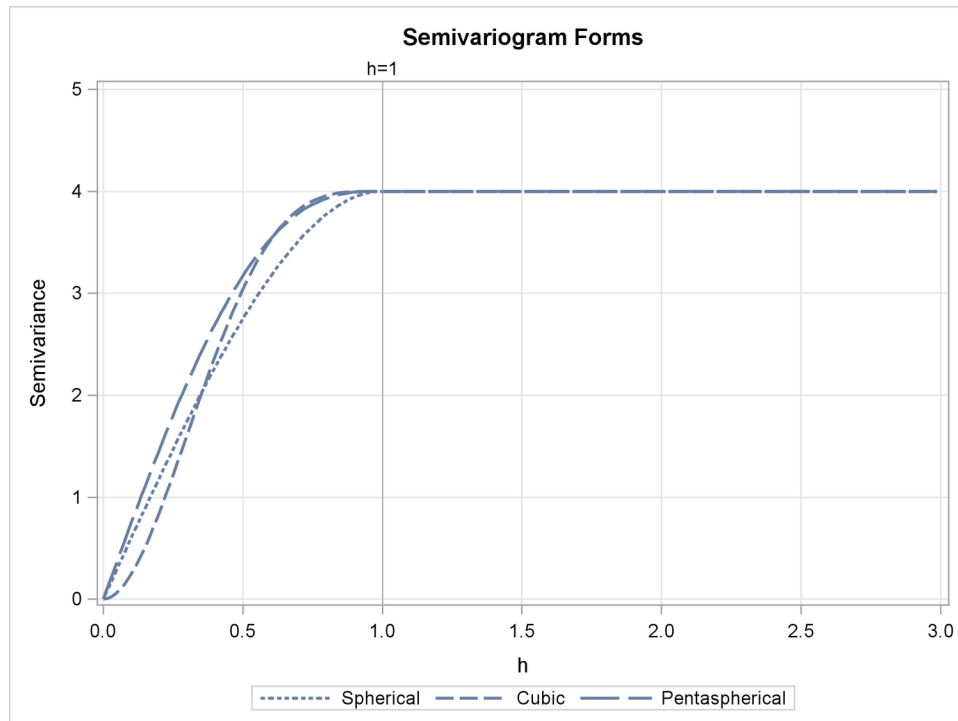
Figure 53.7 Spherical, Cubic, and Pentaspherical Semivariograms with Parameters a_0 = 1 and c_0 = 4
