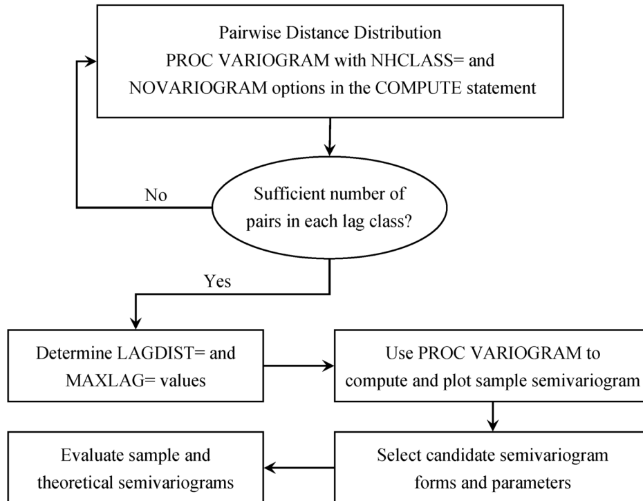
Figure 53.5 Flowchart for Semivariogram Selection
