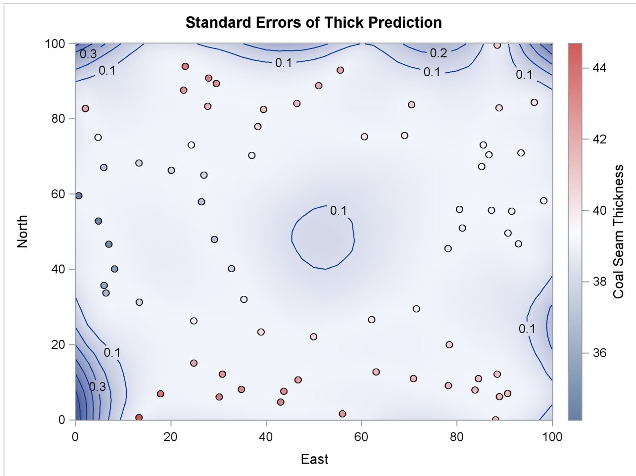
Output 53.3.4 Surface Plot and Contours of Prediction Standard Errors
