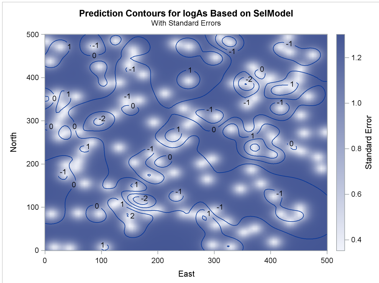
Output 53.1.7 Predicted Arsenic Logarithm Values with Gaussian-Gaussian Covariance
