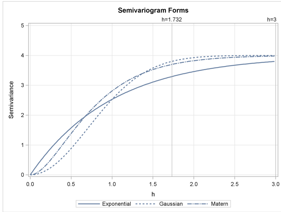
Figure 53.6 Gaussian, Exponential, and Matérn Semivariograms with Parameters a_0 = 1 , c_0 = 4 , and \nu = 1.5
