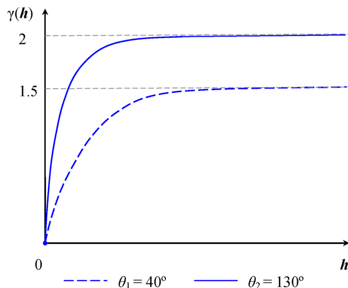
Figure 53.15 Zonal Anisotropy in Two Directions
