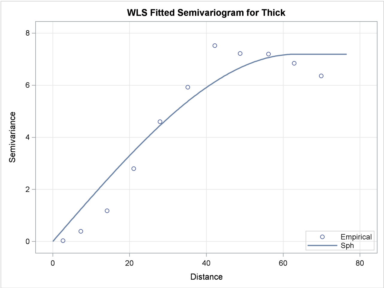
Output 53.2.3 Fitted Spherical and Empirical Thick Semivariogram
