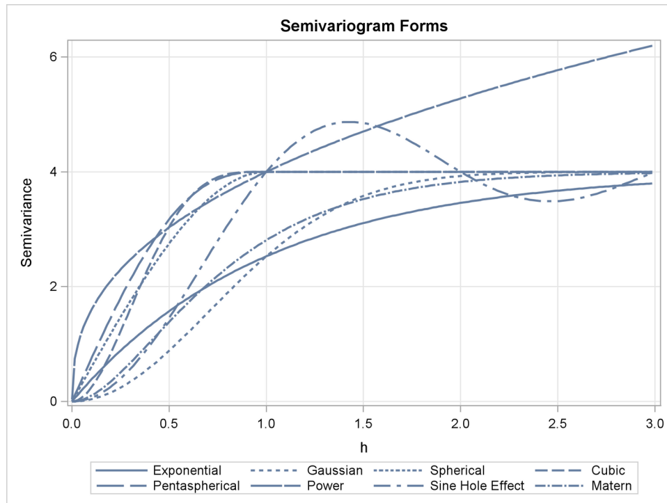
Figure 53.9 Semivariogram Forms Used in PROC KRIGE2D
