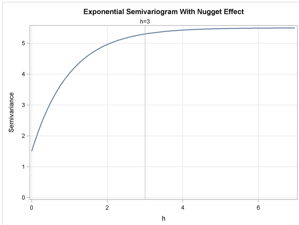
Figure 53.11 Exponential Semivariogram Model with a Nugget Effect c_n = 1.5
