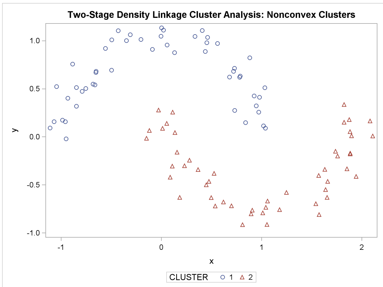
Figure 11.26 Nonconvex Clusters: PROC CLUSTER METHOD=TWOSTAGE
