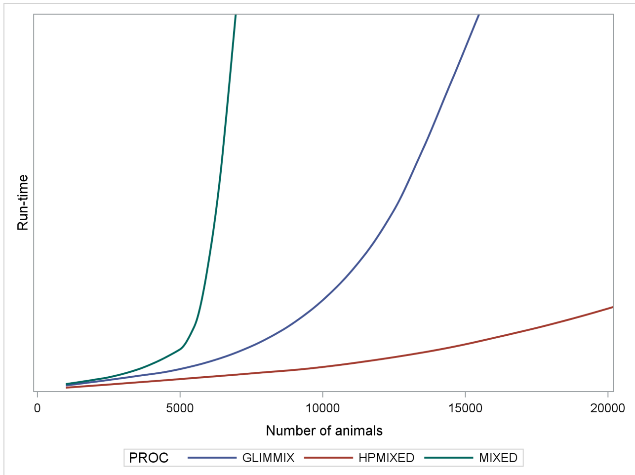
Output 48.1.2 Comparing Mixed Model Tools for Increasingly Sparse Problems
