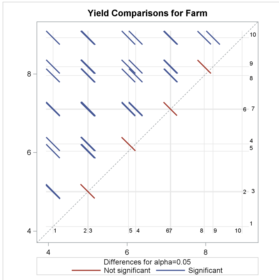
Output 48.3.3 LS-Means Plot of Pairwise Farm Differences
