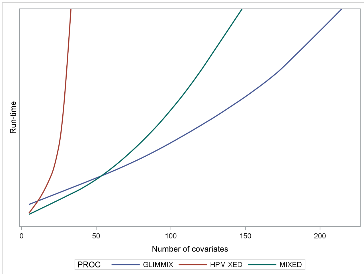
Output 48.1.3 Comparing Mixed Model Tools for Increasingly Dense Problems
