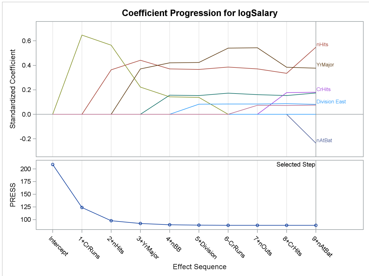
Output 47.1.4 Coefficient Progression Plot
