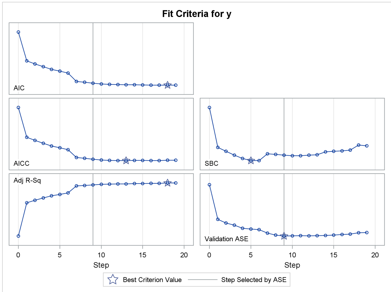
Output 47.2.5 Criterion Panel
