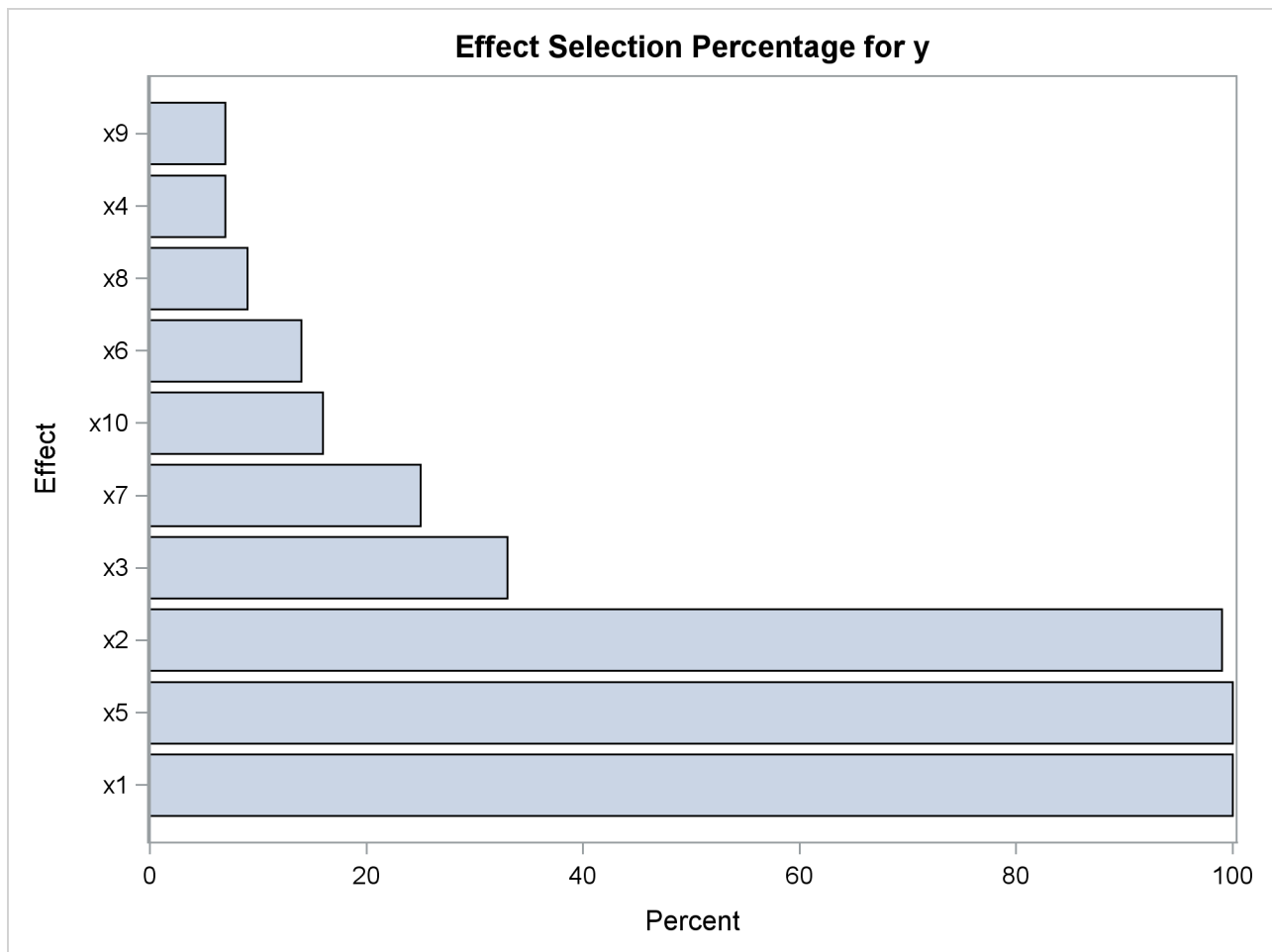
Output 47.5.4 Effect Selection Percentages
