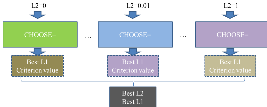
Figure 47.12 Estimation of the Ridge Regression Parameter \lambda_2 (L2) in the Elastic Net Method
