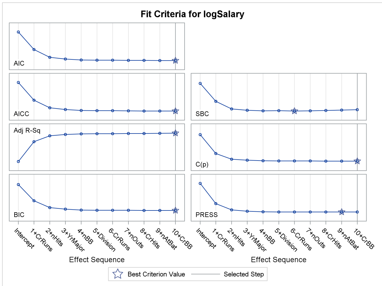
Output 47.1.1 Criterion Panel
