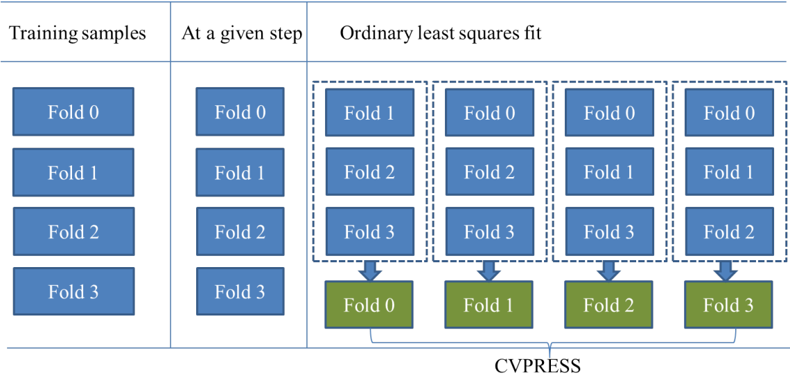
Figure 47.18 Applying k -fold Cross Validation to Computing the CVPRESS Statistic
