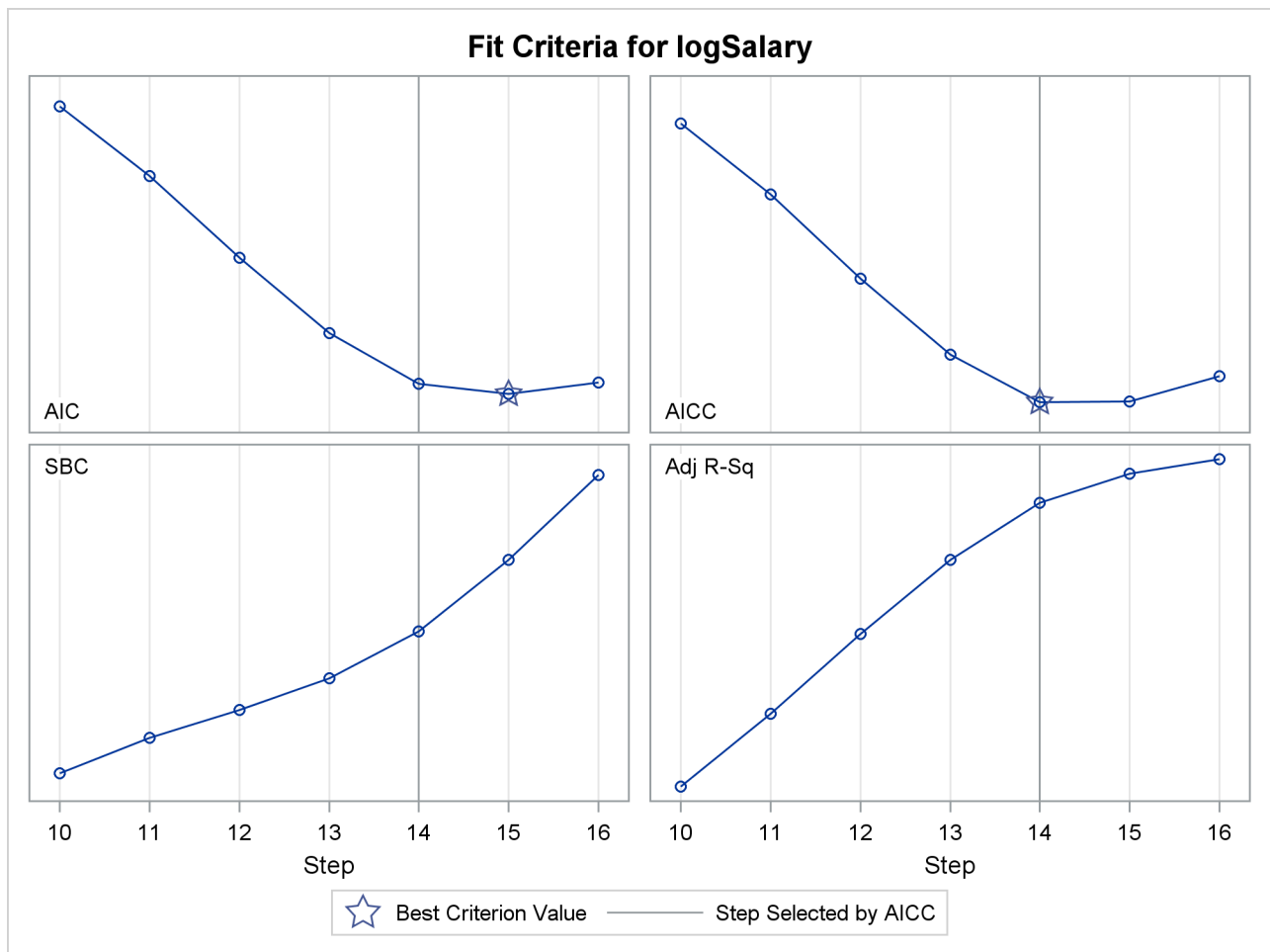
Figure 47.23 Criterion Panel for Specified Step Range
