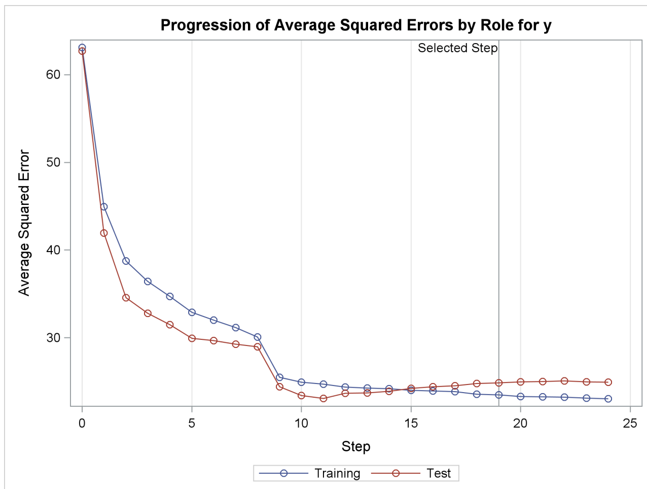
Output 47.2.14 Average Squared Error Plot
