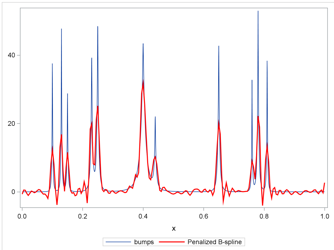
Output 47.3.3 Penalized B-spline Fit
