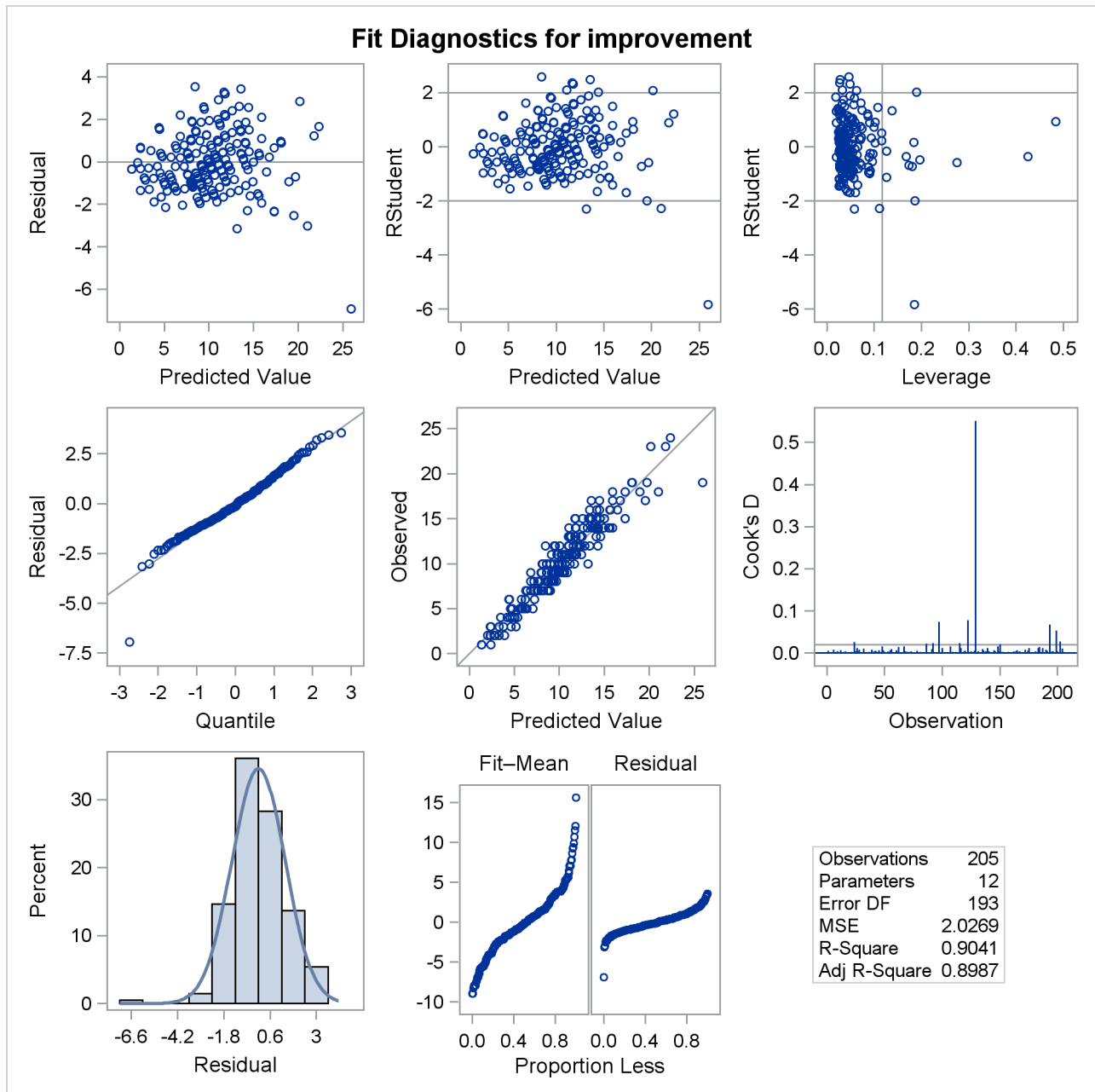
Output 47.4.4 Fit Diagnostics
