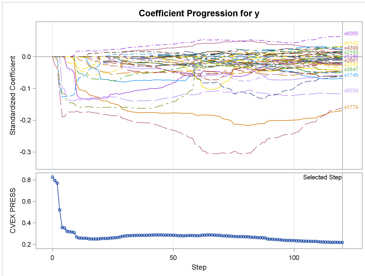
Output 47.6.11 Elastic Net Coefficient Progression Plot
