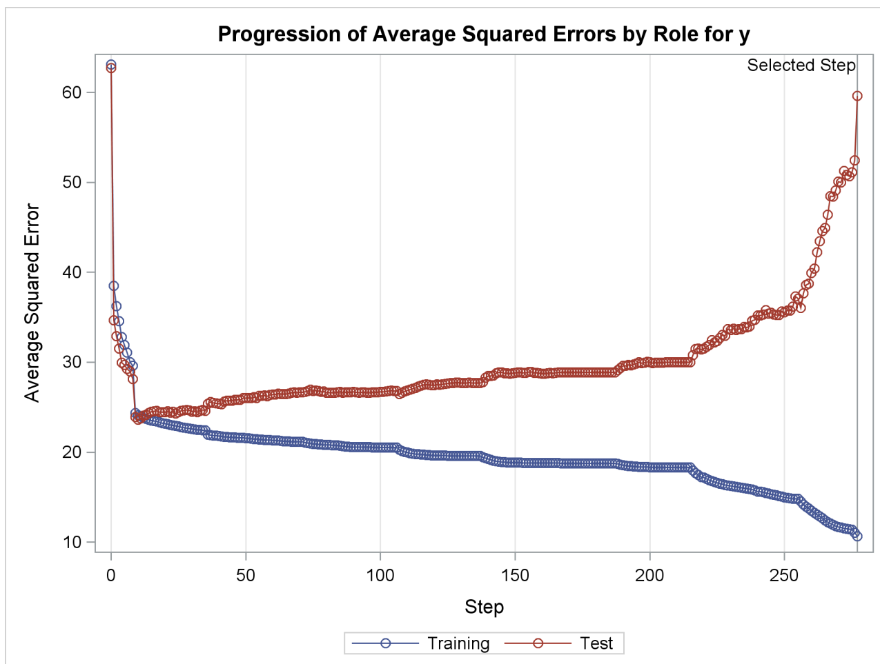
Output 47.2.18 Average Squared Error Plot
