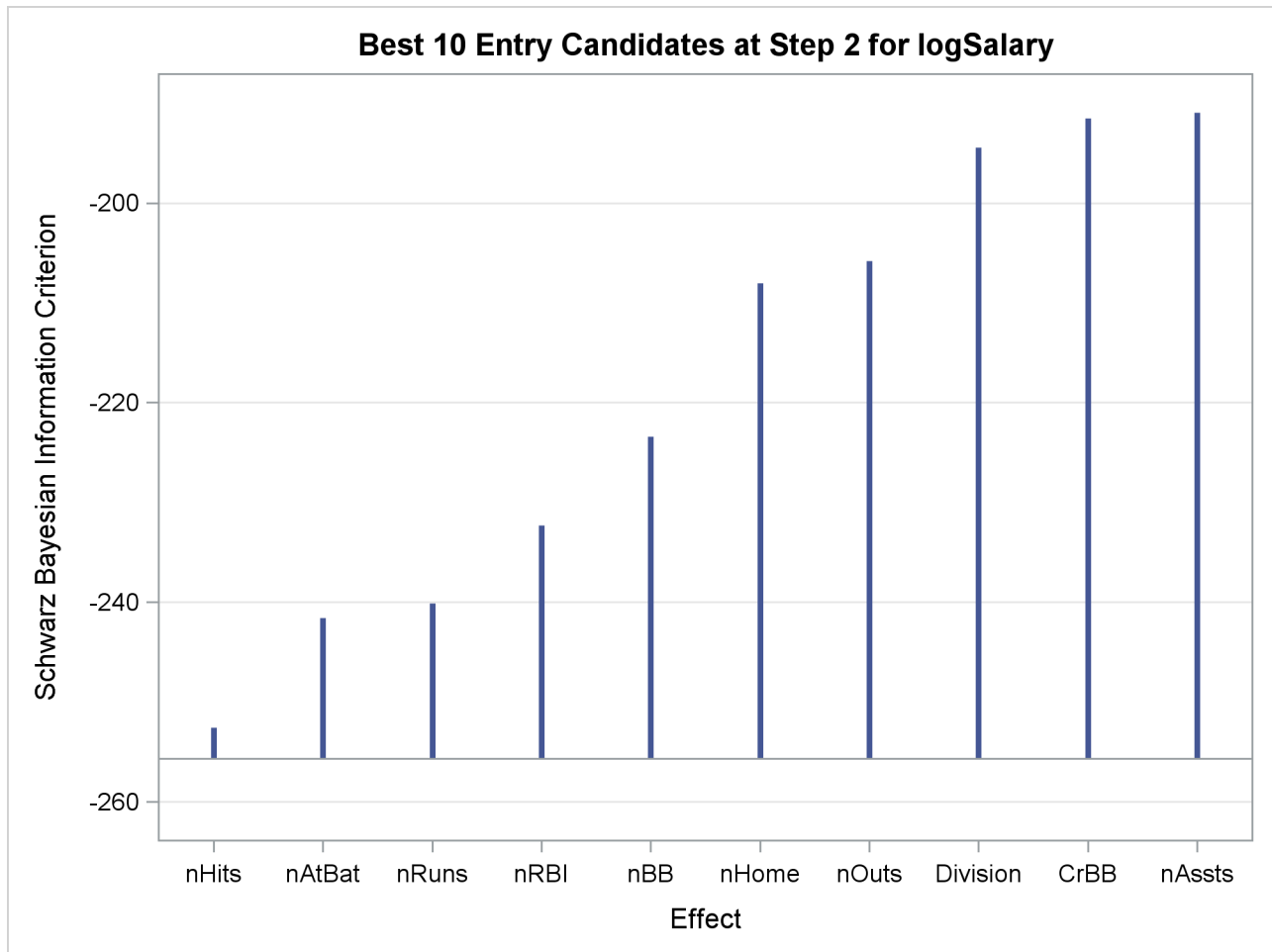
Figure 47.6 Needle Plot of Entry Candidates at Step Two
