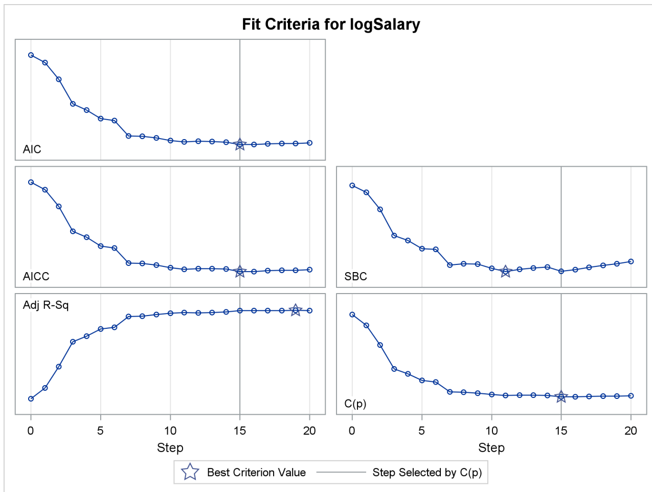
Output 47.1.11 Criterion Panel
