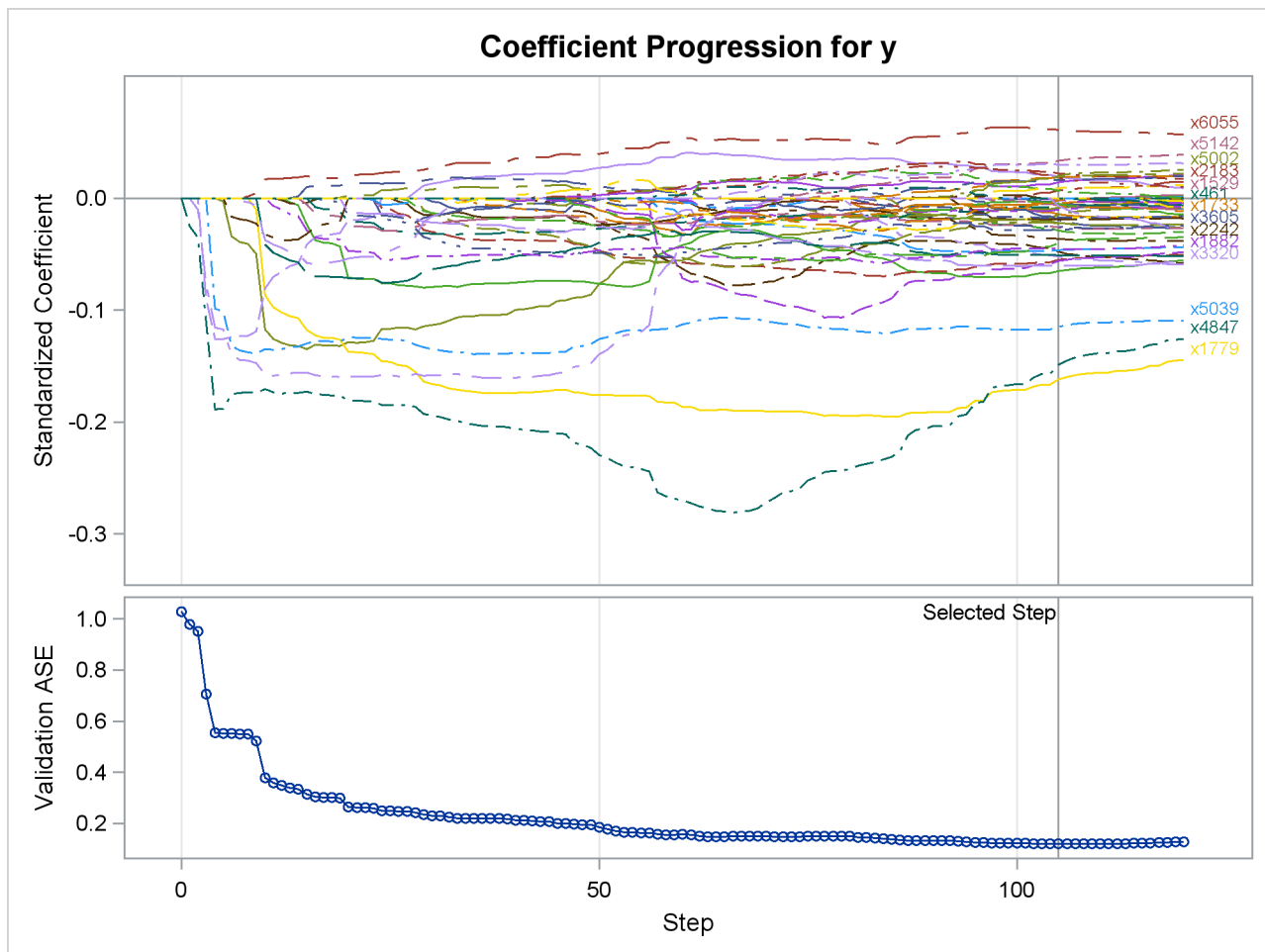
Output 47.6.6 Elastic Net Coefficient Progression Plot
