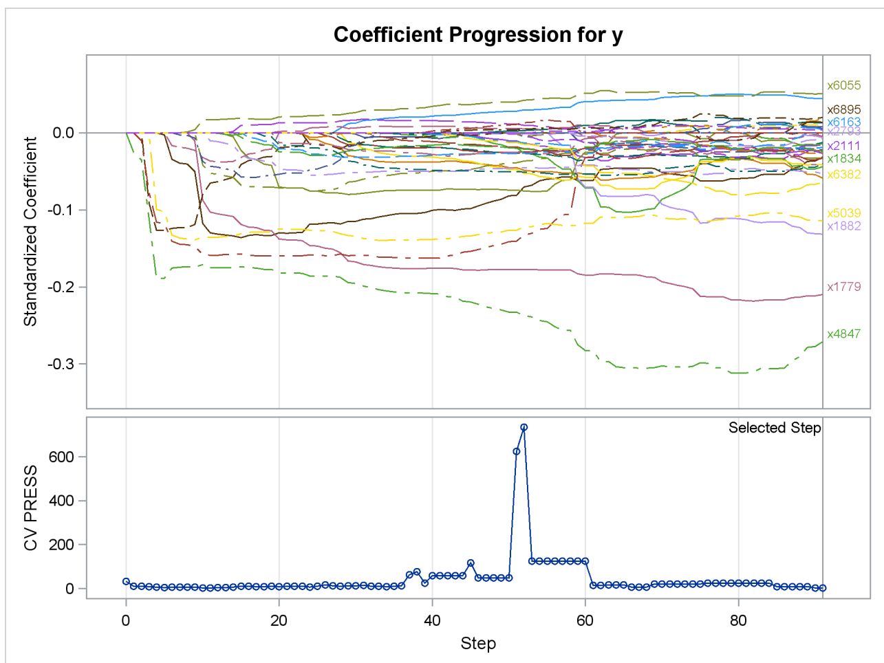
Output 47.6.10 Elastic Net Coefficient Progression Plot
