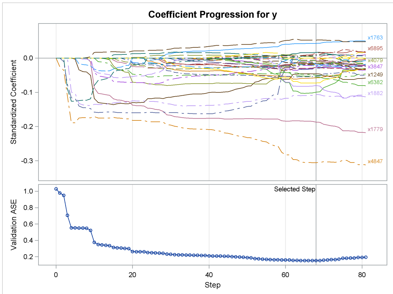
Output 47.6.4 LASSO Coefficient Progression Plot
