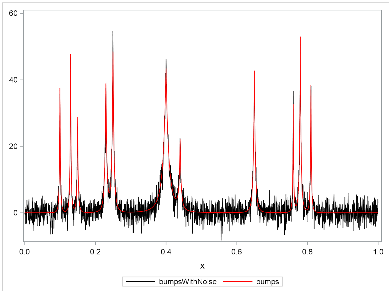
Output 47.3.1 Donoho-Johnstone Bumps Function
