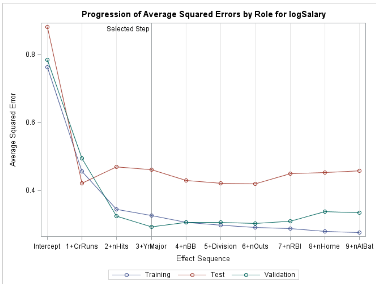
Output 47.1.9 Average Square Errors by Role
