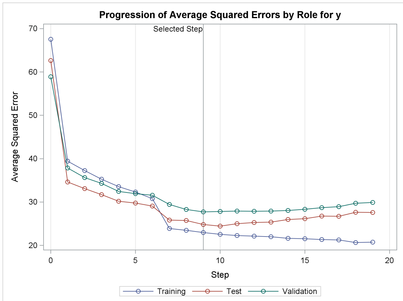
Output 47.2.6 Average Squared Errors
