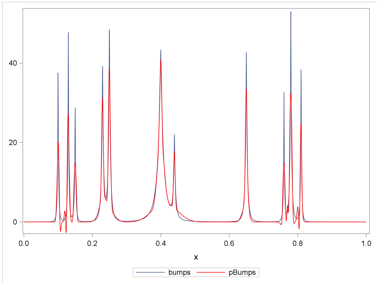
Output 47.3.9 Fit by Selecting B-splines
