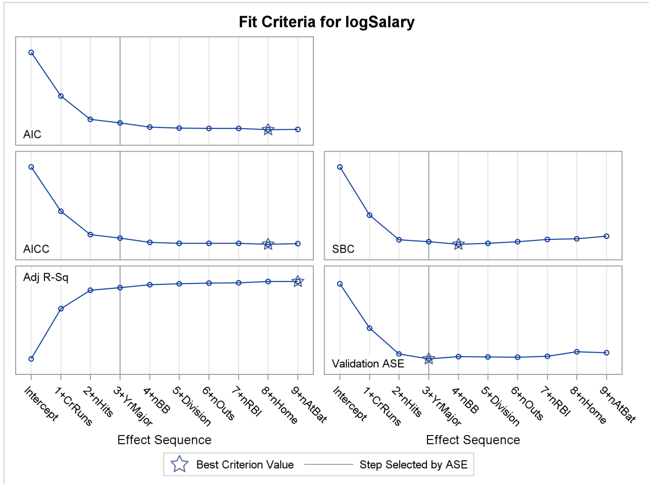
Output 47.1.8 Criterion Panel
