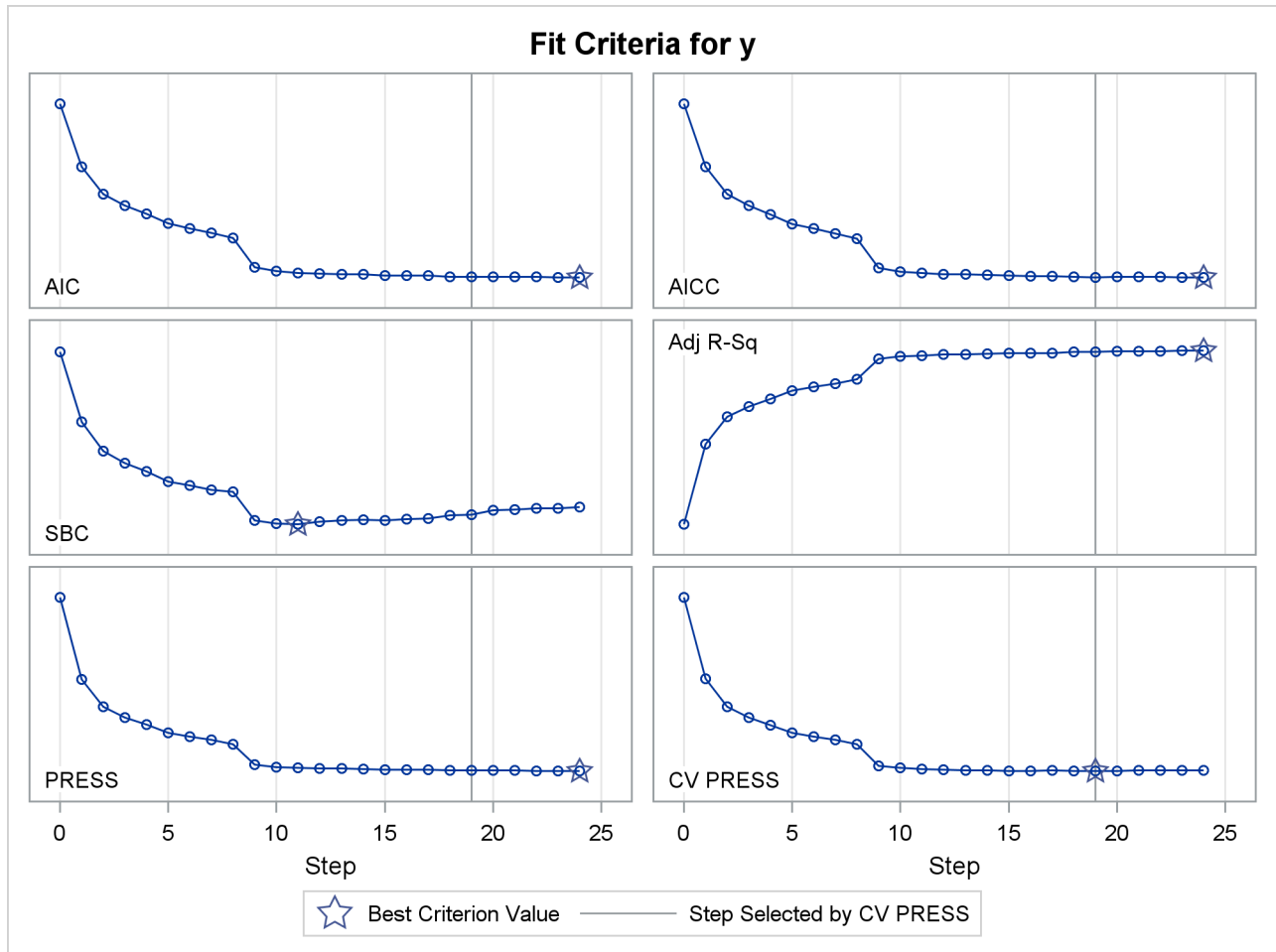
Output 47.2.13 Criterion Panel
