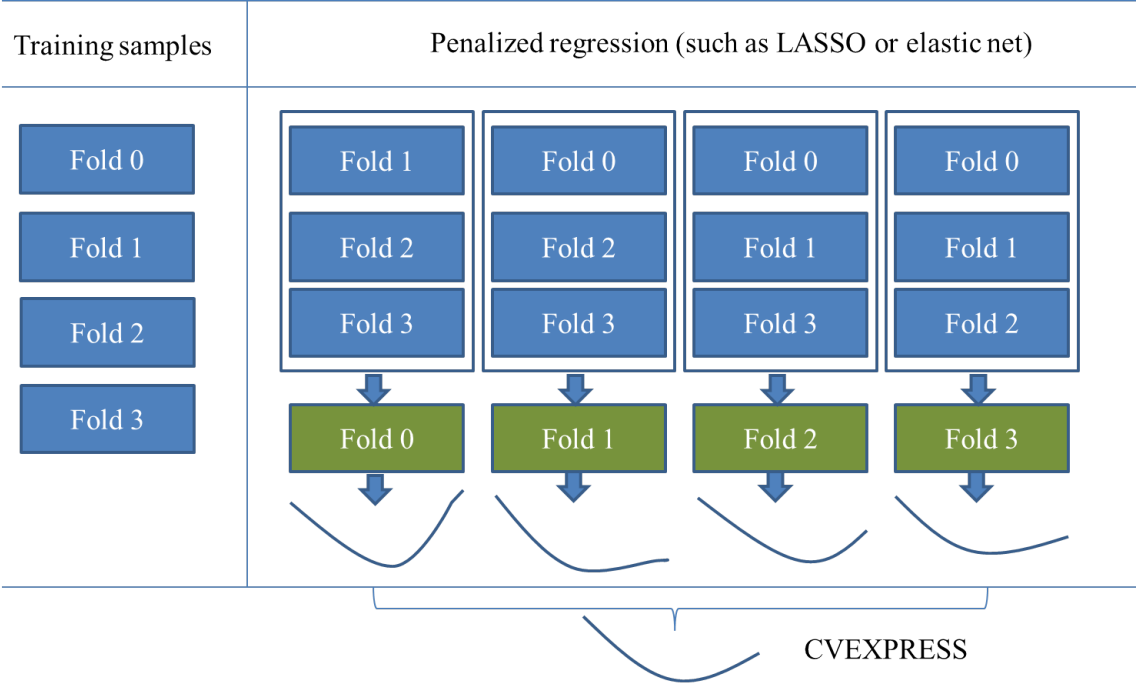
Figure 47.19 k -fold External Cross Validation
