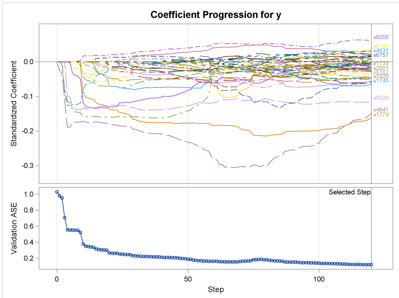
Output 47.6.8 Elastic Net Coefficient Progression Plot
