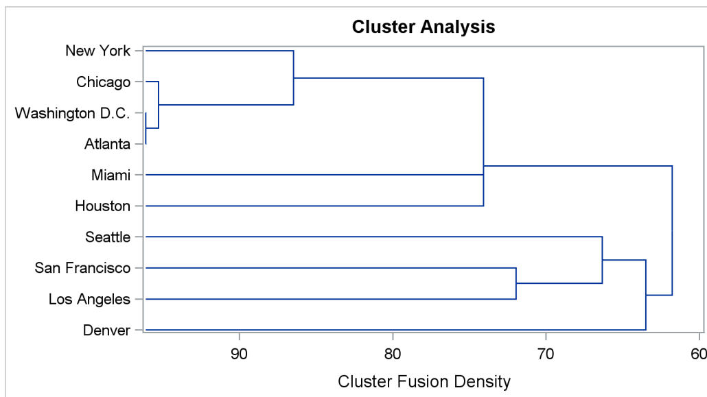
Output 33.1.7 Dendrogram Using METHOD=DENSITY K=3
