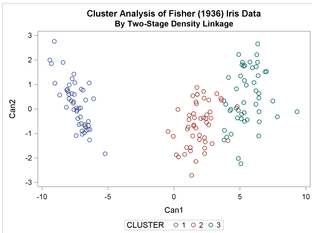
Output 33.3.8 Scatter Plot of Clusters for METHOD=TWOSTAGE
