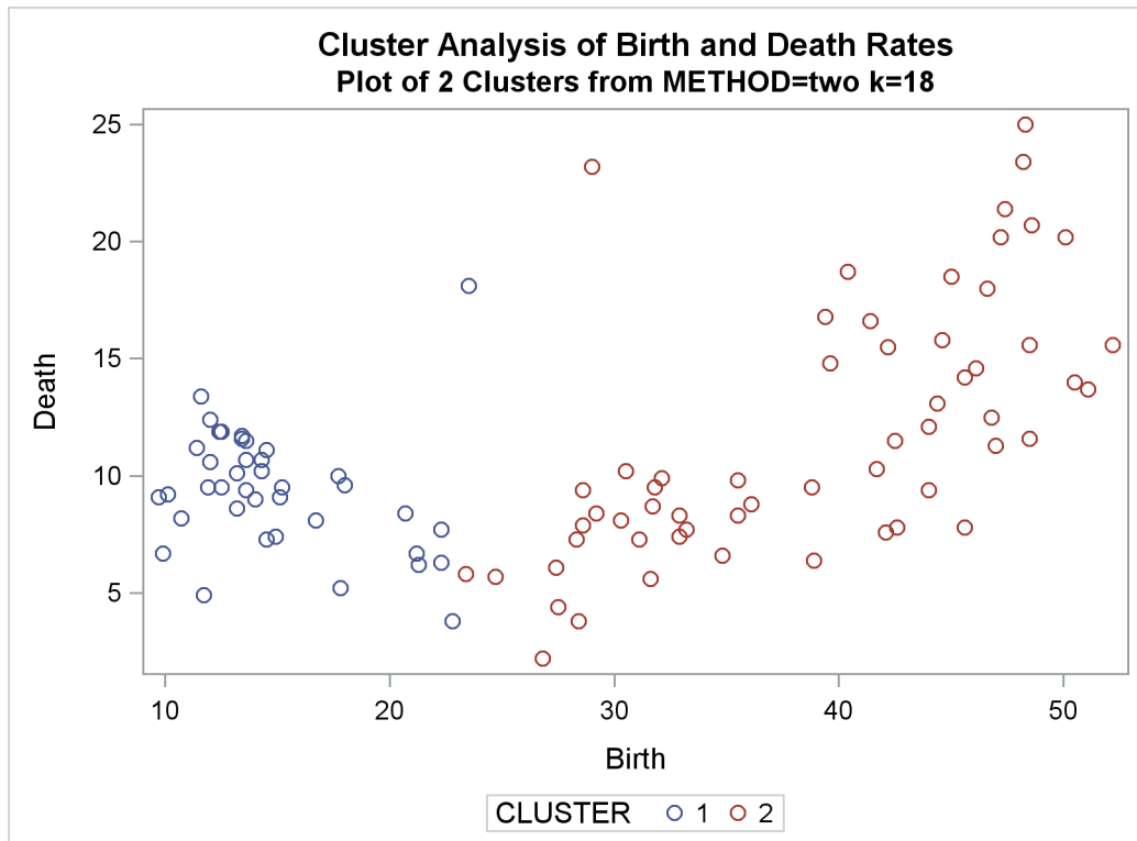
Output 33.2.14 Plot of Clusters for METHOD=TWOSTAGE K=18
