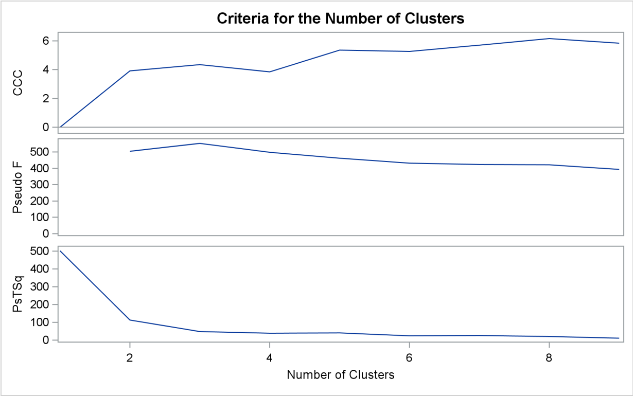
Output 33.3.12 Criteria for the Number of Clusters for Clustering Clusters from Ward's Method
