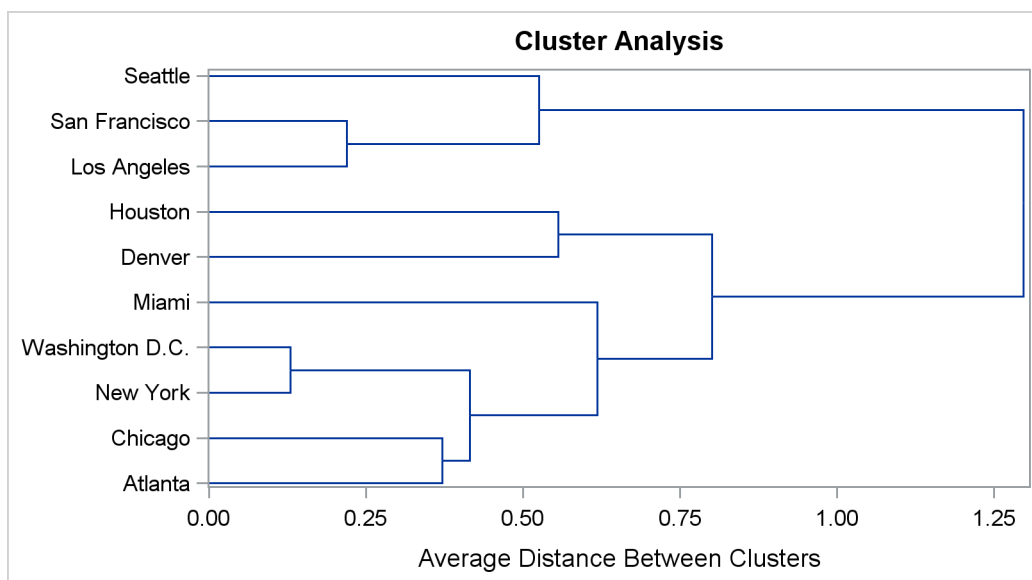
Output 33.1.3 Dendrogram Using METHOD=AVERAGE
