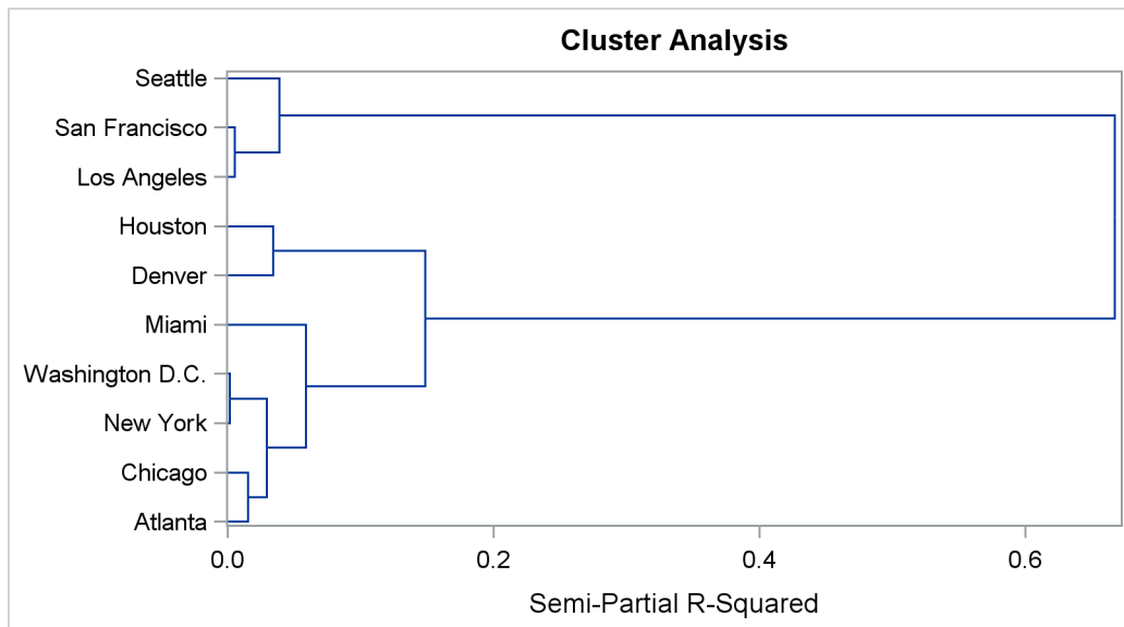
Output 33.1.13 Dendrogram Using METHOD=WARD
