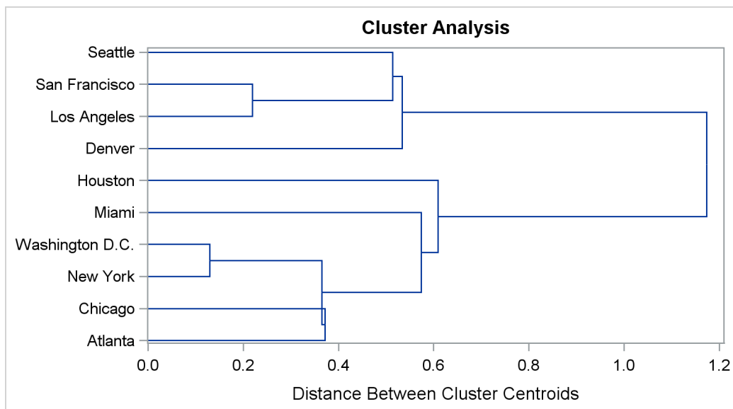
Output 33.1.5 Dendrogram Using METHOD=CENTROID
