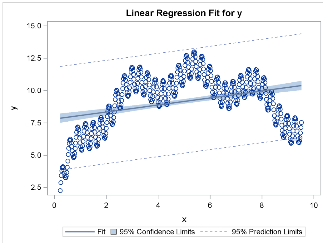
Figure 97.28 Linear Regression
