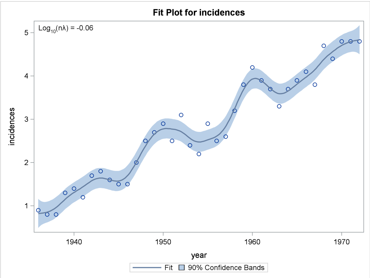
Output 96.5.2 PROC TPSPLINE Estimate and 90% Confidence Interval of Data Set MELANOMA
