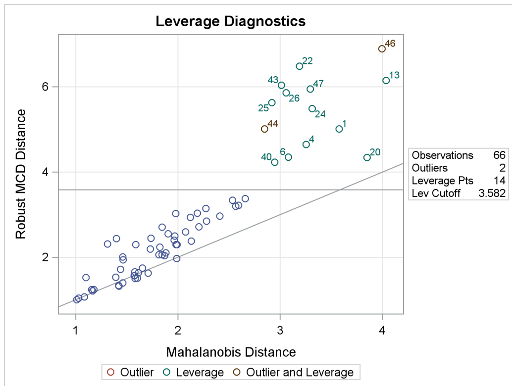
Output 80.5.10 DDPlot for the Reduced Model
