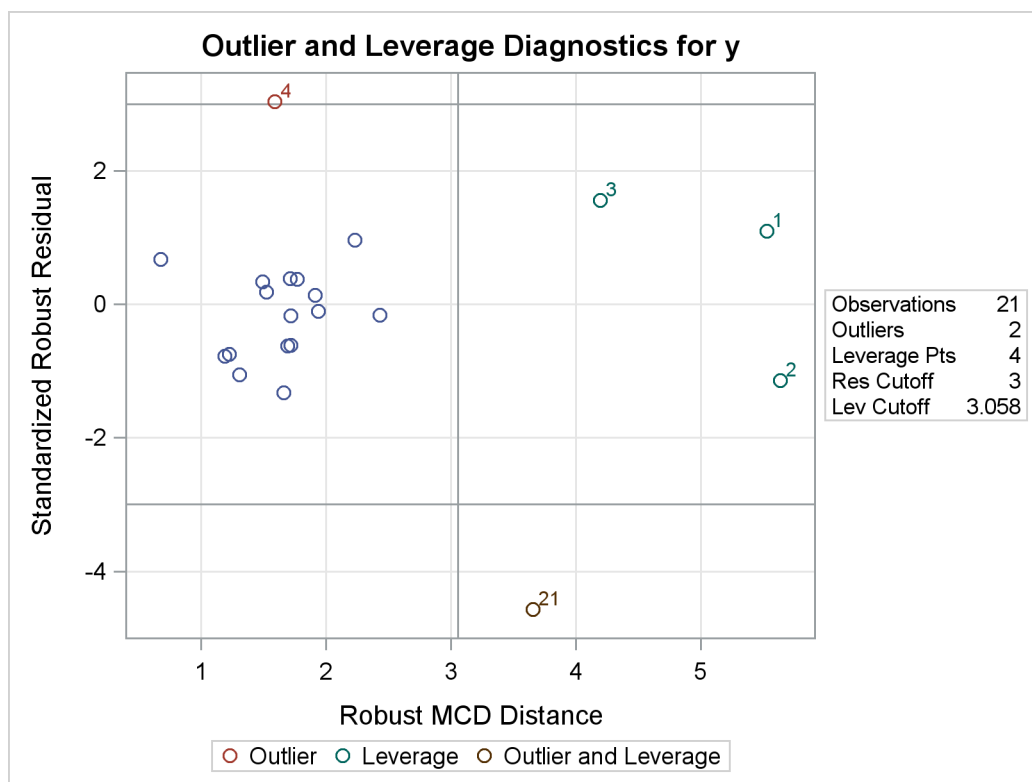
Figure 80.4 RDPLOT for Stackloss Data
