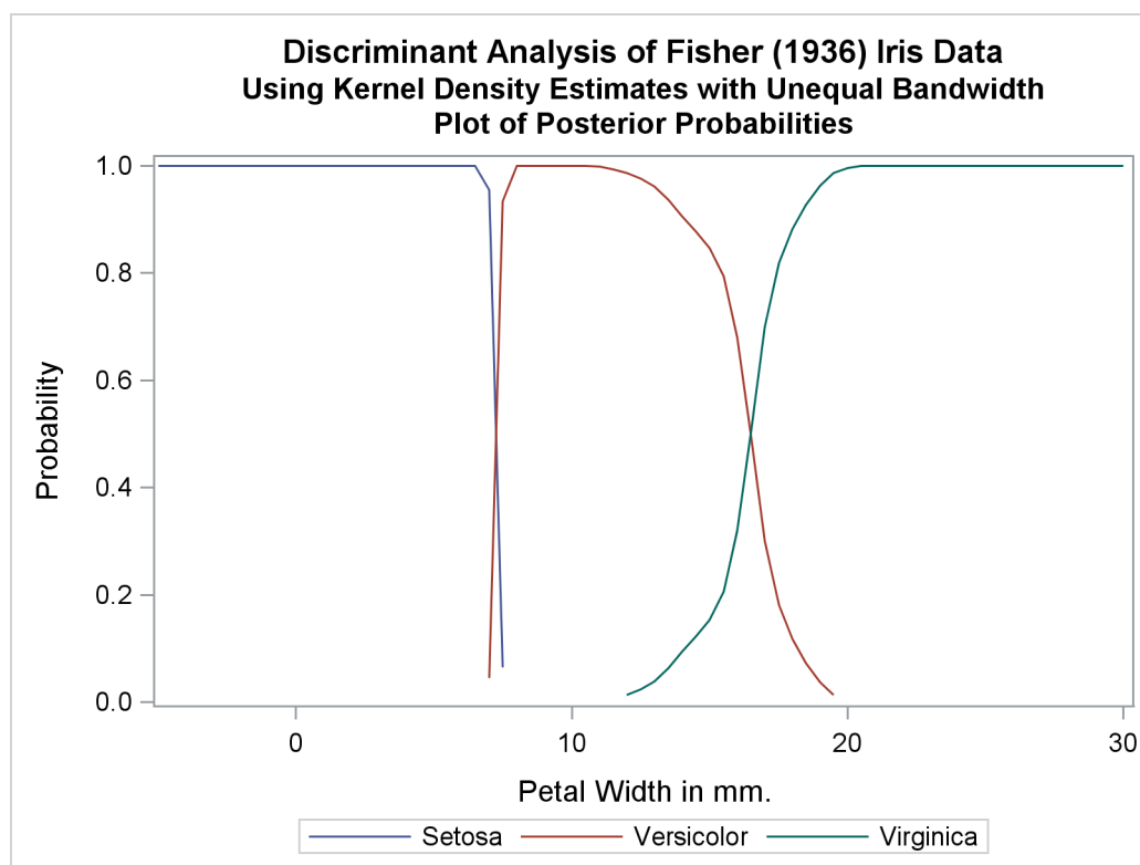
Output 33.1.5 continued
