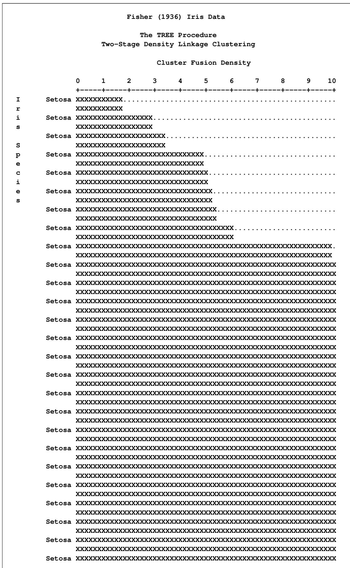
Output 98.2.2 Horizontal Tree for Fisher's Iris Data
