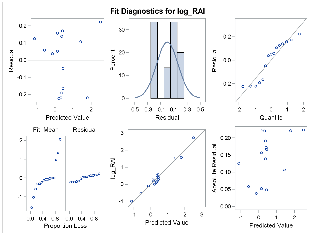
Output 70.2.1 Model Fit Diagnostics
