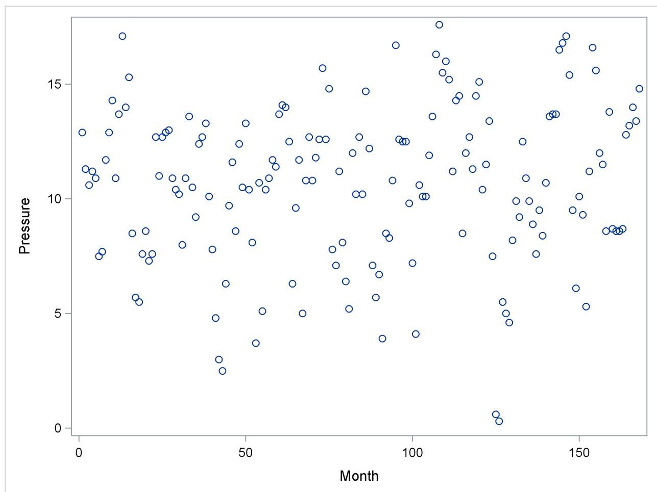
Output 53.4.1 Scatter Plot of ENSO Data
