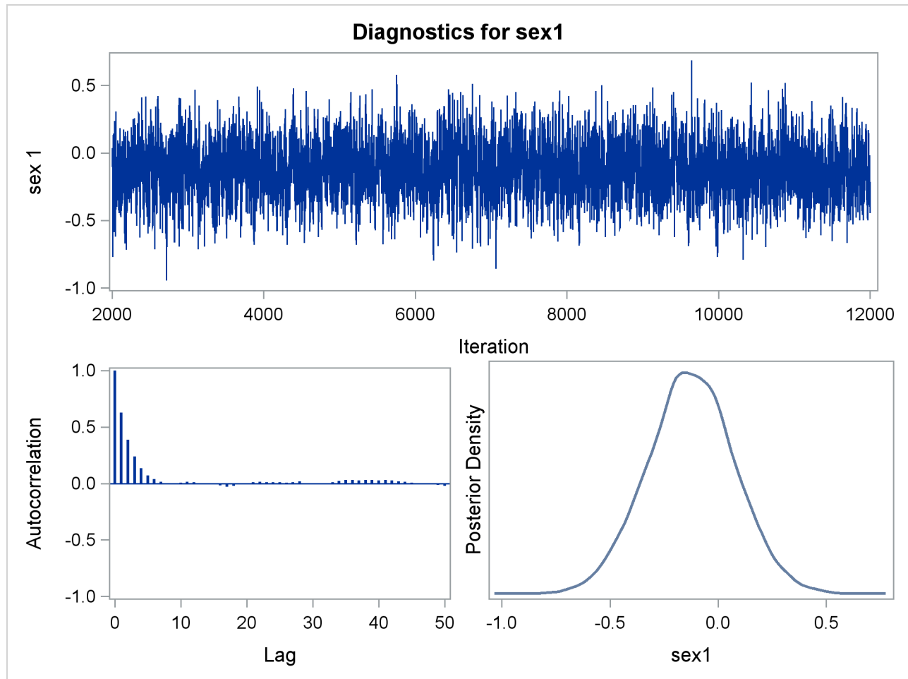
Output 51.7.8 Diagnostic Plots
