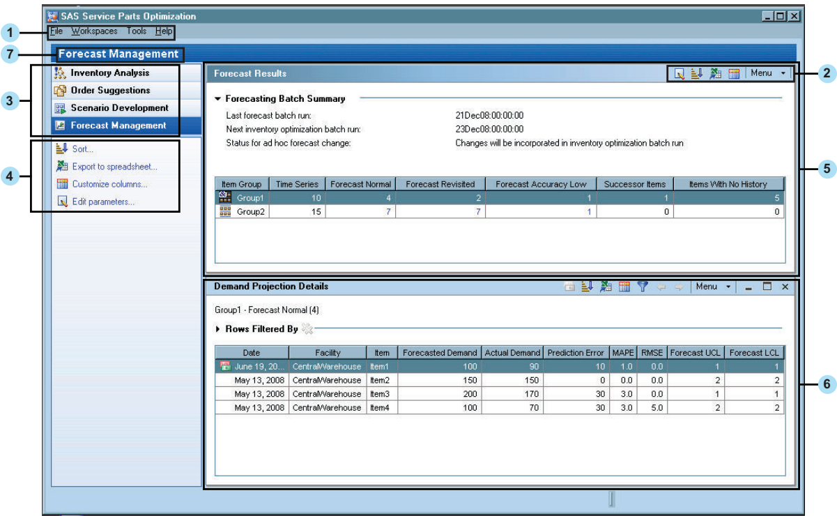
Display 3.1 SAS Service Parts Optimization User Interface
