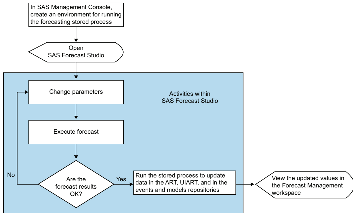
Figure 23.1 Correcting Low Accuracy Forecast Results
