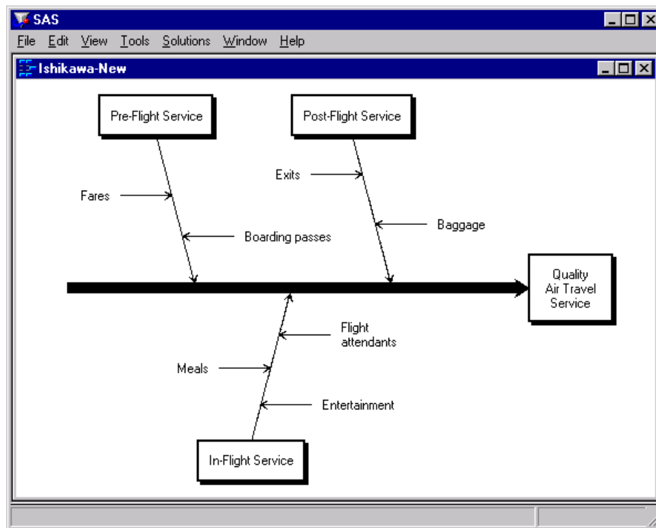
Figure 9.14 Stem-Level Diagram
