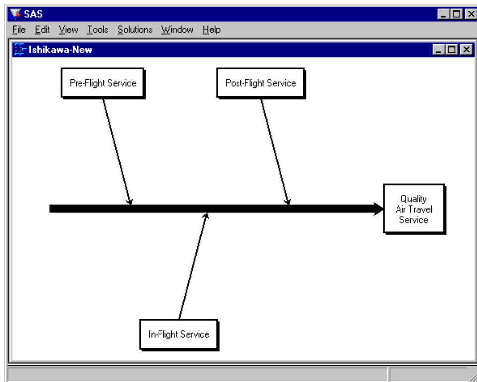
Figure 9.46 Branch-Level Diagram
