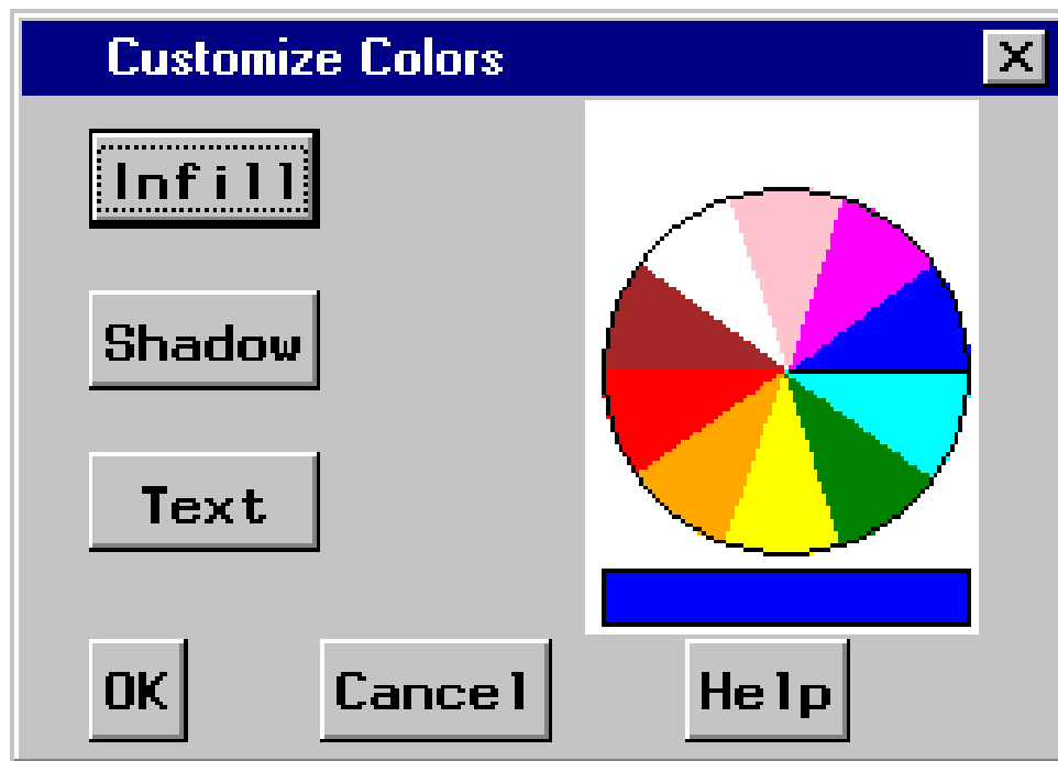
Figure 9.73 Colors Dialog
