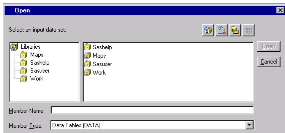
Figure 9.54 Member Selector
