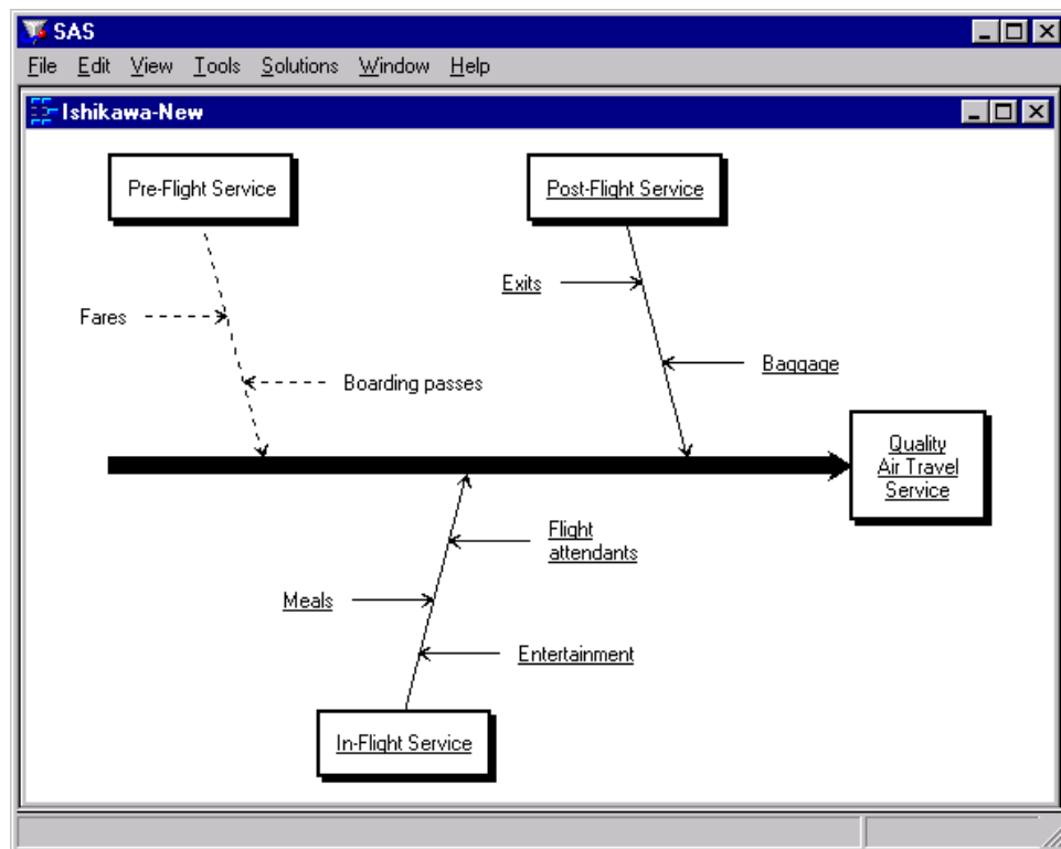
Figure 9.72 Modified Diagram
