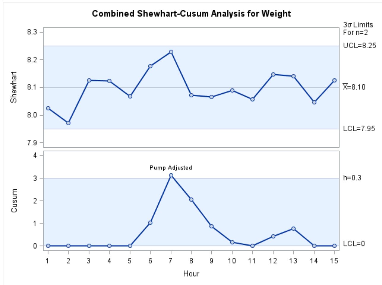
Output 7.3.1 Combined Shewhart–Cusum Scheme
