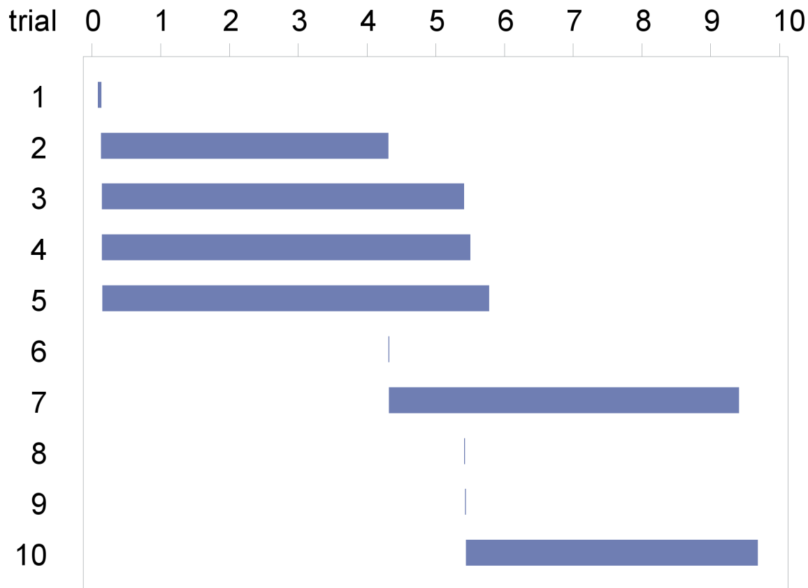
Figure 5.8 Overlapped COFOR Iterations
