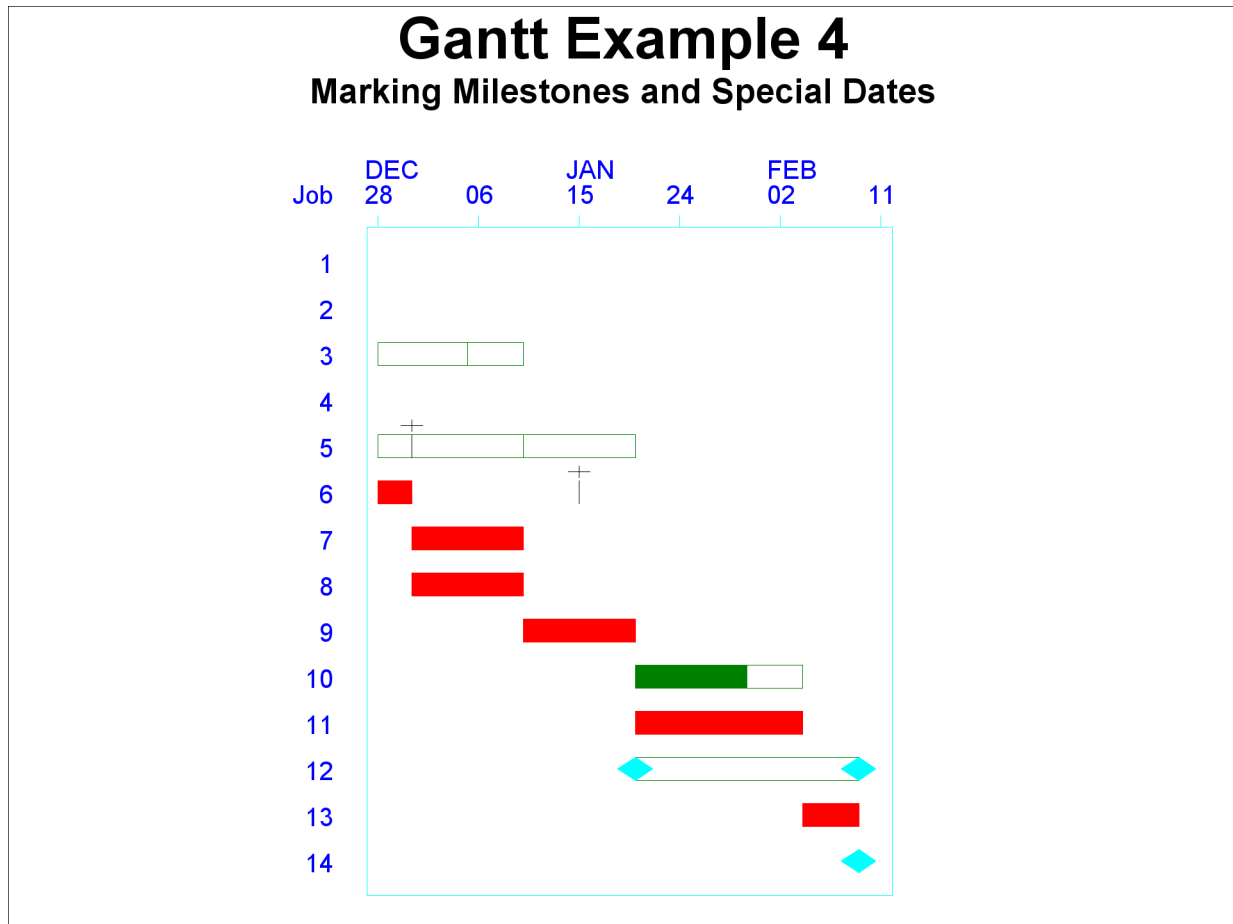
Output 8.4.1 continued
