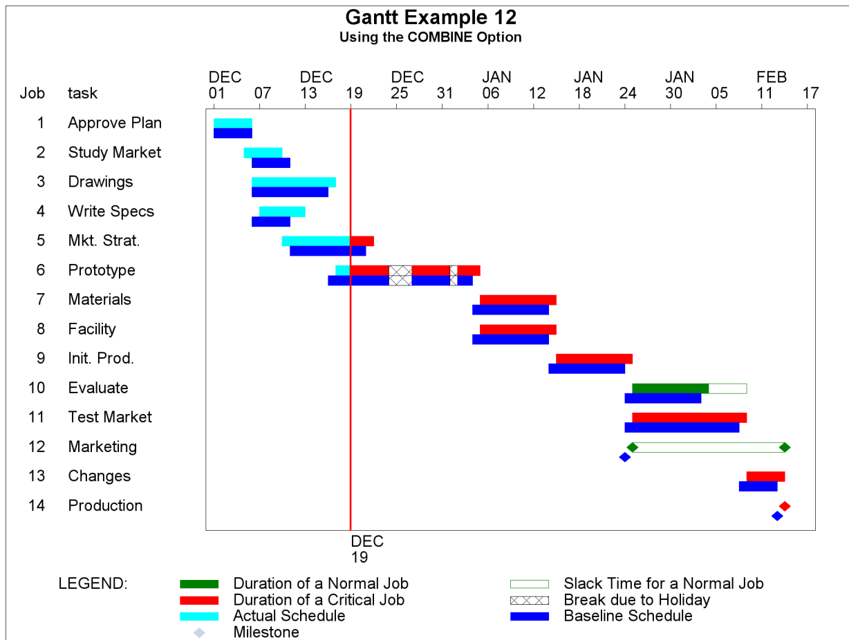
Output 8.12.1 Using the COMBINE Option in Graphics Mode
