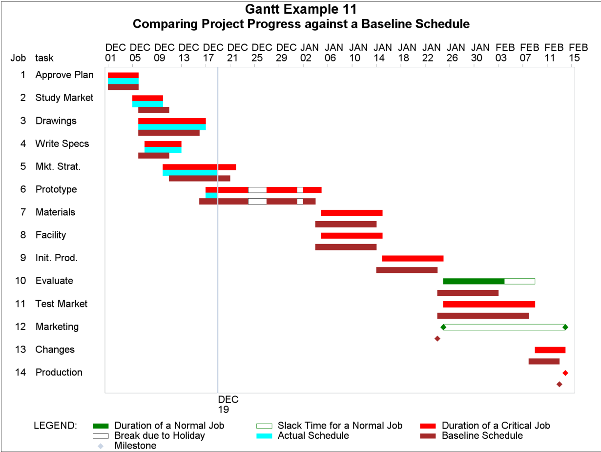
Output 8.11.2 Comparing Project Progress Against a Baseline Schedule
