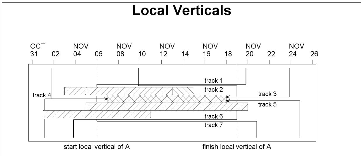
Figure 8.12 Local Verticals
