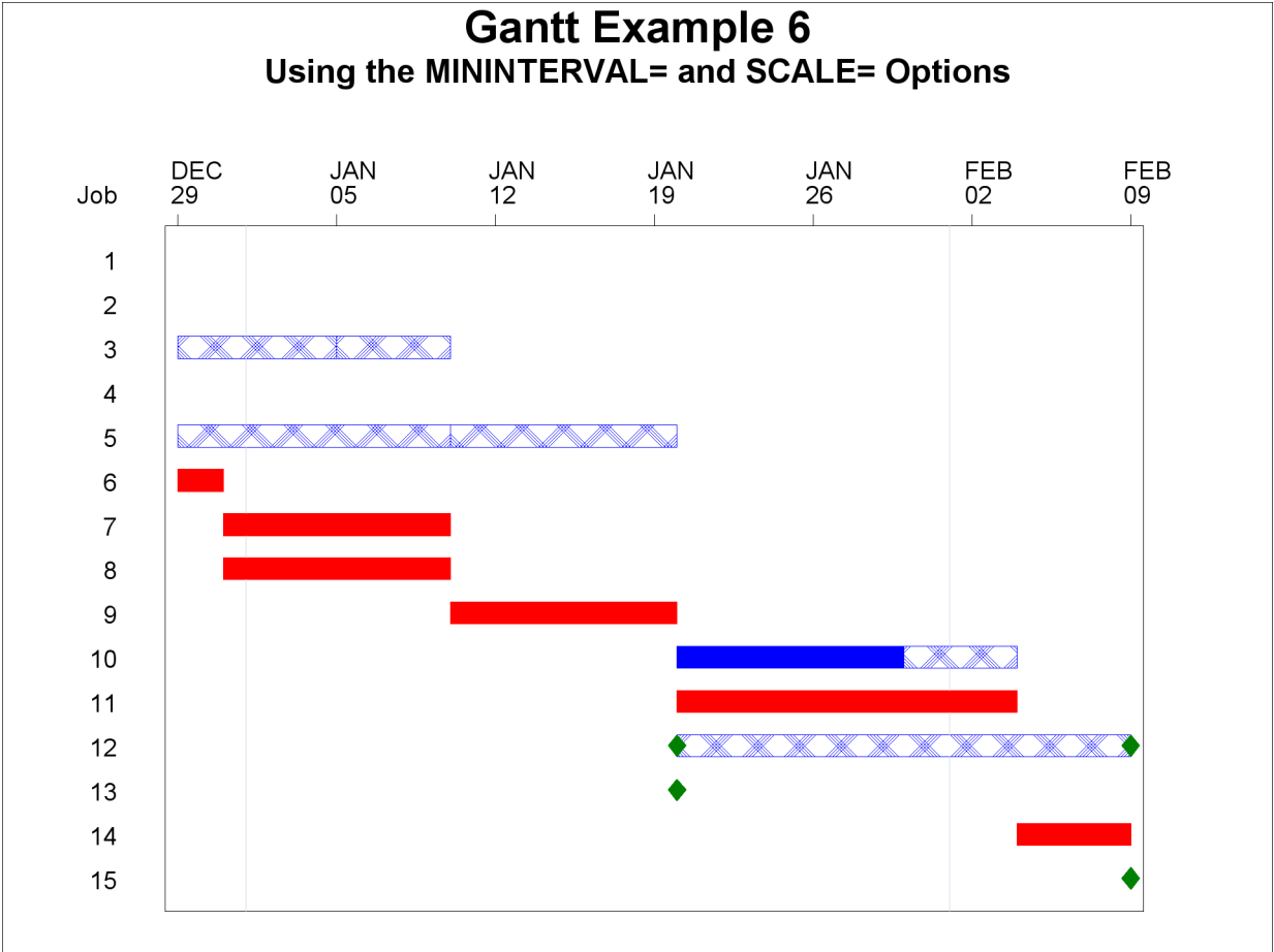
Output 8.6.2 continued
