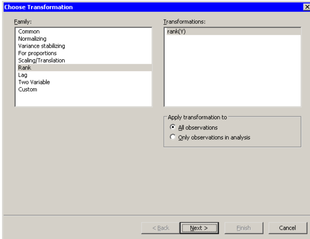
Figure 32.16 Rank Transformations
