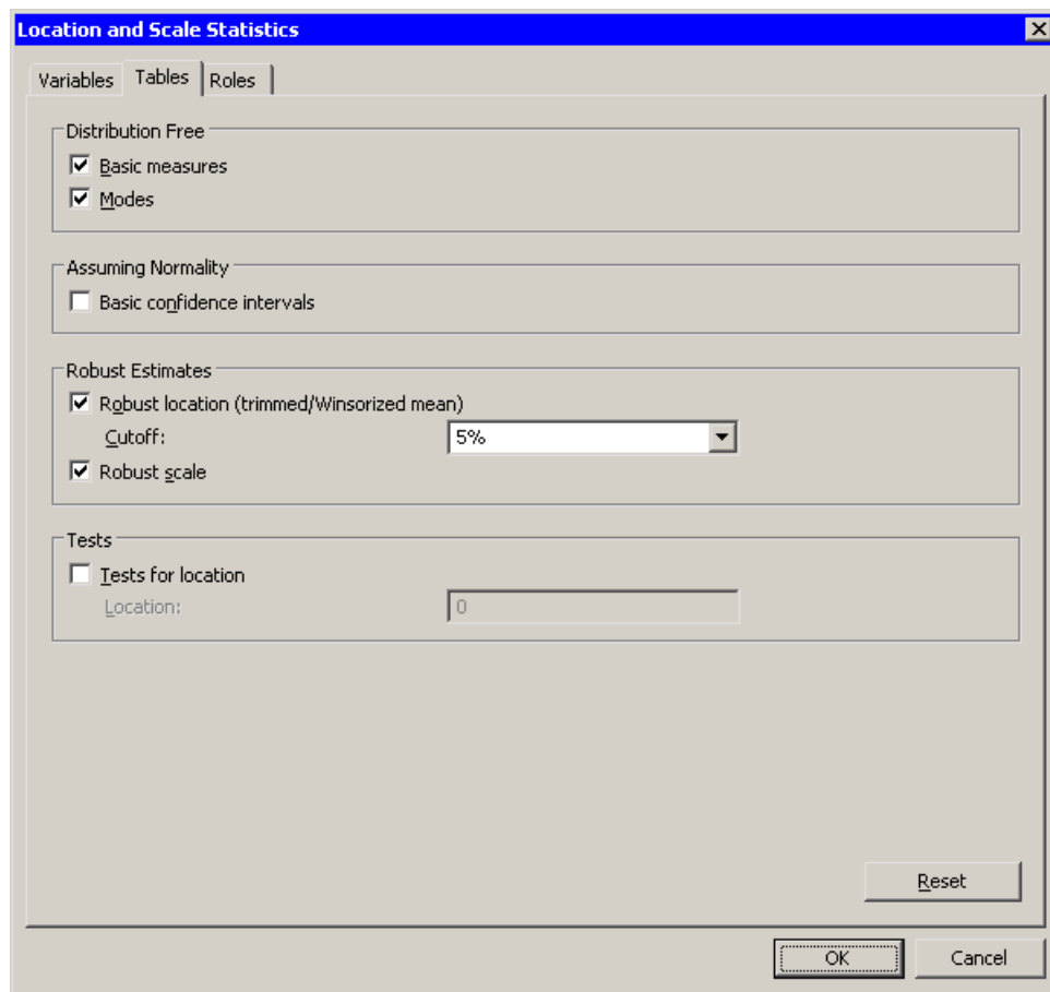
Figure 14.4 Selecting Tables
