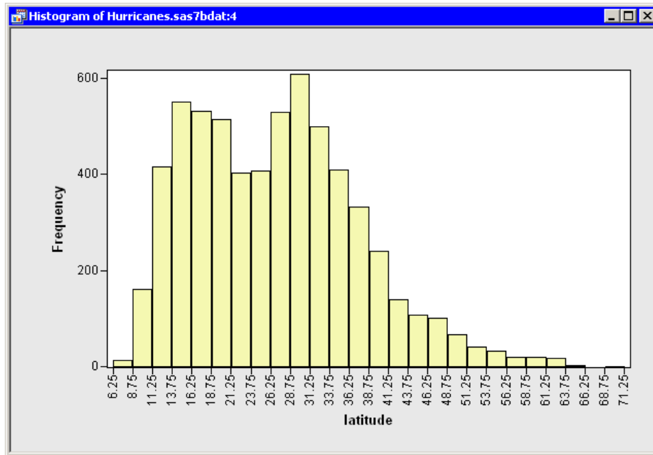
Figure 5.7 A Histogram
