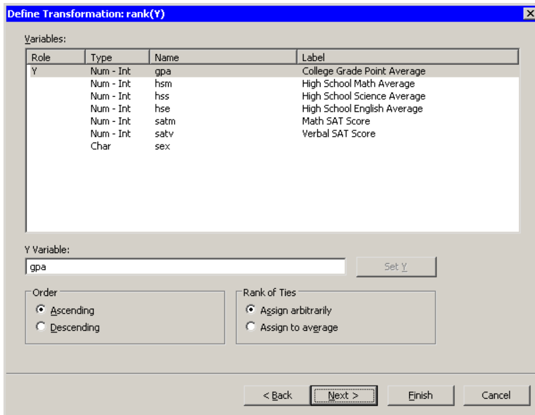
Figure 32.17 Rank Transformations
