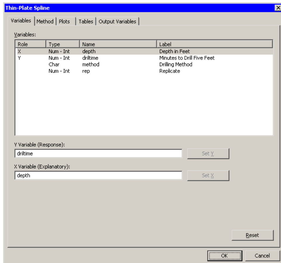
Figure 19.2 Selecting Variables
