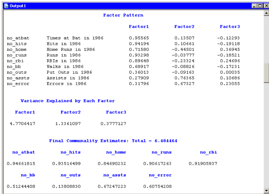
Figure 27.10 Unrotated Factors
