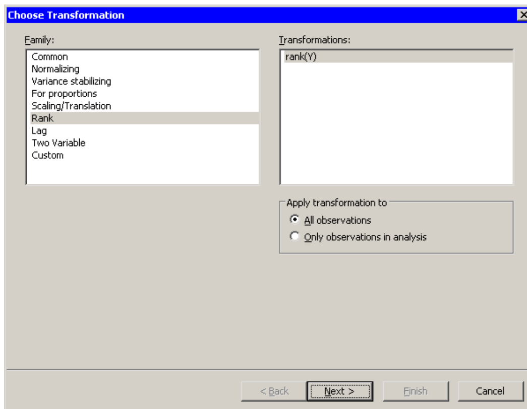
Figure 32.16 Rank Transformations
