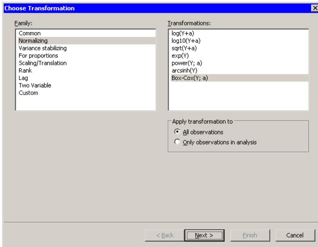
Figure 32.12 Normalizing Transformations
