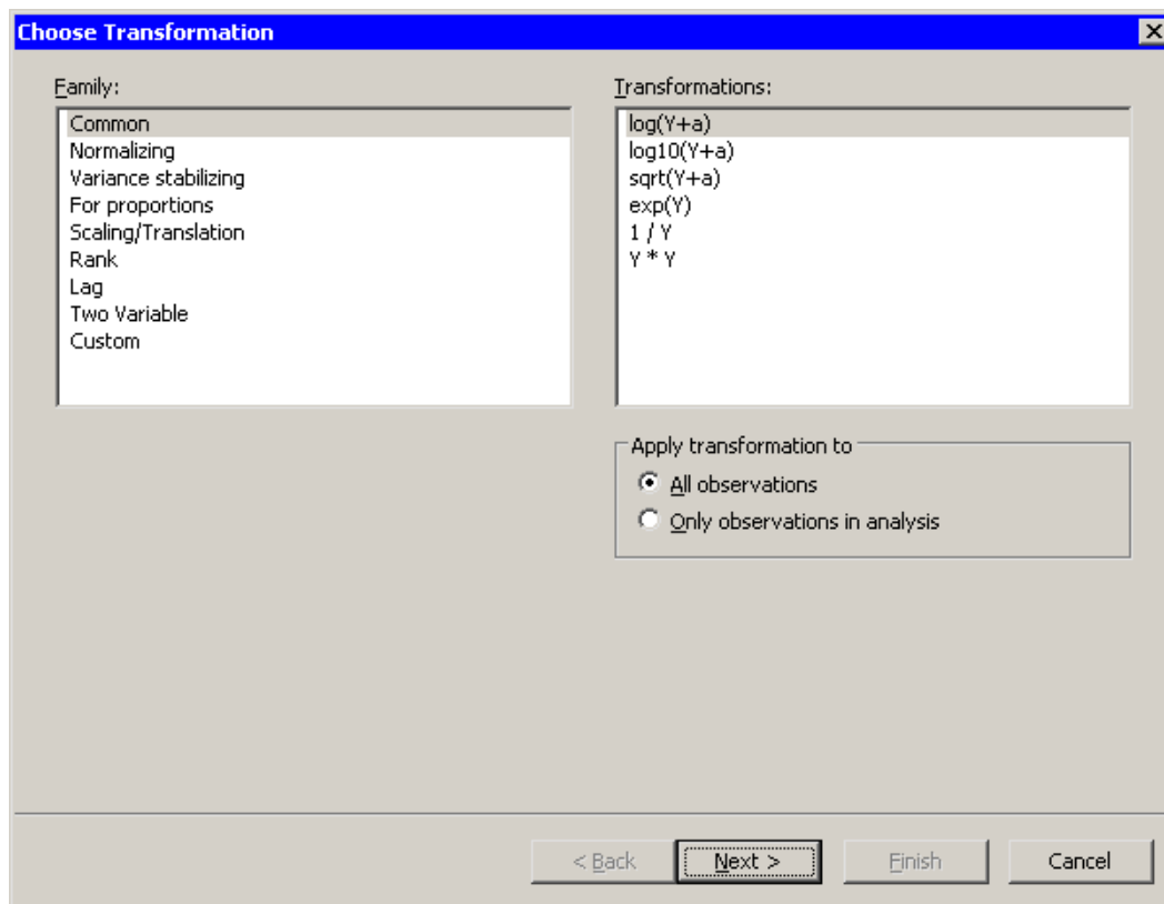
Figure 32.11 Common Transformations
