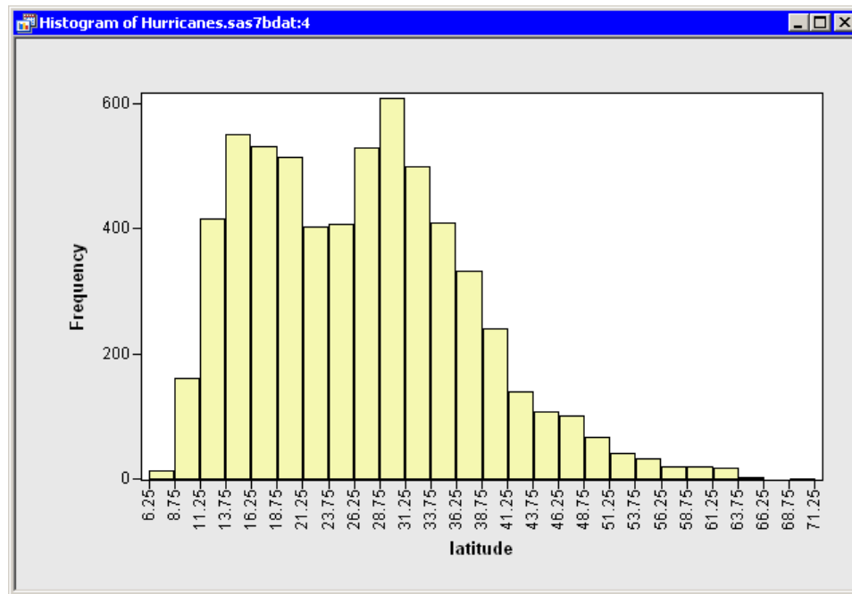
Figure 5.7 A Histogram
