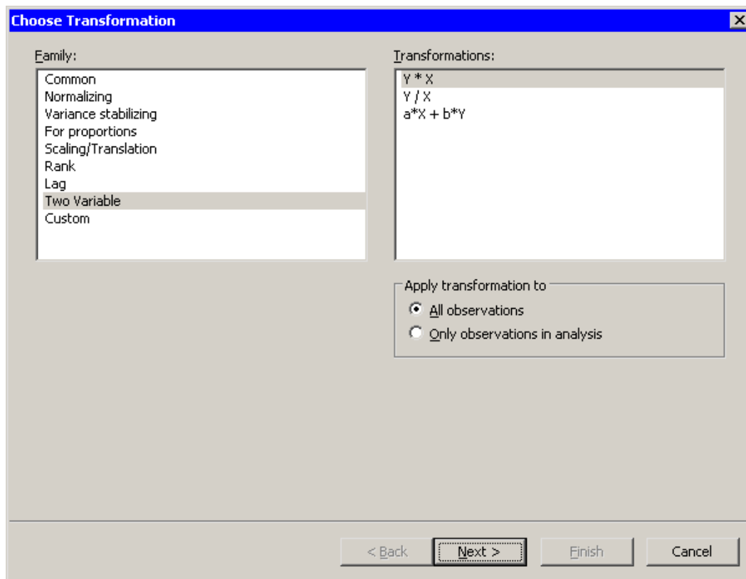
Figure 32.20 Two-Variable Transformations
