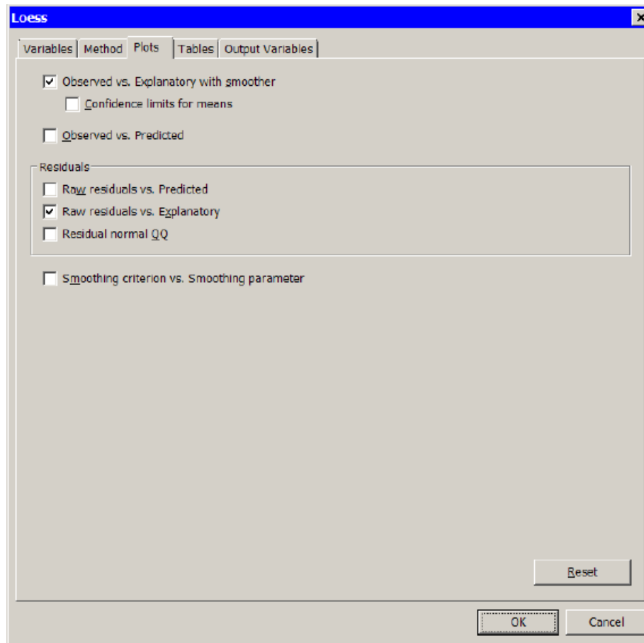
Figure 18.4 Selecting Plots
