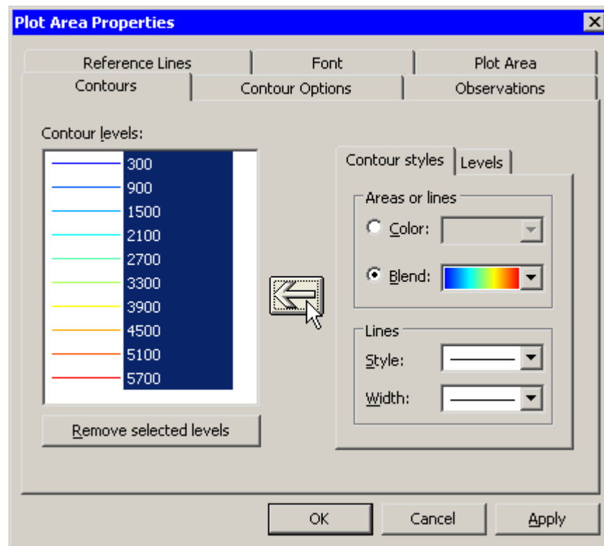
Figure 7.21 Coloring Contours
