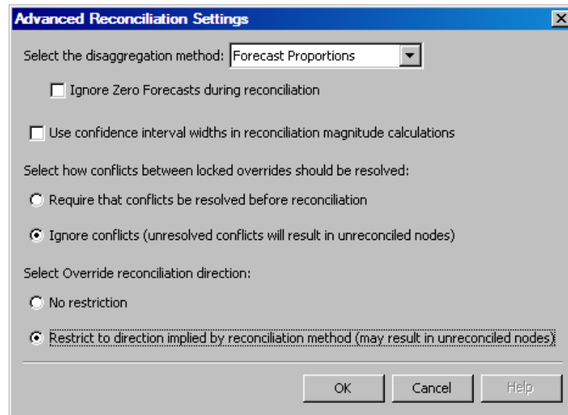
Display 14.5 Advanced Reconciliation Settings Dialog Box
