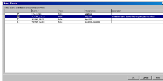
Display 12.7 Select the Events
