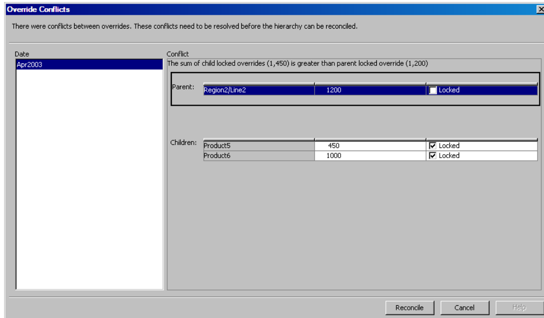
Display 14.3 Reconciling the Apr2003 Node By Using the Override Conflicts Dialog Box
