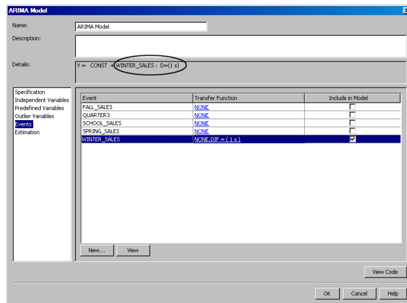
Display 12.11 Event in the ARIMA Model Specification
