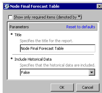
Display 11.2 Example of a Prompt Dialog Box
