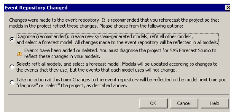
Display 12.9 Event Repository Changed Dialog Box
