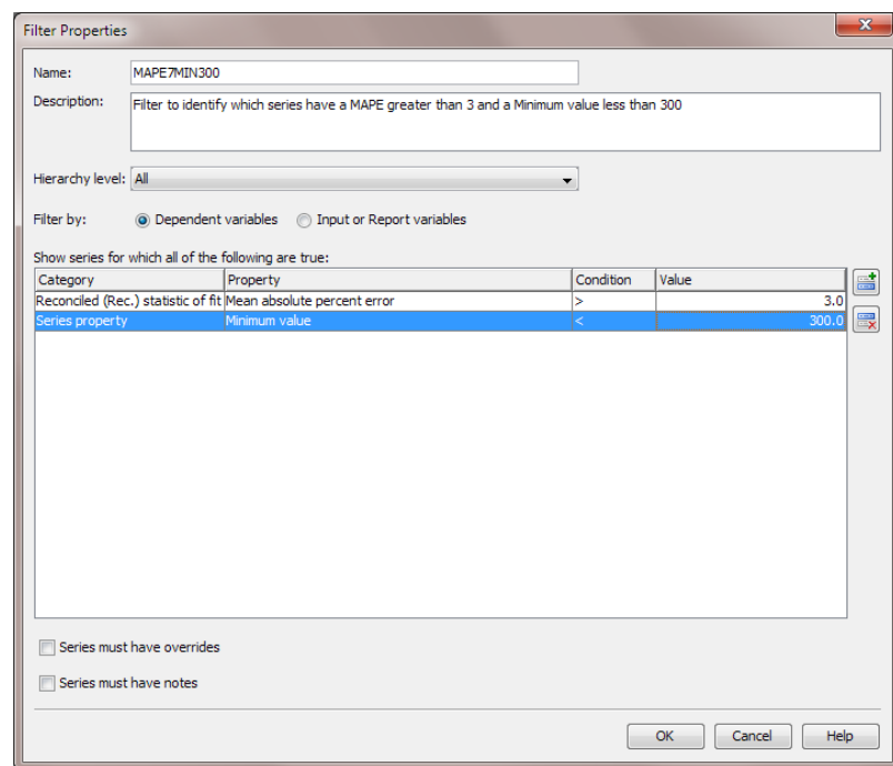
Display 10.4 Completed Filter Properties Dialog Box for Filter Example
