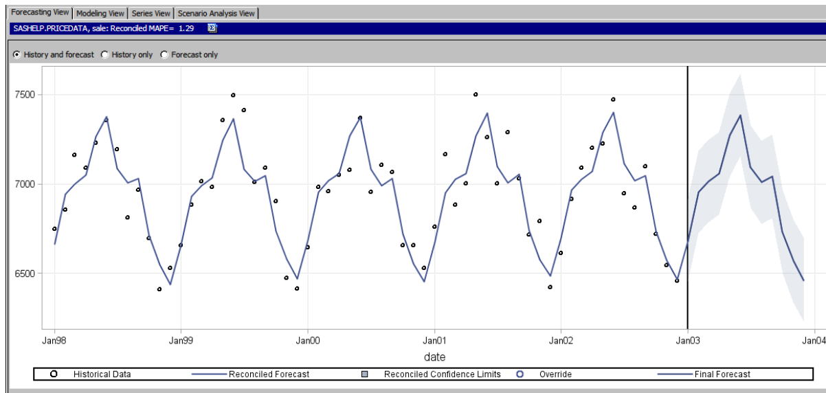
Display 6.4 Forecast Values When Cost Is an Independent Variable
