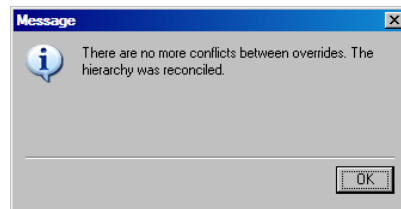
Display 14.4 Message about Hierarchy Reconciliation
