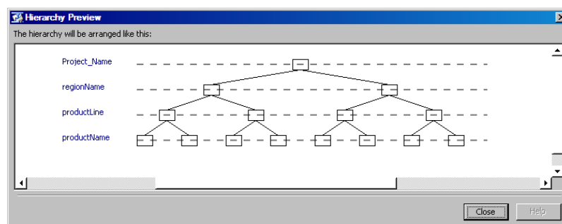
Display 7.1 Example of Hierarchy
