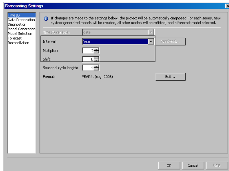
Display 6.1 Specifying June as the Beginning of the Year for Two Years
