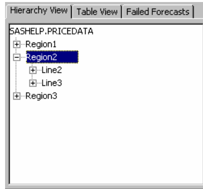
Display 18.1 Region2 in the Hierarchy
