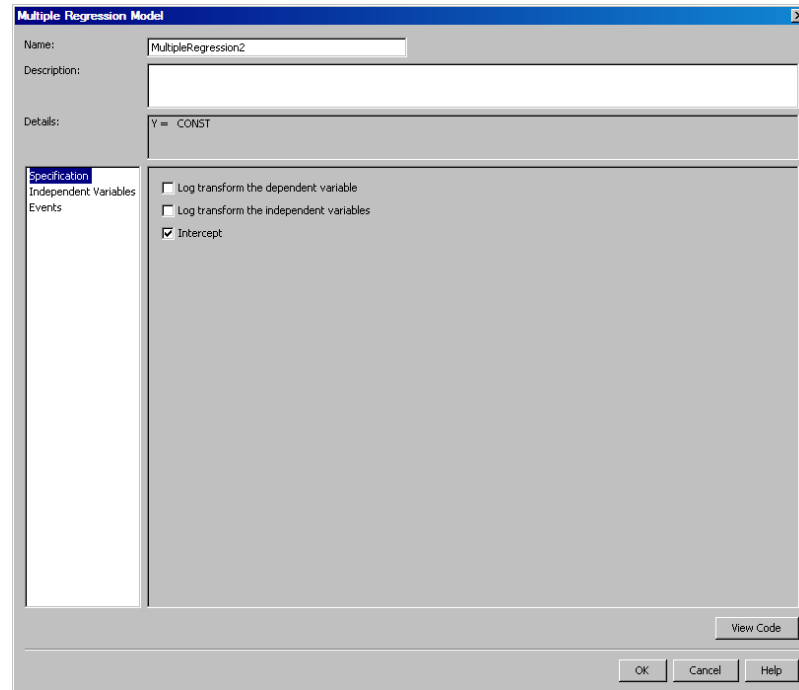
Display 17.6 Multiple Regression Model Dialog Box
