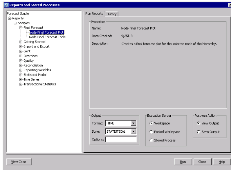
Display 11.1 Selected Report in Reports and Stored Processes Dialog Box
